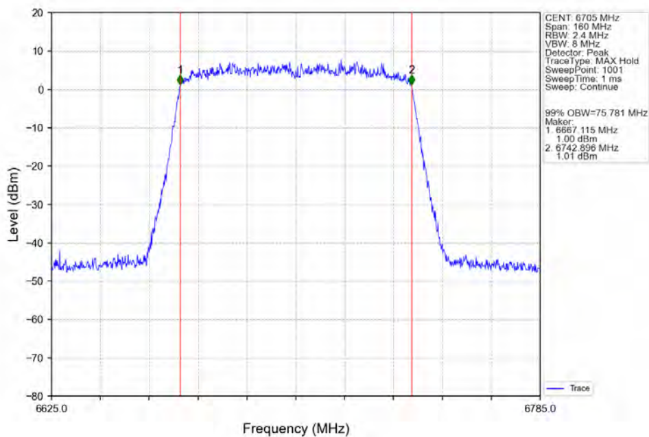
802.11ac(VHT80)_MCH_6705MHz_Ant2_NTNV
