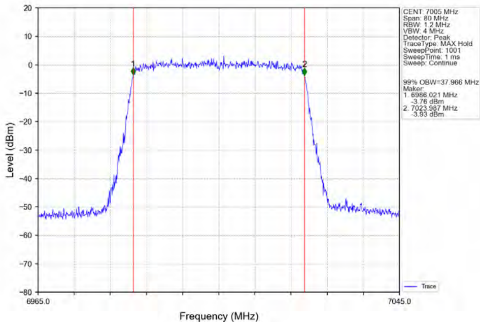
802.11ax(HEW40)_MCH_7005MHz_SU / Ant2_NTNV
