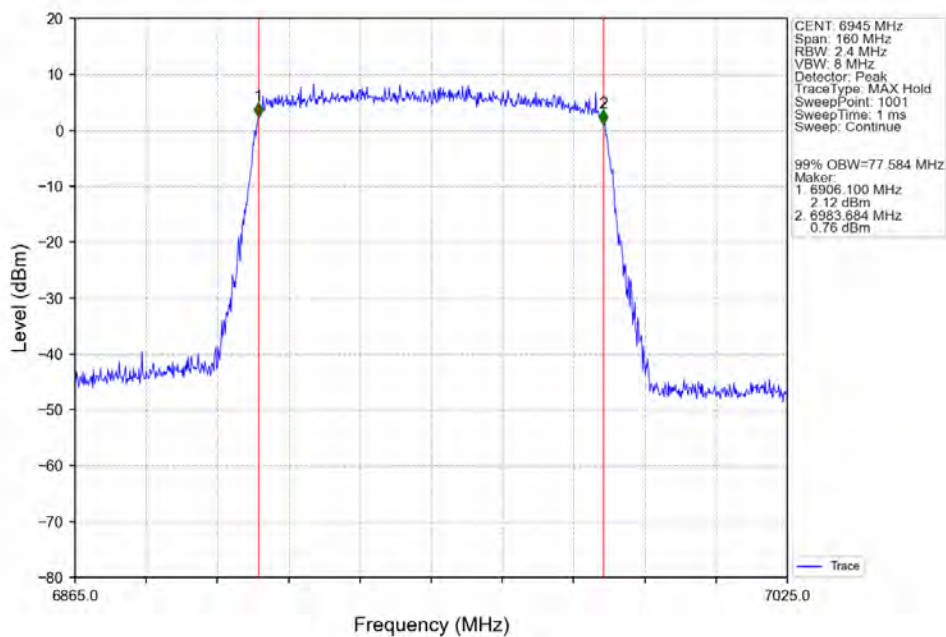
802.11ax(HEW80)_LCH_6945MHz_SU / Ant2_NTNV
