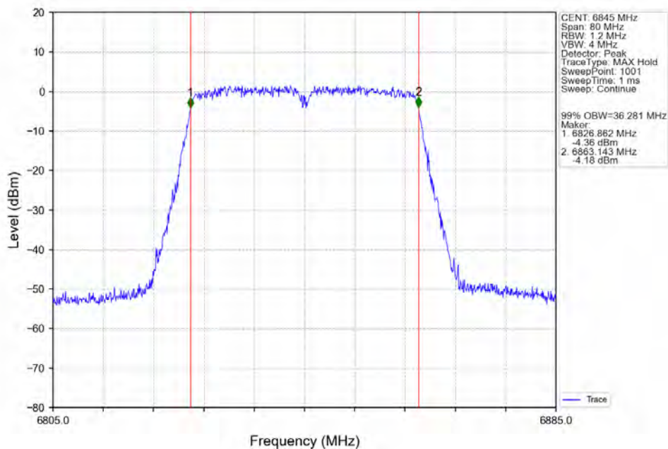
802.11n(HT40) HCH 6845MHz Ant2 NTN
