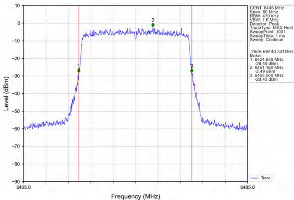
802.11ax(HEW40)_LCH_6445MHz_SU / Ant2_NTNV
