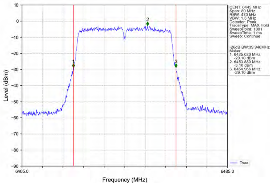
802.11n(HT40) LCH 6445MHz Ant2 NTN
