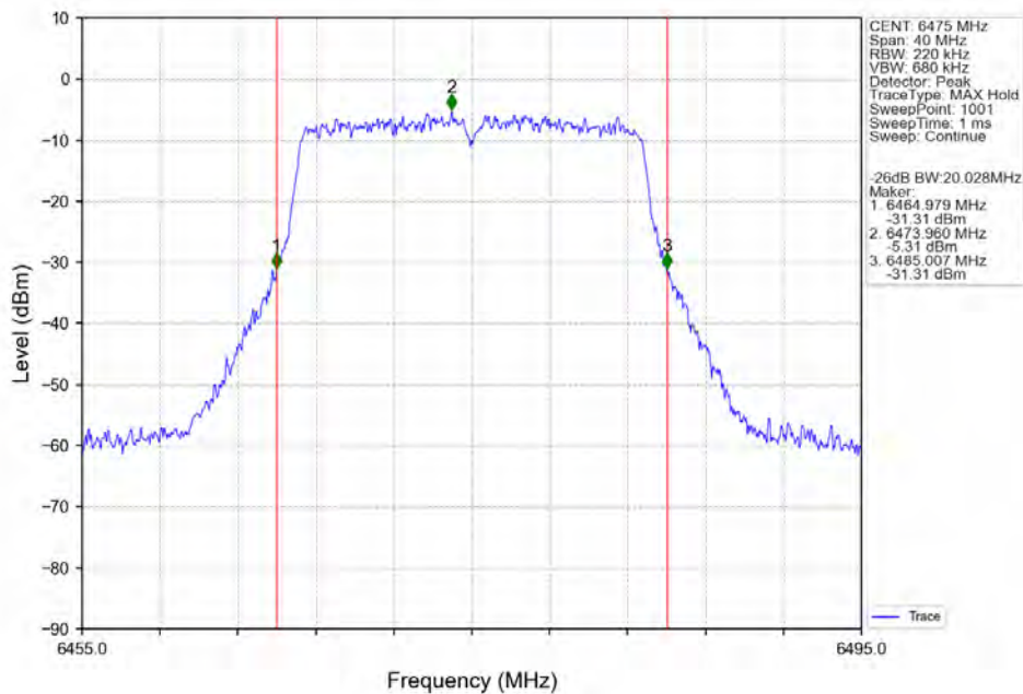
802.11ac(VHT20)_MCH_6475MHz_Ant2_NTNV
