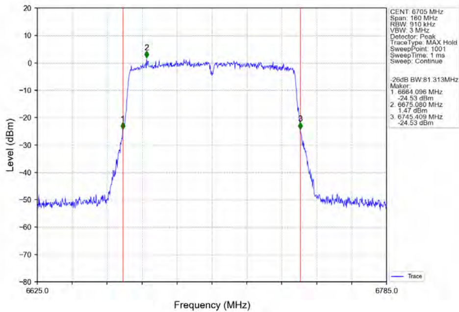
802.11ac(VHT80)_MCH_6705MHz_Ant2_NTNV
