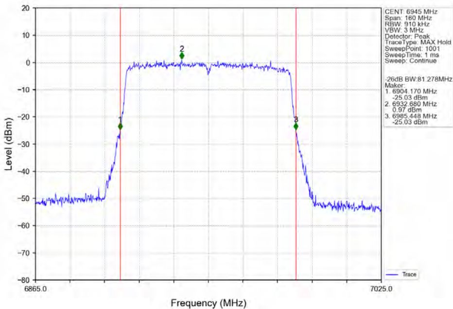
802.11ac(VHT80) LCH 6945MHz Ant2 NTN
