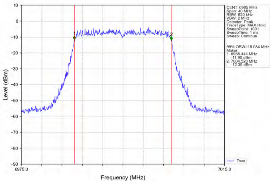
802.11ax(HEW20)_MCH_6995MHz_SU / Ant2_NTNV
