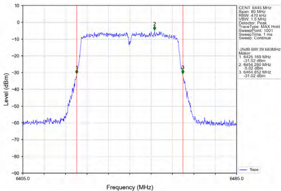
802.11ac(VHT40) LCH_6445MHz_Ant2_NTNV
