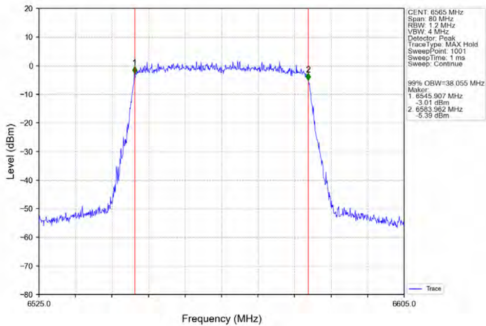
802.11ax(HEW40)_LCH_6565MHz_SU / Ant2_NTNV
