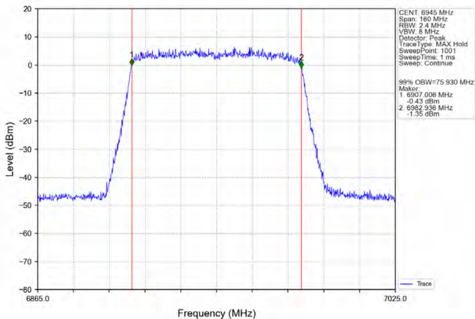
802.11ac(VHT80) LCH_6945MHz_Ant2_NTNV
