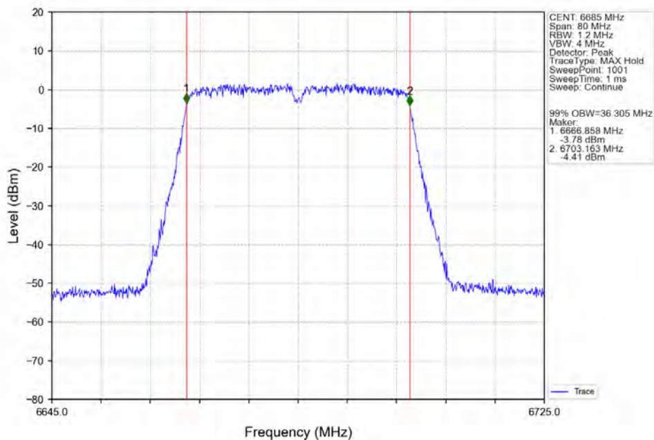
802.11ac(VHT40)_MCH_6685MHz_Ant2_NTNV
