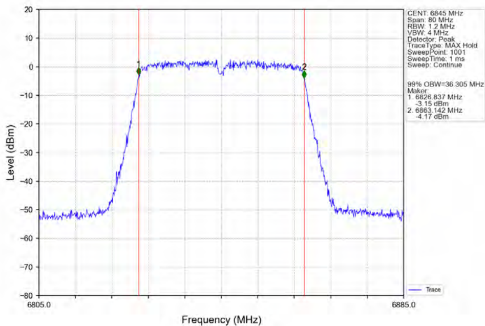
802.11ac(VHT40) HCH 6845MHz Ant2 NTN
