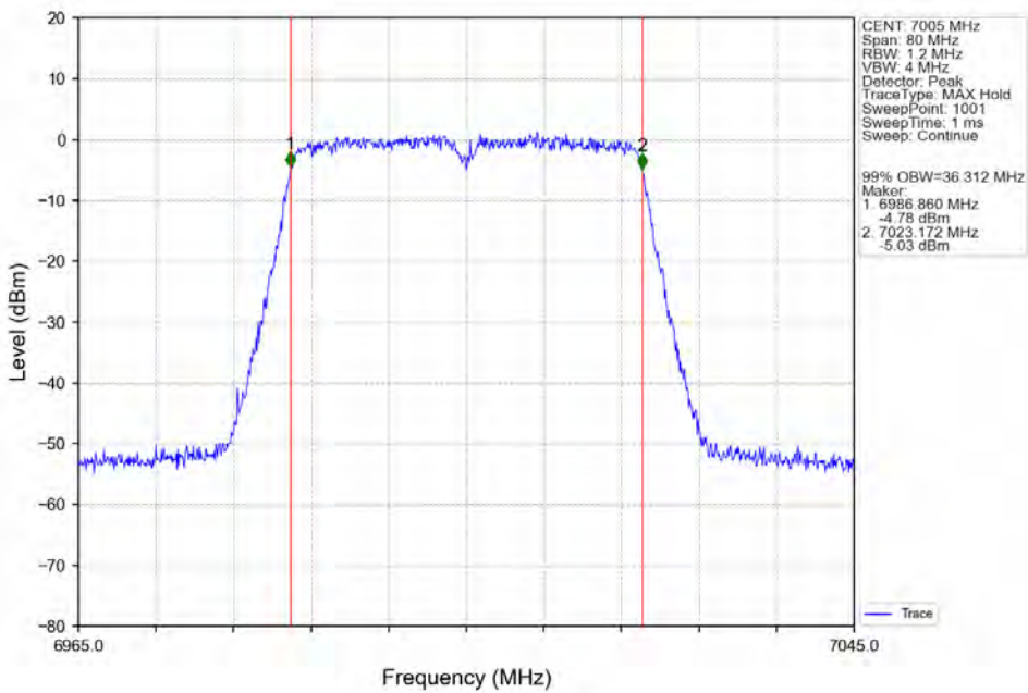
802.11ac(VHT40)_MCH_7005MHz_Ant2_NTNV
