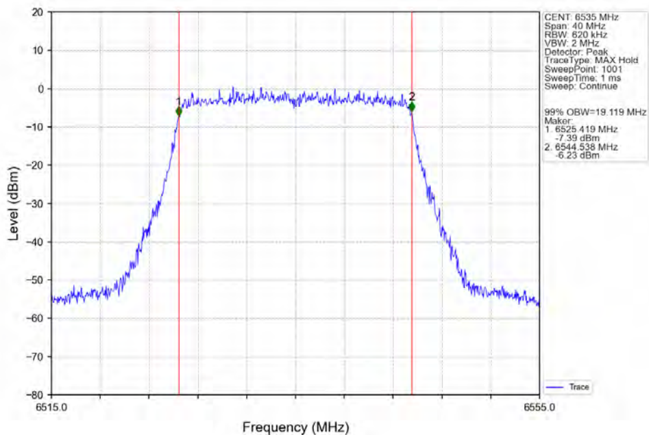
802.11ax(HEW20)_LCH_6535MHz_SU / Ant2_NTNV
