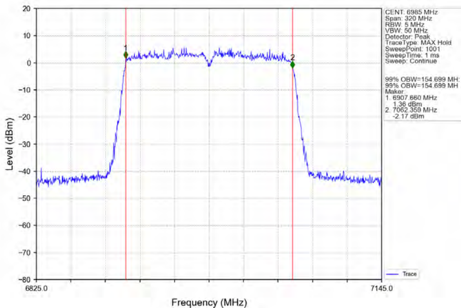
802.11ac(VHT160) MCH_6985MHz_Ant2_NTNV
