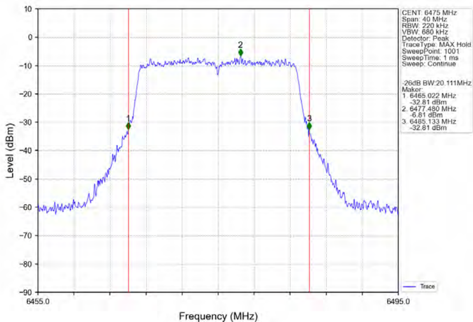
802.11n(HT20)_MCH_6475MHz_Ant2_NTNV
