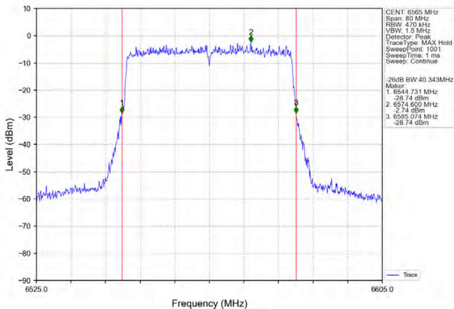
802.11ax(HEW40)_LCH_6565MHz_SU / Ant2_NTNV
