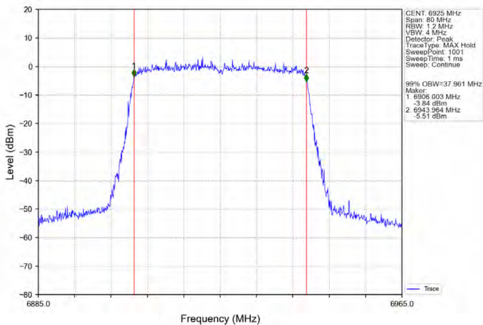
802.11ax(HEW40)_LCH_6925MHz_SU / Ant2_NTNV
