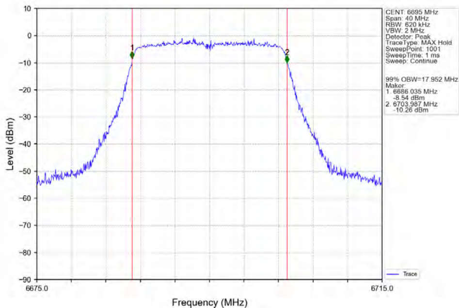
802.11ac(VHT20)_MCH_6695MHz_Ant2_NTNV
