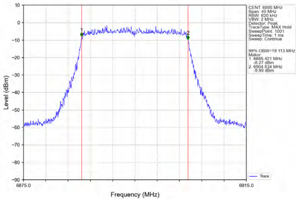
802.11ax(HEW20)_LCH_6895MHz_SU / Ant2_NTNV
