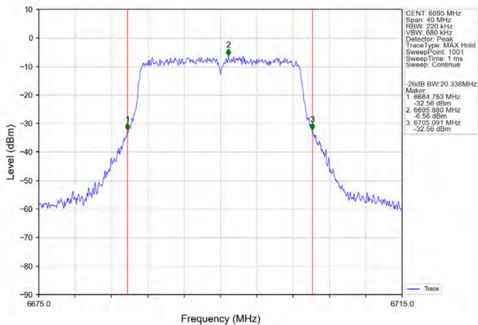
802.11ac(VHT20)_MCH_6695MHz_Ant2_NTNV
