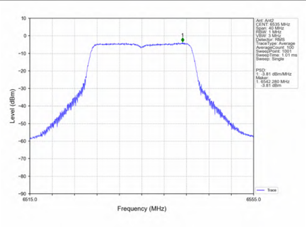
802.11n(HT20)_LCH_6535MHz_MIMO_NTNV
