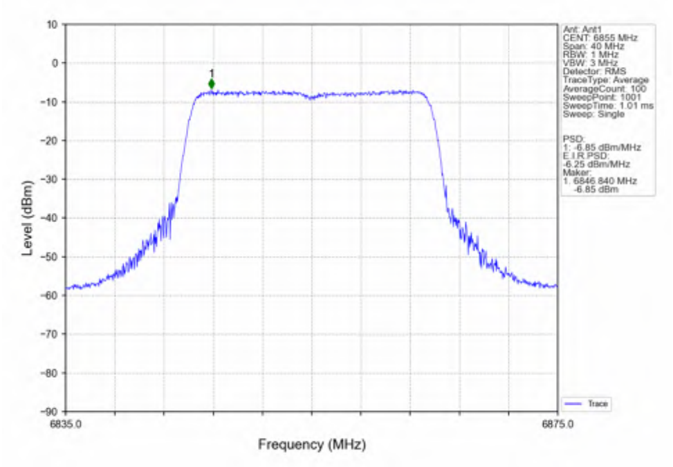
802.11ax(HEW20)_HCH_6855MHz_SU / Ant1_NTNV
