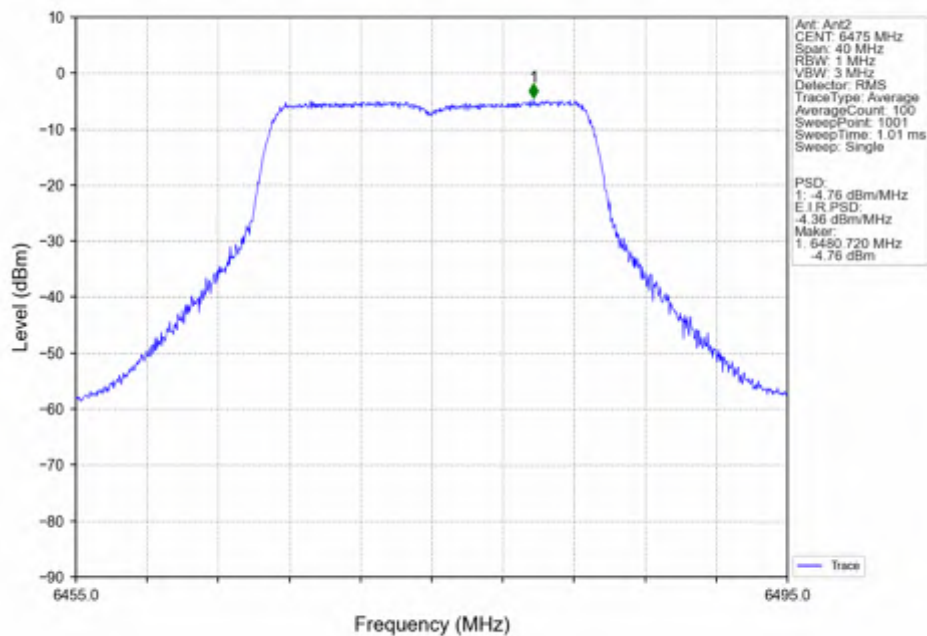
802.11ac(VHT20)_MCH_6475MHz_MIMO_NTNV
