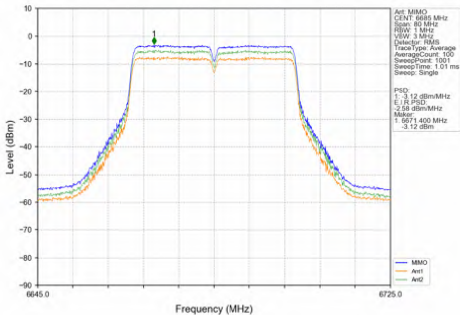
802.11n(HT40)_MCH_6685MHz_MIMO_NTNV
