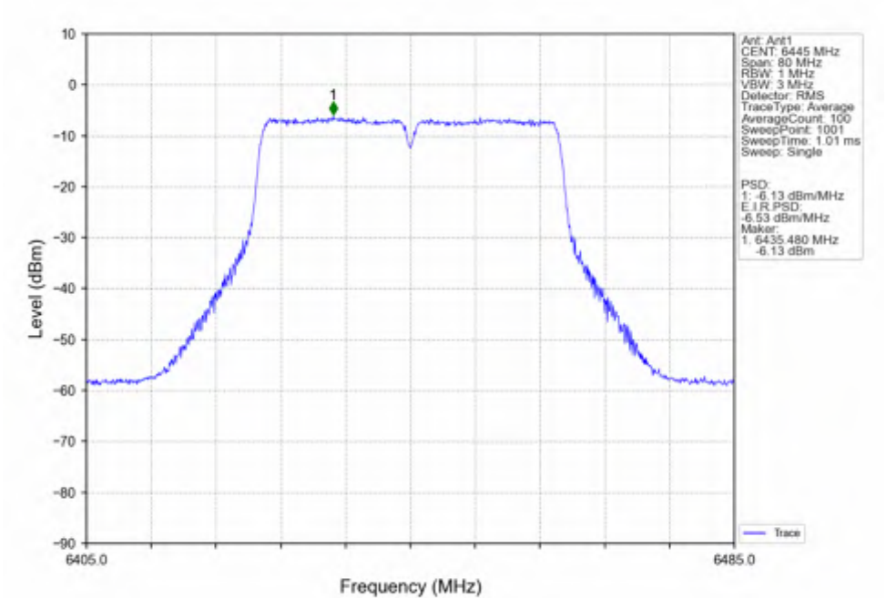
802.11ac(VHT40)_LCH_6445MHz_Ant1_NTNV
