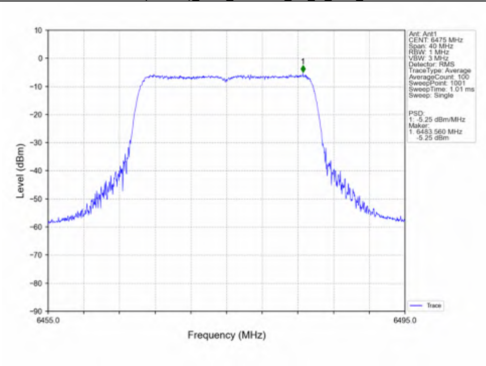
802.11ax(HEW20) MCH_6475MHz_SU / Ant1_NTNV
