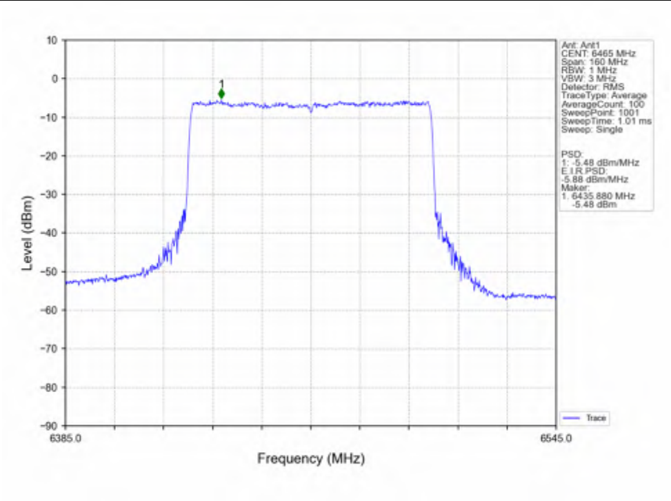
802.11ax(HEW80)_LCH_6465MHz_SU / Ant1_NTNV
