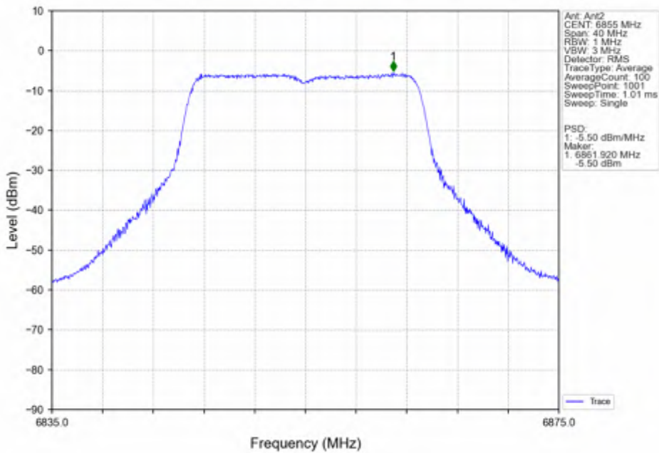
802.11ac(VHT20)_HCH_6855MHz_MIMO_NTNV
