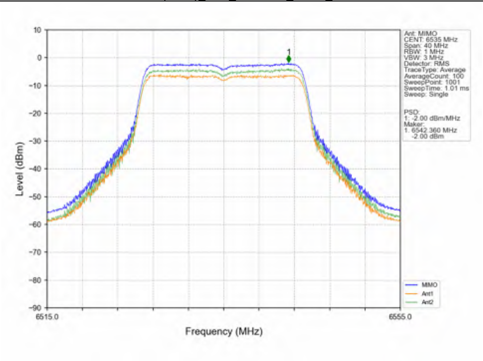
802.11n(HT20)_LCH_6535MHz_MIMO_NTNV
