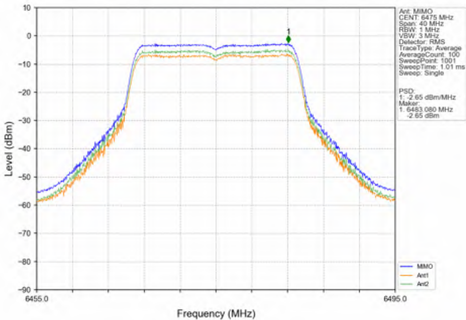
802.11ac(VHT20)_MCH_6475MHz_MIMO_NTNV
