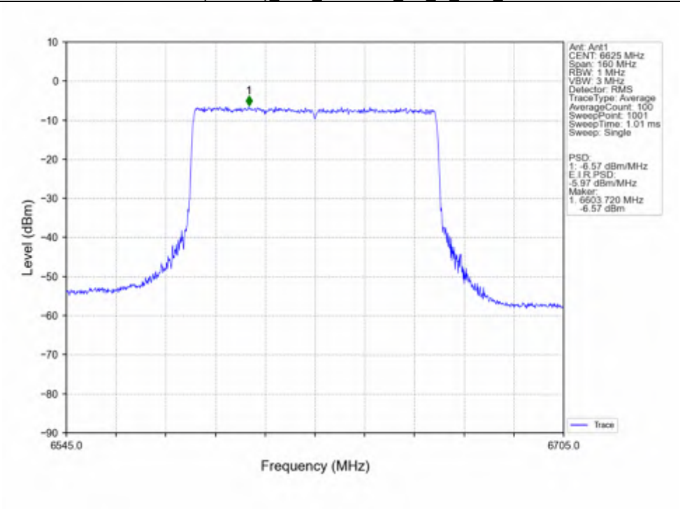
802.11ax(HEW80)_LCH_6625MHz_SU / Ant1_NTNV
