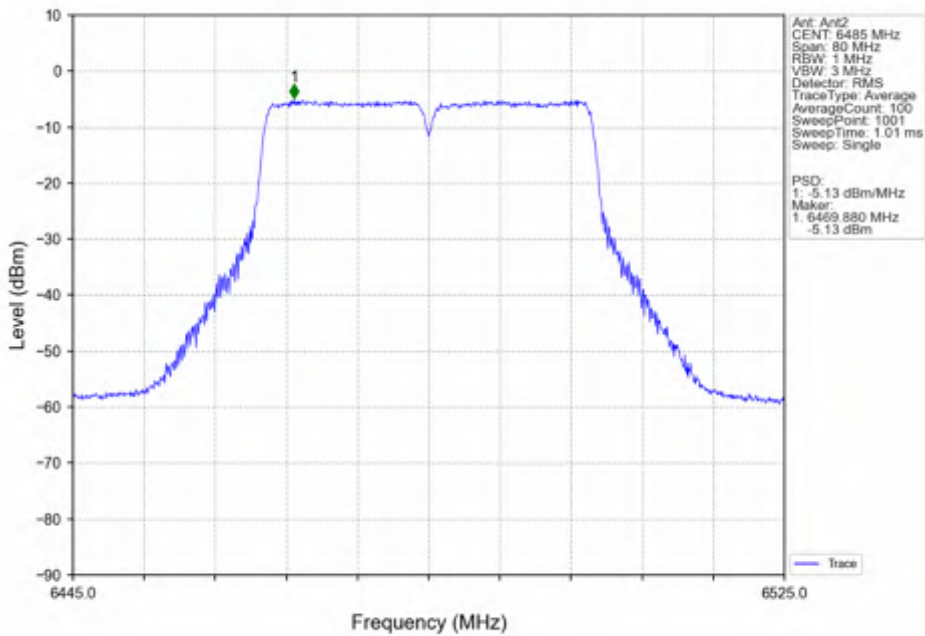
802.11n(HT40)_MCH_6485MHz_MIMO_NTNV
