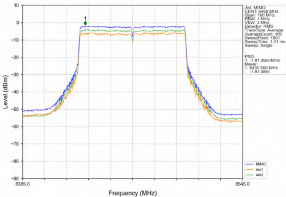
802.11ac(VHT80)_LCH_6465MHz_MIMO_NTNV
