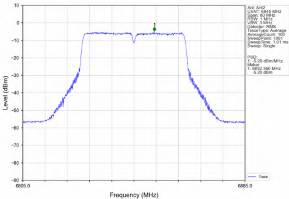
802.11ac(VHT40)_HCH_6845MHz_Ant2_NTNV
