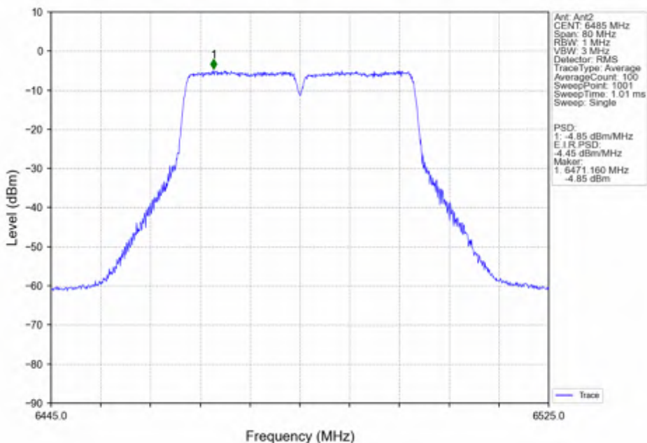
802.11ac(VHT40)_MCH_6485MHz_Ant2_NTNV
