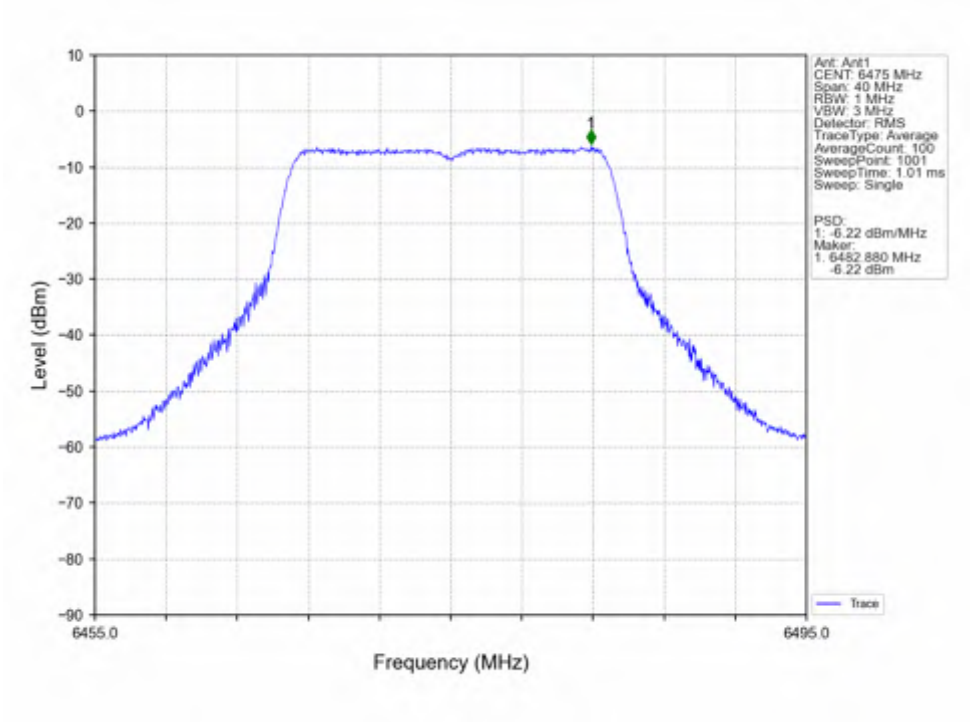
802.11ac(VHT20)_MCH_6475MHz_Ant1_NTNV
