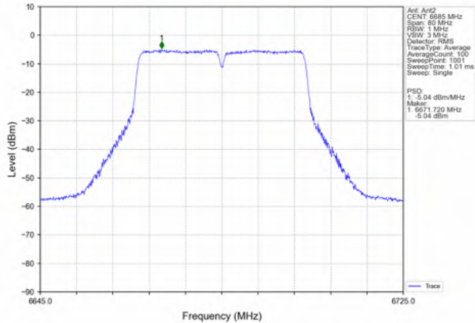
802.11n(HT40)_MCH_6685MHz_MIMO_NTNV
