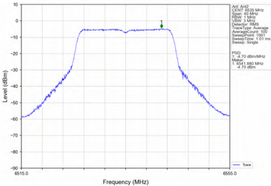
802.11ac(VHT20)_LCH_6535MHz_MIMO_NTNV
