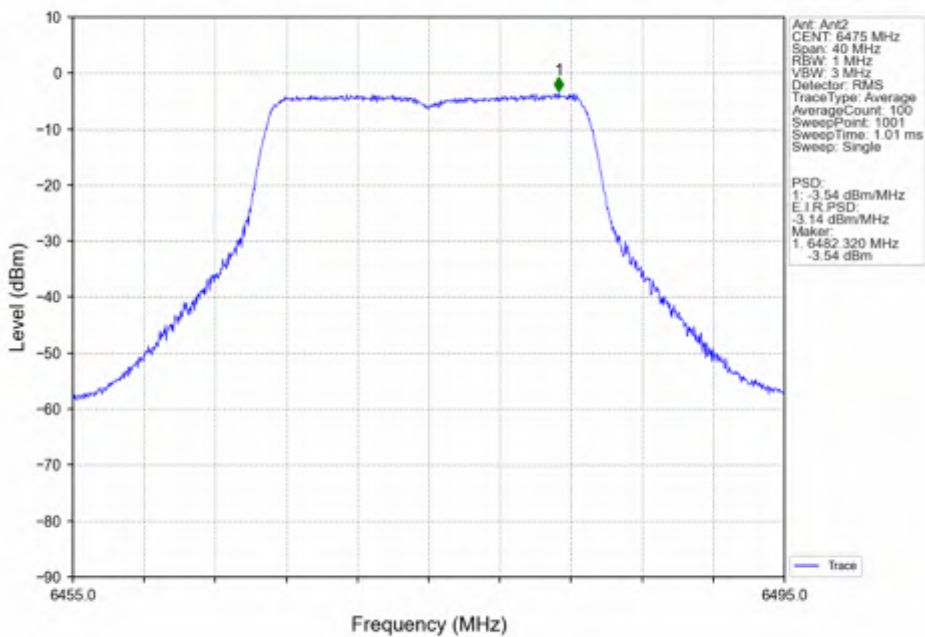
802.11n(HT20)_MCH_6475MHz_Ant2_NTNV
