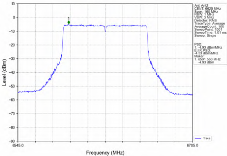
802.11ac(VHT80)_LCH_6625MHz_MIMO_NTNV
