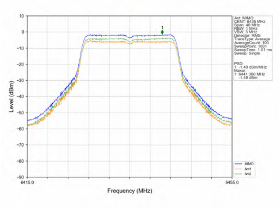
802.11n(HT20)_LCH_6435MHz_MIMO_NTNV
