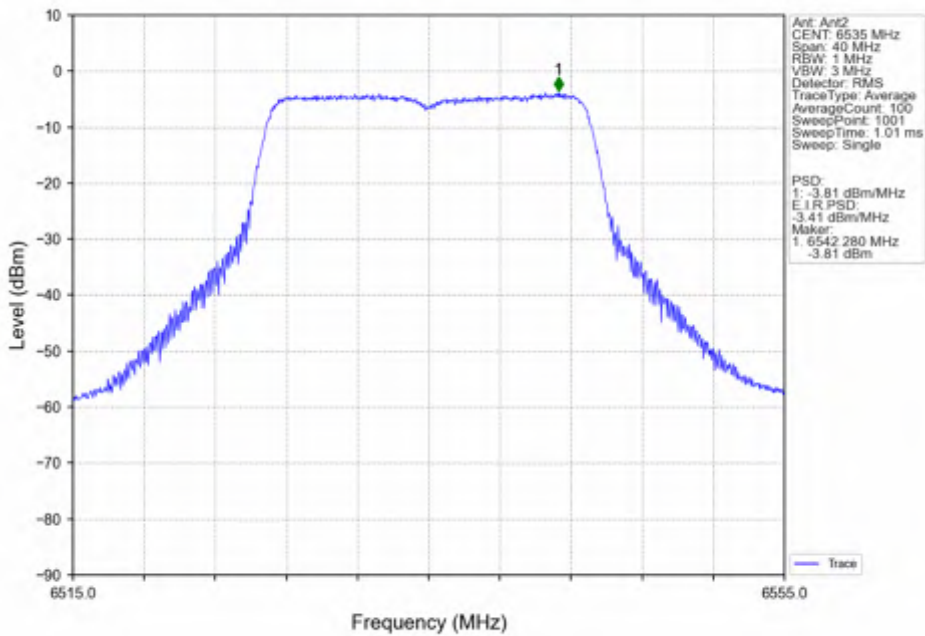
802.11n(HT20)_LCH_6535MHz_MIMO_NTNV
