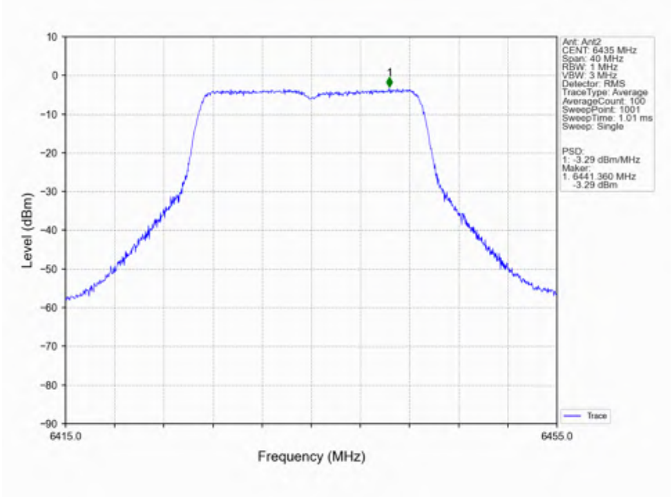
802.11n(HT20)_LCH_6435MHz_MIMO_NTNV
