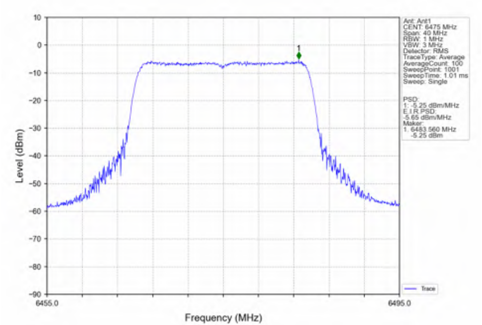
802.11ax(HEW20) MCH_6475MHz_SU / Ant1_NTNV
