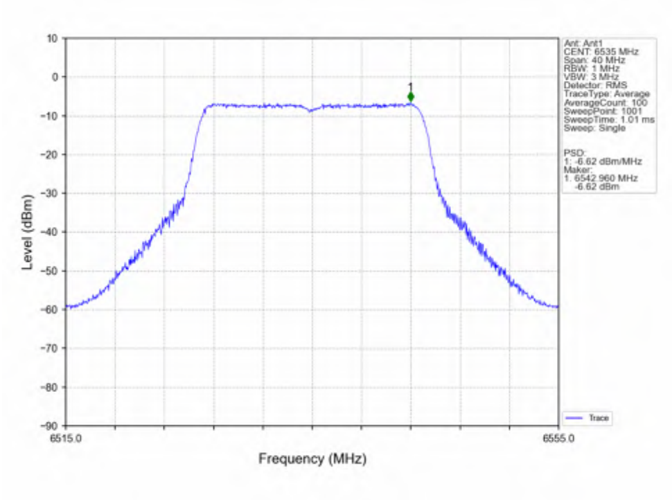
802.11ac(VHT20)_LCH_6535MHz_Ant1_NTNV
