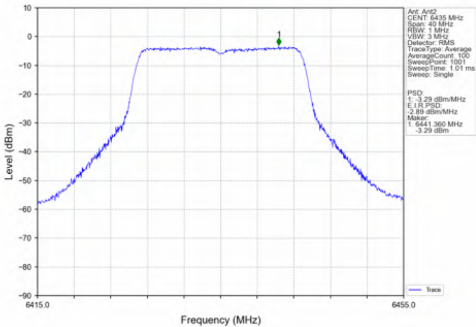
802.11n(HT20)_LCH_6435MHz_MIMO_NTNV
