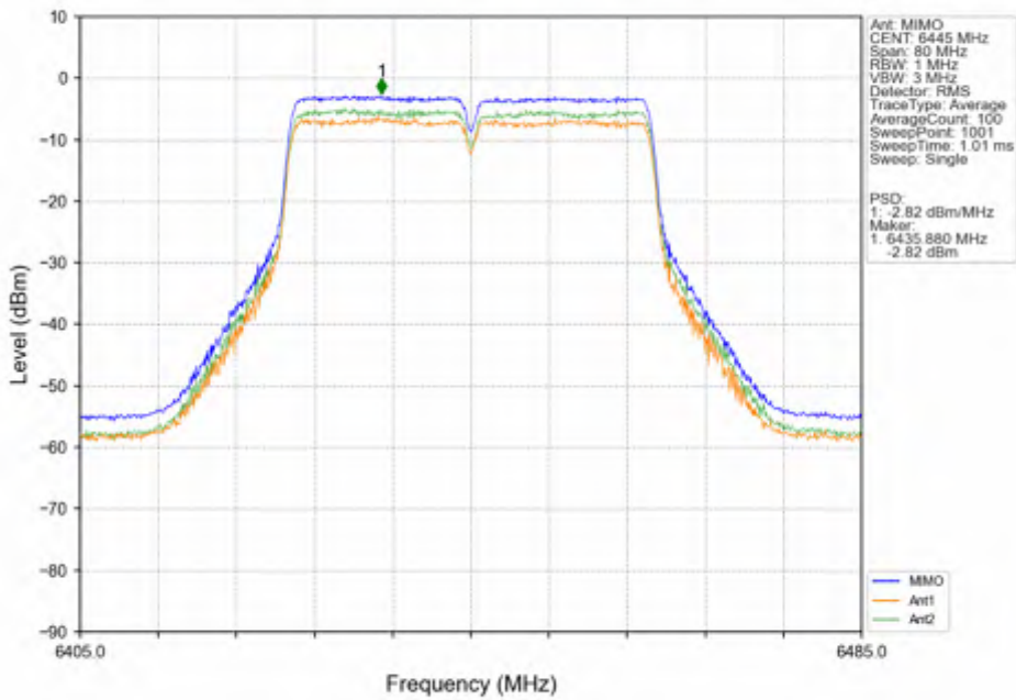
802.11ac(VHT40)_LCH_6445MHz_MIMO_NTNV
