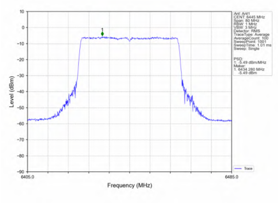
802.11ax(HEW40)_LCH_6445MHz_SU / Ant1_NTNV
