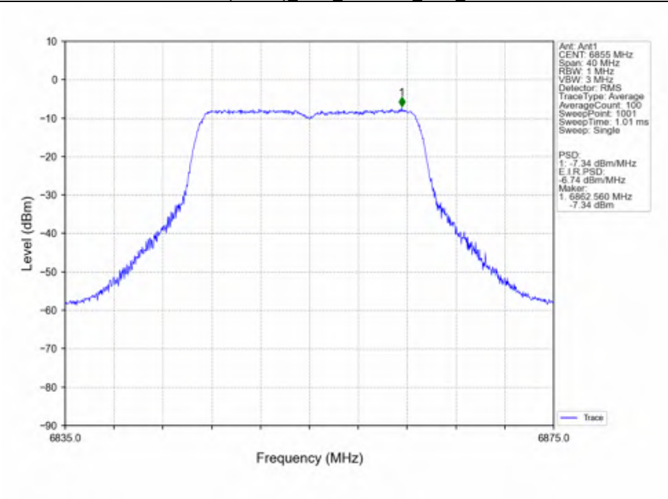
802.11ac(VHT20)_HCH_6855MHz_Ant1_NTNV
