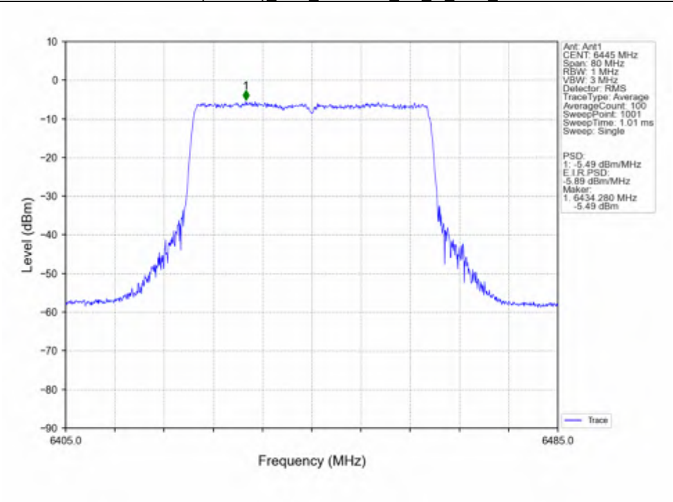
802.11ax(HEW40)_LCH_6445MHz_SU / Ant1_NTNV
