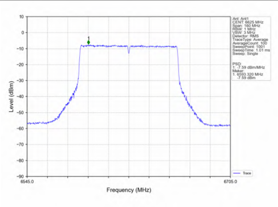
802.11ac(VHT80)_LCH_6625MHz_Ant1_NTNV
