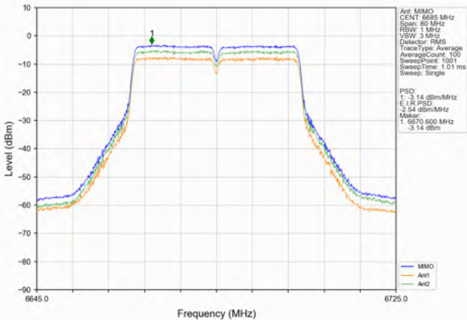
802.11ac(VHT40)_MCH_6685MHz_MIMO_NTNV
