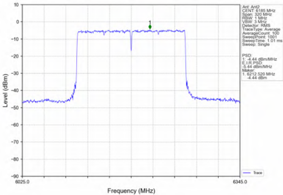
802.11ax(HEW160)_MCH_6185MHz_SU / MIMO_NTNV
