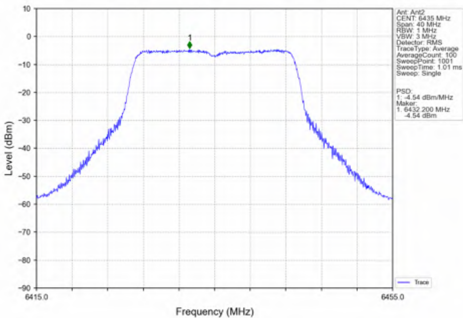
802.11ac(VHT20)_LCH_6435MHz_Ant2_NTNV
