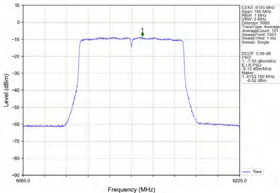
802.11ac(VHT80)_MCH_6145MHz_Ant2_NTNV
