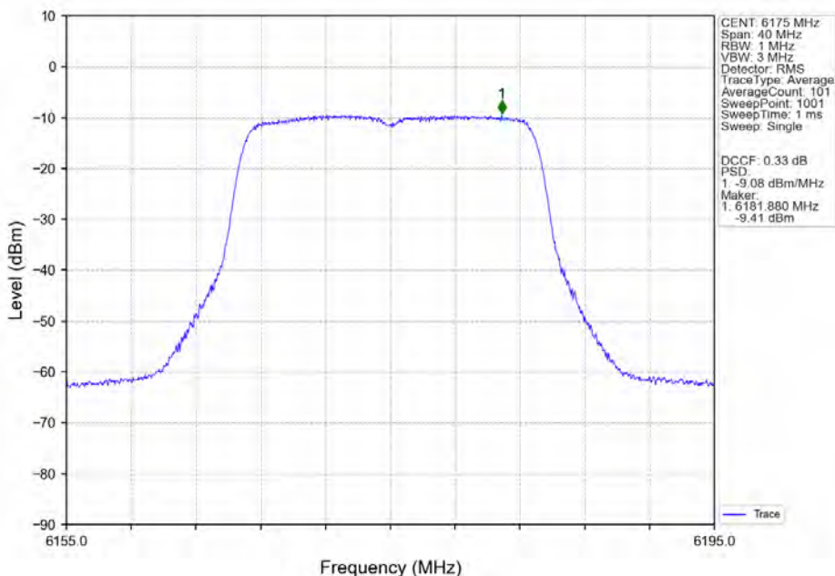
802.11ac(VHT20) MCH 6175MHz Ant2 NTN
