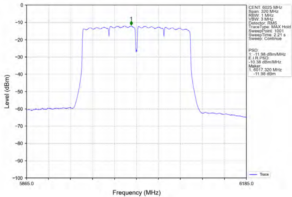
802.11ac(VHT160) LCH_6025MHz_Ant2_NTNV
