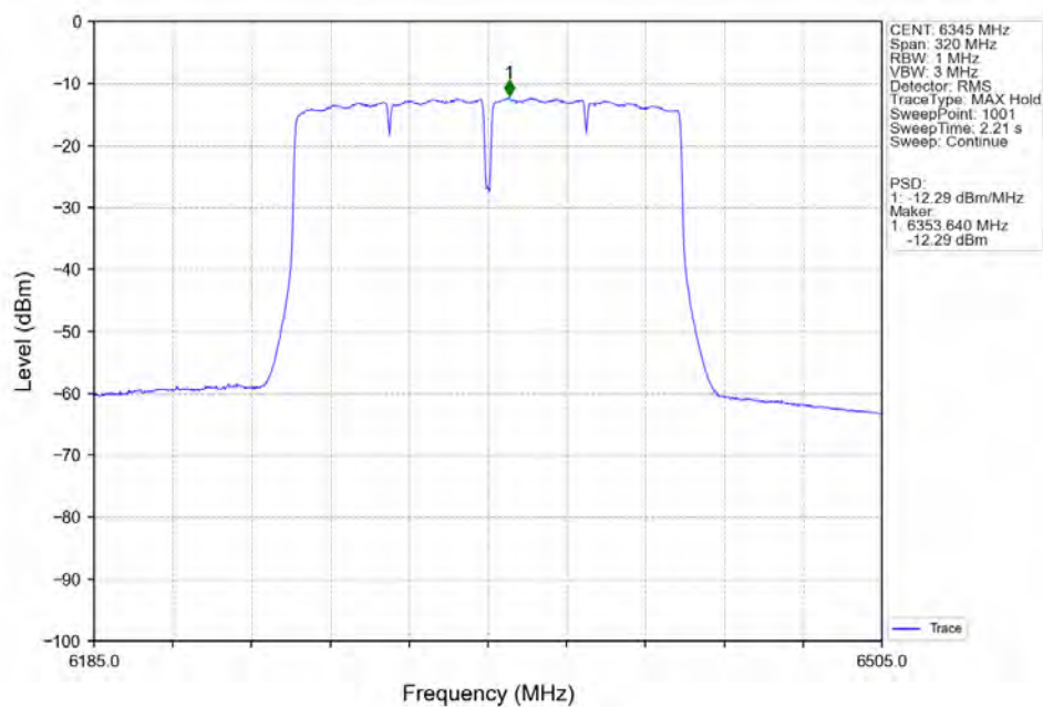
802.11ac(VHT160) HCH 6345MHz Ant2 NTN
