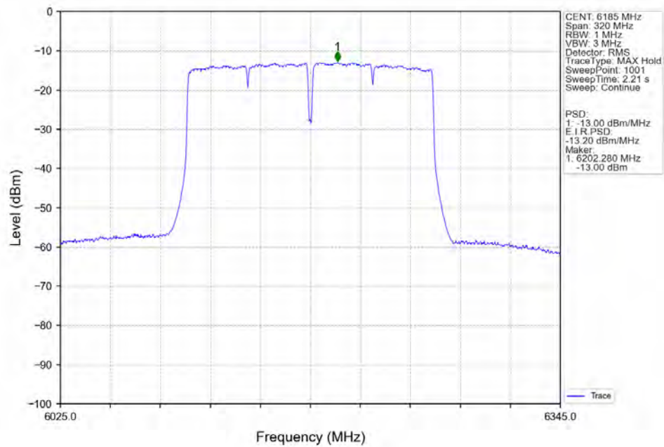
802.11ac(VHT160) MCH_6185MHz_MIMO_NTNV
