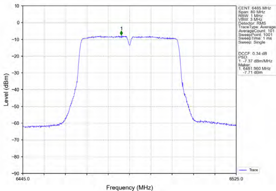
802.11ac(VHT40)_MCH_6485MHz_Ant2_NTNV
