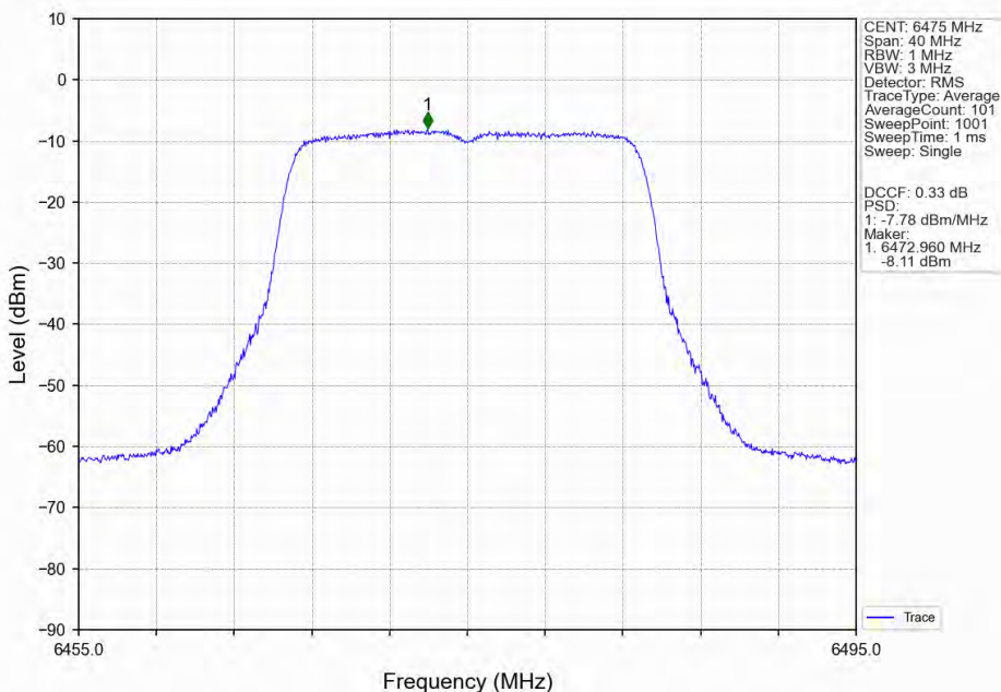
802.11n(HT20)_MCH_6475MHz_Ant2_NTNV
