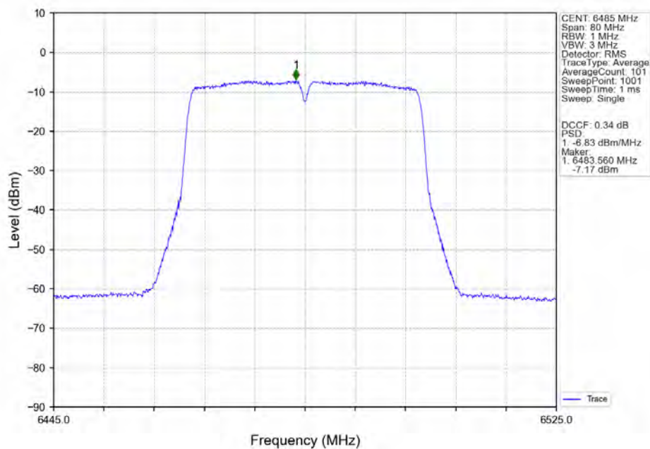
802.11ac(VHT40)_MCH_6485MHz_Ant2_NTNV
