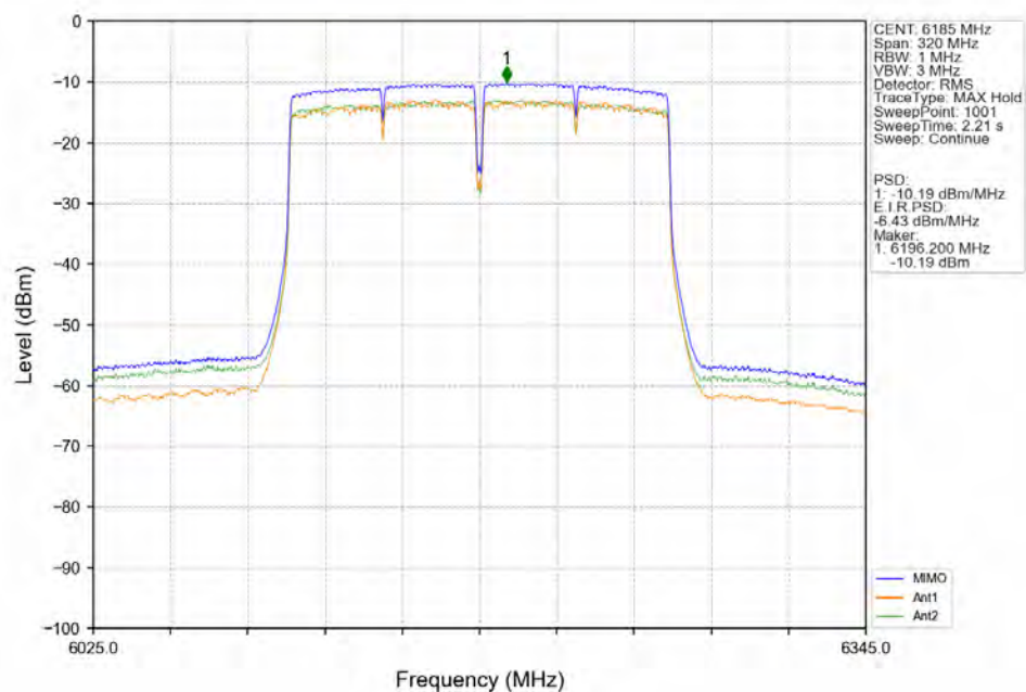
802.11ac(VHT160) MCH_6185MHz_MIMO_NTNV
