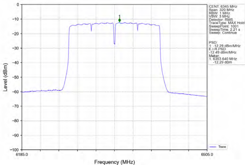
802.11ac(VHT160) HCH_6345MHz_Ant2_NTNV
