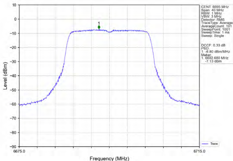
802.11ac(VHT20)_MCH_6695MHz_Ant2_NTNV
