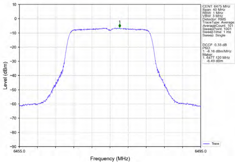
802.11ac(VHT20)_MCH_6475MHz_Ant1_NTNV
