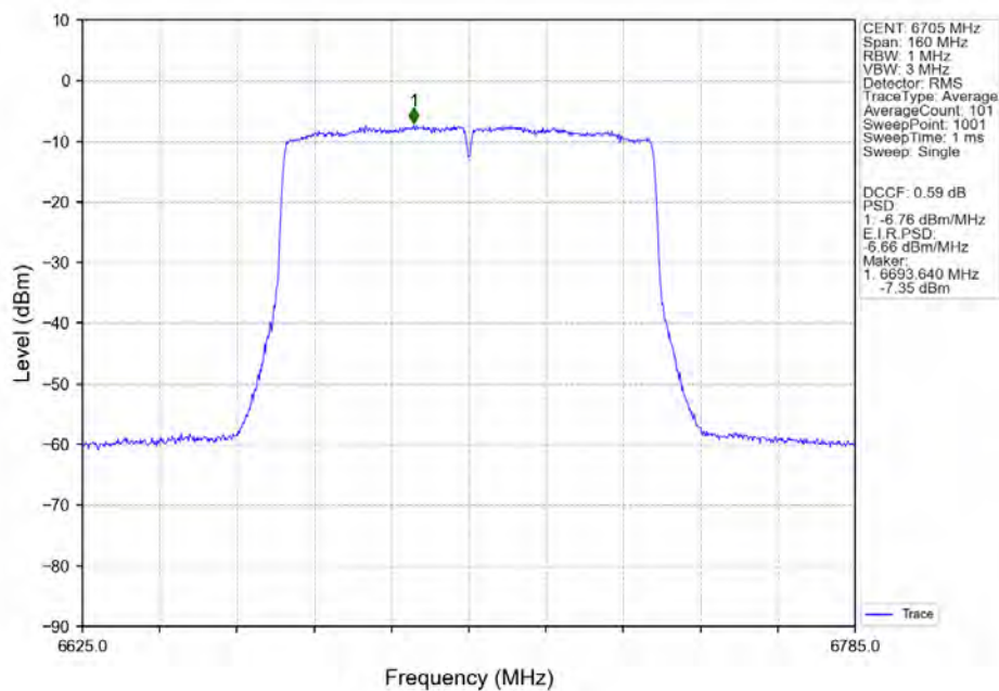
802.11ac(VHT80)_MCH_6705MHz_Ant2_NTNV
