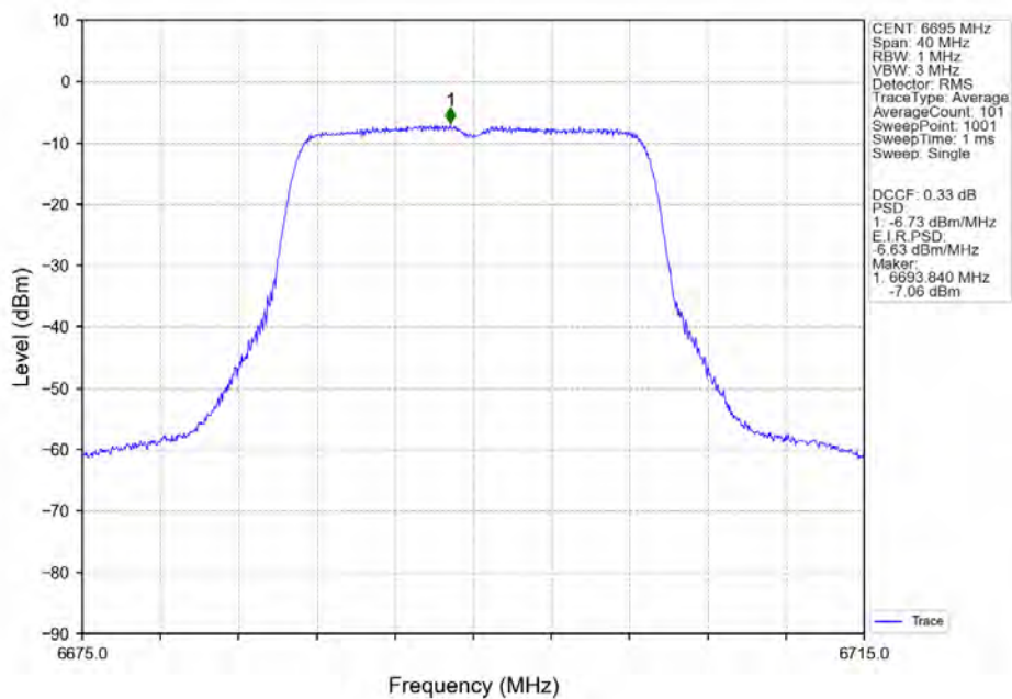
802.11ac(VHT20) MCH 6695MHz Ant2 NTN
