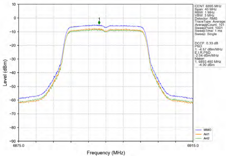
802.11ac(VHT20)_LCH_6895MHz_MIMO_NTNV
