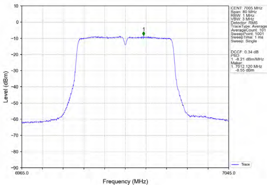
802.11ac(VHT40) MCH_7005MHz_MIMO_NTNV
