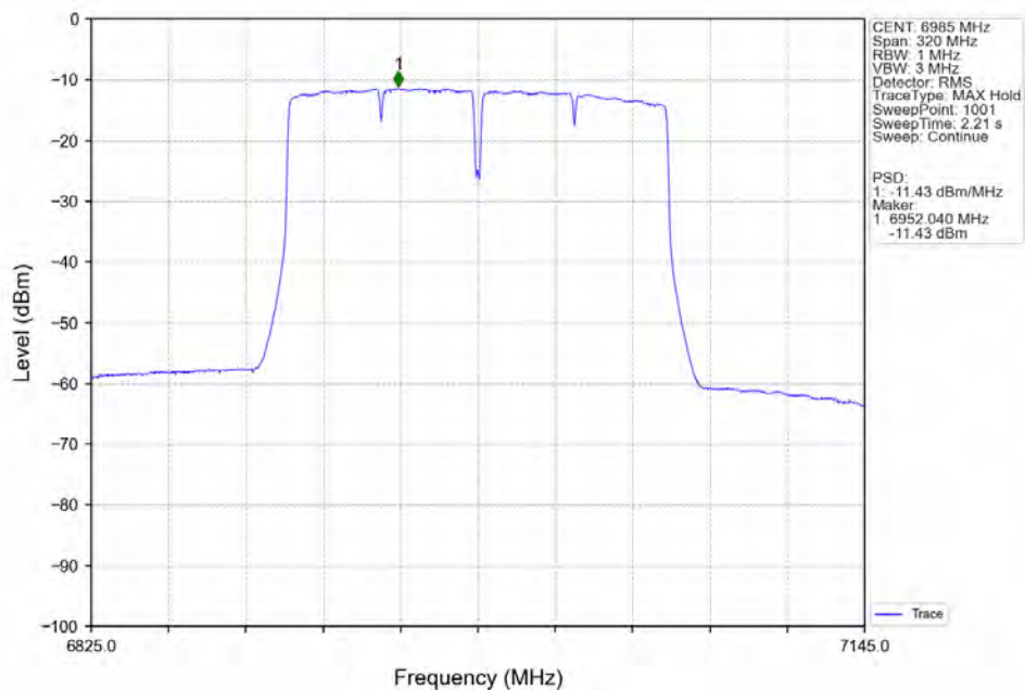
802.11ac(VHT160) MCH_6985MHz_Ant1_NTNV
