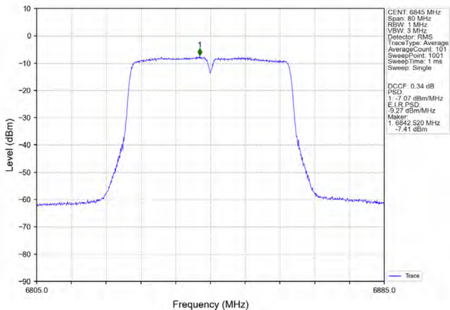
802.11ac(VHT40) HCH 6845MHz Ant2 NTN
