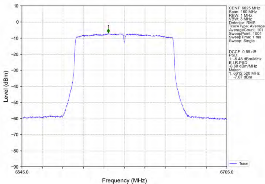
802.11ac(VHT80)_LCH_6625MHz_MIMO_NTNV
