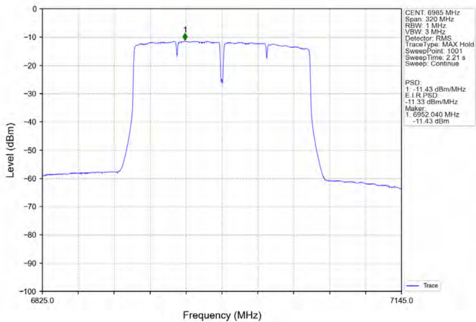
802.11ac(VHT160) MCH_6985MHz_Ant1_NTNV
