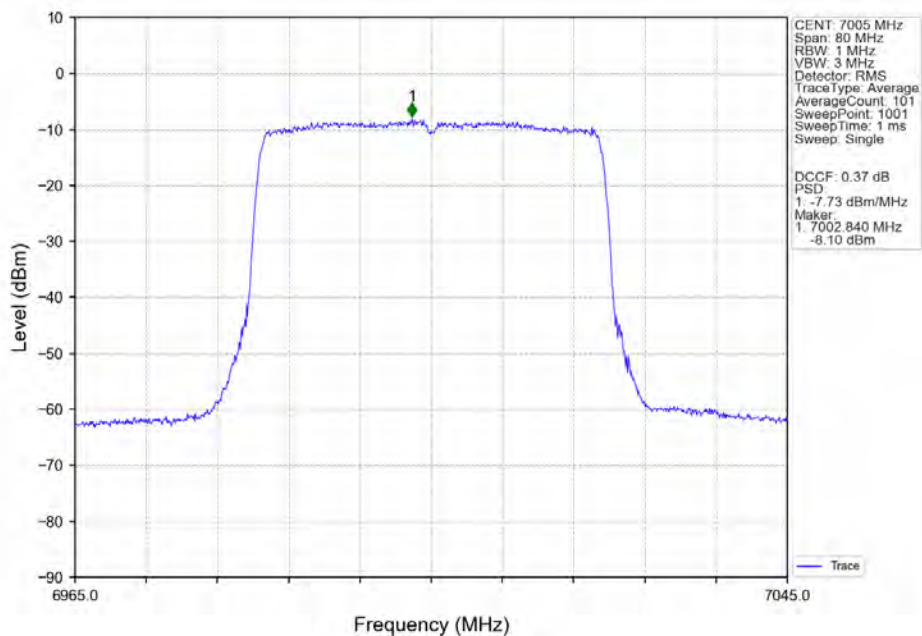
802.11ax(HEW40) MCH_7005MHz_SU / Ant2_NTNV
