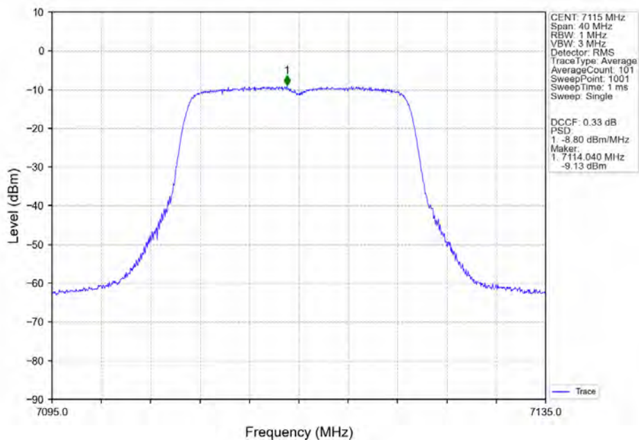
802.11ac(VHT20) HCH_7115MHz Ant1_NTNV
