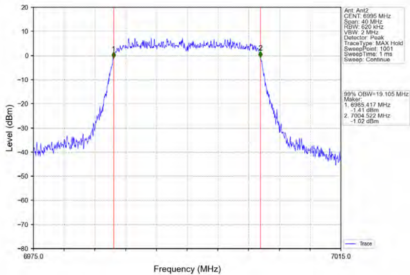
802.11ax(HEW20)_MCH_6995MHz_RU242_Left_Ant2_NTNV
