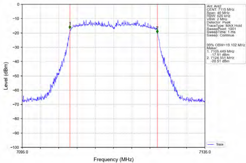
802.11ax(HEW20)_HCH_7115MHz_RU242_Left_Ant2_NTNV
