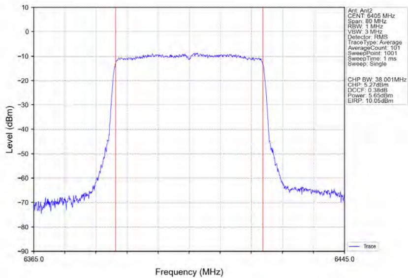
802.11ax(HEW40)_HCH_6405MHz_RU484_Left_Ant2_NTNV
