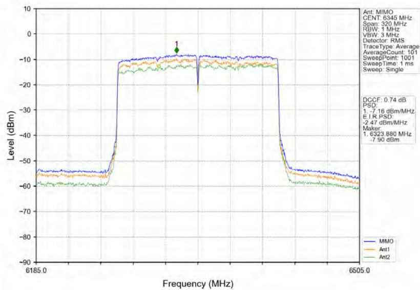
802.11ax(HEW160) HCH 6345MHz 2xRU996 Left MIMO NTV
