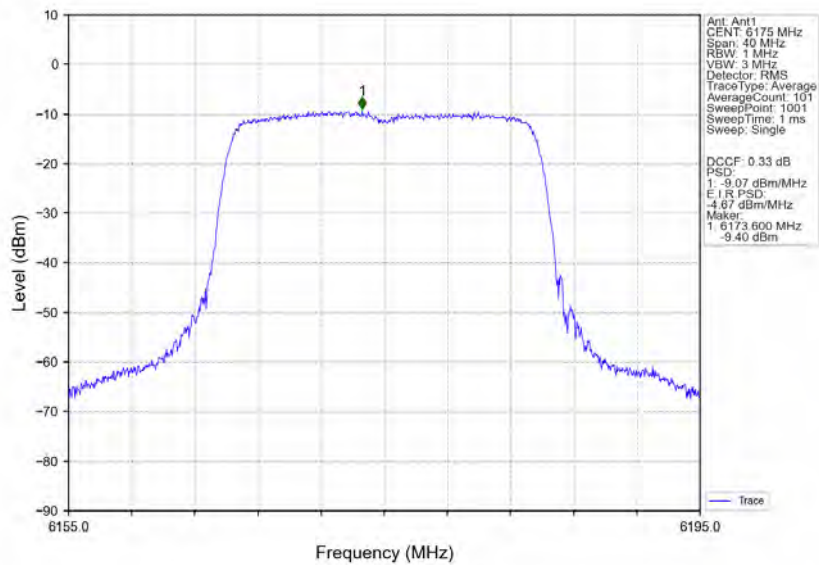
802.11ax(HEW20) MCH 6175MHz RU242 Left Ant1 NTN
