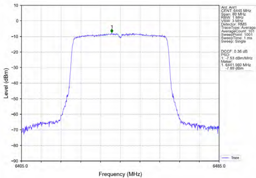
802.11ax(HEW40) LCH 6445MHz RU484 Left Ant1 NTN
