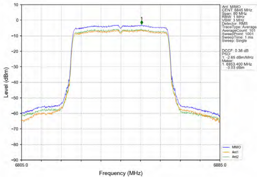
802.11ax(HEW40) HCH 6845MHz RU484 Left MIMO NTN
