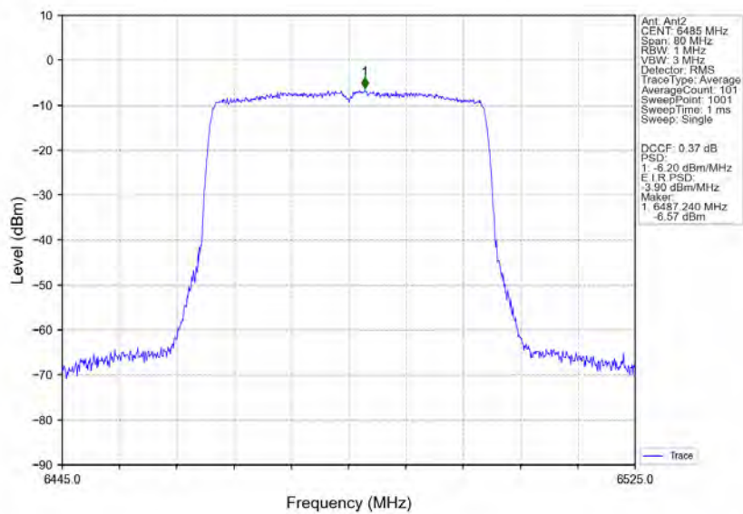
802.11ax(HEW40)_MCH_6485MHz_RU484_Left_Ant2_NTNV
