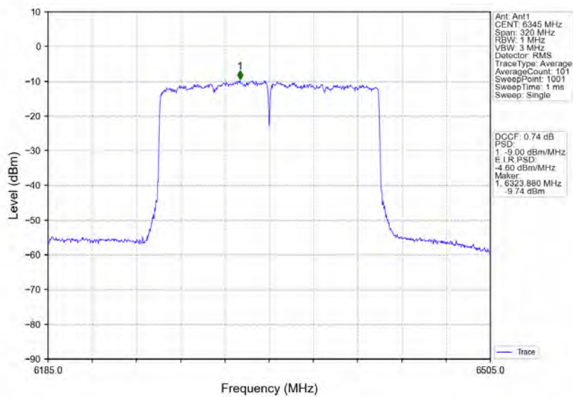
802.11ax(HEW160) HCH 6345MHz 2xRU996 Left Ant1 NTNV
