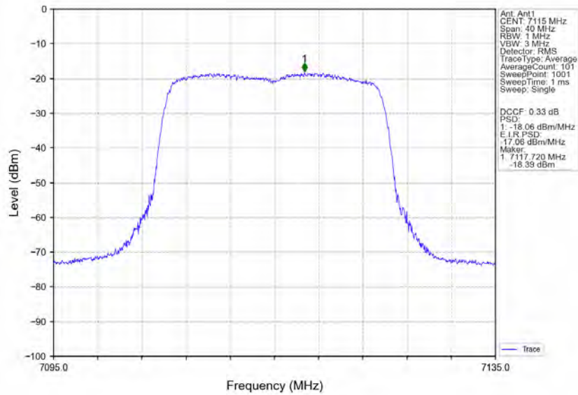
802.11ax(HEW20)_HCH_7115MHz_RU242_Left_Ant2_NTNV
