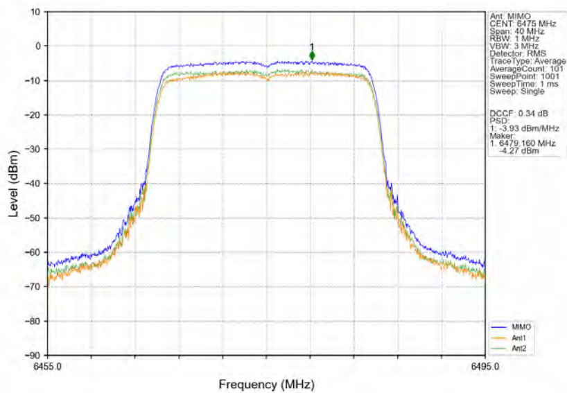
802.11ax(HEW20)_MCH_6475MHz_RU242_Left_MIMO_NTNV
