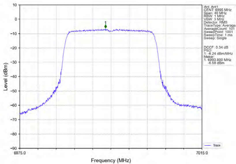
802.11ax(HEW20) MCH 6995MHz RU242 Left Ant1 NTN
