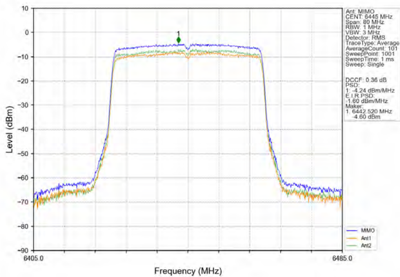
802.11ax(HEW40) LCH_6445MHz RU484 Left MIMO NTN
