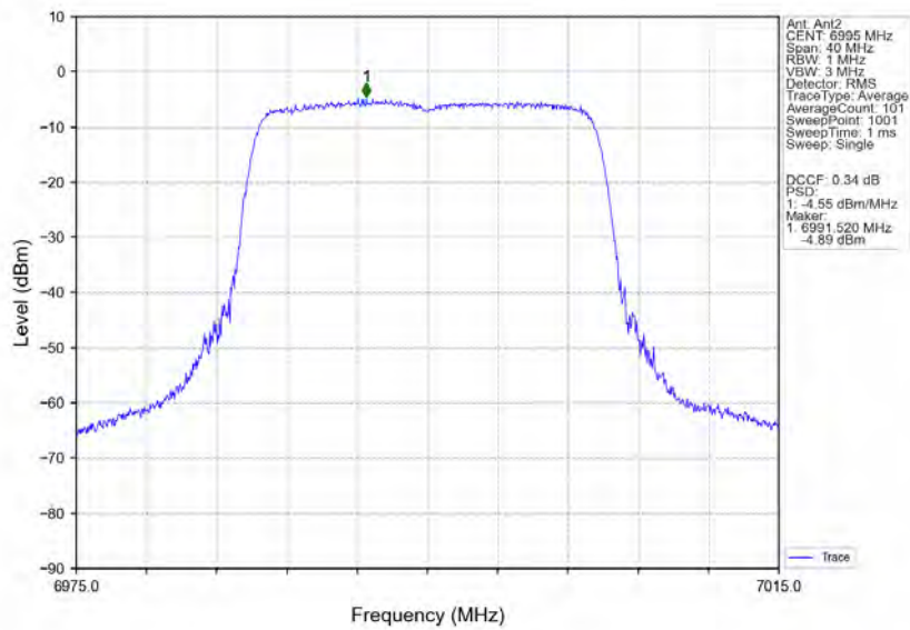
802.11ax(HEW20)_MCH_6995MHz_RU242_Left_MIMO_NTNV
