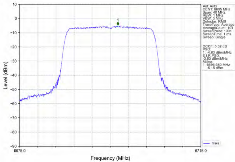
802.11ax(HEW20)_MCH_6695MHz_RU242_Left_MIMO_NTNV
