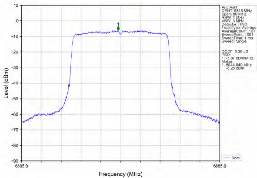
802.11ax(HEW40) HCH 6845MHz RU484 Left Ant1 NTN
