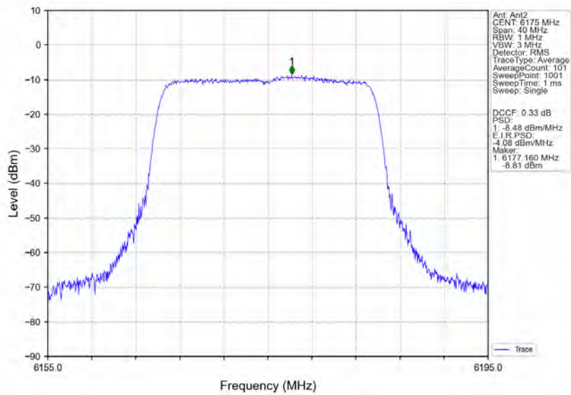
802.11ax(HEW20)_MCH_6175MHz_RU242_Left_MIMO_NTNV
