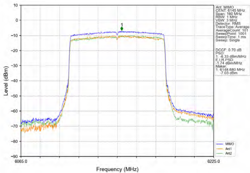
802.11ax(HEW80)_MCH_6145MHz_RU996_Left_MIMO_NTNV
