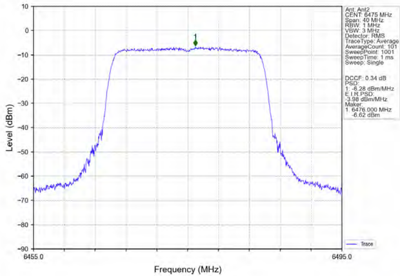
802.11ax(HEW20)_MCH_6475MHz_RU242_Left_MIMO_NTNV
