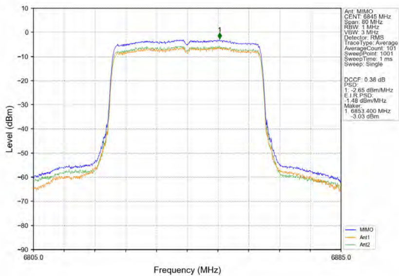
802.11ax(HEW40)_HCH_6845MHz_RU484_Left_MIMO_NTNV
