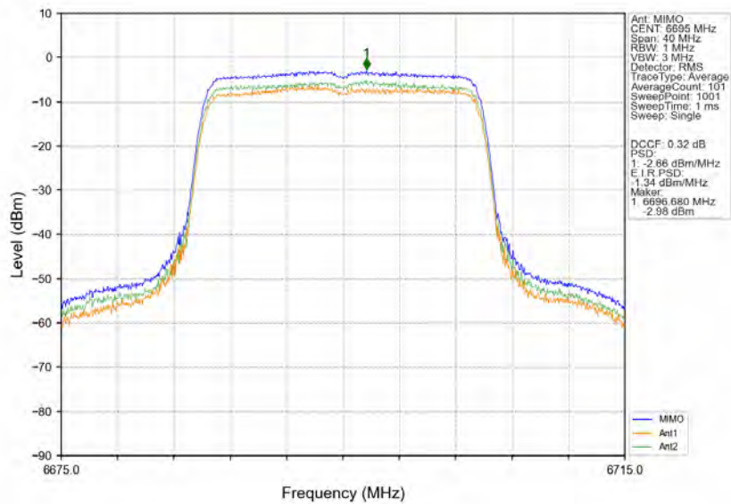
802.11ax(HEW20)_MCH_6695MHz_RU242_Left_MIMO_NTNV
