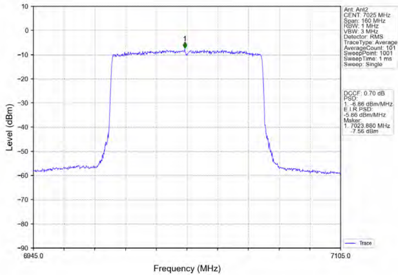
802.11ax(HEW80)_HCH_7025MHz_RU996_Left_MIMO_NTNV
