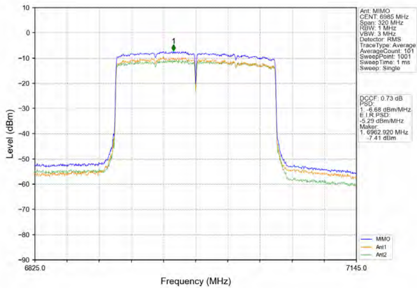
802.11ax(HEW160)_MCH_6985MHz_2xRU996_Left_MIMO_NTNV
