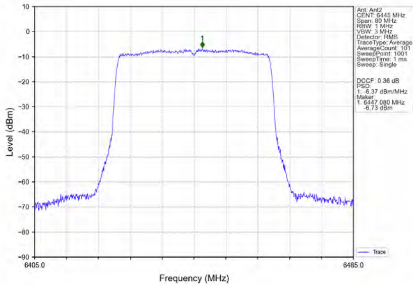
802.11ax(HEW40)_LCH_6445MHz_RU484_Left_MIMO_NTNV
