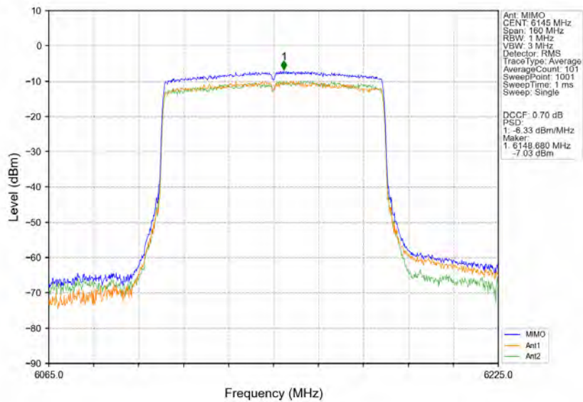
802.11ax(HEW80)_MCH_6145MHz_RU996_Left_MIMO_NTNV
