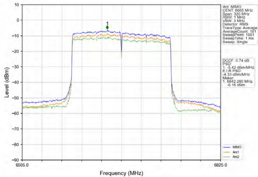
802.11ax(HEW160)_MCH_6665MHz_2xRU996_Left_MIMO_NTNV
