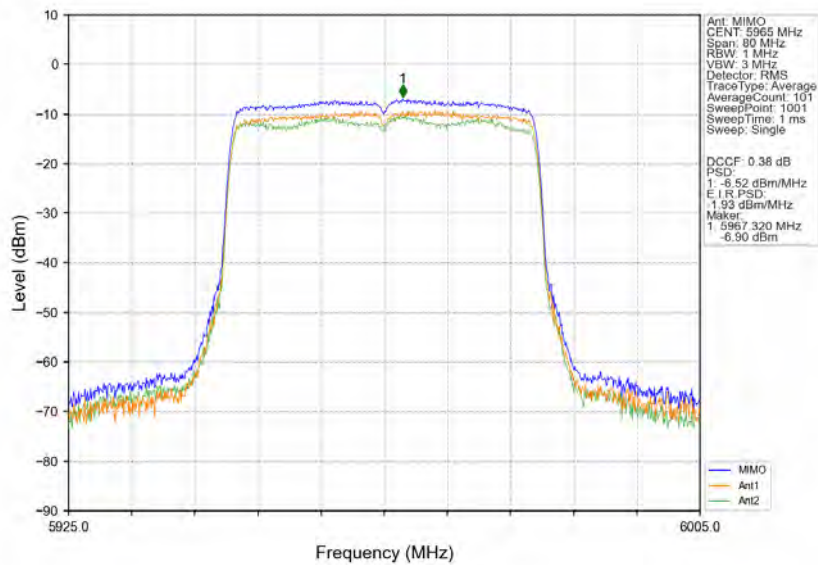
802.11ax(HEW40)_LCH_5965MHz_RU484_Left_MIMO_NTNV
