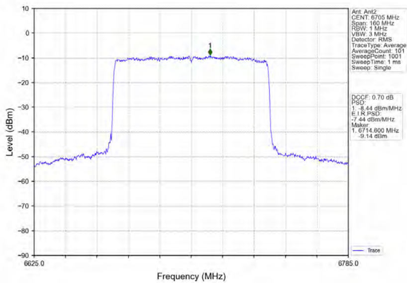
802.11ax(HEW80)_MCH_6705MHz_RU996_Left_MIMO_NTNV
