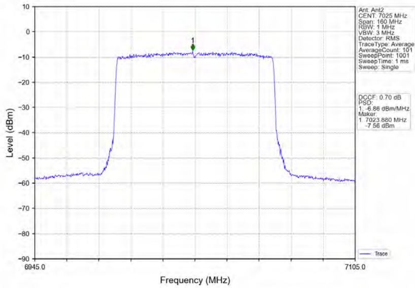
802.11ax(HEW80)_HCH_7025MHz_RU996_Left_MIMO_NTNV
