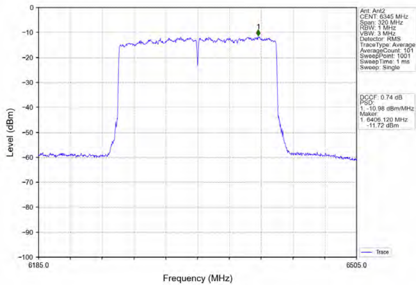
802.11ax(HEW160)_HCH_6345MHz_2xRU996_Left_MIMO_NTNV
