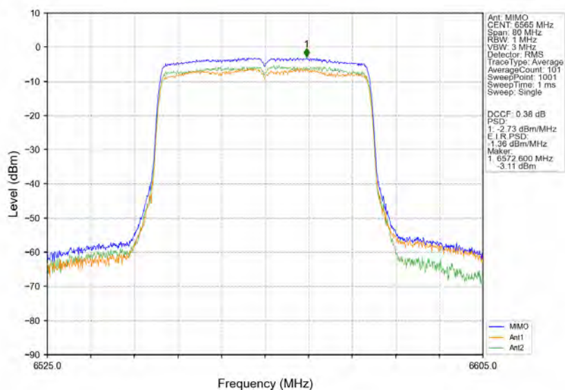
802.11ax(HEW40)_LCH_6565MHz_RU484_Left_MIMO_NTNV
