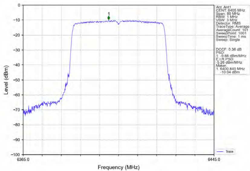
802.11ax(HEW40)_HCH_6405MHz_RU484_Left_Ant1_NTNV
