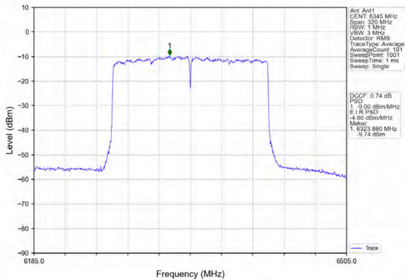
802.11ax(HEW160)_HCH_6345MHz_2xRU996_Left_Ant1_NTNV
