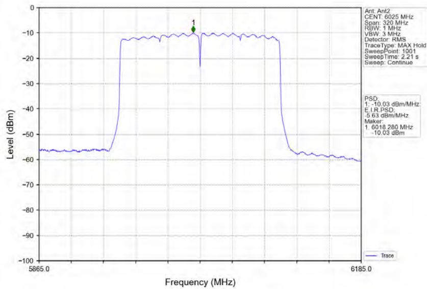
802.11ax(HEW160)_LCH_6025MHz_2xRU996_Left_MIMO_NTNV
