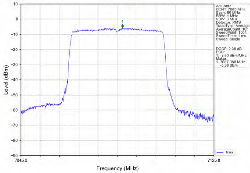
802.11ax(HEW40)_HCH_7085MHz_RU484_Left_MIMO_NTNV
