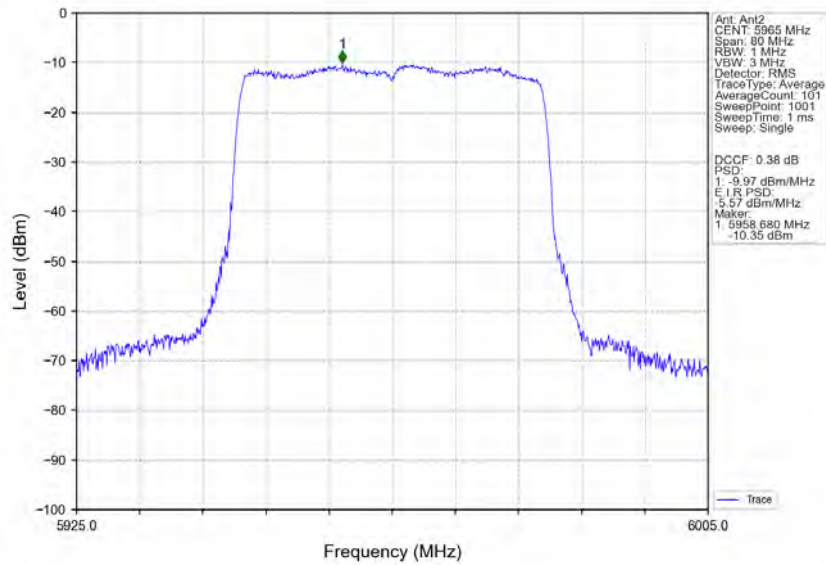
802.11ax(HEW40)_LCH_5965MHz_RU484_Left_MIMO_NTNV
