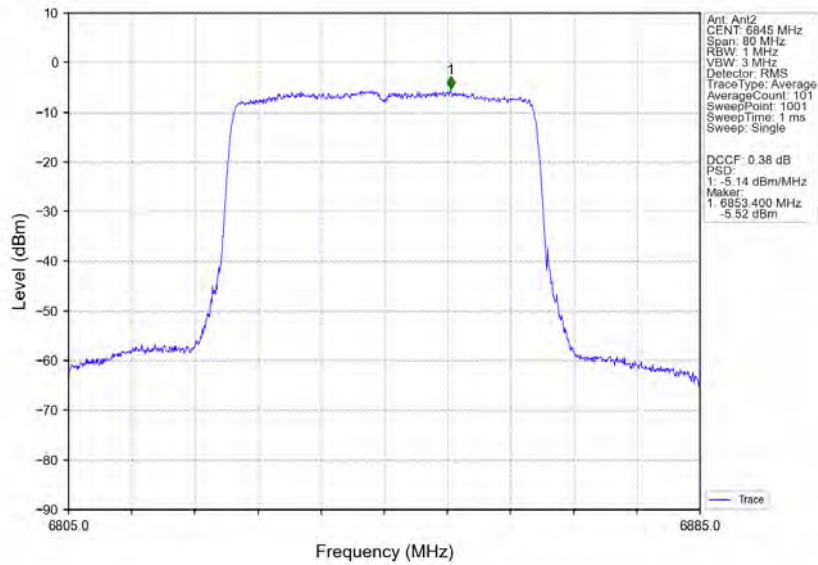
802.11ax(HEW40)_HCH_6845MHz_RU484_Left_MIMO_NTNV
