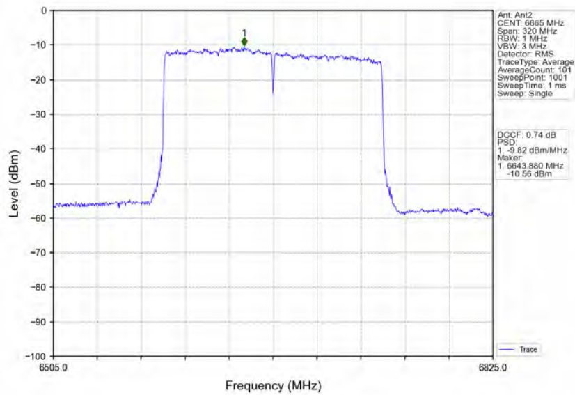
802.11ax(HEW160)_MCH_6665MHz_2xRU996_Left_MIMO_NTNV
