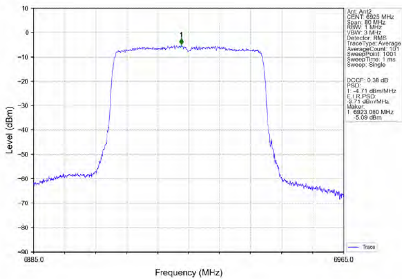
802.11ax(HEW40)_LCH_6925MHz_RU484_Left_MIMO_NTNV
