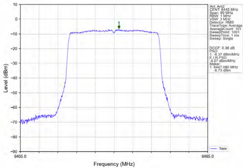
802.11ax(HEW40)_LCH_6445MHz_RU484_Left_MIMO_NTNV
