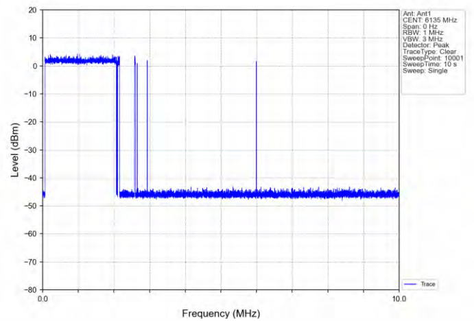
11AX20SISO-Ant 1-6135-Center-6135-Minimal
