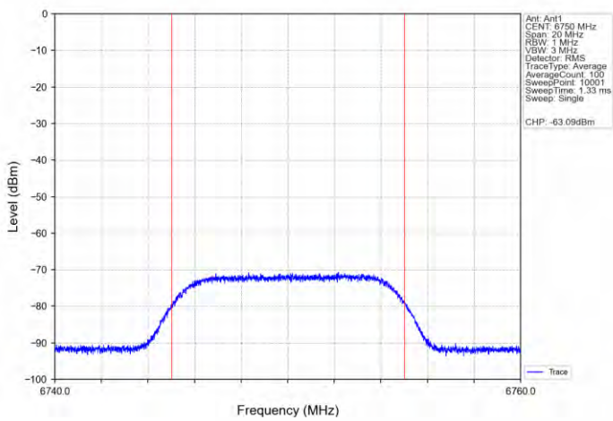
11AX160SISO-Ant 1-6825-Center-6750-Minimal
