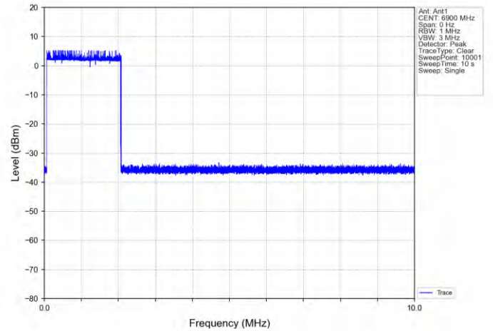
11AX160SISO-Ant 1-6825-Center-6900-Minimal
