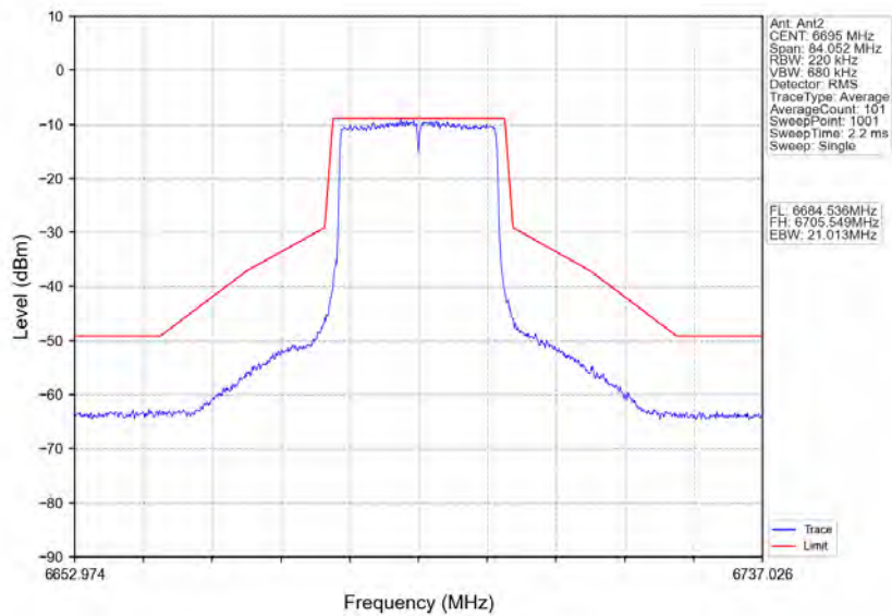
802.11ax(HEW20)_MCH_6695MHz_RU242_Left_Ant2_NTNV
