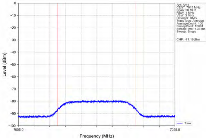
11AX20SISO-Ant 107015-Center-7015-Minimal
