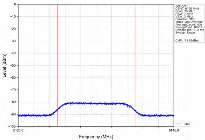
11AX20SISO-Ant 1-6135-Center-6135-Minimal
