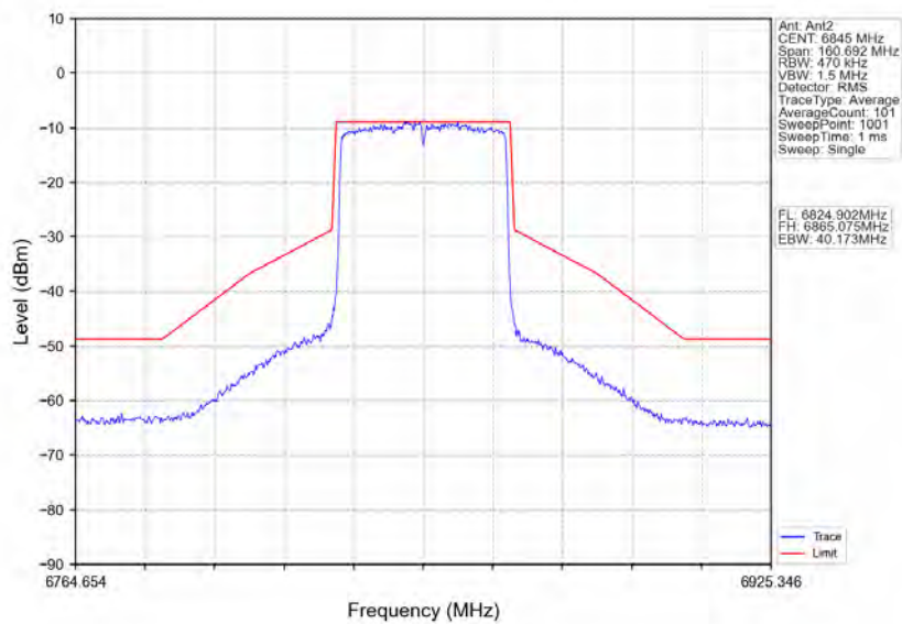
802.11ax(HEW40) HCH 6845MHz RU484 Left Ant2 NTVN
