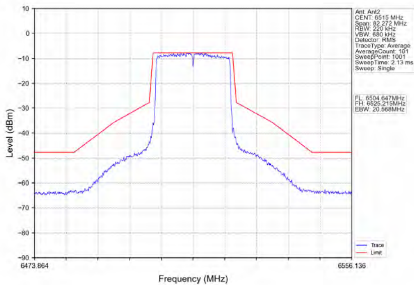
802.11ax(HEW20)_HCH_6515MHz_RU242_Left_Ant2_NTNV
