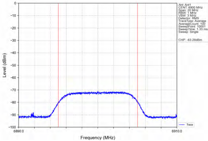
11AX160SISO-Ant 1-6825-Center-6900-Minimal
