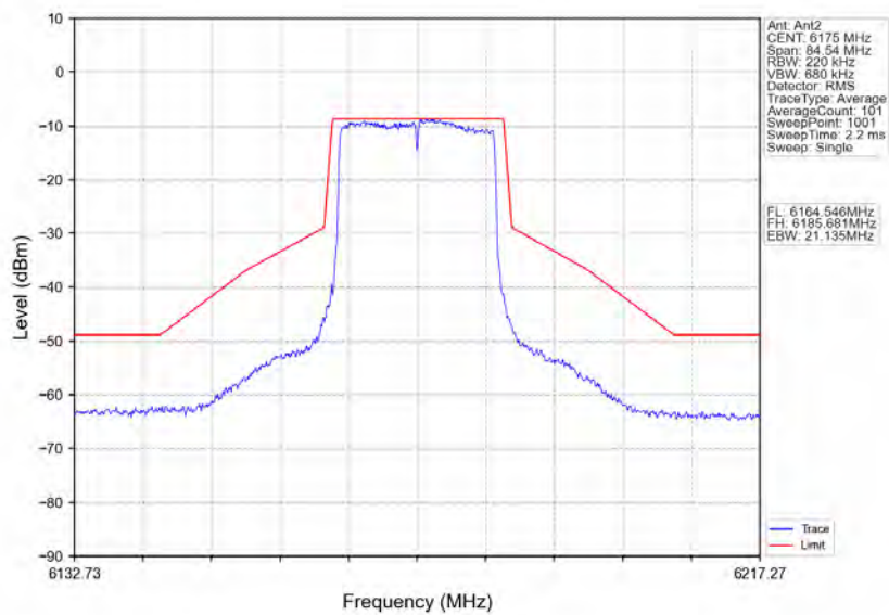
802.11ax(HEW20) MCH 6175MHz RU242 Left Ant2 NTVN
