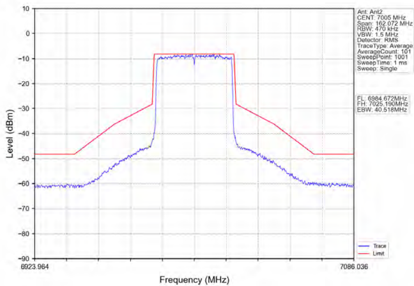
802.11ax(HEW40) MCH 7005MHz RU484 Left Ant2 NTVN
