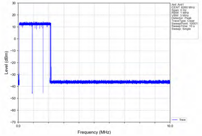
11AX160SISO-Ant 1-6185-Center-6260-Minimal
