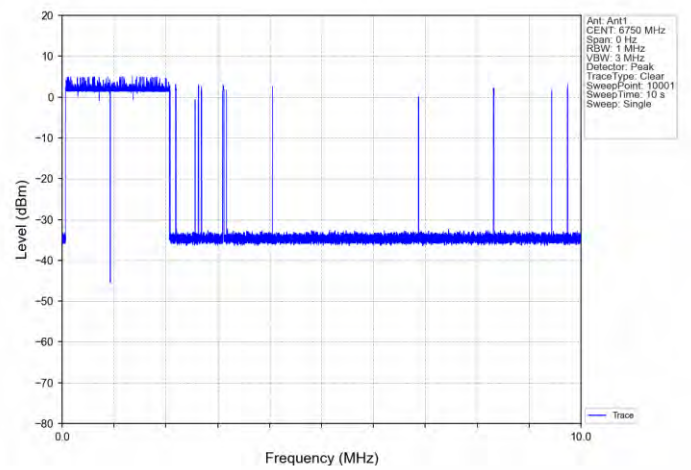
11AX160SISO-Ant 1-6825-Center-6750-Minimal
