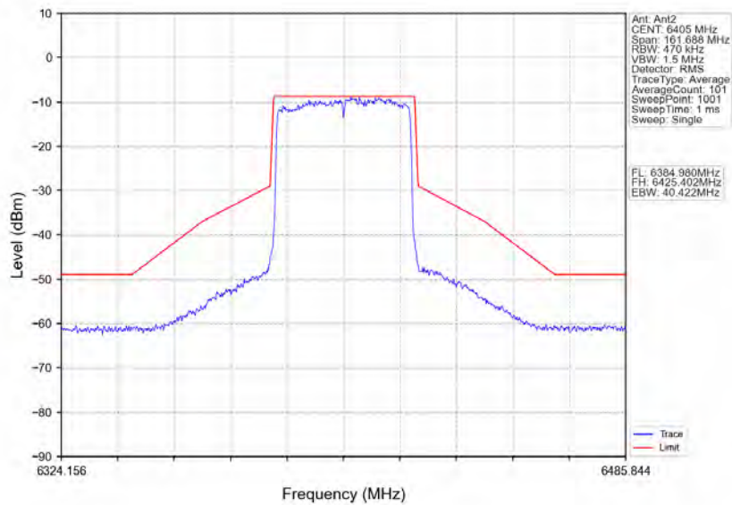
802.11ax(HEW40)_HCH_6405MHz_RU484_Left_Ant2_NTNV
