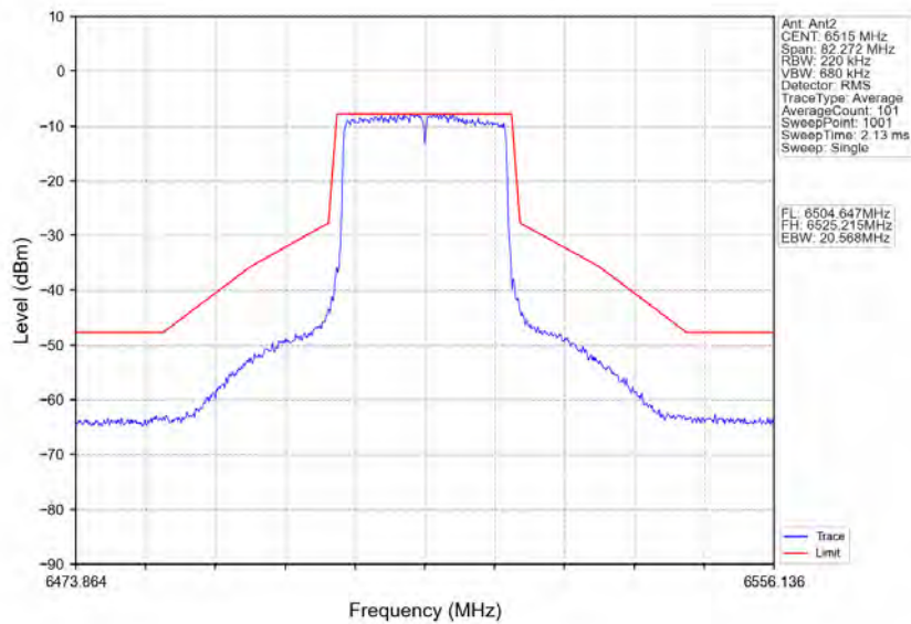
802.11ax(HEW20)_HCH_6515MHz_RU242_Left_Ant2_NTNV
