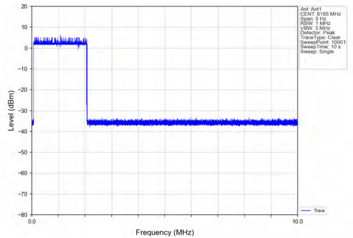
11AX160SISO-Ant 1-6185-Center-6185-Minimal
