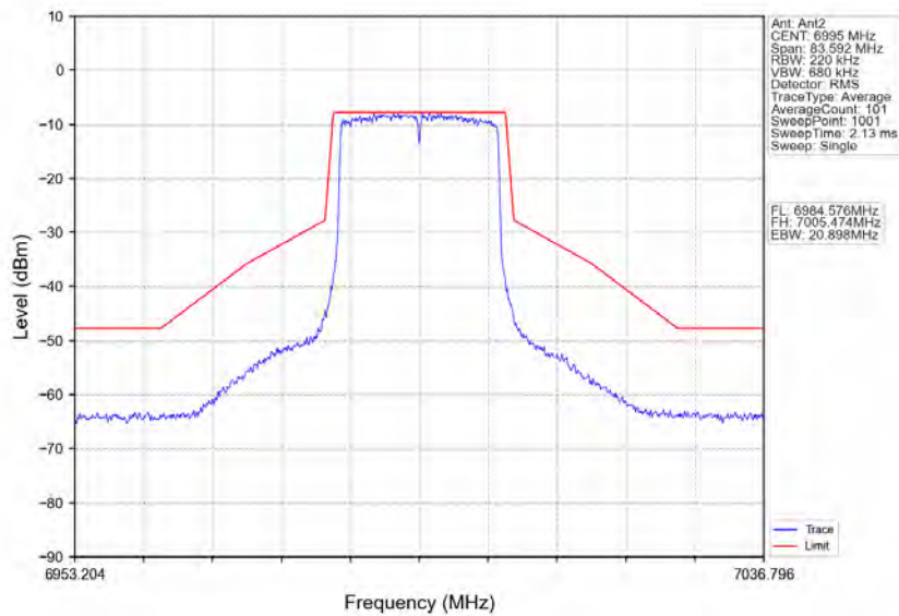
802.11ax(HEW20)_MCH_6995MHz_RU242_Left_Ant2_NTNV
