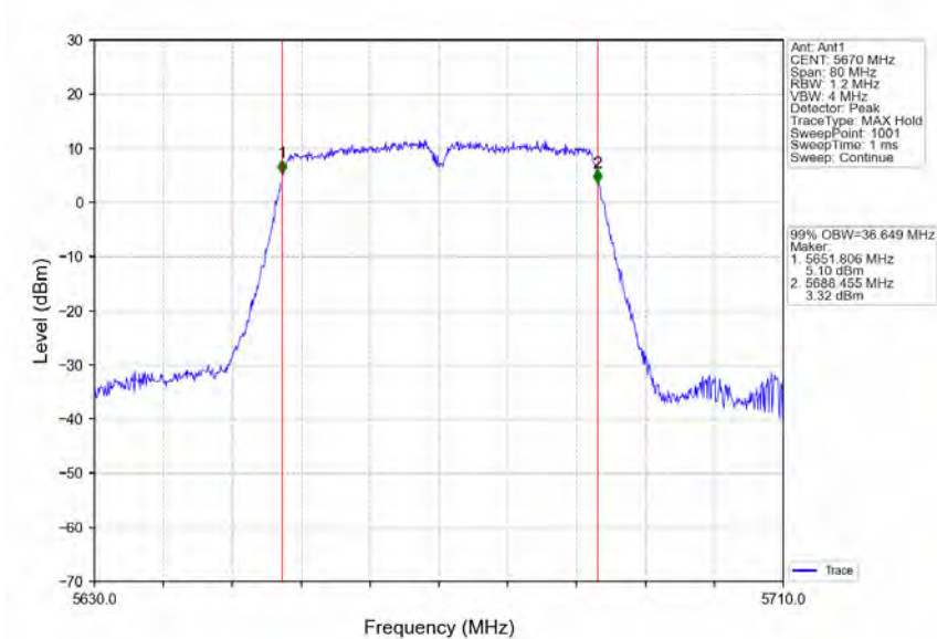
802.11n(HT40)_HCH_5670MHz_Ant1_NTNV
