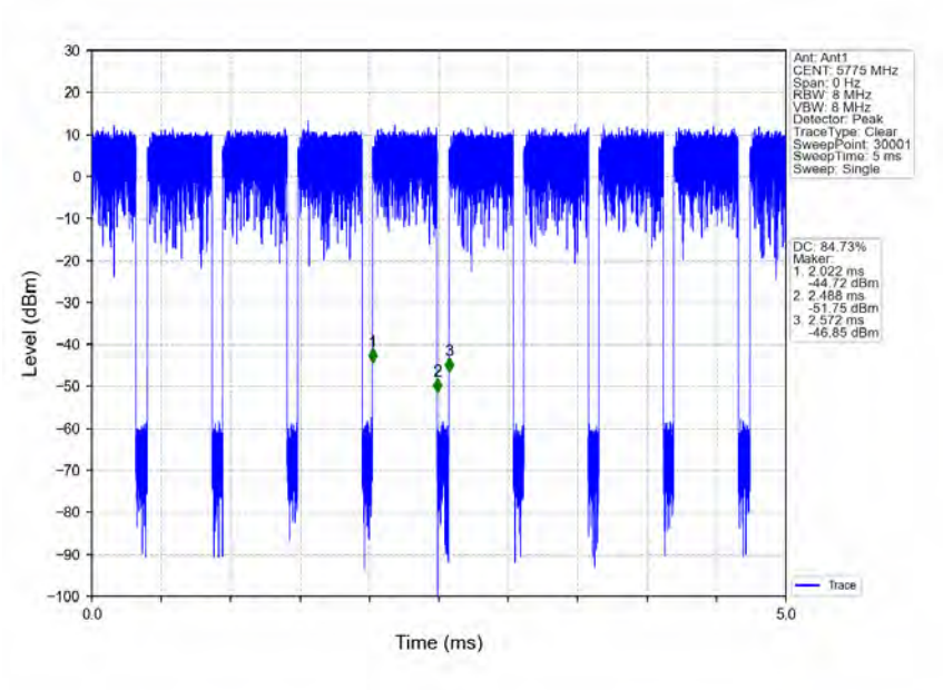
802.11ac(VHT80)_MCH_5775MHz_Ant1_NTNV
