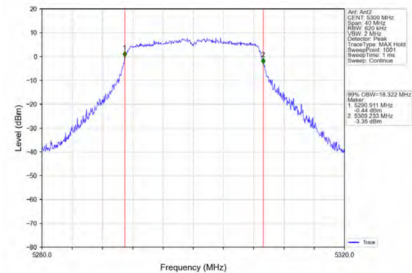
802.11ac(VHT20)_MCH_5300MHz_Ant2_NTNV
