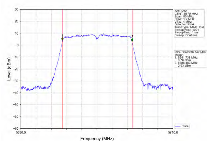
802.11n(HT40)_HCH_5670MHz_Ant2_NTNV
