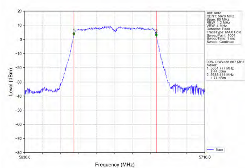
802.11n(HT40)_HCH_5670MHz_Ant2_NTNV
