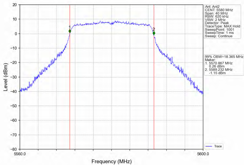
802.11n(HT20)_MCH_5580MHz_Ant2_NTNV
