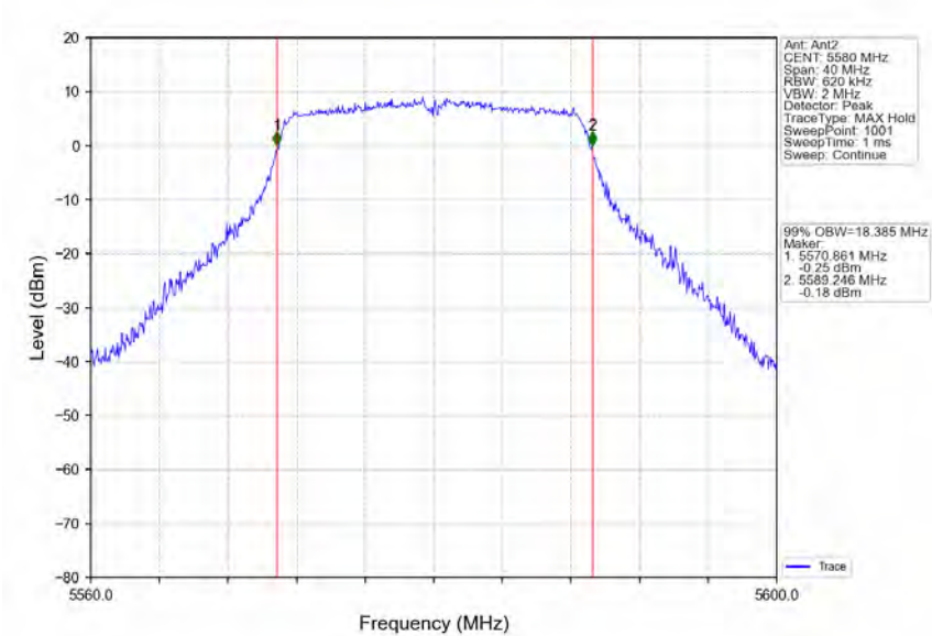
802.11n(HT20)_MCH_5580MHz_Ant2_NTNV
