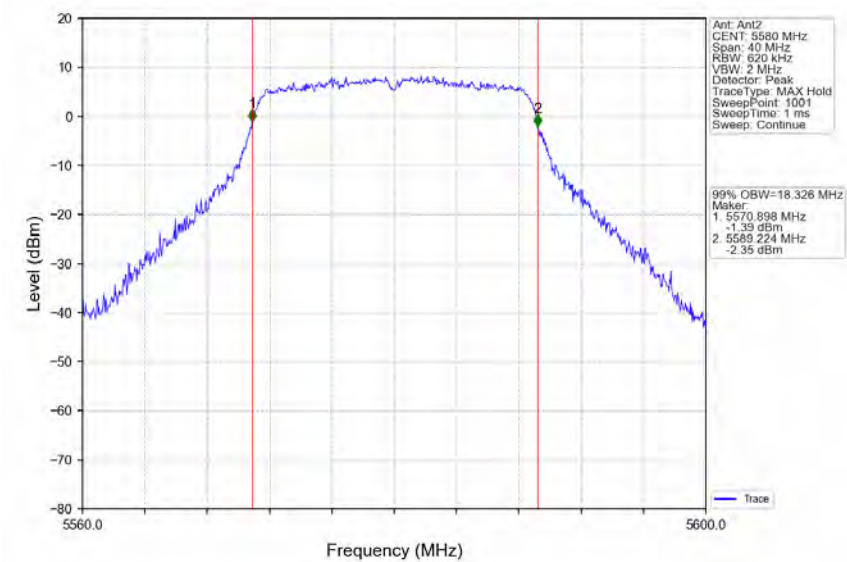
802.11ac(VHT20)_MCH_5580MHz_Ant2_NTNV
