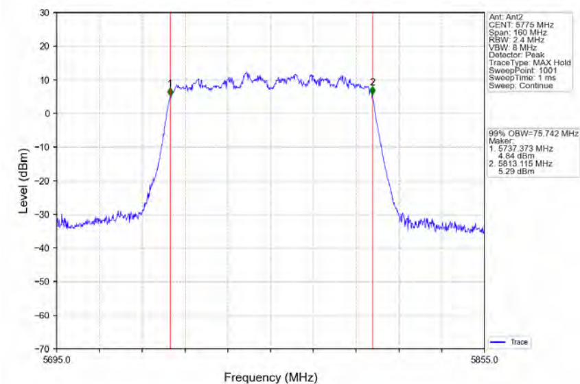
802.11ac(VHT80)_MCH_5775MHz_Ant2_NTNV
