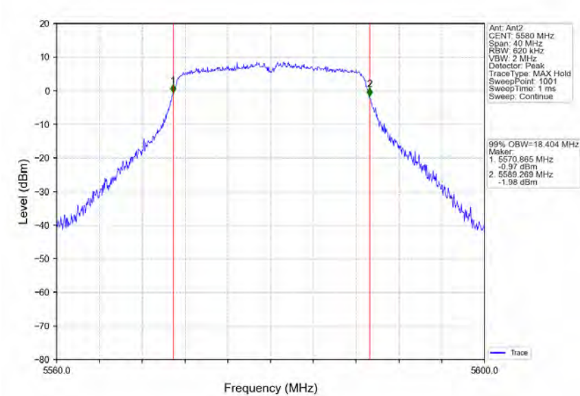
802.11ac(VHT20)_MCH_5580MHz_Ant2_NTNV
