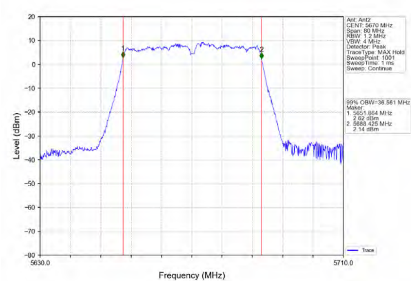
802.11ac(VHT40)_HCH_5670MHz_Ant2_NTNV
