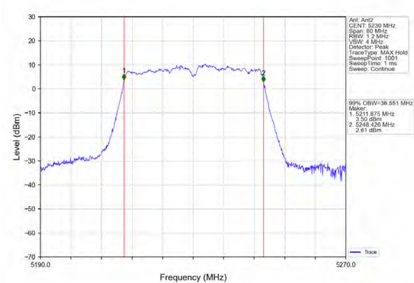
802.11ac(VHT40)_HCH_5230MHz_Ant2_NTNV
