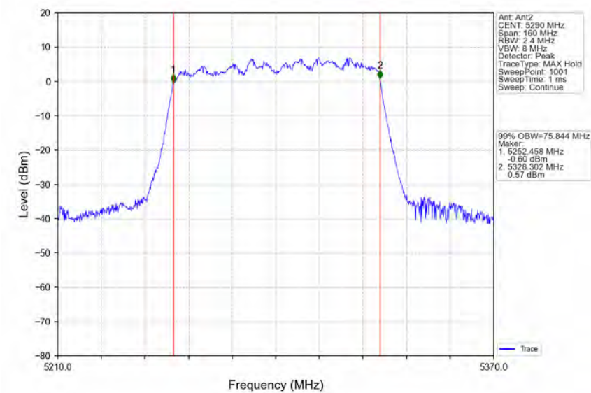
802.11ac(VHT80)_MCH_5290MHz_Ant2_NTNV
