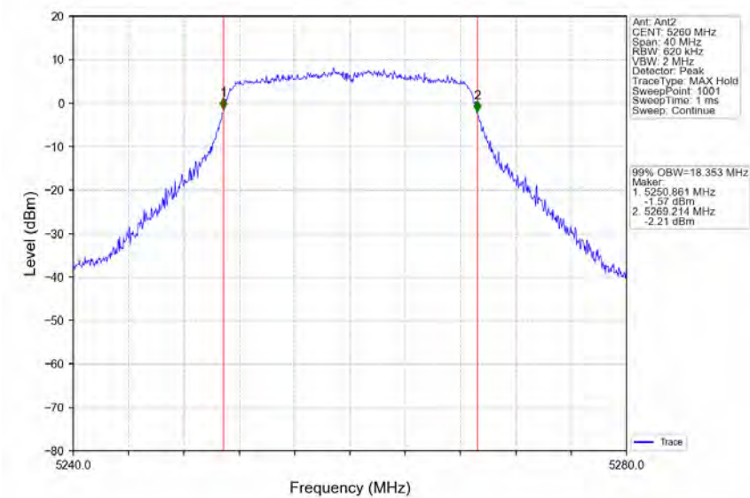
802.11ac(VHT20)_LCH_5260MHz_Ant2_NTNV
