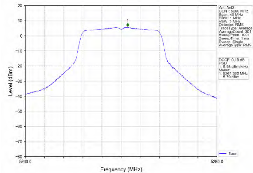
802.11a_LCH_5260MHz_Ant2_NTNV
