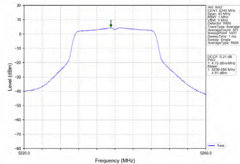
802.11n(HT20)_HCH_5240MHz_Ant2_NTNV
