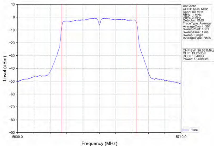
802.11ac(VHT40)_HCH_5670MHz_Ant2_NTNV
