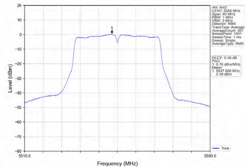
802.11n(HT40)_MCH_5550MHz_Ant2_NTNV
