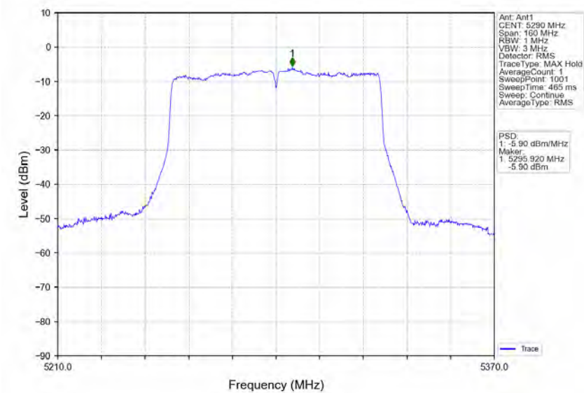
802.11ac(VHT80)_MCH_5290MHz_Ant1_NTNV
