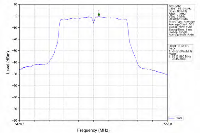
802.11ac(VHT40)_LCH_5510MHz_Ant2_NTNV
