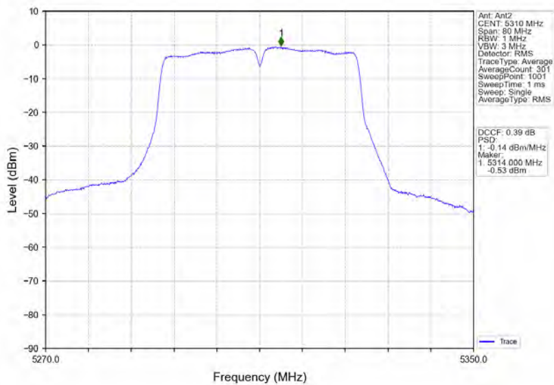
802.11ac(VHT40)_HCH_5310MHz_Ant2_NTNV
