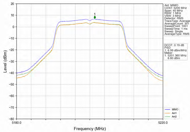
802.11ac(VHT20)_MCH_5200MHz_MIMO_NTNV
