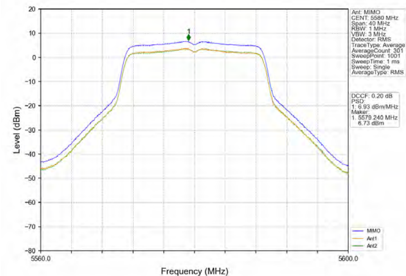
802.11ac(VHT20)_MCH_5580MHz_MIMO_NTNV
