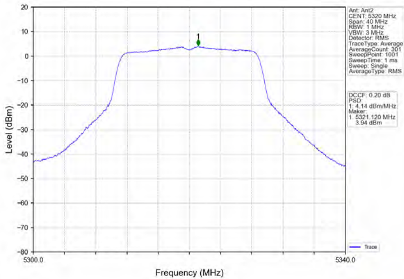
802.11ac(VHT20)_HCH_5320MHz_MIMO_NTNV
