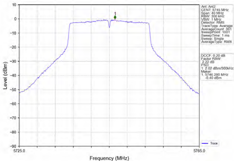
802.11n(HT20)_LCH_5745MHz_Ant2_NTNV
