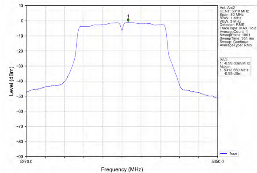
802.11n(HT40)_HCH_5310MHz_Ant2_NTNV
