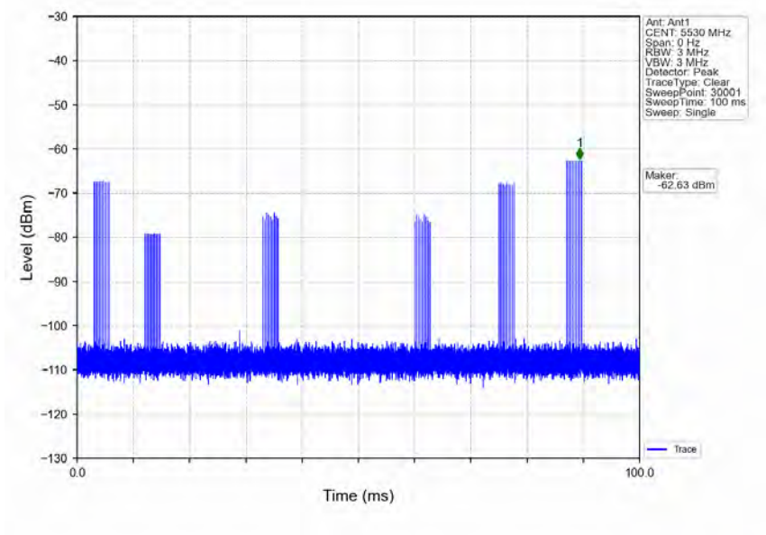
Signal Calibration_802.11ac(VHT80)_2C_5530MHz_RadarType6_Trial0
