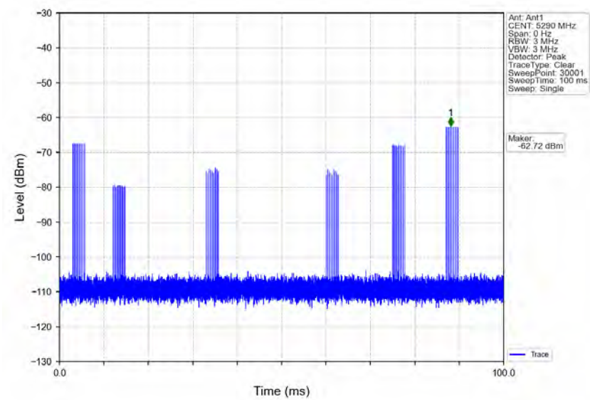
Signal Calibration_802.11ac(VHT80)_2A_5290MHz_RadarType6_Trial0
