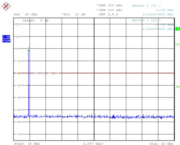
Fig.57 Conducted Spurious Emission
