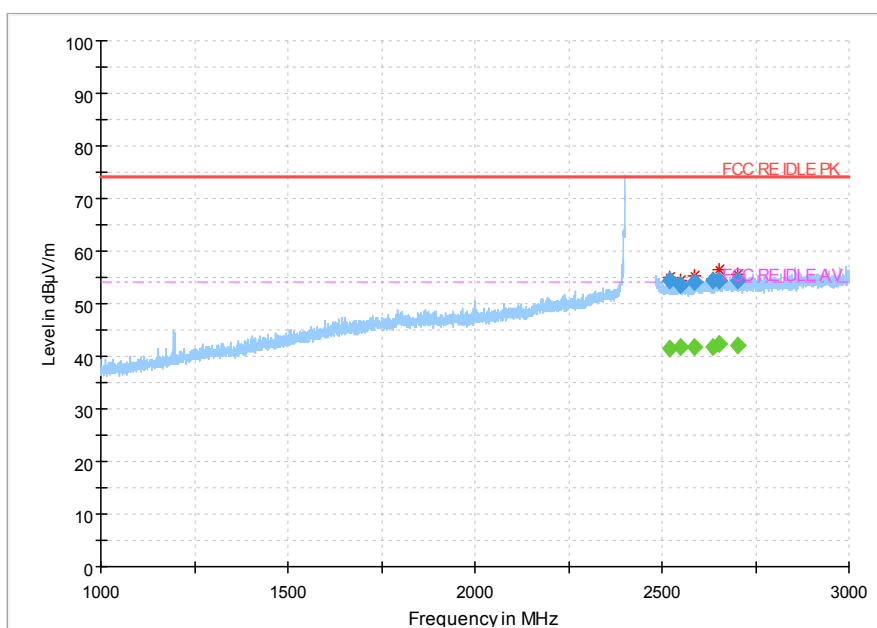
Fig.115 Radiated Spurious Emission (802.11 n-40MHz,Ch3,1GHz~3GHz)
