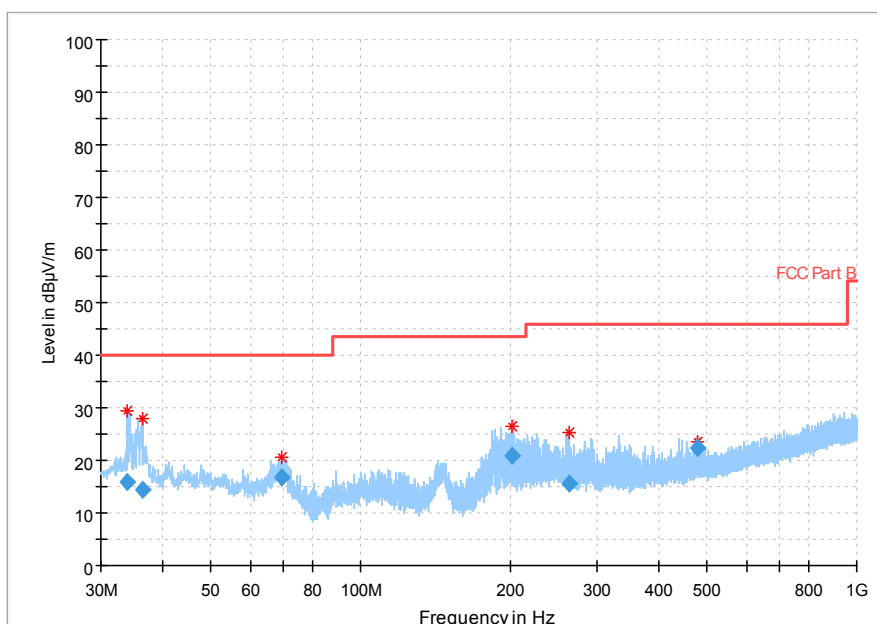
Fig.104 Radiated Spurious Emission (802.11g,Ch1,30MHz~1GHz)
