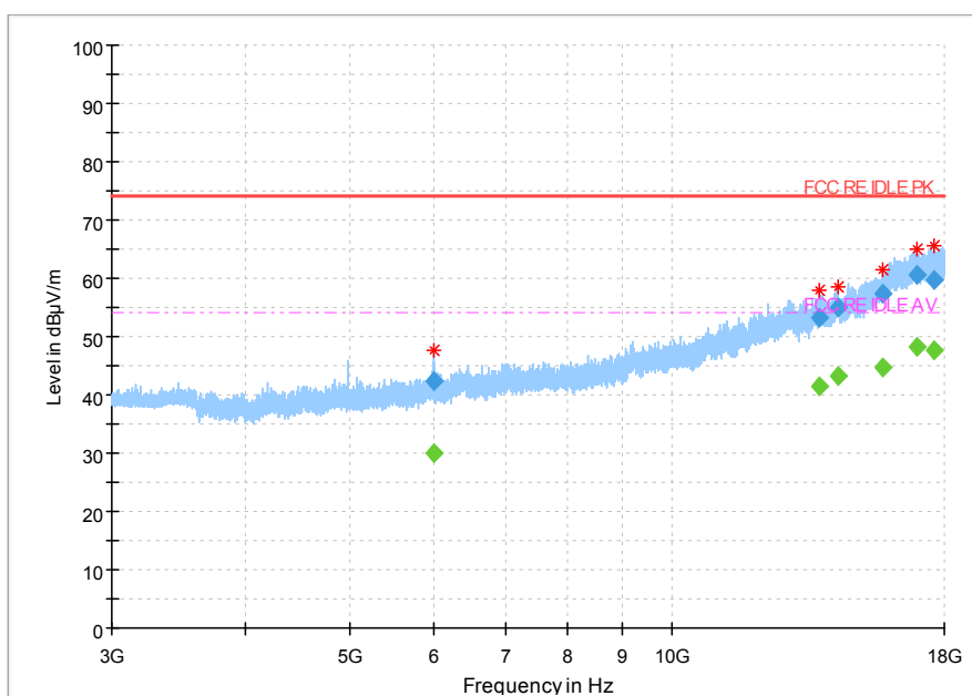
Fig.101 Radiated Spurious Emission (802.11b,Ch1,3GHz~18GHz)
