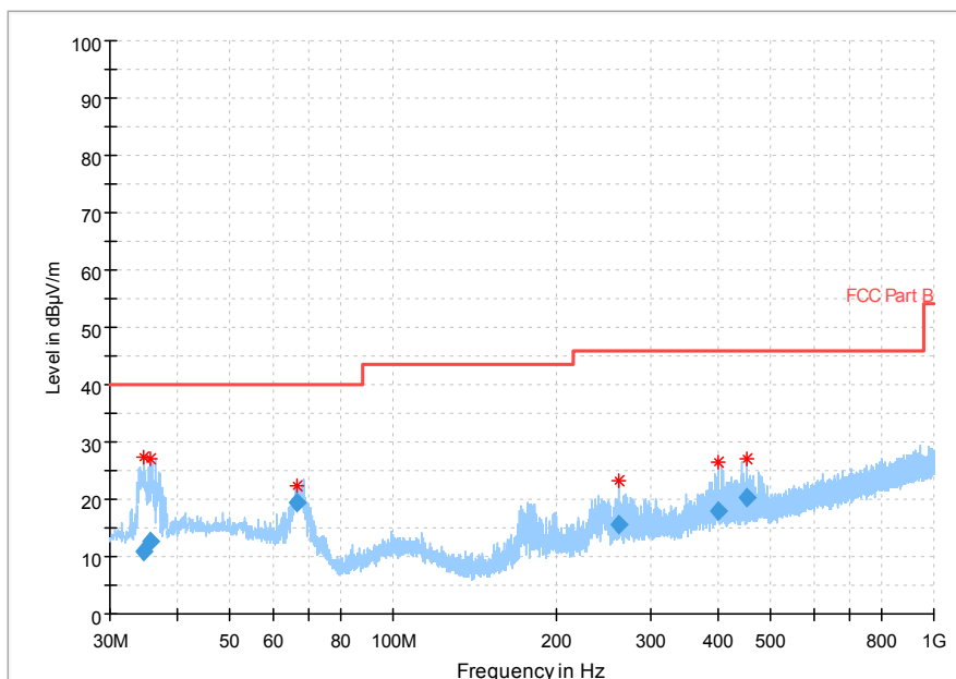
Fig.99 Radiated Spurious Emission (802.11b,Ch1,30MHz~1GHz)
