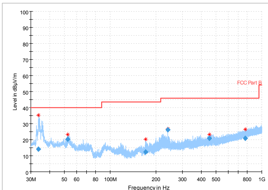
Fig.109 Radiated Spurious Emission (802.11 n-20MHz,Ch1,30MHz~1GHz)
