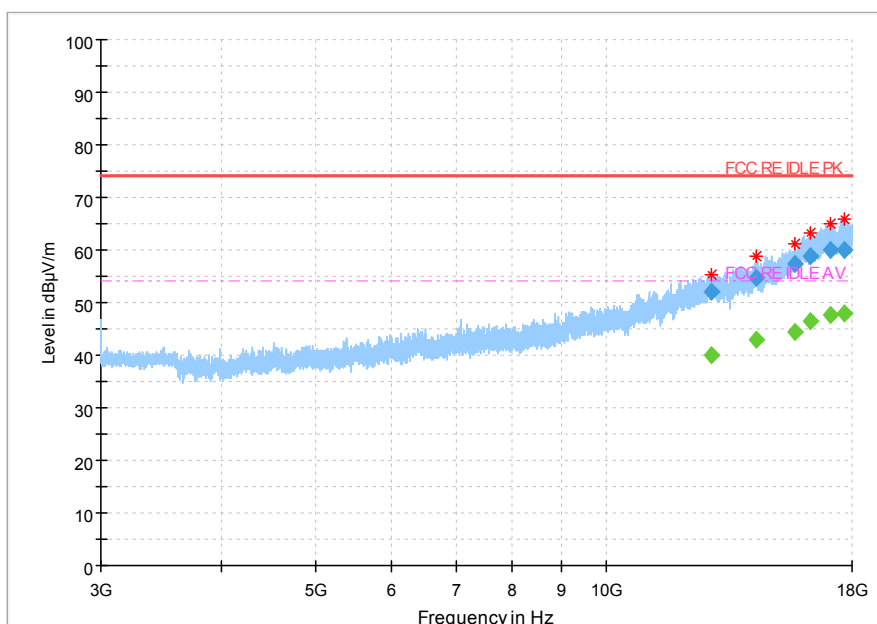
Fig.106 Radiated Spurious Emission (802.11g,Ch1,3GHz~18GHz)
