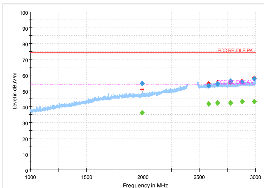
Fig.100 Radiated Spurious Emission (802.11b,Ch1,1GHz~3GHz)
