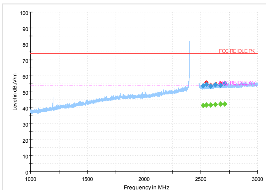
Fig.110 Radiated Spurious Emission (802.11 n-20MHz,Ch1,1GHz~3GHz)
