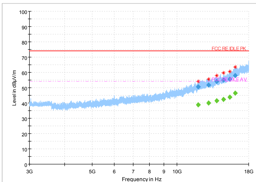
Fig.111 Radiated Spurious Emission (802.11 n-20MHz,Ch1,3GHz~18GHz)
