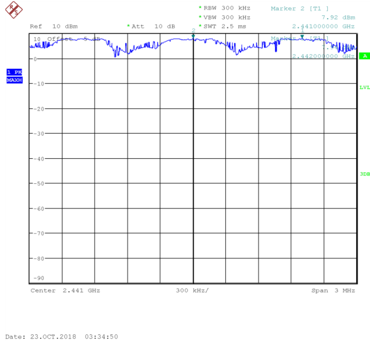
Fig.84 Carrier separation measurement: 8DPSK, Ch39
