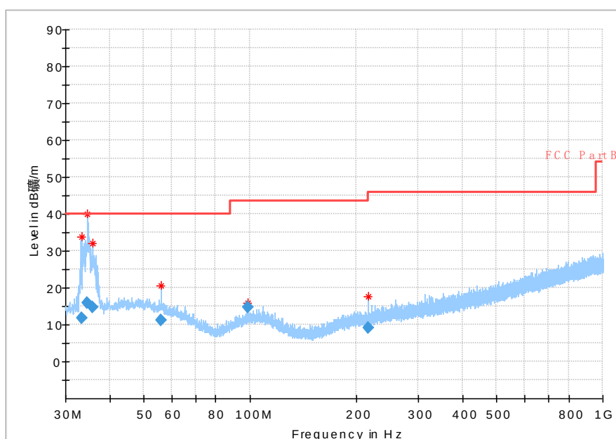
Fig.45 Radiated emission: \pi/4 DQPSK, Ch0, 30MHz~1GHz
