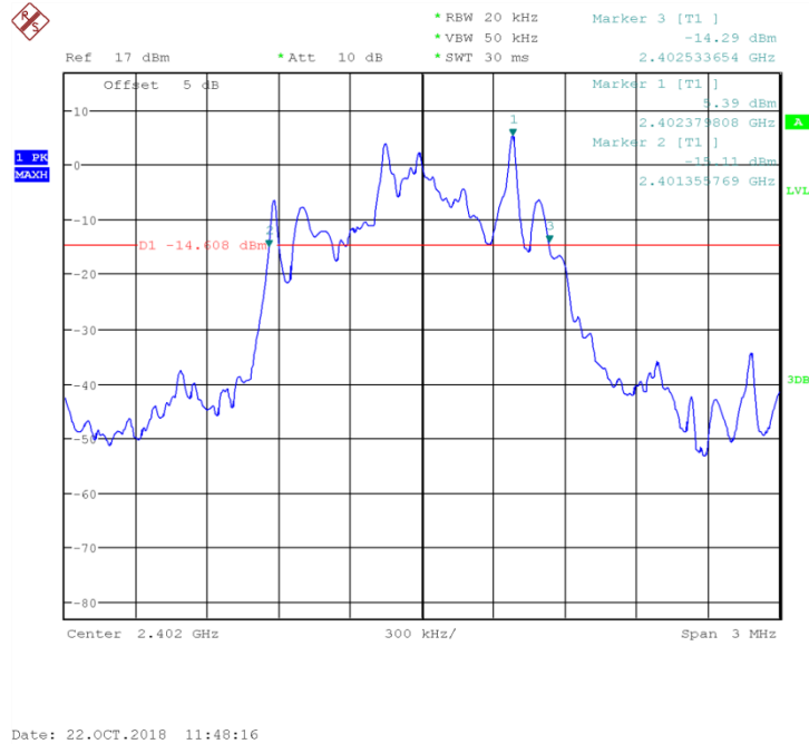
Fig.76 20dB Bandwidth: \pi/4 DQPSK, Ch0
