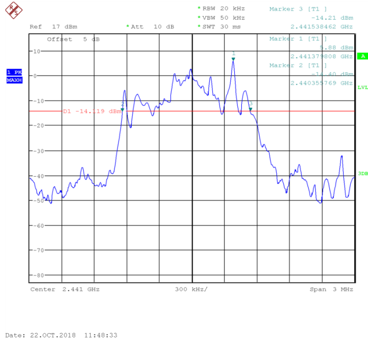
Fig.77 20dB Bandwidth: \pi/4 DQPSK, Ch39
