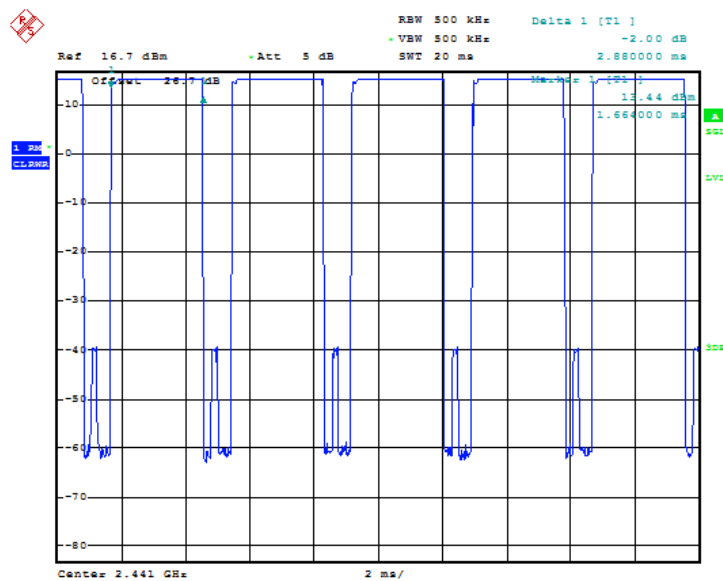
Fig.58 Number of Transmissions Measurement: Ch39, Packet DH3
