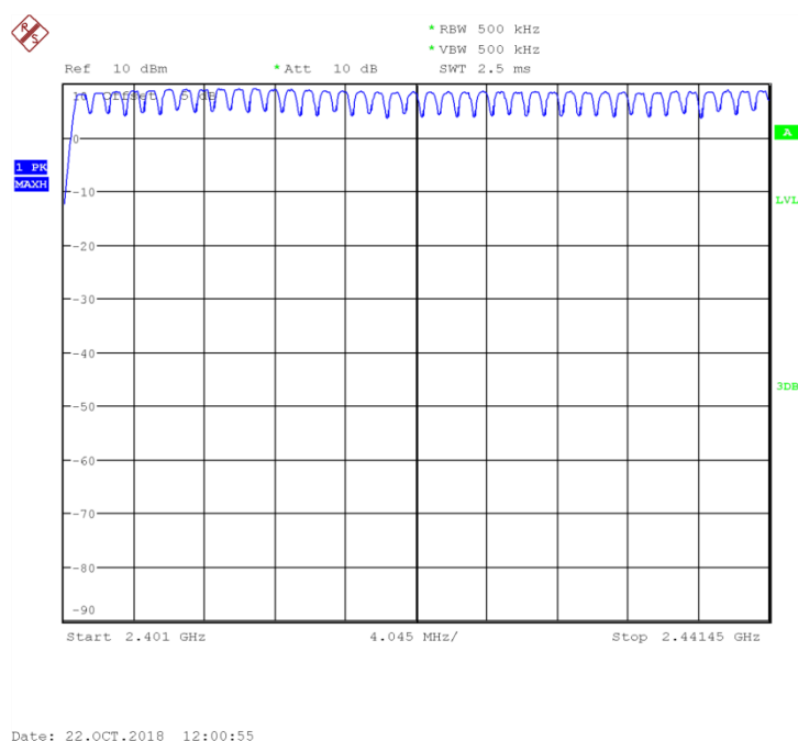
Fig.85 Number of hopping frequency: GFSK, Ch0~39
