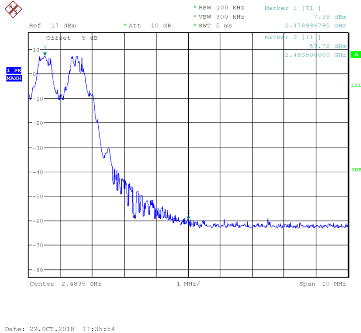
Fig.21 Frequency Band Edge: 8DPSK, Ch78, Hopping ON
