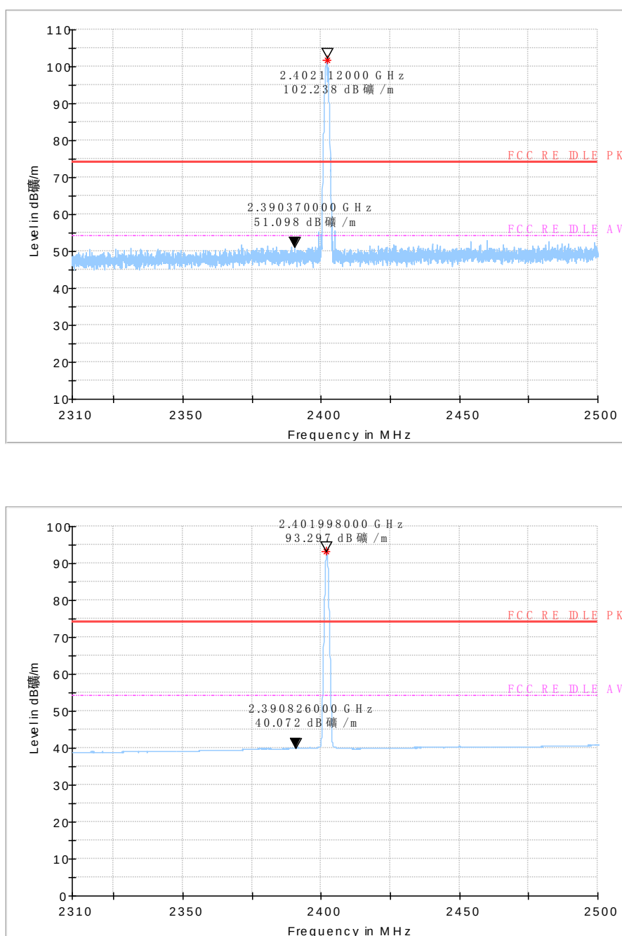
Fig.43 Radiated emission (Low): GFSK, low channel
