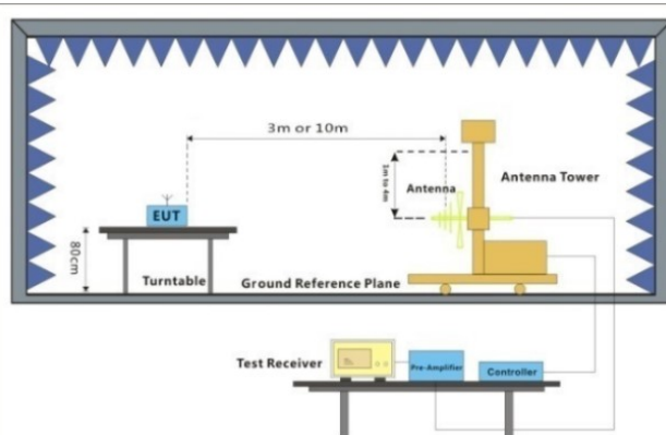
Figure 2. Above 30MHz
