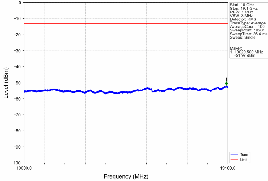
Band2_RMC_HCH_1907.6MHz_12.2kbps RMC_NTNV
