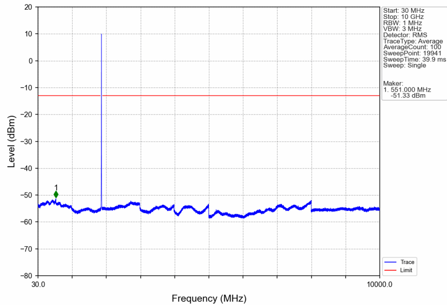
Band2_RMC_MCH_1880MHz_12.2kbps RMC_NTNV
