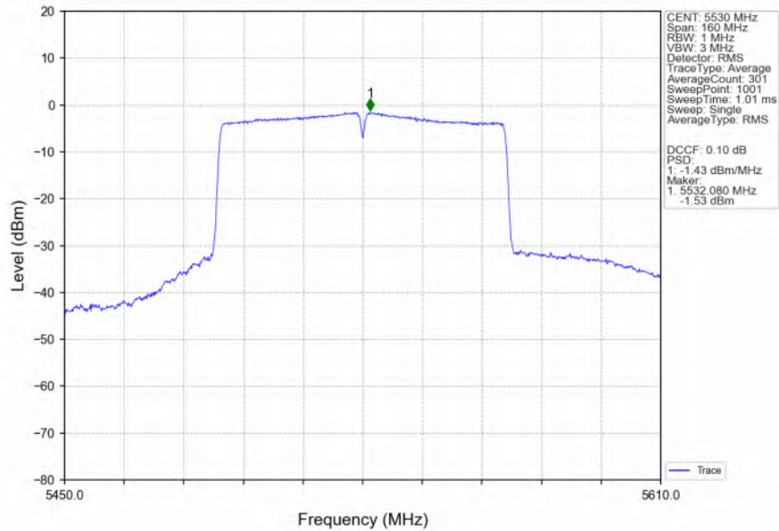
802.11ac(VHT80)_LCH_5530MHz_Ant3_NTNV
