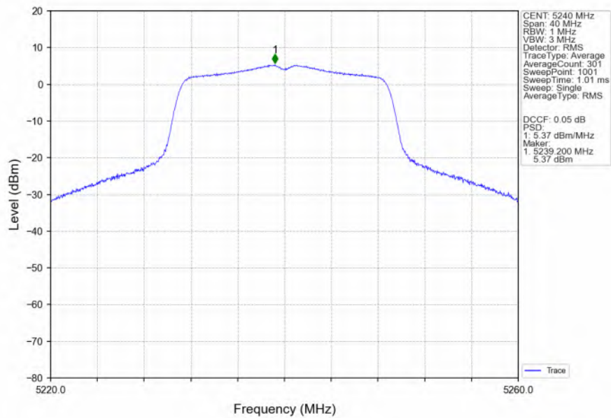
802.11n(HT20)_HCH_5240MHz_Ant3_NTNV
