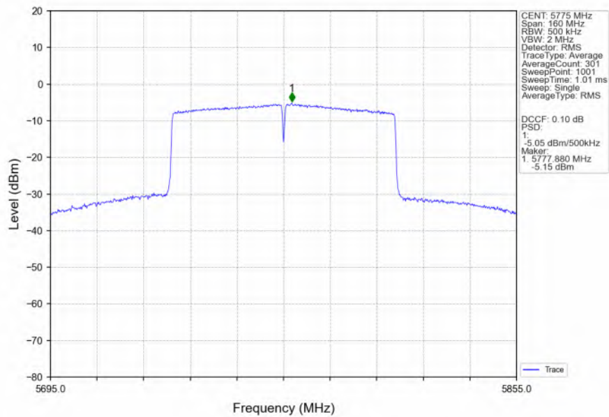
802.11ac(VHT80)_MCH_5775MHz_MIMO_NTNV
