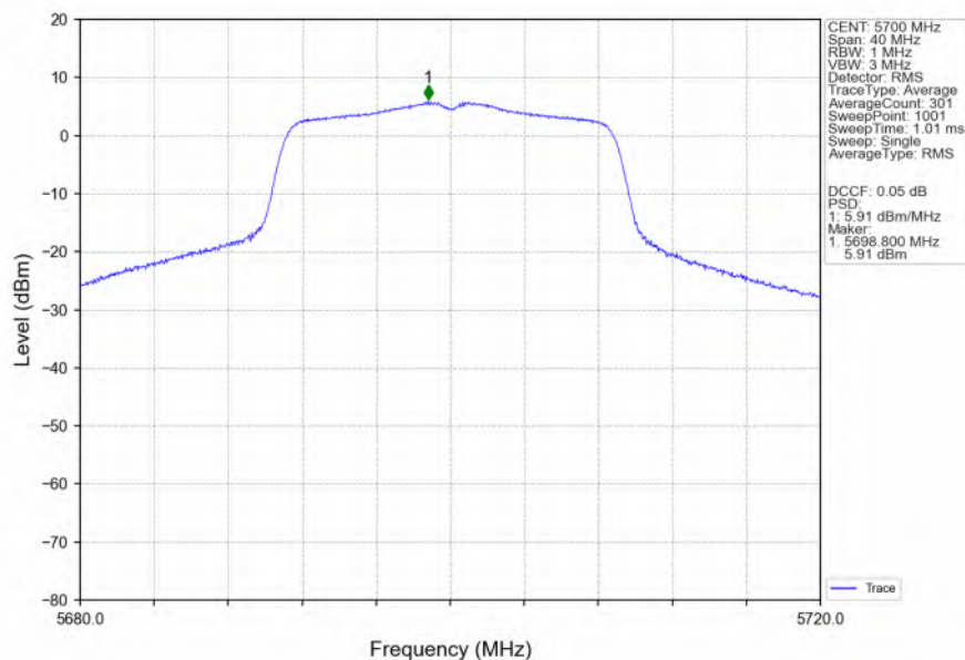
802.11n(HT20)_HCH_5700MHz_Ant3_NTNV
