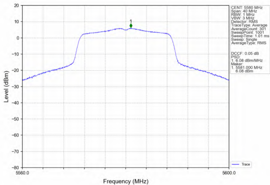
802.11n(HT20)_MCH_5580MHz_Ant2_NTNV
