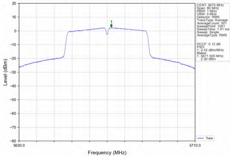
802.11n(HT40)_HCH_5670MHz_MIMO_NTNV
