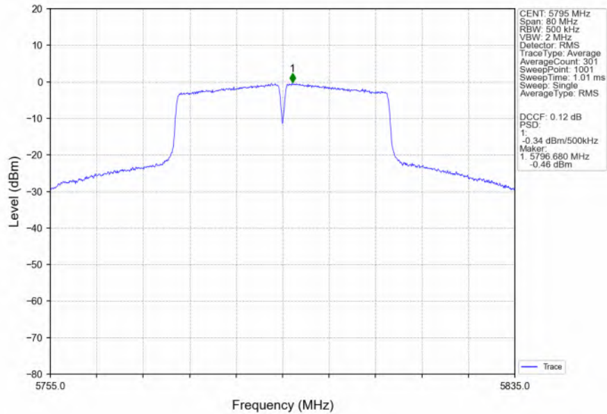
802.11n(HT40)_HCH_5795MHz_Ant3_NTNV
