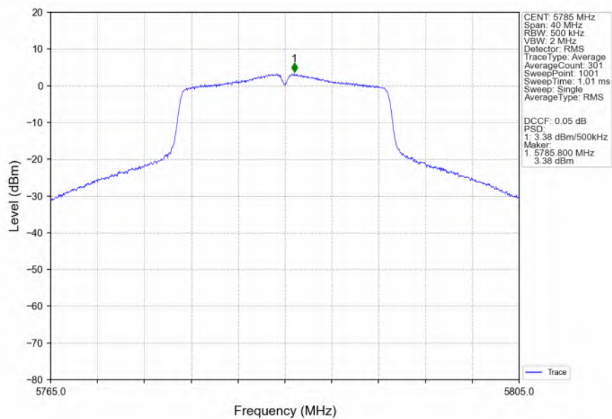
802.11n(HT20)_MCH_5785MHz_Ant2_NTNV
