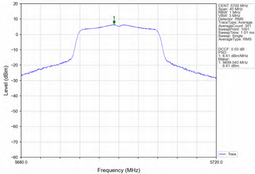
802.11a_HCH_5700MHz_Ant3_NTNV
