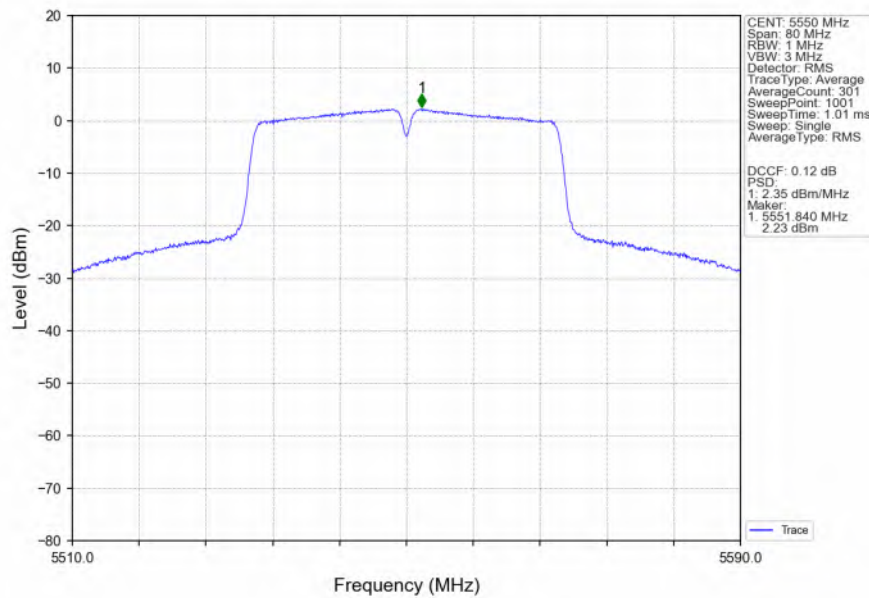
802.11n(HT40)_MCH_5550MHz_Ant3_NTNV
