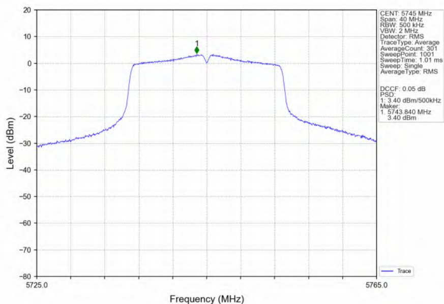
802.11n(HT20)_LCH_5745MHz_Ant3_NTNV
