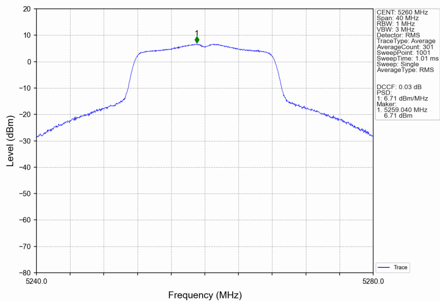
802.11a_LCH_5260MHz_Ant3_NTNV
