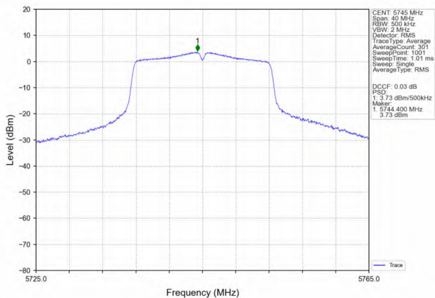
802.11a LCH 5745MHz Ant3 NTN
