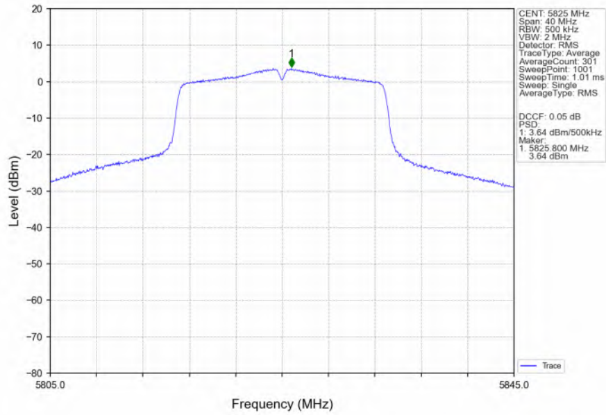
802.11n(HT20)_HCH_5825MHz_Ant3_NTNV
