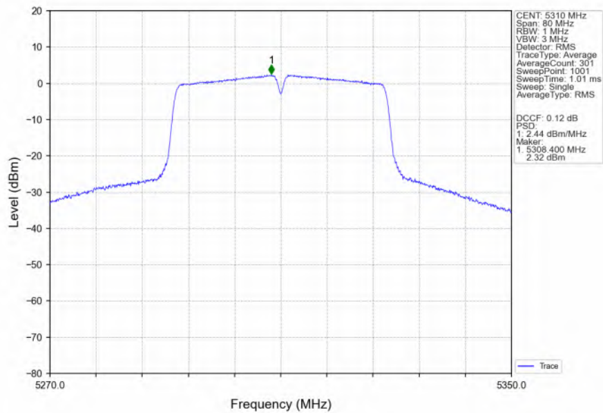
802.11n(HT40)_HCH_5310MHz_Ant3_NTNV
