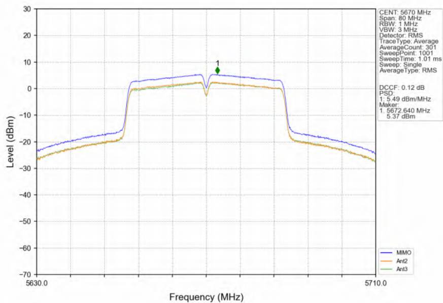
802.11n(HT40)_HCH_5670MHz_MIMO_NTNV
