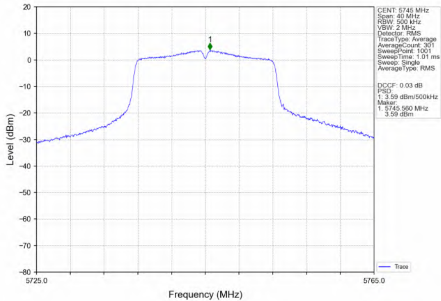
802.11a LCH 5745MHz Ant3 NTN
