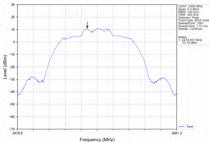
Pi/4DQPSK_2DH5_HCH_2480MHz_Ant2_NTNV
