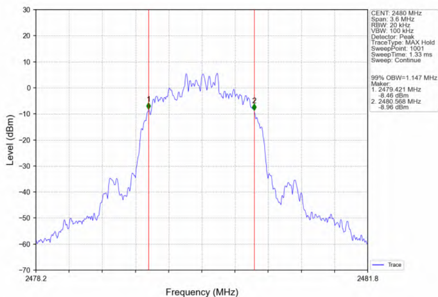
Pi/4DQPSK_2DH5_HCH_2480MHz_Ant2_NTNV
