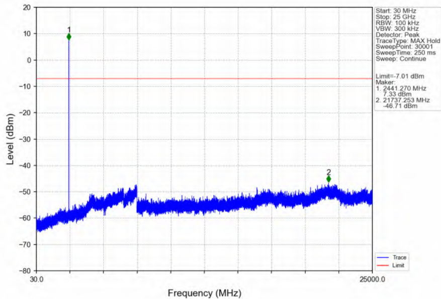
Pi/4DQPSK_2DH5_MCH_2441MHz_Ant2_NTNV
