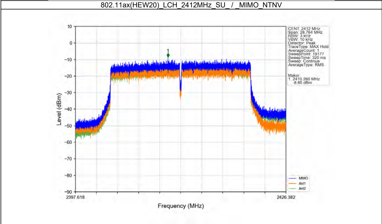
802.11ax(HEW20) LCH 2412MHz_SU / MIMO NTN
