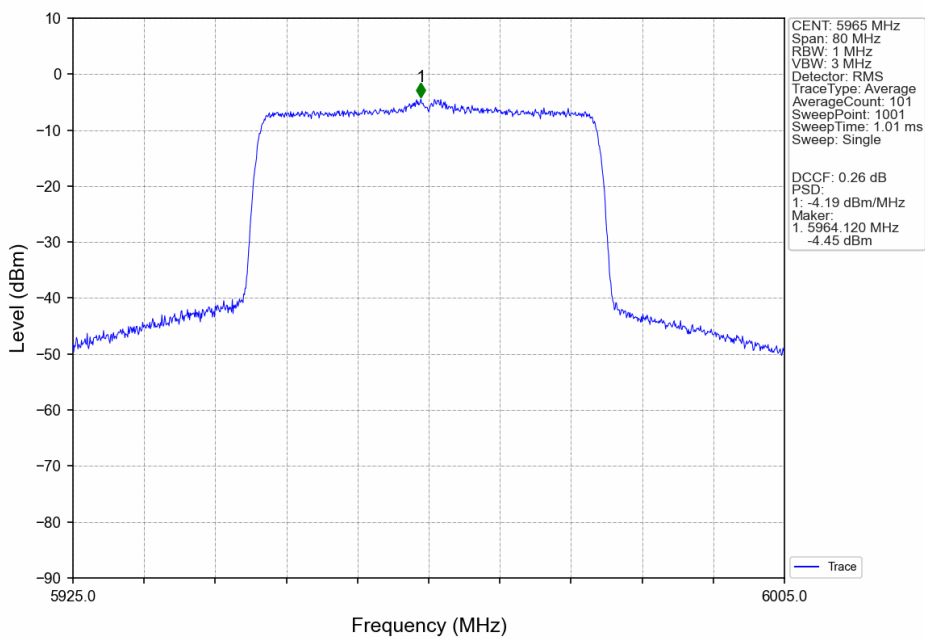
802.11ax(HEW40)_LCH_5965MHz_SU_/_ANT2_NTNV
