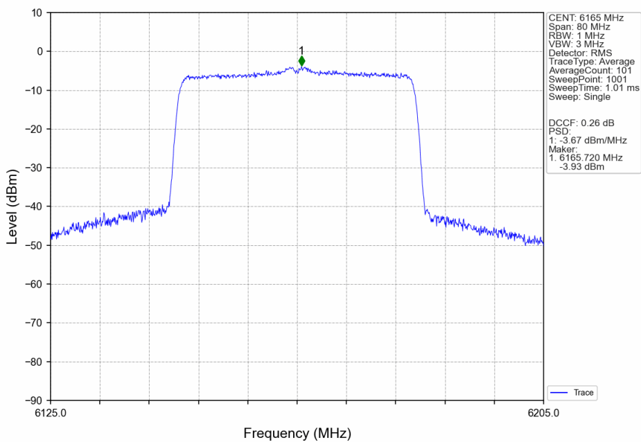
802.11ax(HEW40)_MCH_6165MHz_SU_/_ANT3_NTNV
