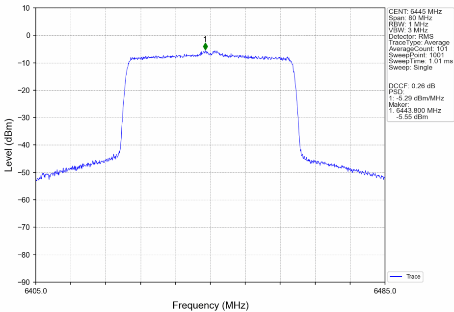
802.11ax(HEW40)_LCH_6445MHz_SU_/_ANT2_NTNV
