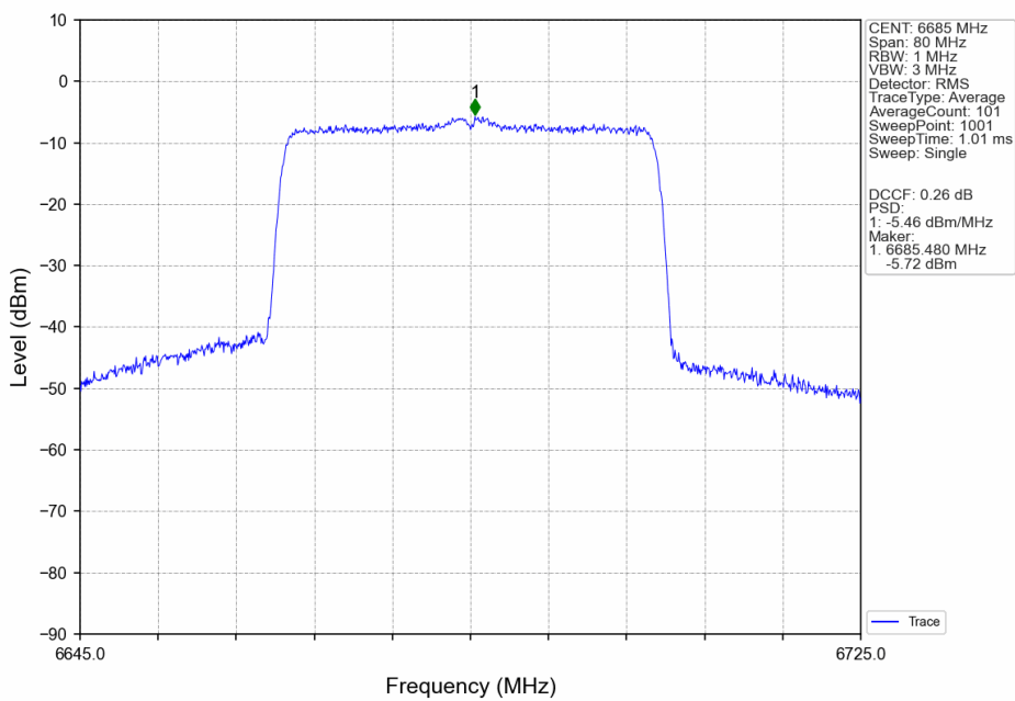
802.11ax(HEW40)_MCH_6685MHz_SU_/_ANT3_NTNV
