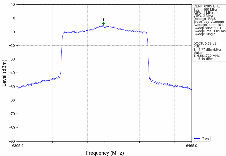
802.11ax(HEW80)_HCH_6385MHz_SU_/_ANT3_NTNV
