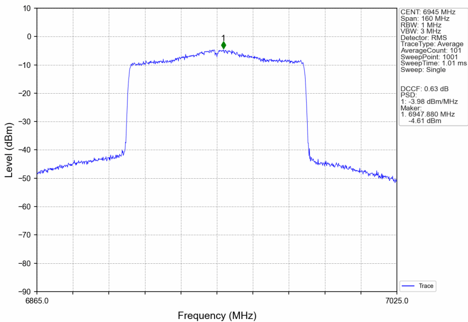
802.11ax(HEW80)_LCH_6945MHz_SU_/_ANT3_NTNV
