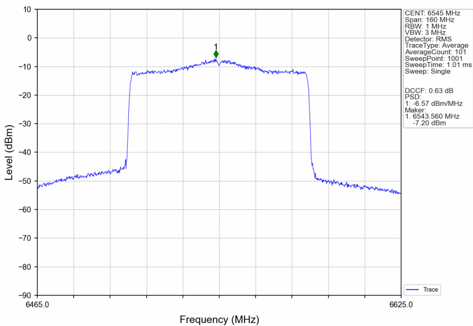
802.11ax(HEW80)_HCH_6545MHz_SU_/_MIMO_NTNV
