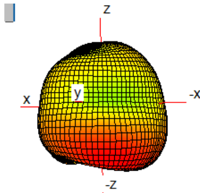
ANT2
