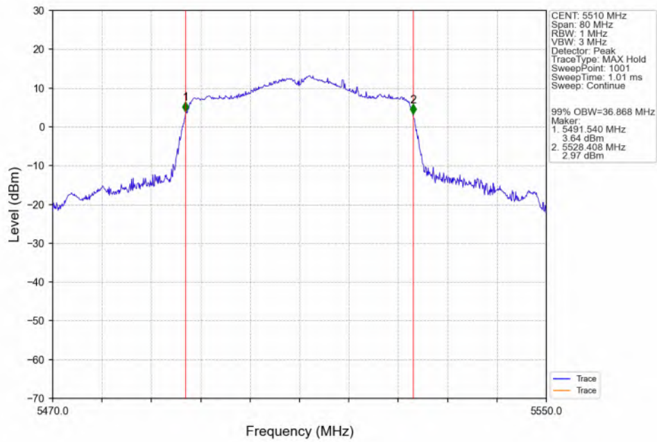
802.11n(HT40)_LCH_5510MHz_ANT3_NTNV
