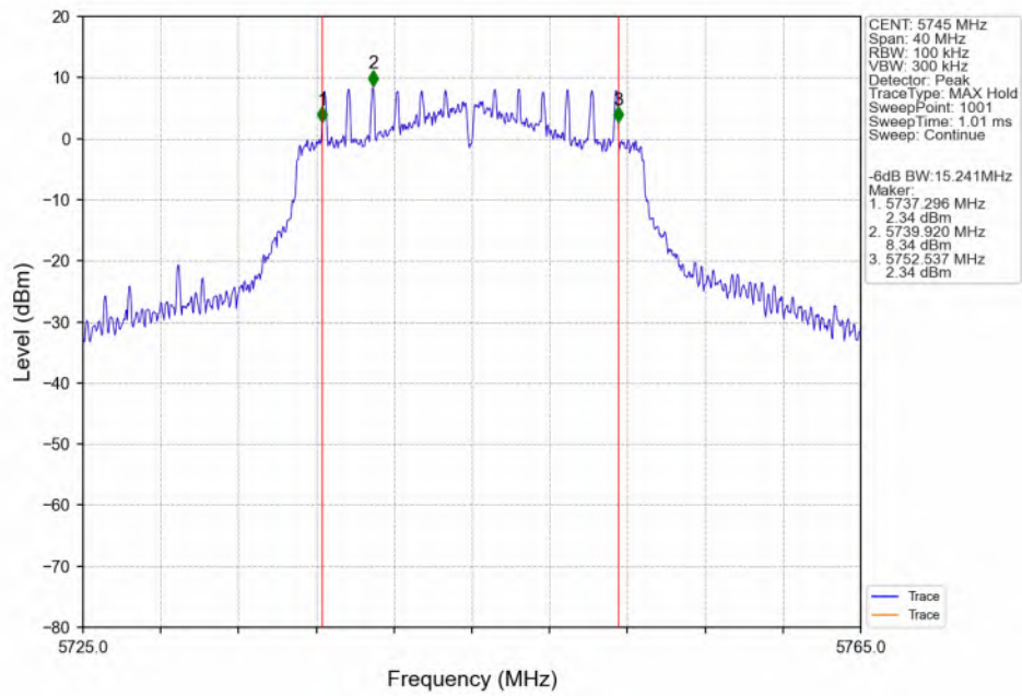
802.11n(HT20)_LCH_5745MHz_ANT3_NTNV
