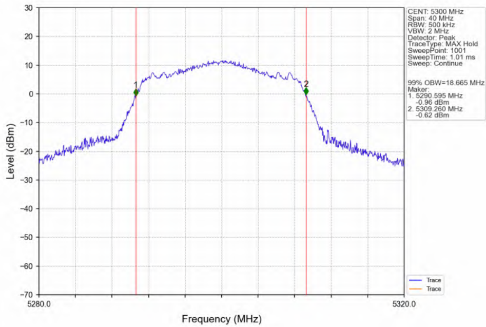
802.11ax(HEW20)_MCH_5300MHz_SU / _ANT3_NTNV
