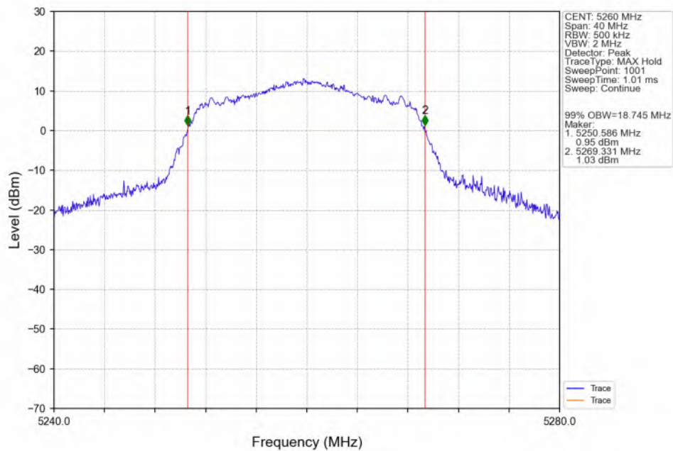
802.11n(HT20)_LCH_5260MHz_ANT3_NTNV
