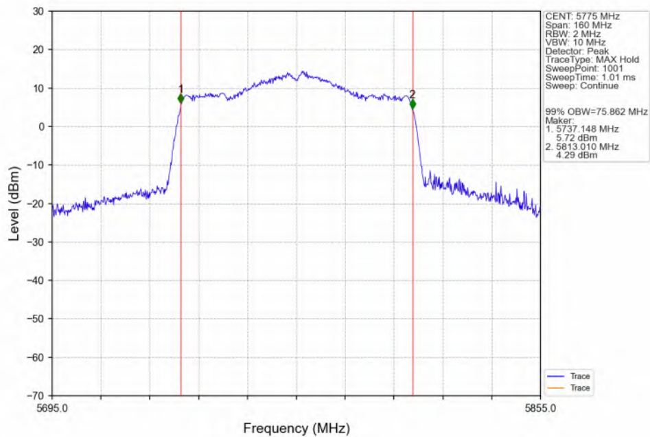
802.11ac(VHT80)_MCH_5775MHz_ANT3_NTNV
