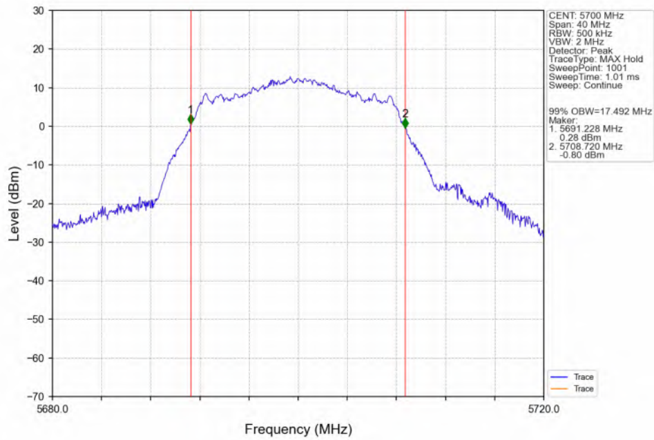
802.11a_HCH_5700MHz_ANT3_NTNV
