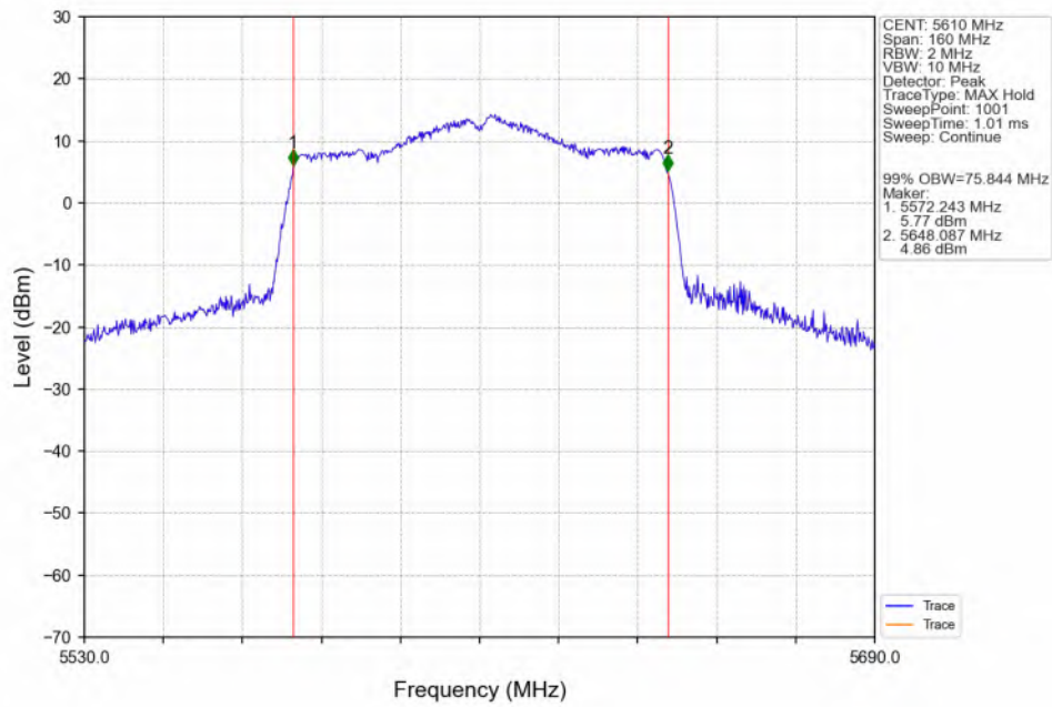
802.11ac(VHT80)_HCH_5610MHz_ANT3_NTNV
