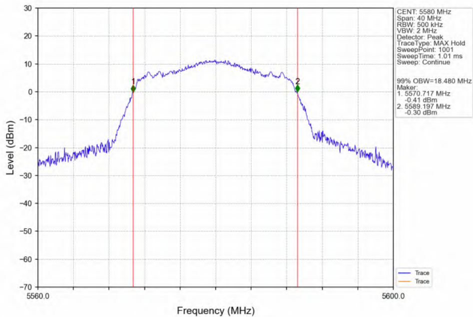
802.11ax(HEW20)_MCH_5580MHz_SU / _ANT3_NTNV
