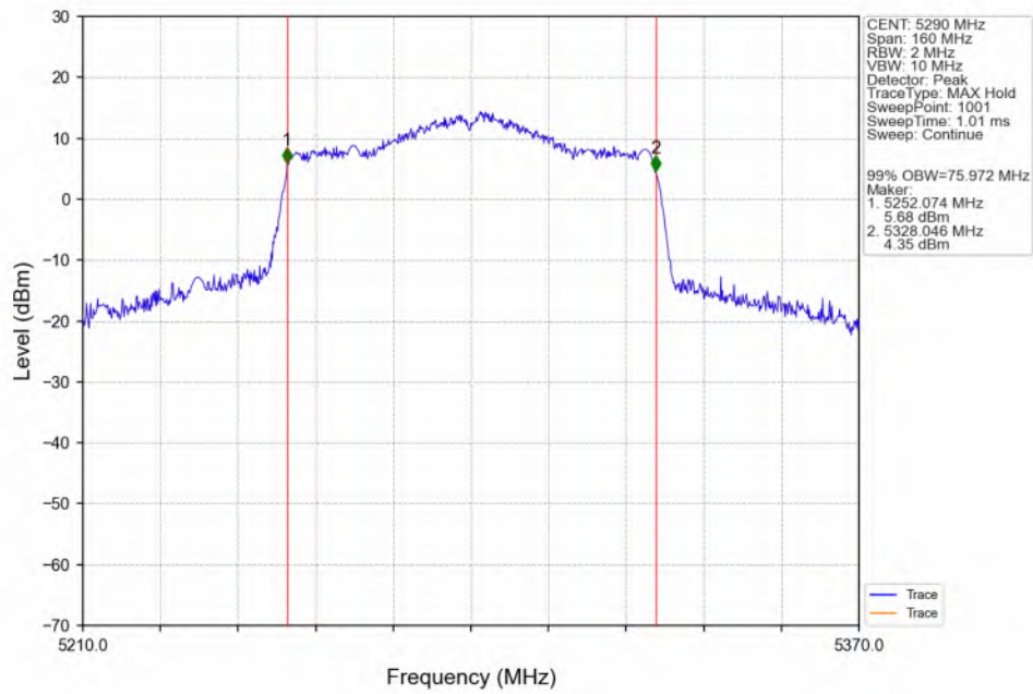
802.11ac(VHT80)_MCH_5290MHz_ANT3_NTNV
