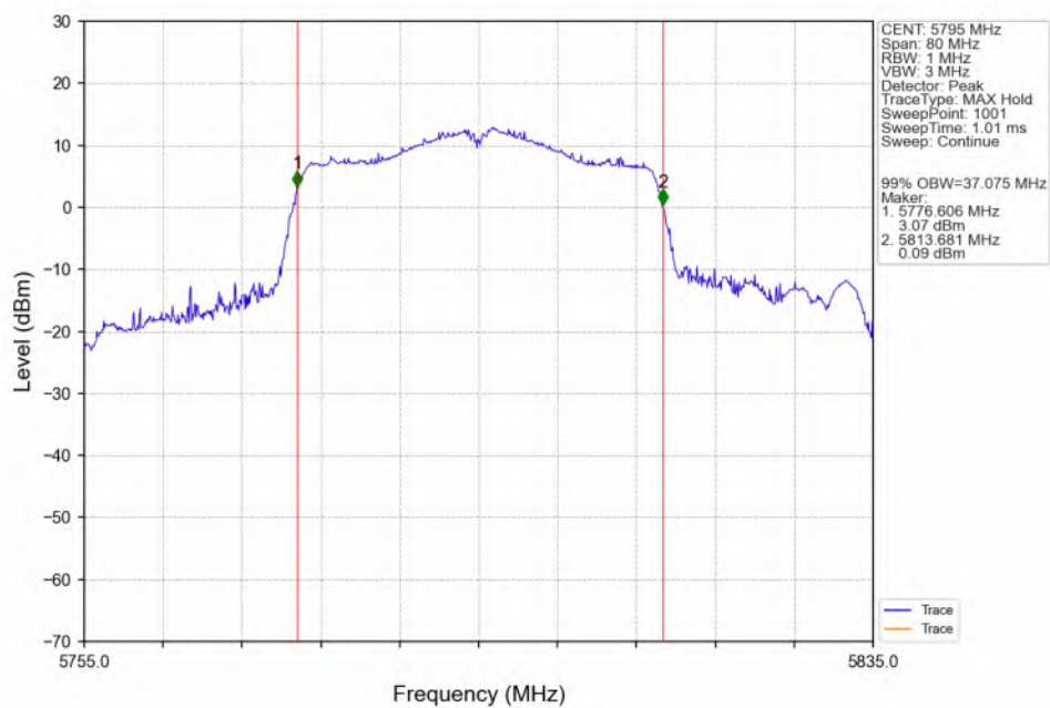
802.11n(HT40)_HCH_5795MHz_ANT3_NTNV
