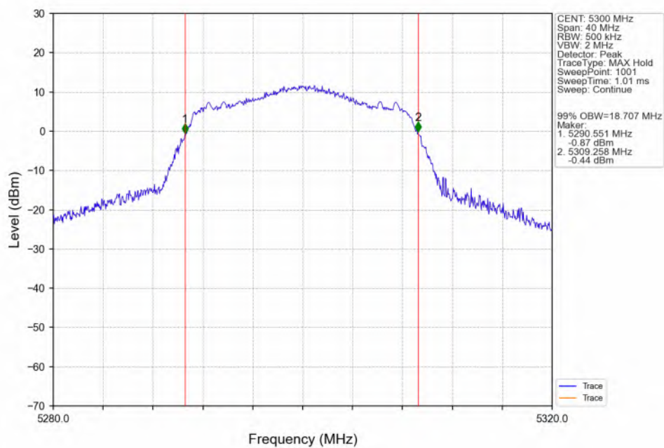
802.11ax(HEW20)_MCH_5300MHz_SU / _ANT3_NTNV
