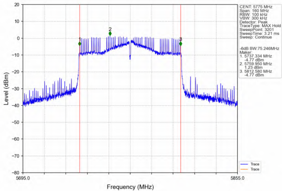
802.11ac(VHT80)_MCH_5775MHz_ANT3_NTNV
