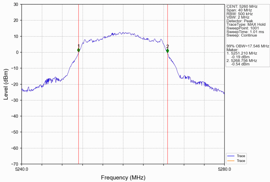
802.11a_LCH_5260MHz_ANT3_NTNV
