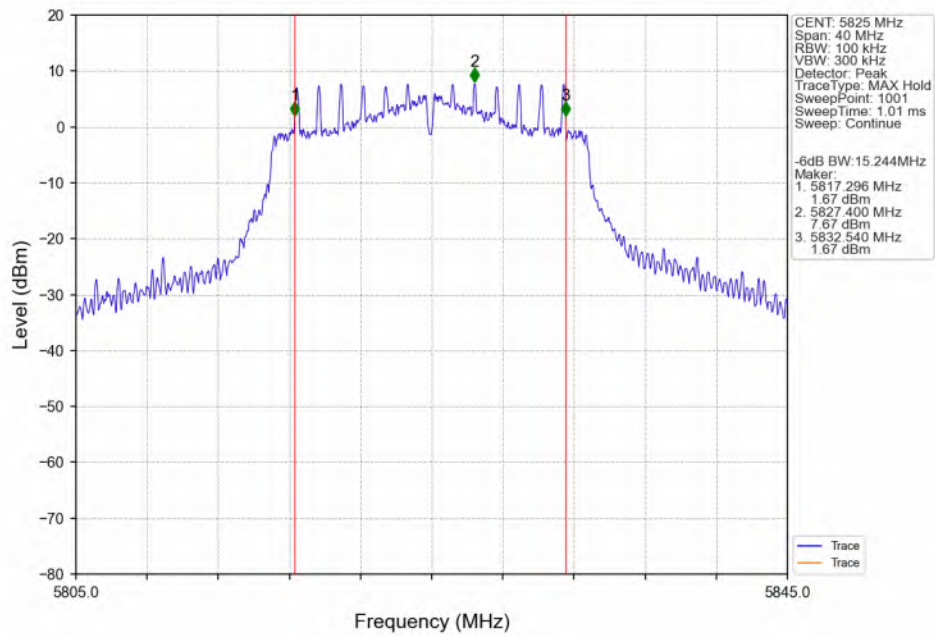
802.11n(HT20)_HCH_5825MHz_ANT3_NTNV
