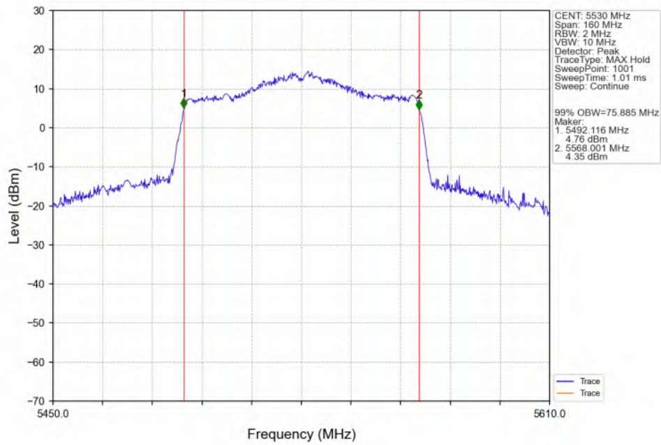
802.11ac(VHT80)_LCH_5530MHz_ANT3_NTNV
