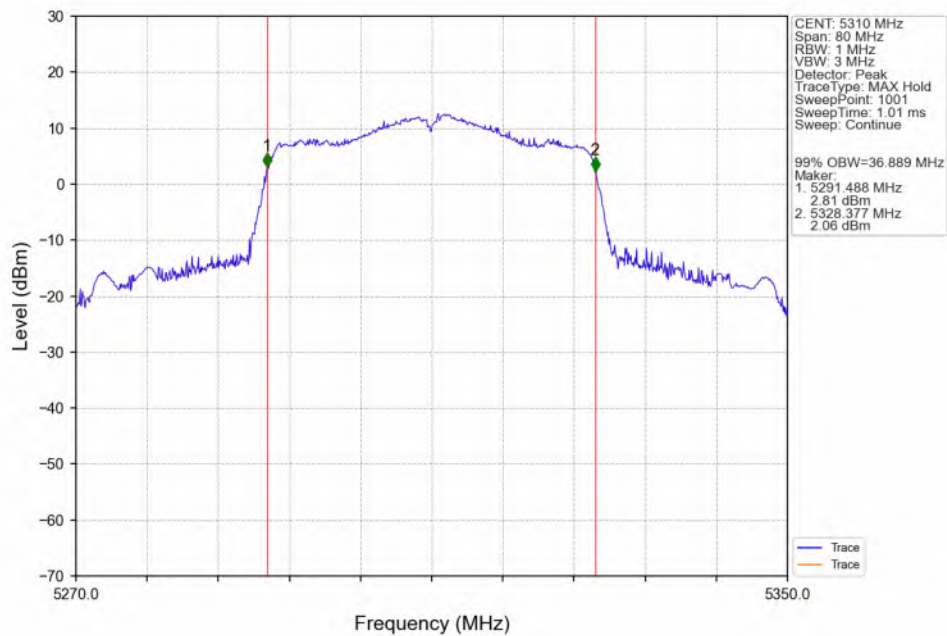
802.11n(HT40)_HCH_5310MHz_ANT3_NTNV
