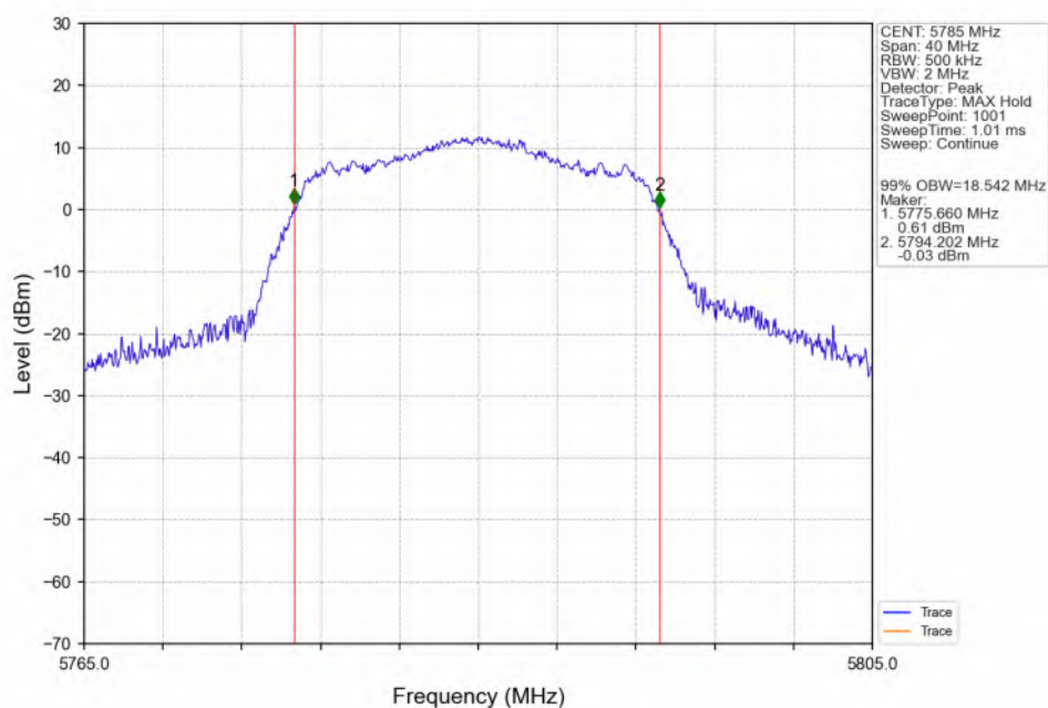
802.11ax(HEW20)_MCH_5785MHz_SU_/_ANT3_NTNV
