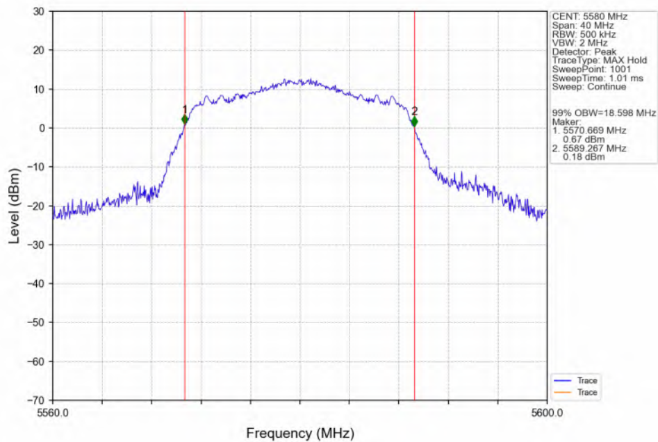
802.11n(HT20)_MCH_5580MHz_ANT3_NTNV
