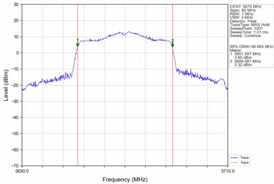
802.11n(HT40)_HCH_5670MHz_ANT3_NTNV
