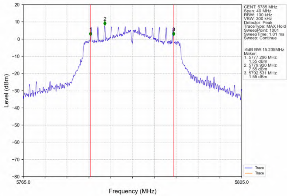
802.11n(HT20)_MCH_5785MHz_ANT3_NTNV
