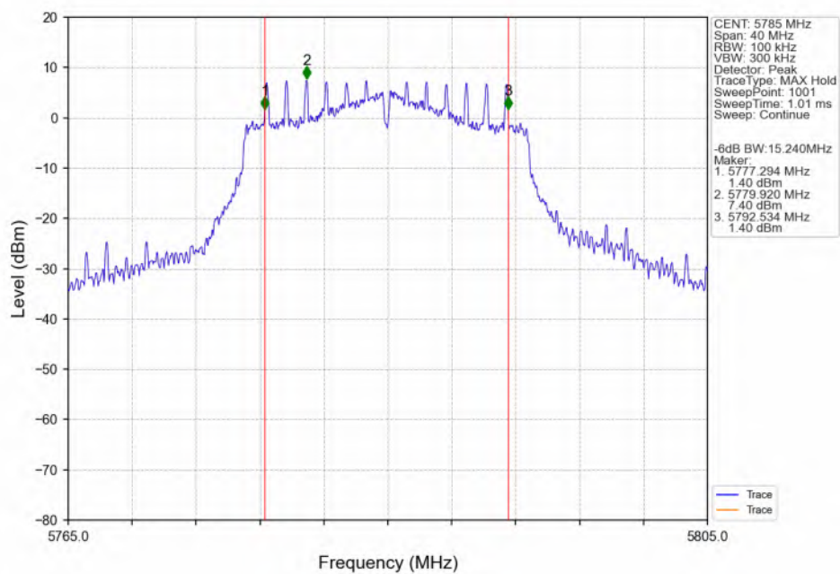
802.11n(HT20)_MCH_5785MHz_ANT3_NTNV
