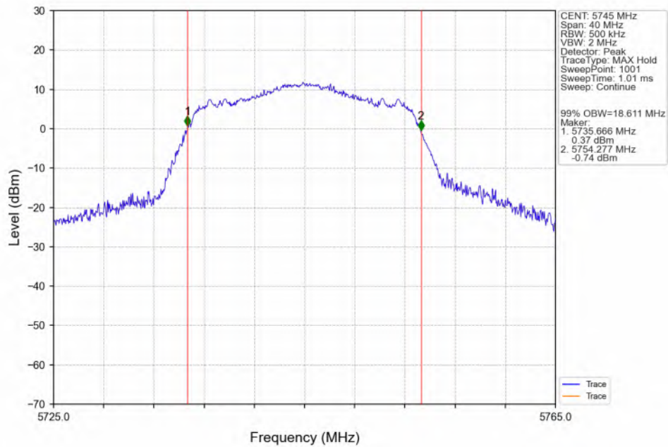
802.11ax(HEW20)_LCH_5745MHz_SU / _ANT3_NTNV
