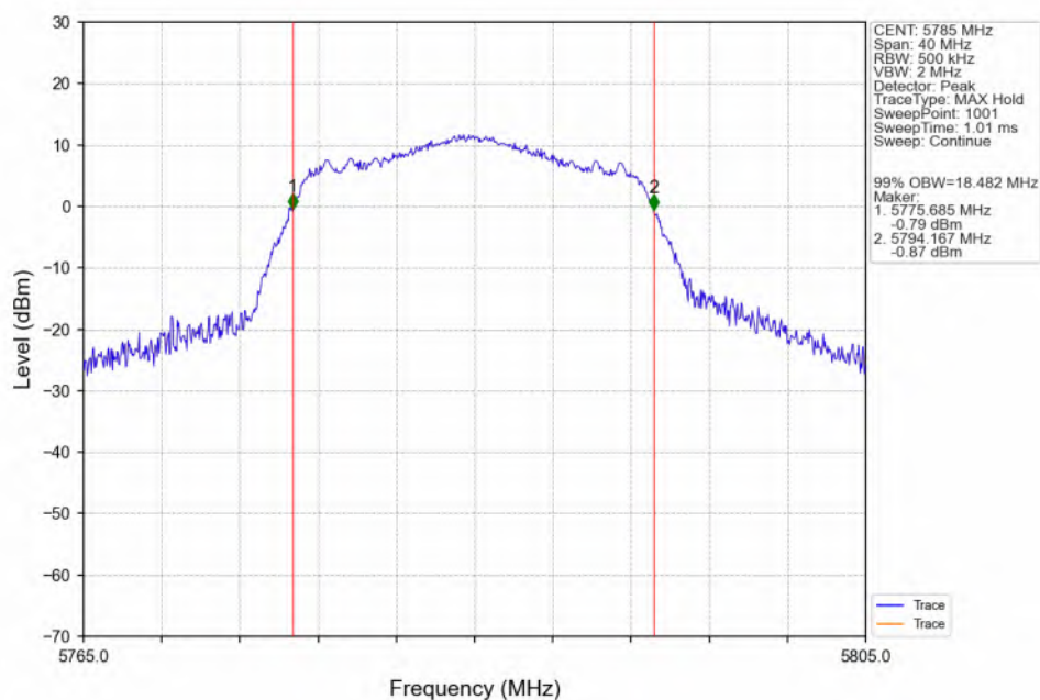
802.11ax(HEW20)_MCH_5785MHz_SU_/_ANT3_NTNV
