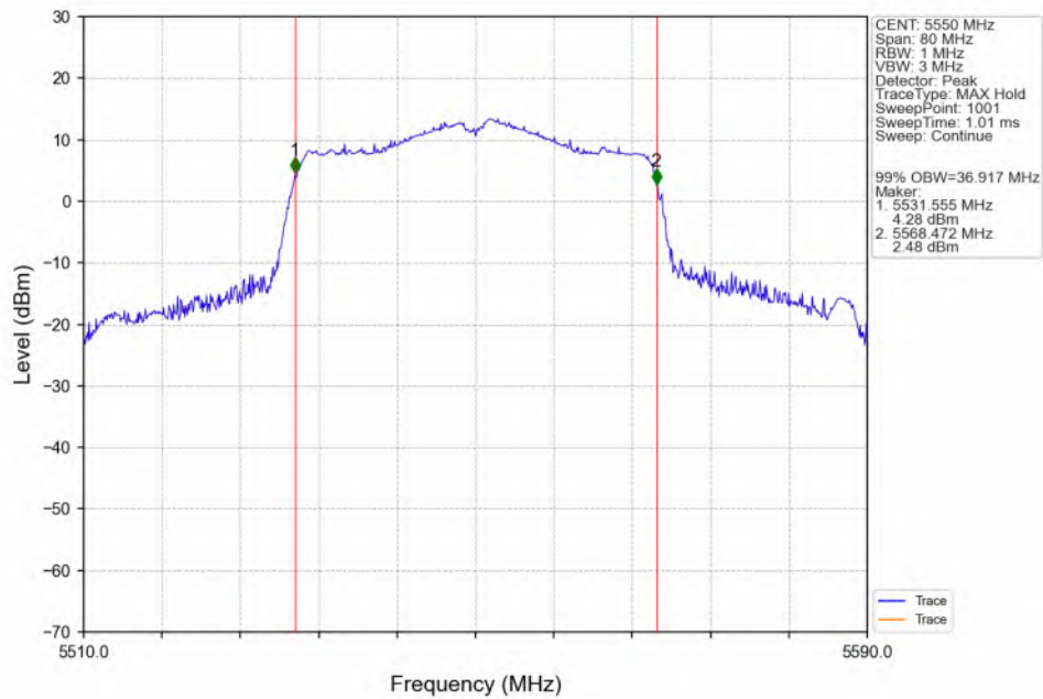
802.11n(HT40)_MCH_5550MHz_ANT3_NTNV
