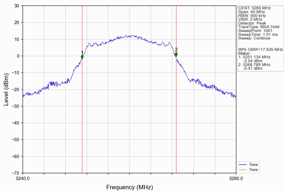
802.11a_LCH_5260MHz_ANT3_NTNV
