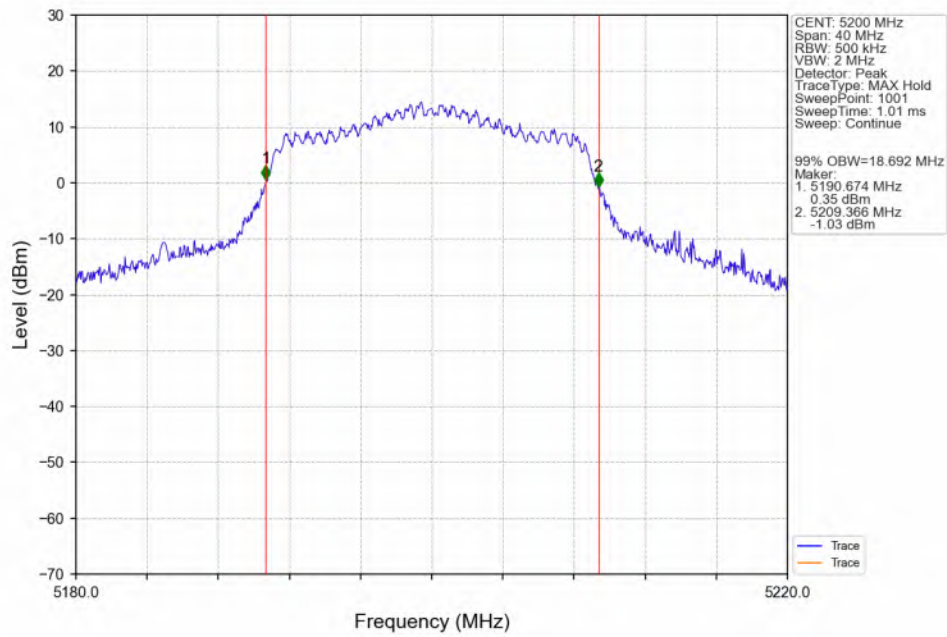
802.11n(HT20)_MCH_5200MHz_ANT3_NTNV
