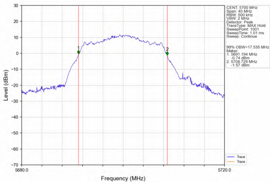
802.11a_HCH_5700MHz_ANT3_NTNV
