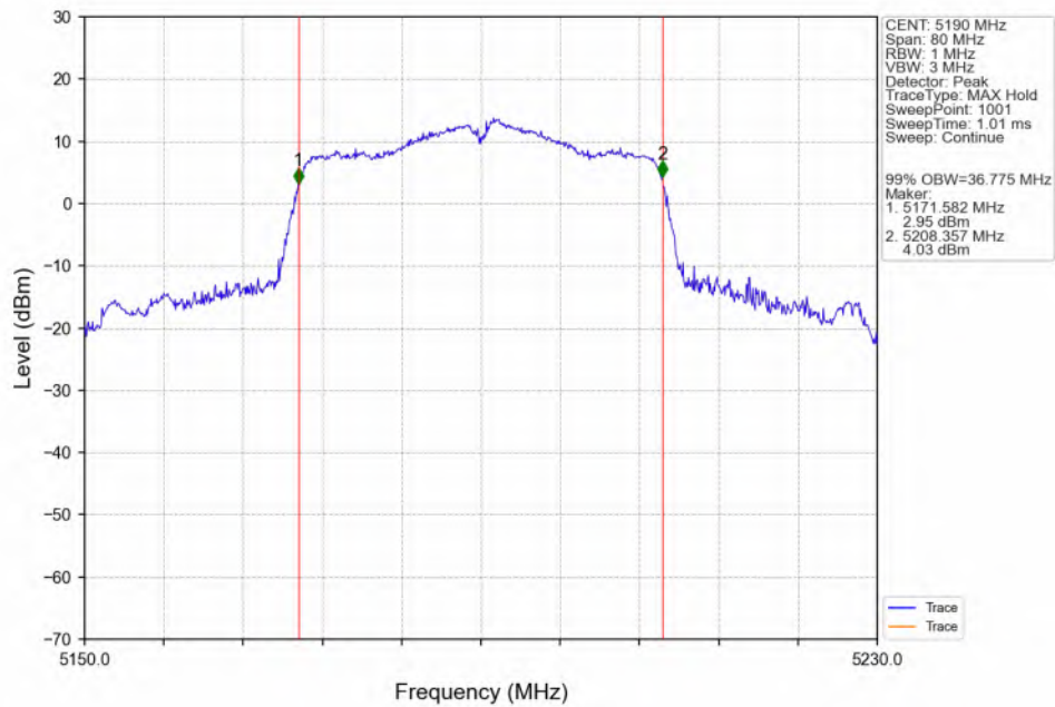
802.11n(HT40)_LCH_5190MHz_ANT3_NTNV
