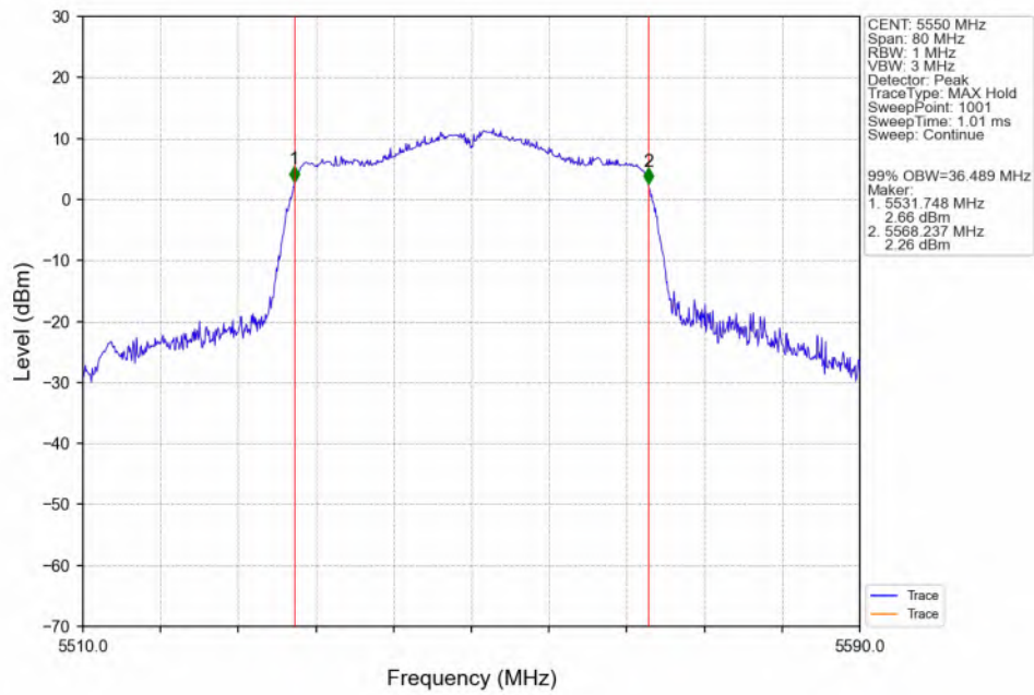
802.11ax(HEW40)_MCH_5550MHz_SU_/_ANT3_NTNV
