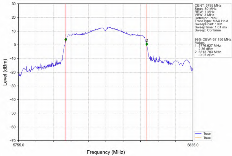
802.11n(HT40)_HCH_5795MHz_ANT3_NTNV
