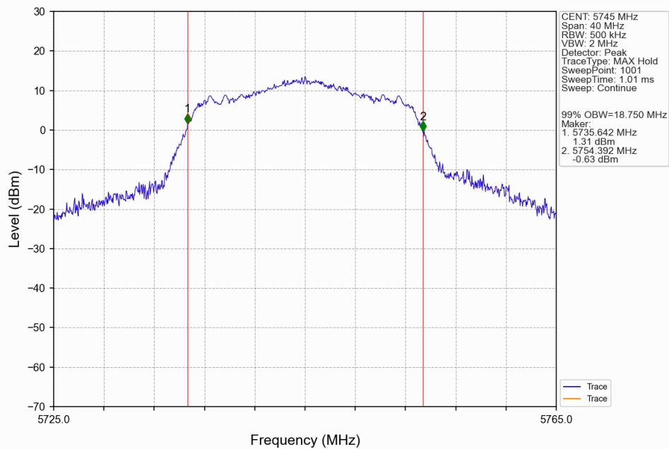
802.11n(HT20)_LCH_5745MHz_ANT3_NTNV
