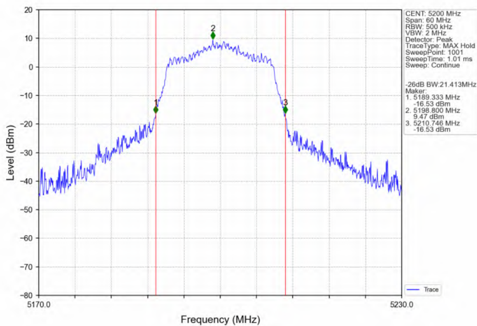
802.11n(HT20)_MCH_5200MHz_ANT3_NTNV
