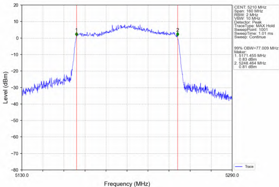
802.11ax(HEW80)_MCH_5210MHz_SU_/_ANT3_NTNV
