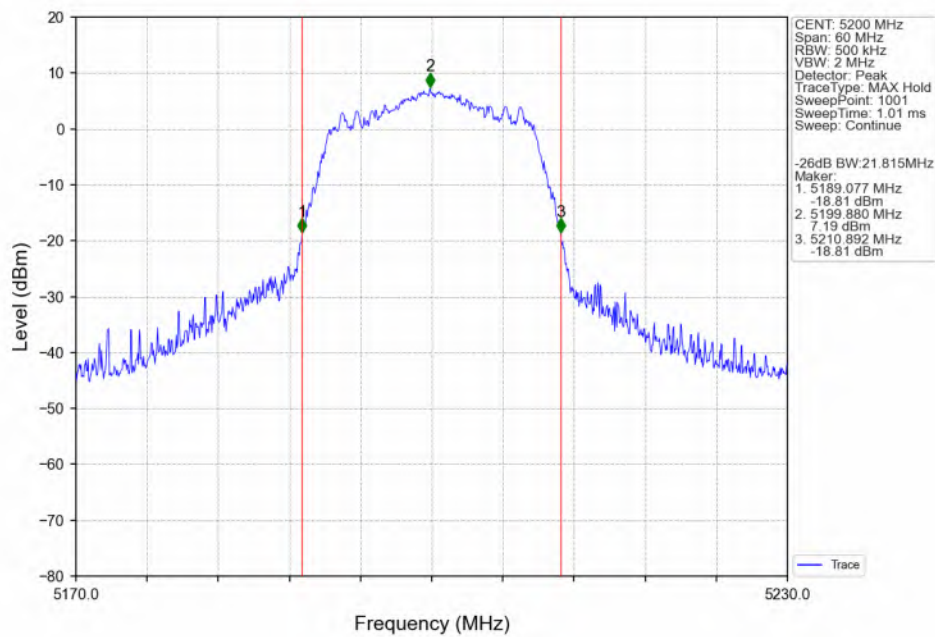
802.11n(HT20)_MCH_5200MHz_ANT3_NTNV
