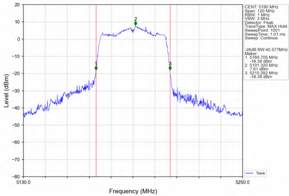
802.11n(HT40)_LCH_5190MHz_ANT3_NTNV
