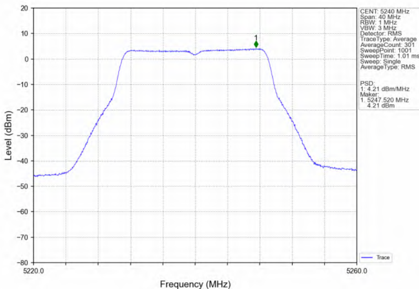
802.11n(HT20)_HCH_5240MHz_ANT3_NTNV
