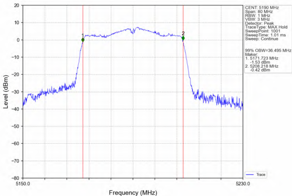
802.11n(HT40)_LCH_5190MHz_ANT3_NTNV
