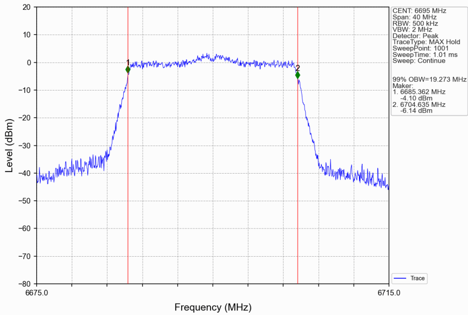
802.11ax(HEW20)_MCH_6695MHz_SU_/_ANT3_NTNV
