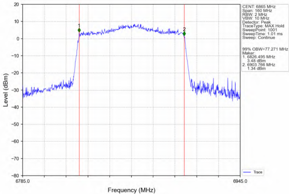
802.11ax(HEW80)_HCH_6865MHz_SU_/_ANT3_NTNV
