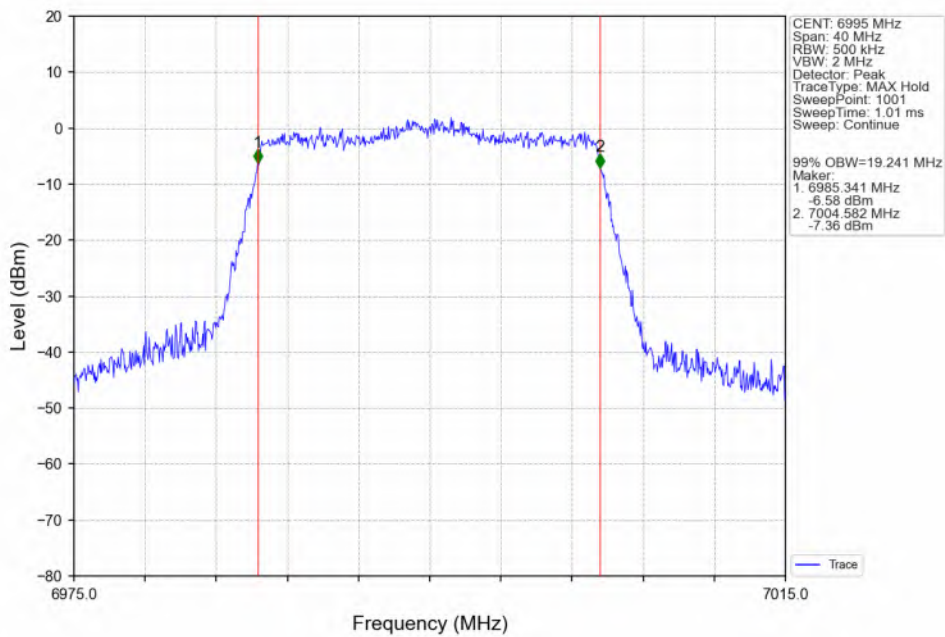
802.11ax(HEW20)_MCH_6995MHz_SU_/_ANT3_NTNV
