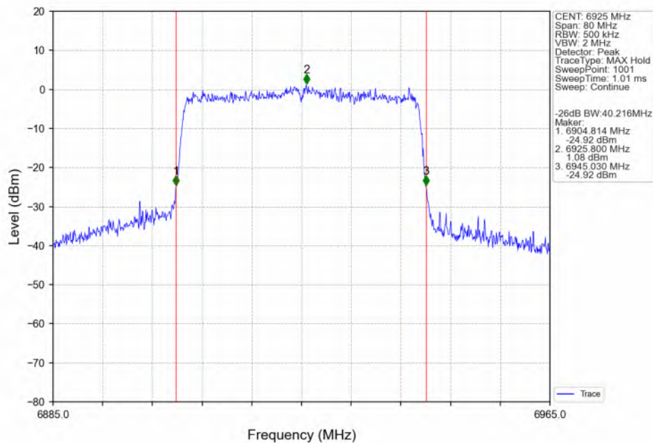
802.11ax(HEW40)_LCH_6925MHz_SU_/_ANT3_NTNV
