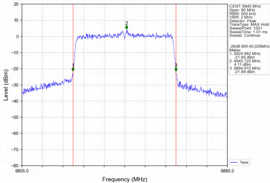
802.11ax(HEW40)_HCH_6845MHz_SU_/_ANT3_NTNV
