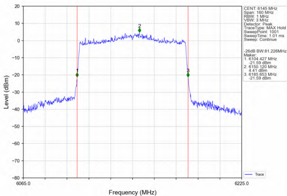
802.11ax(HEW80)_MCH_6145MHz_SU_/_ANT3_NTNV
