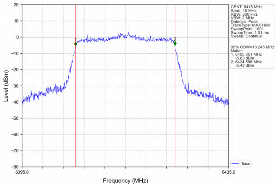
802.11ax(HEW20)_HCH_6415MHz_SU_/_ANT3_NTNV
