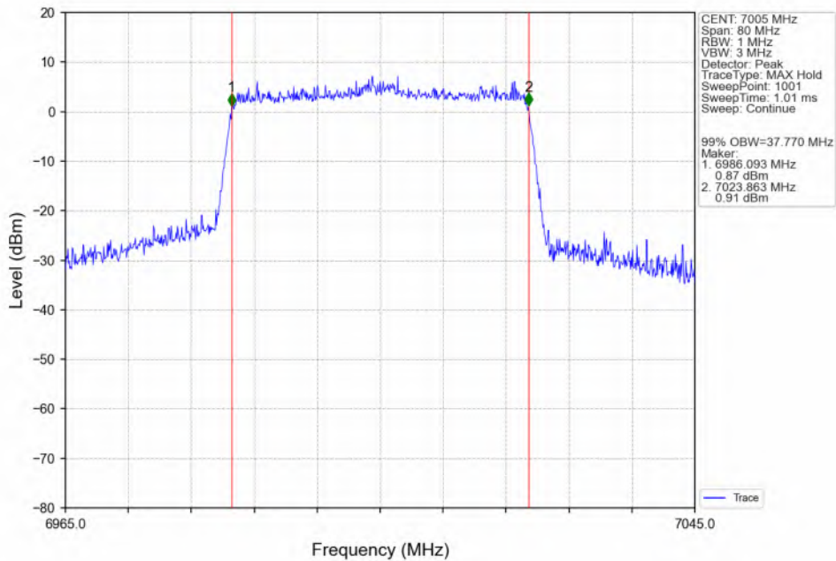
802.11ax(HEW40)_MCH_7005MHz_SU_/_ANT3_NTNV
