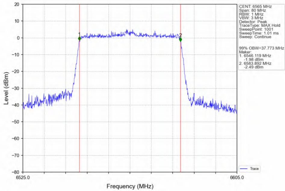
802.11ax(HEW40)_LCH_6565MHz_SU_/_ANT3_NTNV
