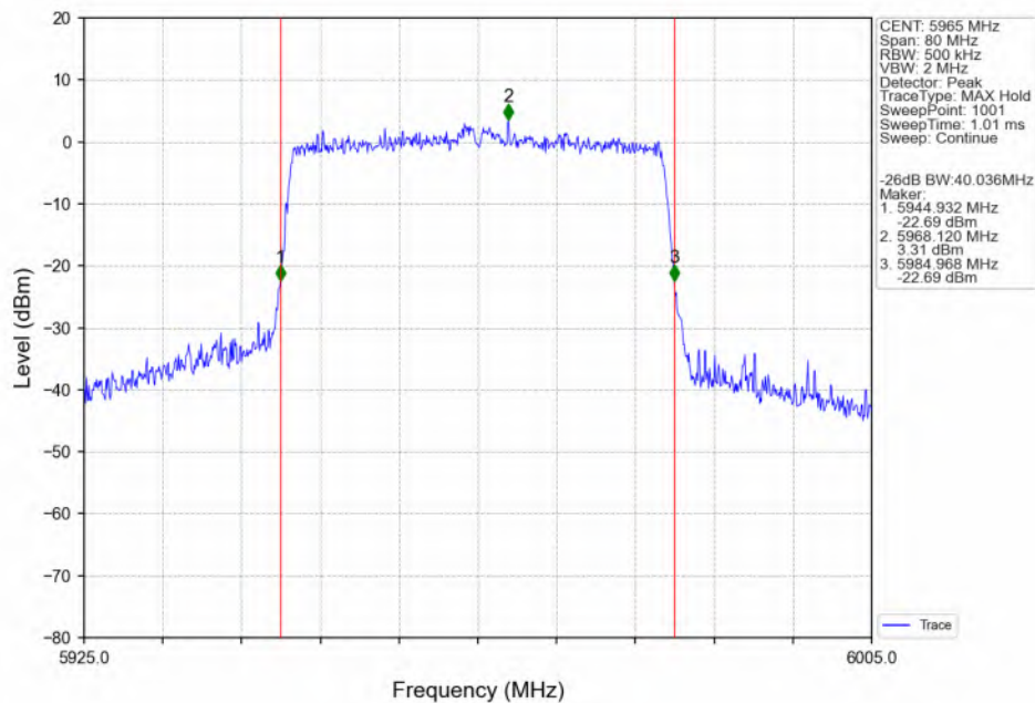
802.11ax(HEW40)_LCH_5965MHz_SU_/_ANT3_NTNV
