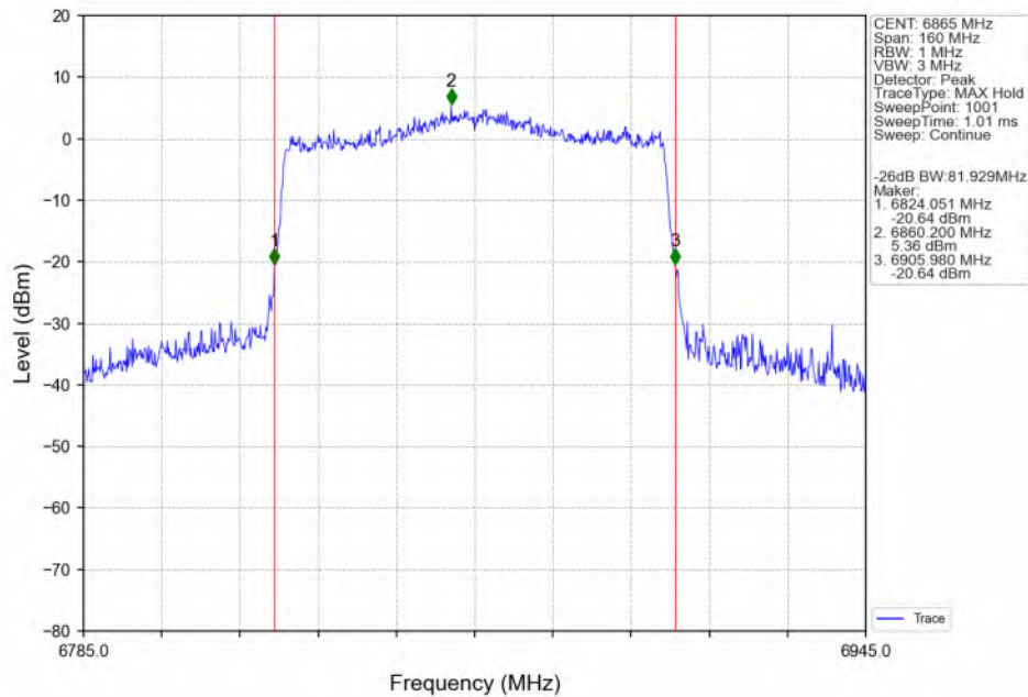
802.11ax(HEW80)_HCH_6865MHz_SU_/_ANT3_NTNV
