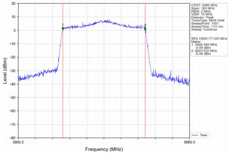
802.11ax(HEW80)_LCH_5985MHz_SU_/_ANT3_NTNV
