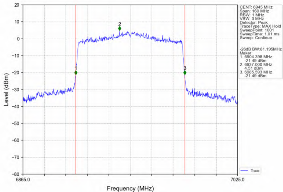
802.11ax(HEW80)_LCH_6945MHz_SU_/_ANT3_NTNV
