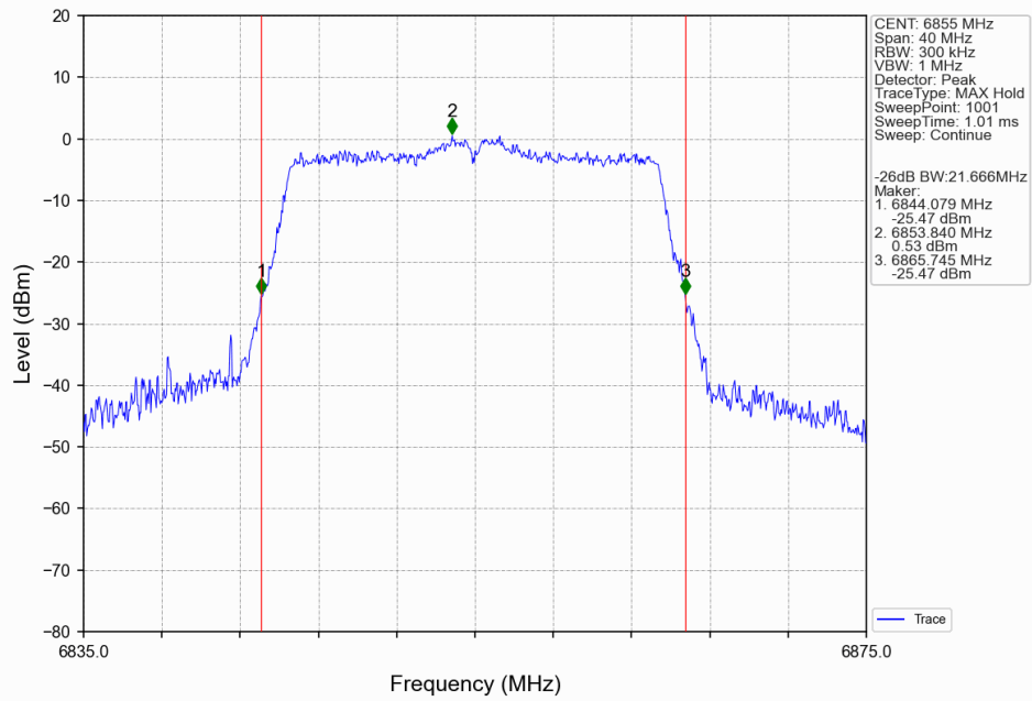
802.11ax(HEW20)_HCH_6855MHz_SU_/_ANT3_NTNV
