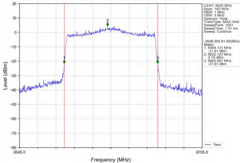
802.11ax(HEW80)_LCH_6625MHz_SU_/_ANT3_NTNV
