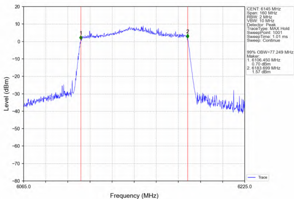
802.11ax(HEW80)_MCH_6145MHz_SU_/_ANT3_NTNV
