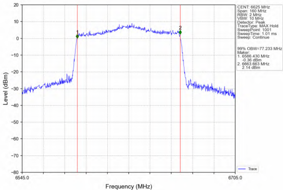
802.11ax(HEW80)_LCH_6625MHz_SU_/_ANT3_NTNV
