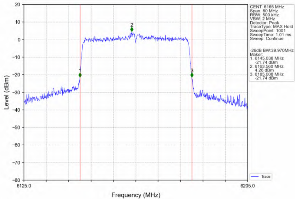
802.11ax(HEW40)_MCH_6165MHz_SU_/_ANT3_NTNV
