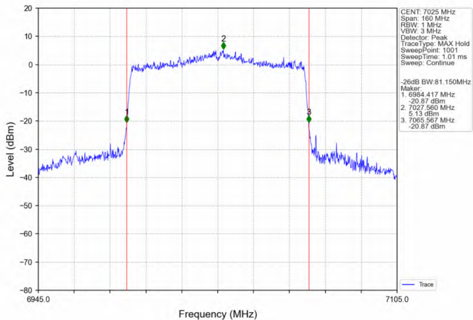
802.11ax(HEW80)_HCH_7025MHz_SU_/_ANT3_NTNV
