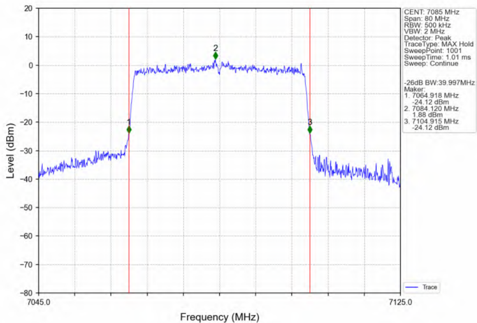
802.11ax(HEW40)_HCH_7085MHz_SU_/_ANT3_NTNV
