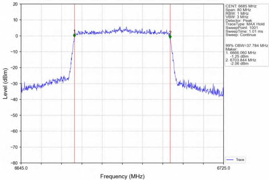
802.11ax(HEW40)_MCH_6685MHz_SU_/_ANT3_NTNV
