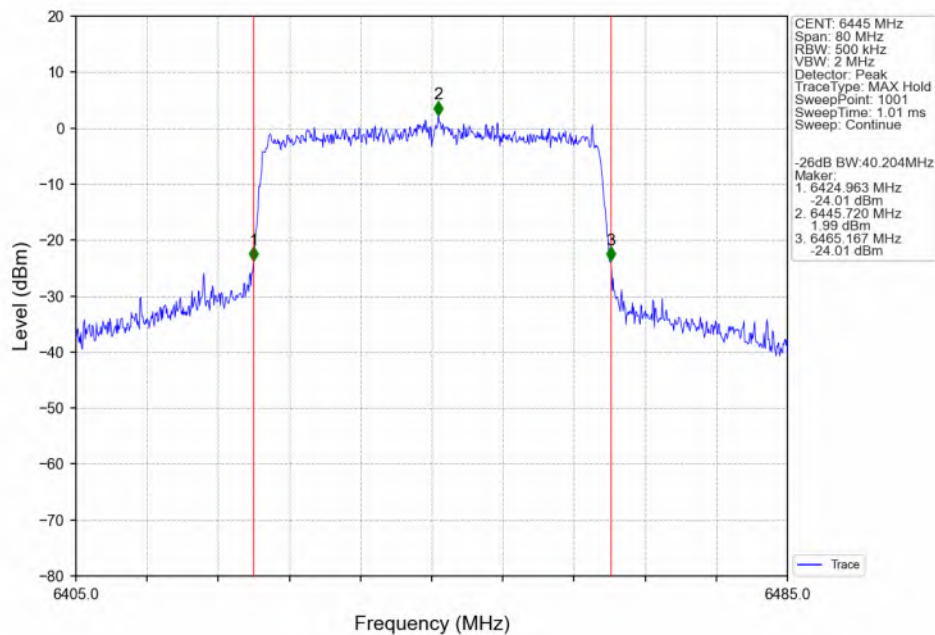
802.11ax(HEW40)_LCH_6445MHz_SU_/_ANT3_NTNV
