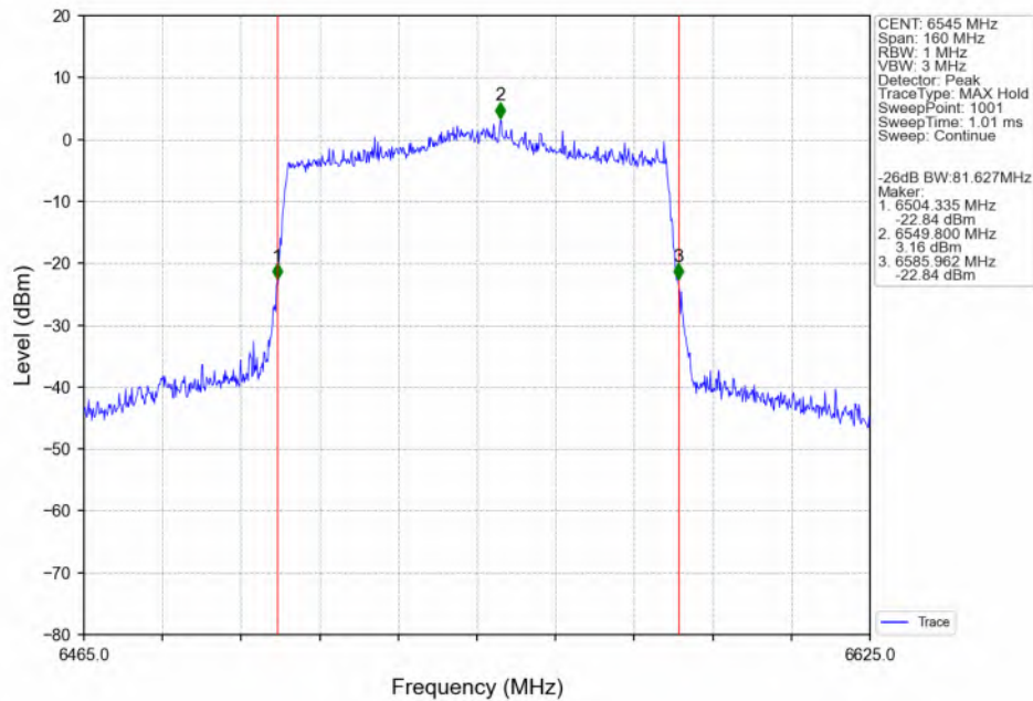
802.11ax(HEW80)_HCH_6545MHz_SU_/_ANT3_NTNV
