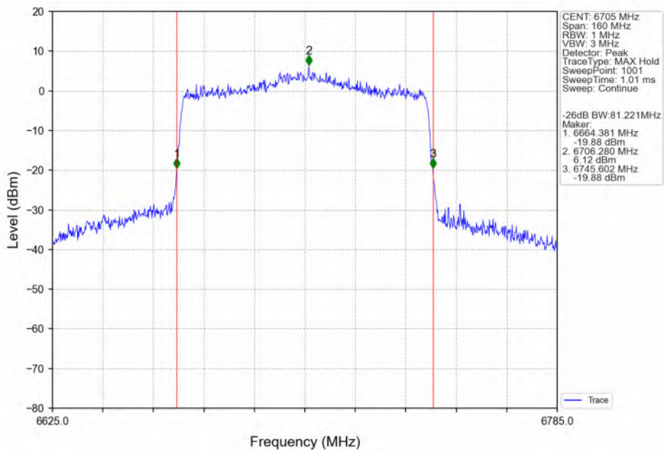
802.11ax(HEW80)_MCH_6705MHz_SU_/_ANT3_NTNV
