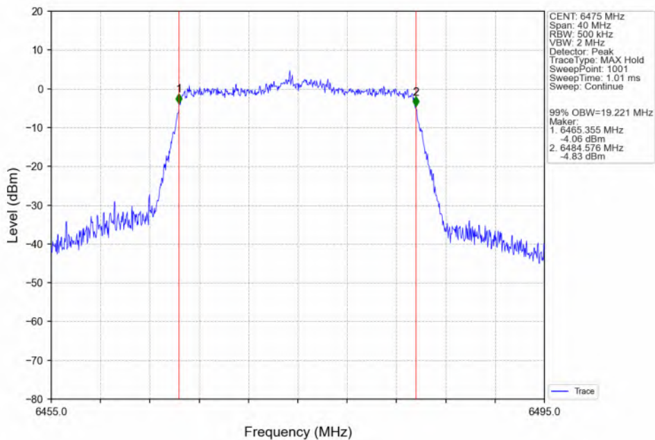
802.11ax(HEW20)_MCH_6475MHz_SU_/_ANT3_NTNV
