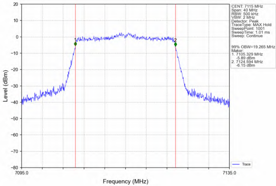
802.11ax(HEW20)_HCH_7115MHz_SU_/_ANT3_NTNV
