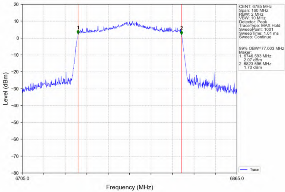
802.11ax(HEW80)_HCH_6785MHz_SU_/_ANT3_NTNV
