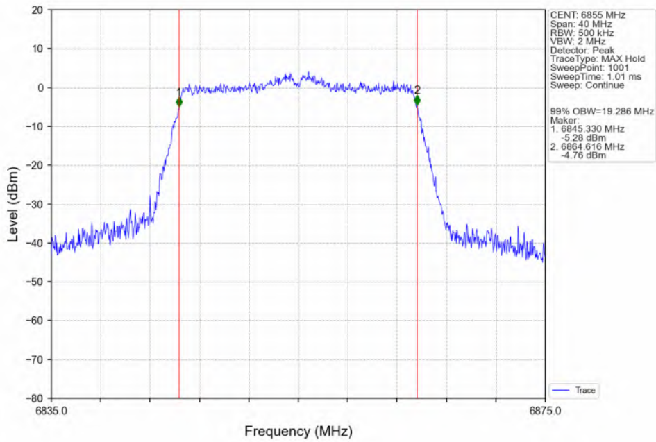
802.11ax(HEW20)_HCH_6855MHz_SU_/_ANT3_NTNV
