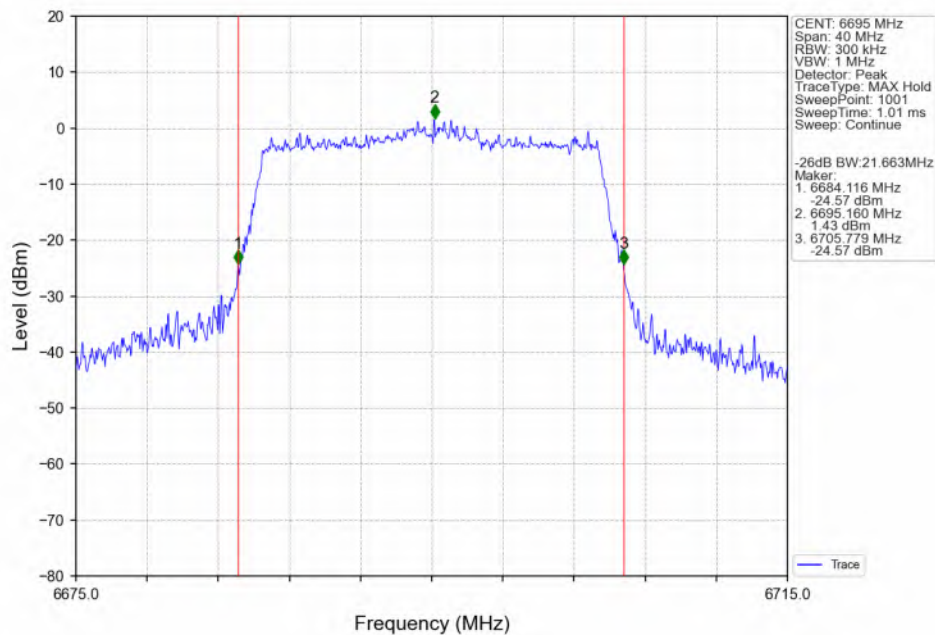
802.11ax(HEW20)_MCH_6695MHz_SU_/_ANT3_NTNV
