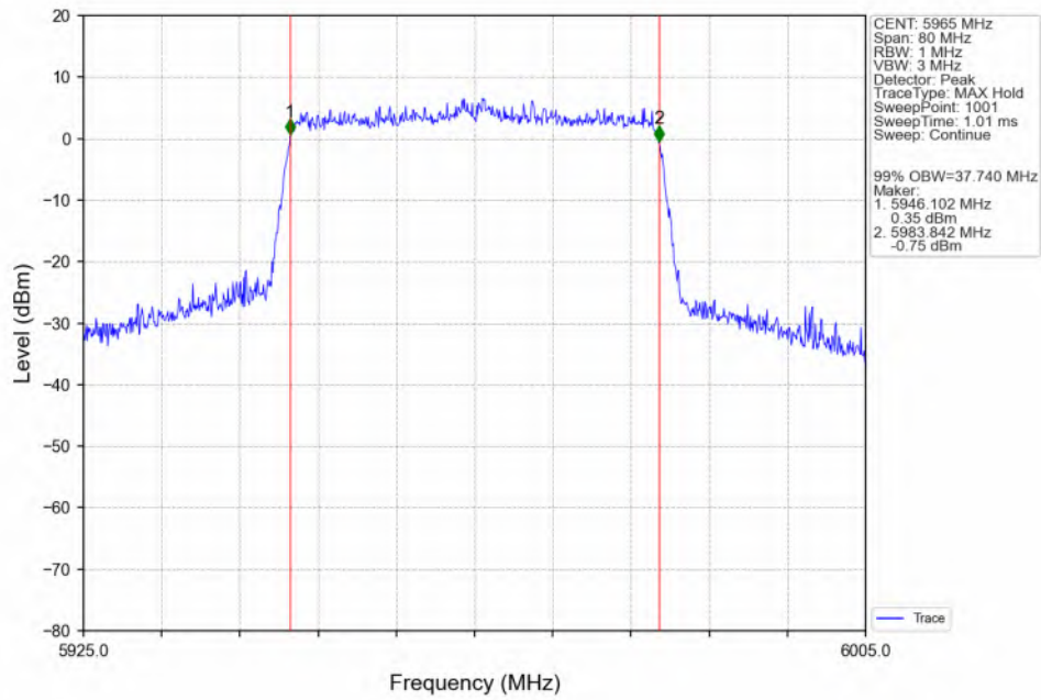
802.11ax(HEW40)_LCH_5965MHz_SU_/_ANT3_NTNV
