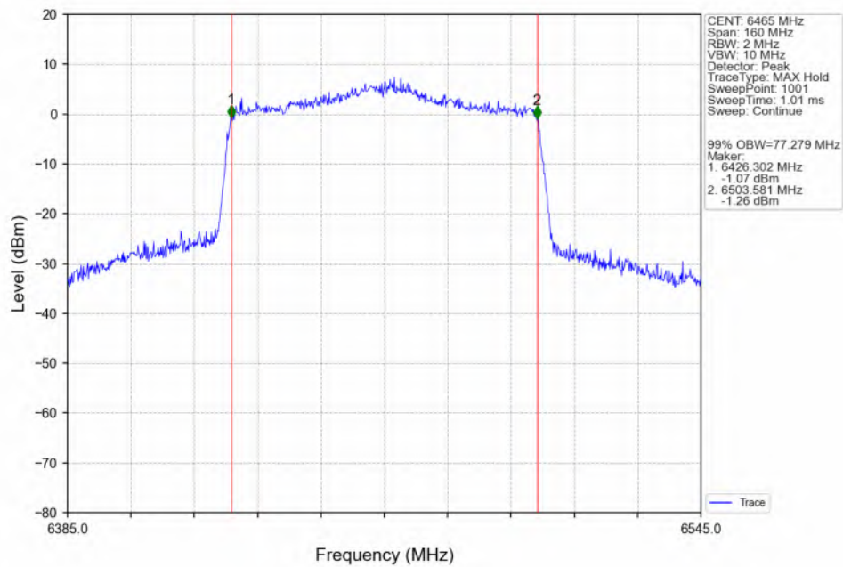
802.11ax(HEW80)_LCH_6465MHz_SU_/_ANT3_NTNV
