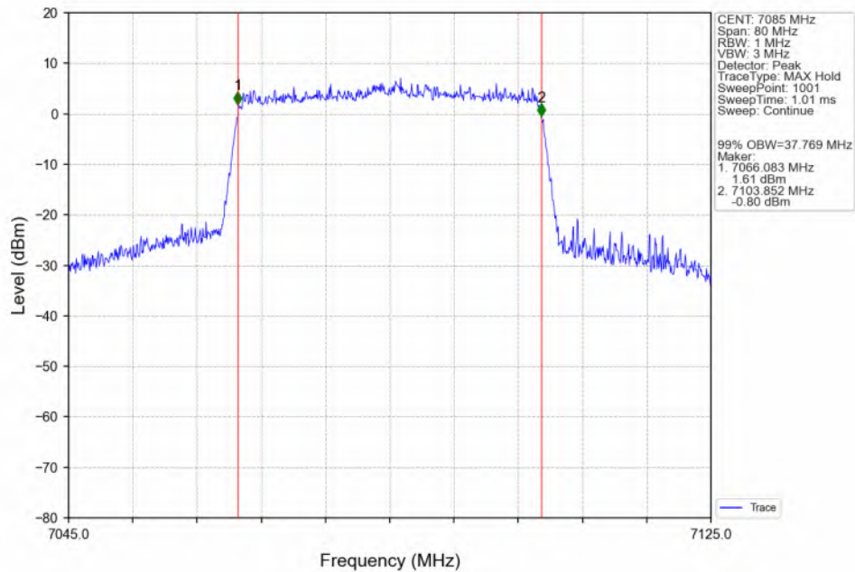
802.11ax(HEW40)_HCH_7085MHz_SU_/_ANT3_NTNV
