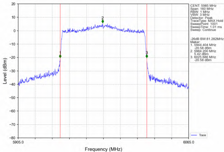
802.11ax(HEW80)_LCH_5985MHz_SU_/_ANT3_NTNV
