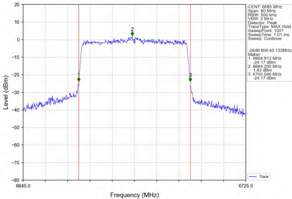
802.11ax(HEW40)_MCH_6685MHz_SU_/_ANT3_NTNV
