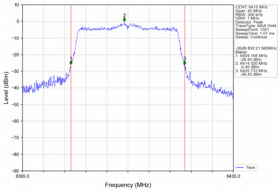
802.11ax(HEW20)_HCH_6415MHz_SU_/_ANT3_NTNV
