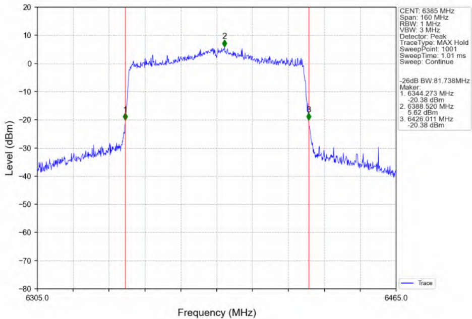
802.11ax(HEW80)_HCH_6385MHz_SU_/_ANT3_NTNV
