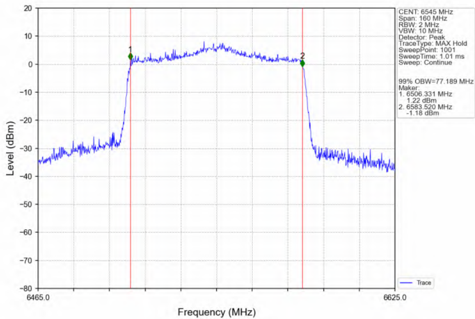
802.11ax(HEW80)_HCH_6545MHz_SU_/_ANT3_NTNV
