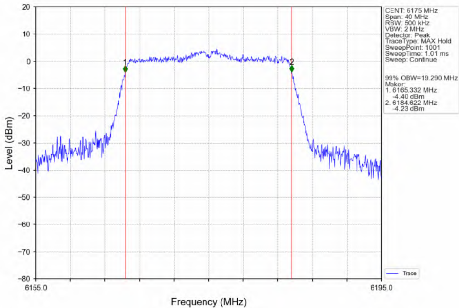
802.11ax(HEW20)_MCH_6175MHz_SU_/_ANT3_NTNV
