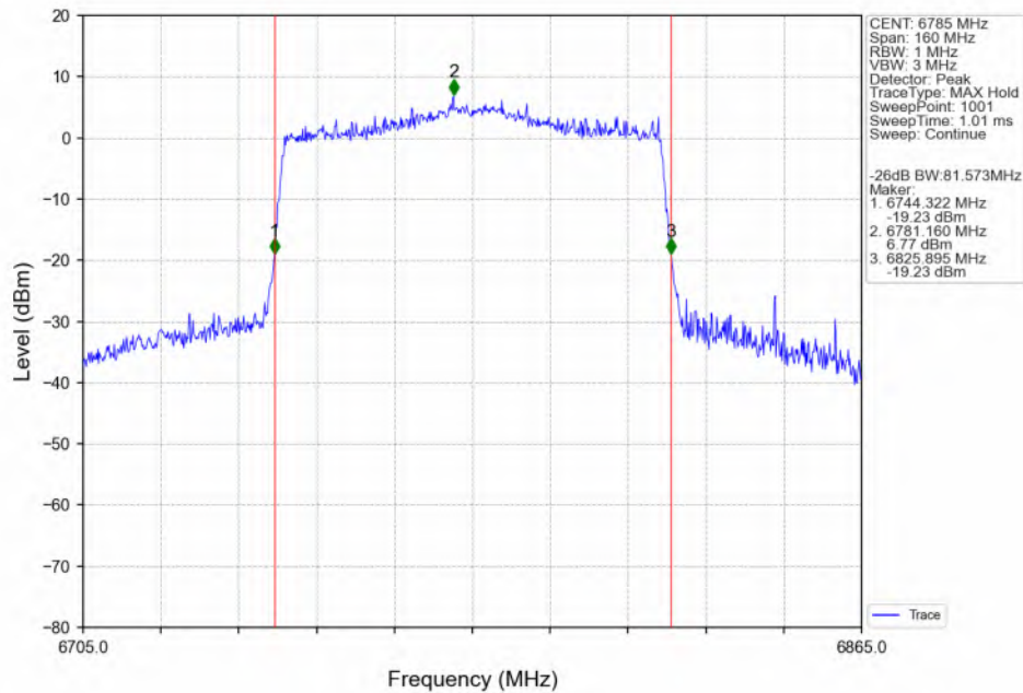
802.11ax(HEW80)_HCH_6785MHz_SU_/_ANT3_NTNV
