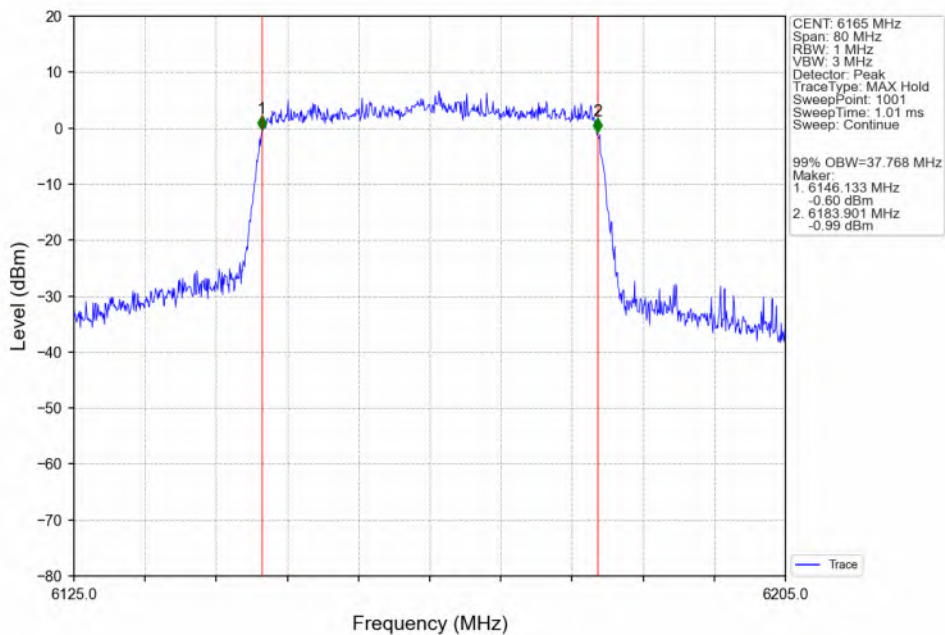
802.11ax(HEW40)_MCH_6165MHz_SU_/_ANT3_NTNV
