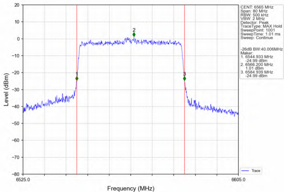
802.11ax(HEW40)_LCH_6565MHz_SU_/_ANT3_NTNV
