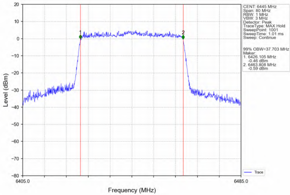
802.11ax(HEW40)_LCH_6445MHz_SU_/_ANT3_NTNV
