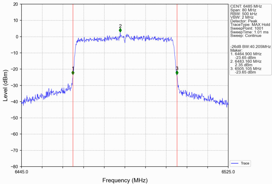
802.11ax(HEW40)_MCH_6485MHz_SU_/_ANT3_NTNV
