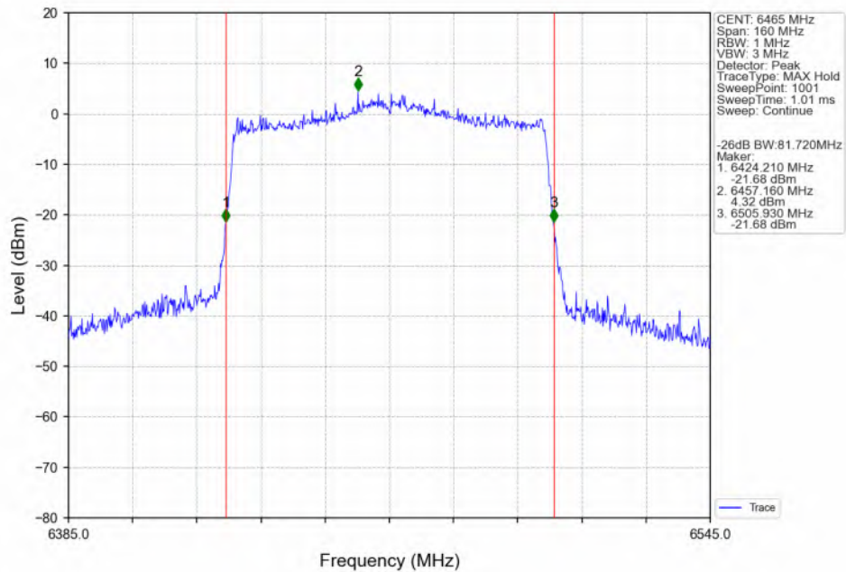
802.11ax(HEW80)_LCH_6465MHz_SU_/_ANT3_NTNV
