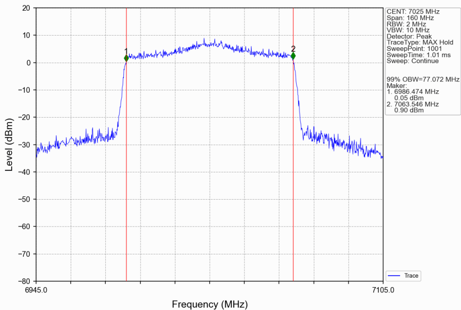
802.11ax(HEW80)_HCH_7025MHz_SU_/_ANT3_NTNV
