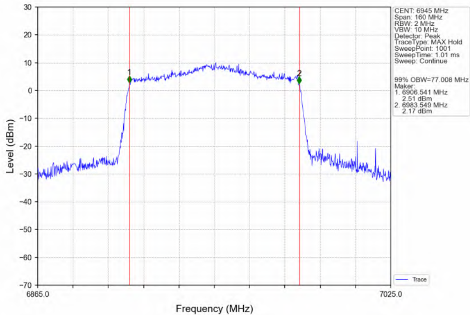
802.11ax(HEW80)_LCH_6945MHz_SU_/_ANT3_NTNV
