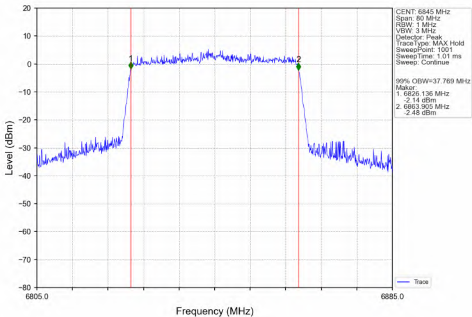
802.11ax(HEW40)_HCH_6845MHz_SU_/_ANT3_NTNV
