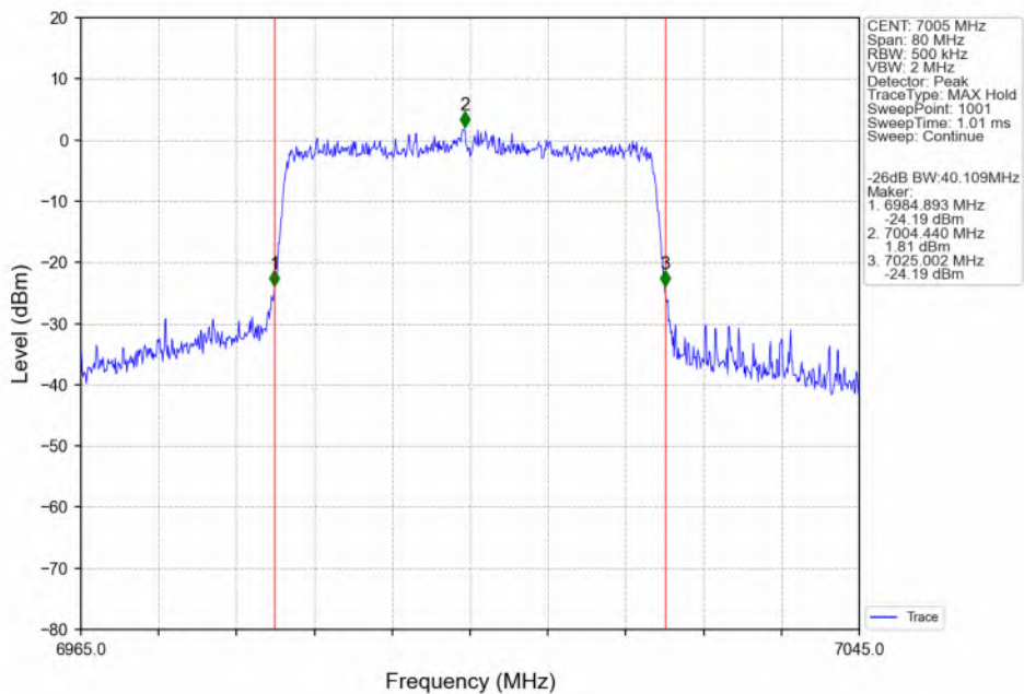
802.11ax(HEW40)_MCH_7005MHz_SU_/_ANT3_NTNV
