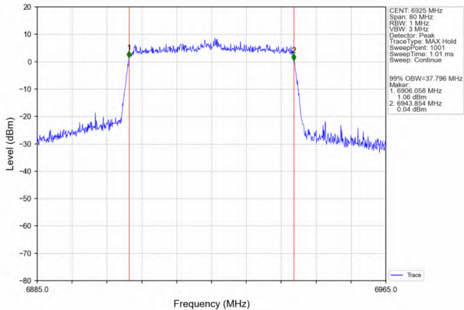
802.11ax(HEW40)_LCH_6925MHz_SU_/_ANT3_NTNV
