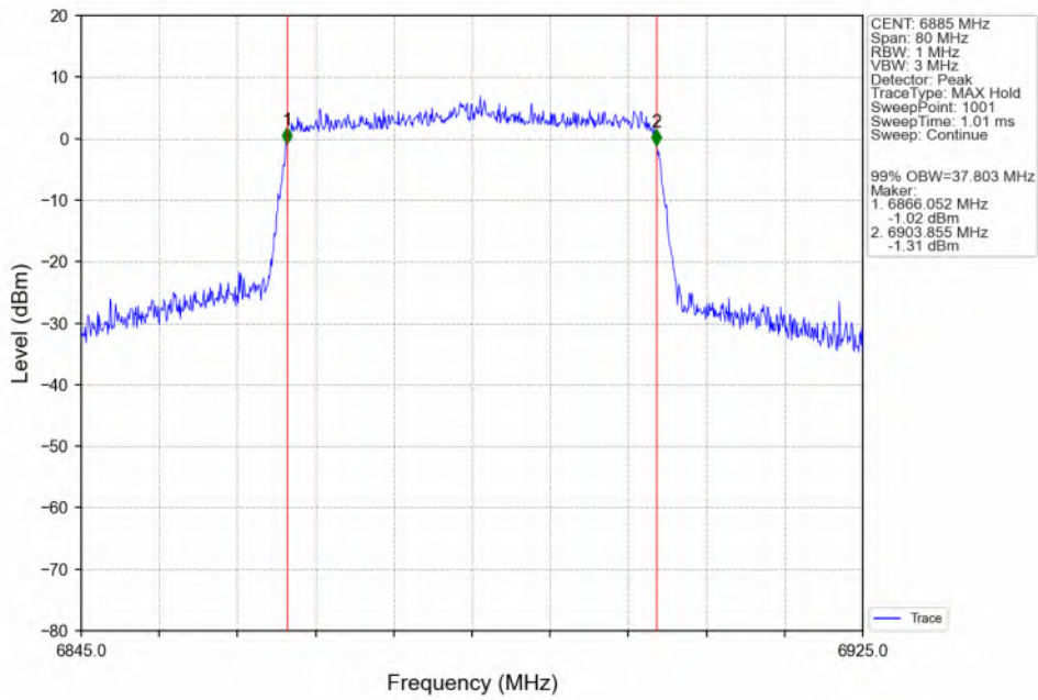
802.11ax(HEW40)_HCH_6885MHz_SU_/_ANT3_NTNV
