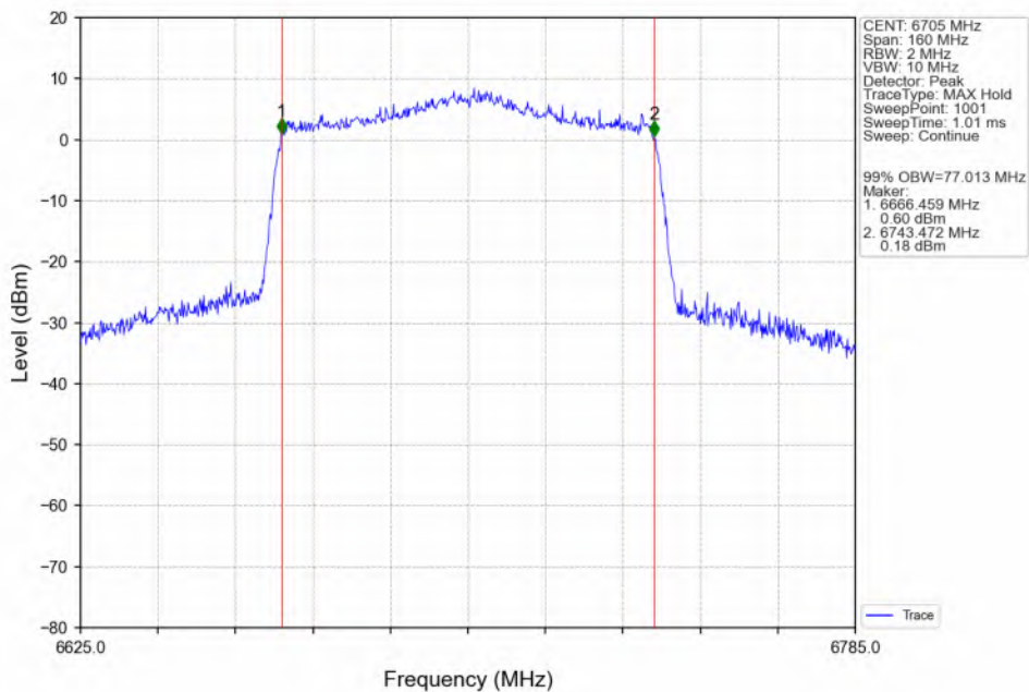
802.11ax(HEW80)_MCH_6705MHz_SU_/_ANT3_NTNV
