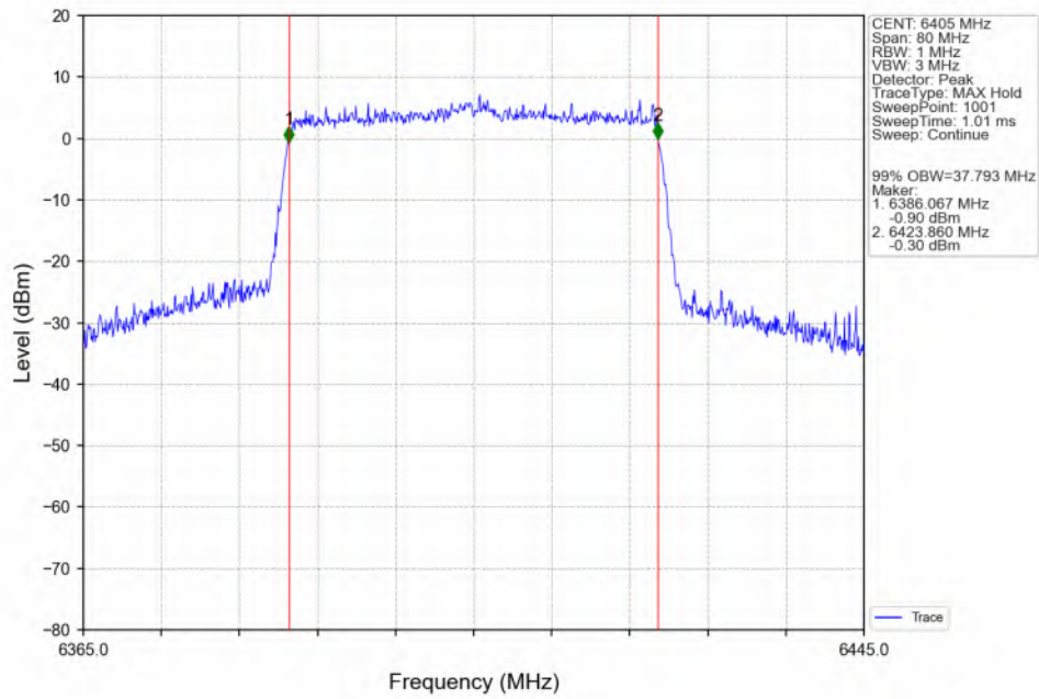
802.11ax(HEW40)_HCH_6405MHz_SU_/_ANT3_NTNV
