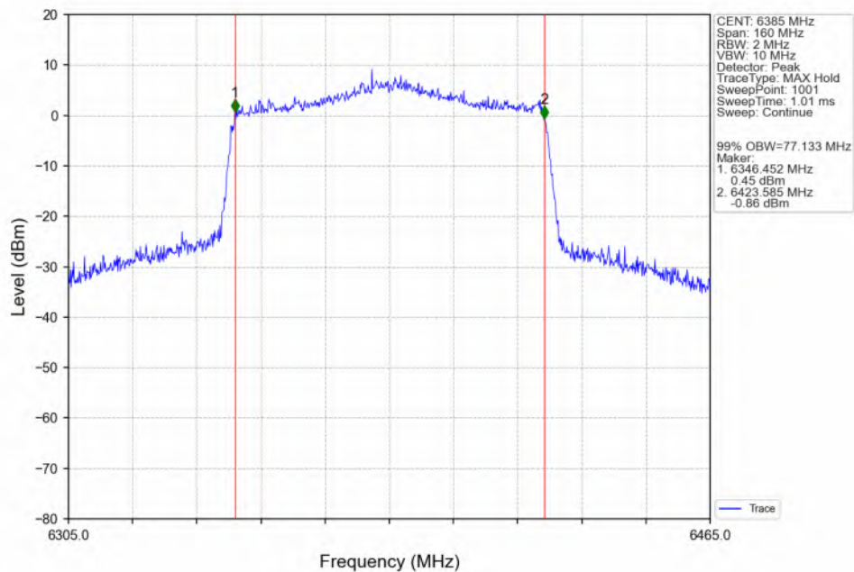
802.11ax(HEW80)_HCH_6385MHz_SU_/_ANT3_NTNV
