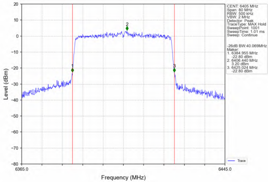
802.11ax(HEW40)_HCH_6405MHz_SU_/_ANT3_NTNV
