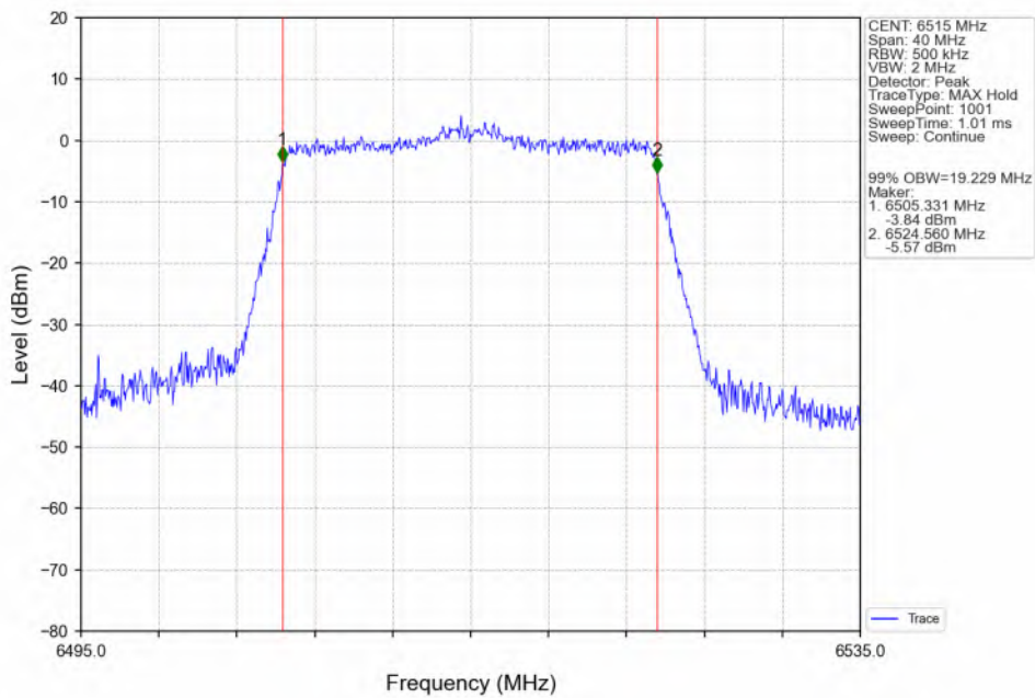
802.11ax(HEW20)_HCH_6515MHz_SU_/_ANT3_NTNV
