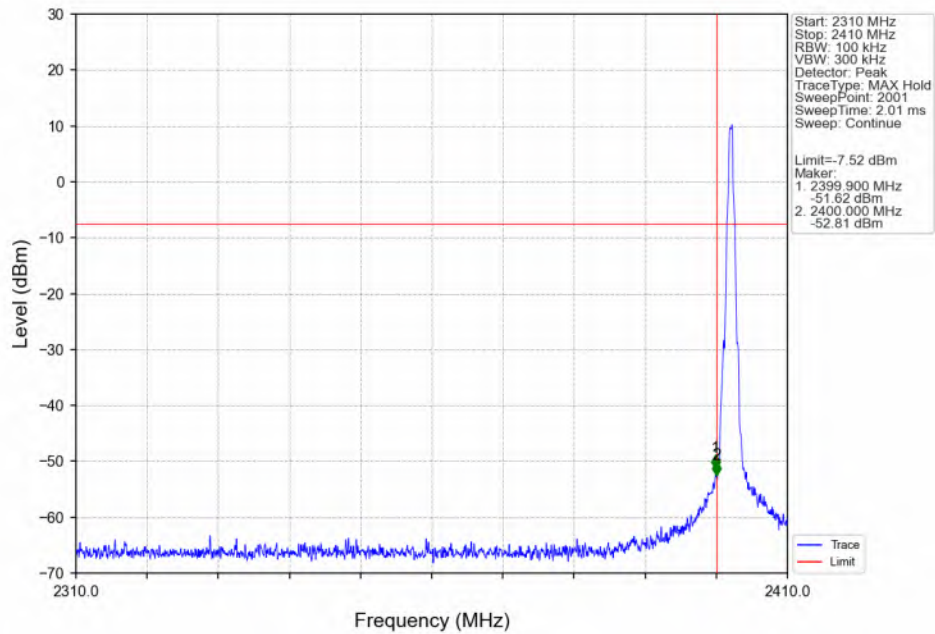
GFSK_DH5_LCH_2402MHz_Ant2_NTNV
