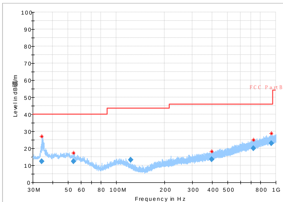
Fig 59. Radiated Spurious Emission (802.11b, Ch11, 30MHz~1GHz)
