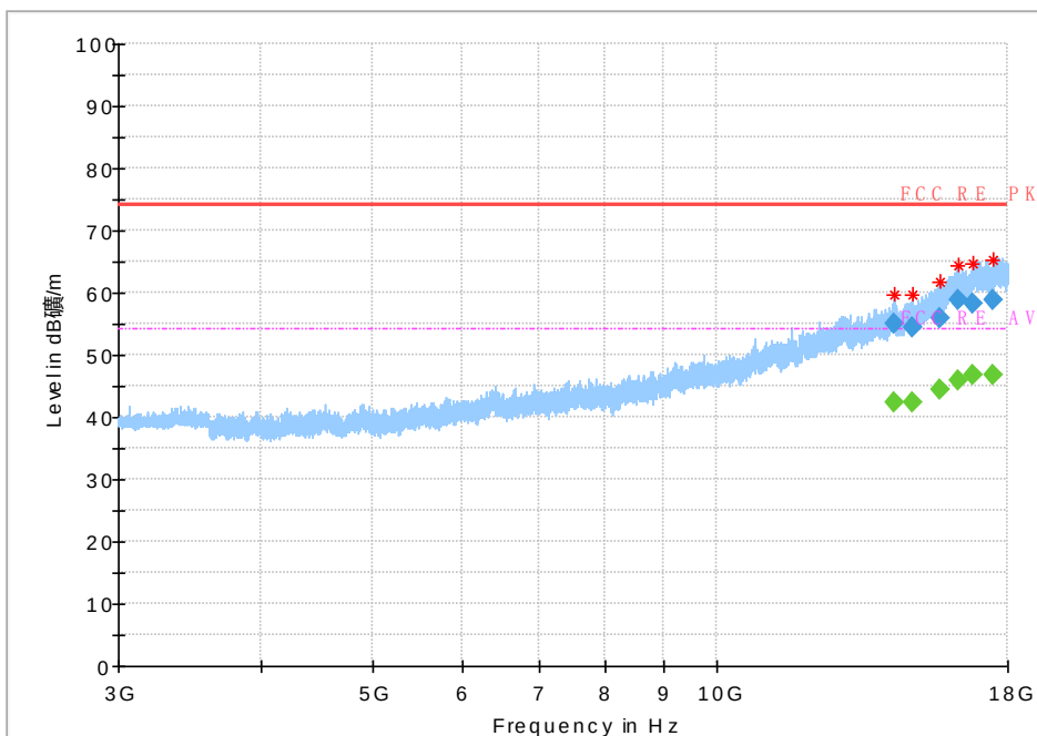
Fig 76. Radiated Spurious Emission (802.11 n-40MHz,Ch9, 3GHz~18GHz)
