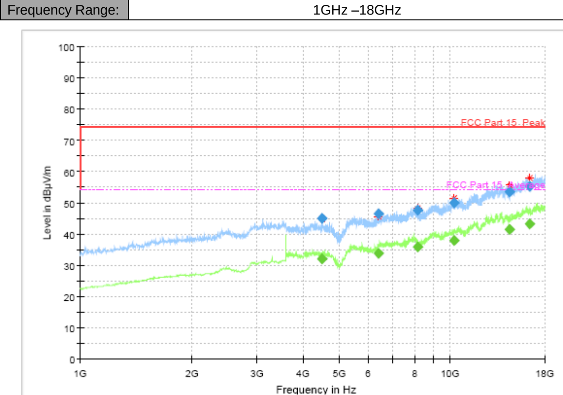
Mode 1: Charging mode (Full system) &lt;Figure 1&gt;
