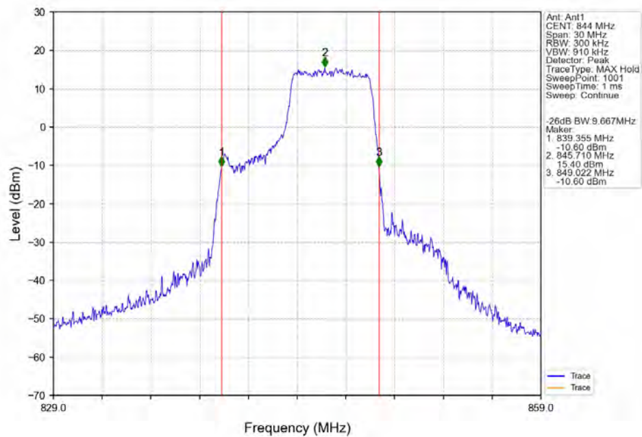
Band5_10MHz_16QAM_HCH_844MHz_RB_27_23_NTNV
