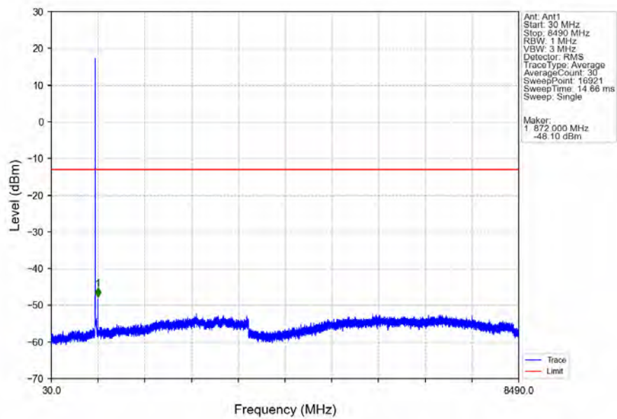
Band5_3MHz_QPSK_LCH_825.5MHz_RB_1_0_NTNV
