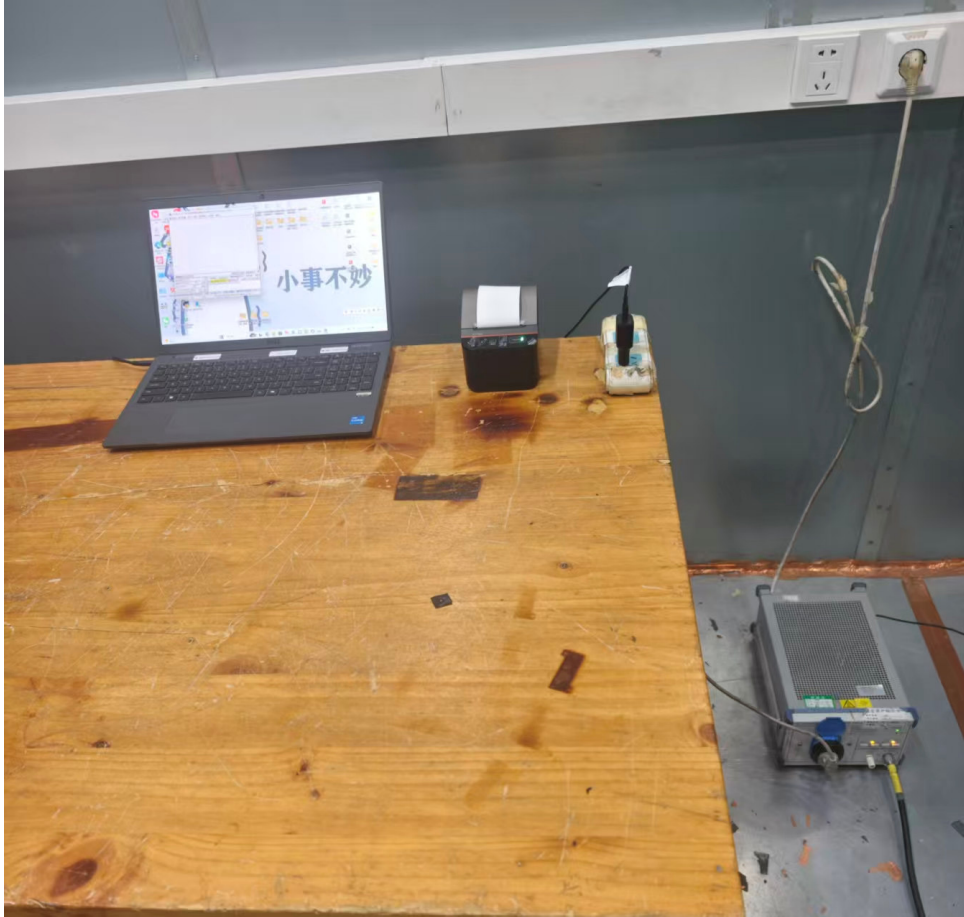
Picture 2: Conducted Emissions Test Setup
