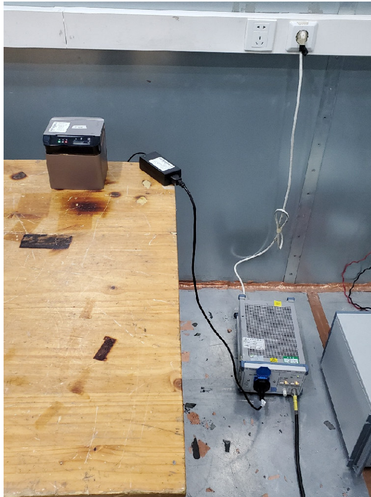
Picture 2 Conducted Emission Test Setup
