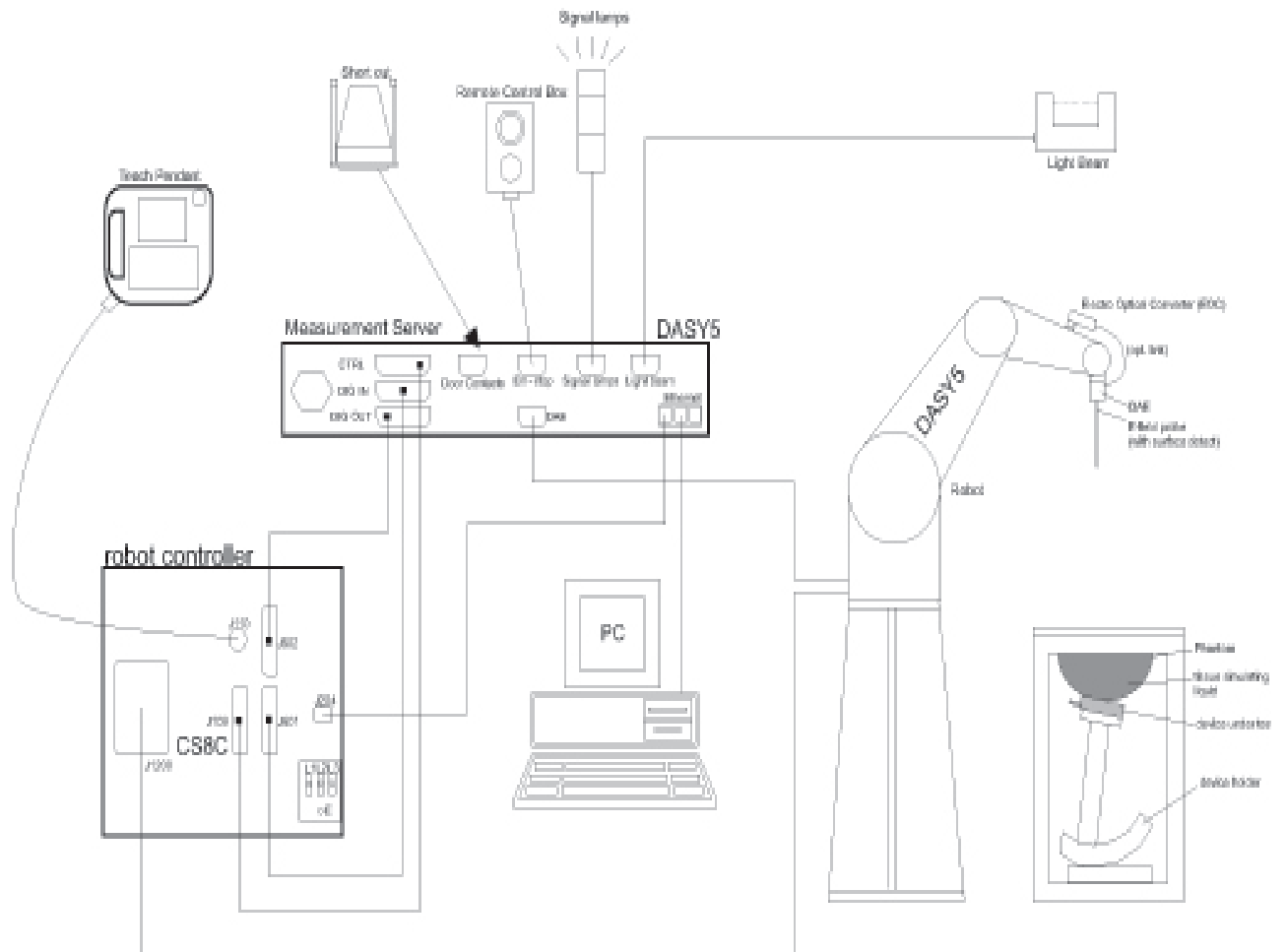
Figure 5-1 SAR Lab Test Measurement Set-up
