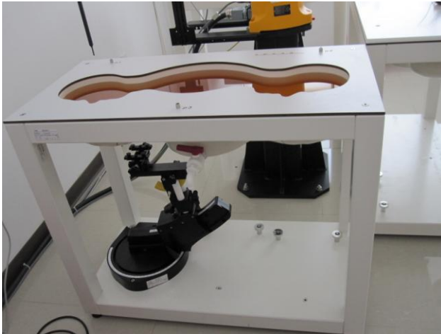
Figure 5-5. Generic Twin Phantom
