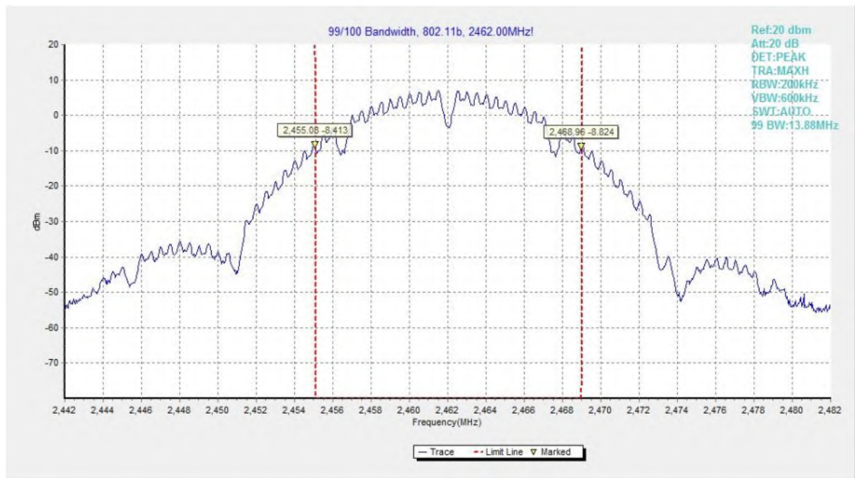
Fig.72 99% Occupied Bandwidth (802.11b, CH 11)
