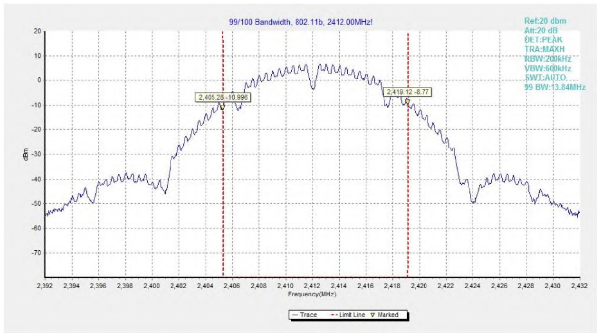
Fig.70 99% Occupied Bandwidth (802.11b, CH 1)
