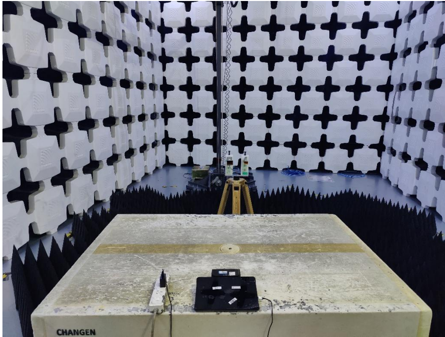
3. Radiated Emissions (Part 15B, Scanner and printer, 18GHz-26.5GHz)
