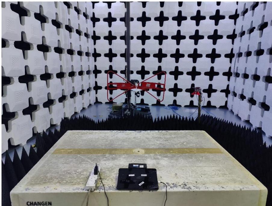
2. Radiated Emissions (Part 15B, Scanner and printer, 1GHz-18GHz)
