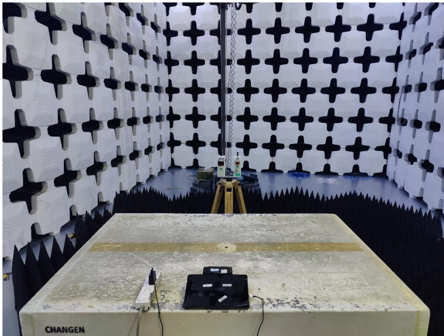
4. Radiated Emissions (Part 15B, Scanner and printer, 26.5GHz-40GHz)
