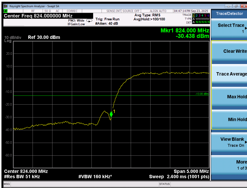
Band edge\WCDMA B5\L
