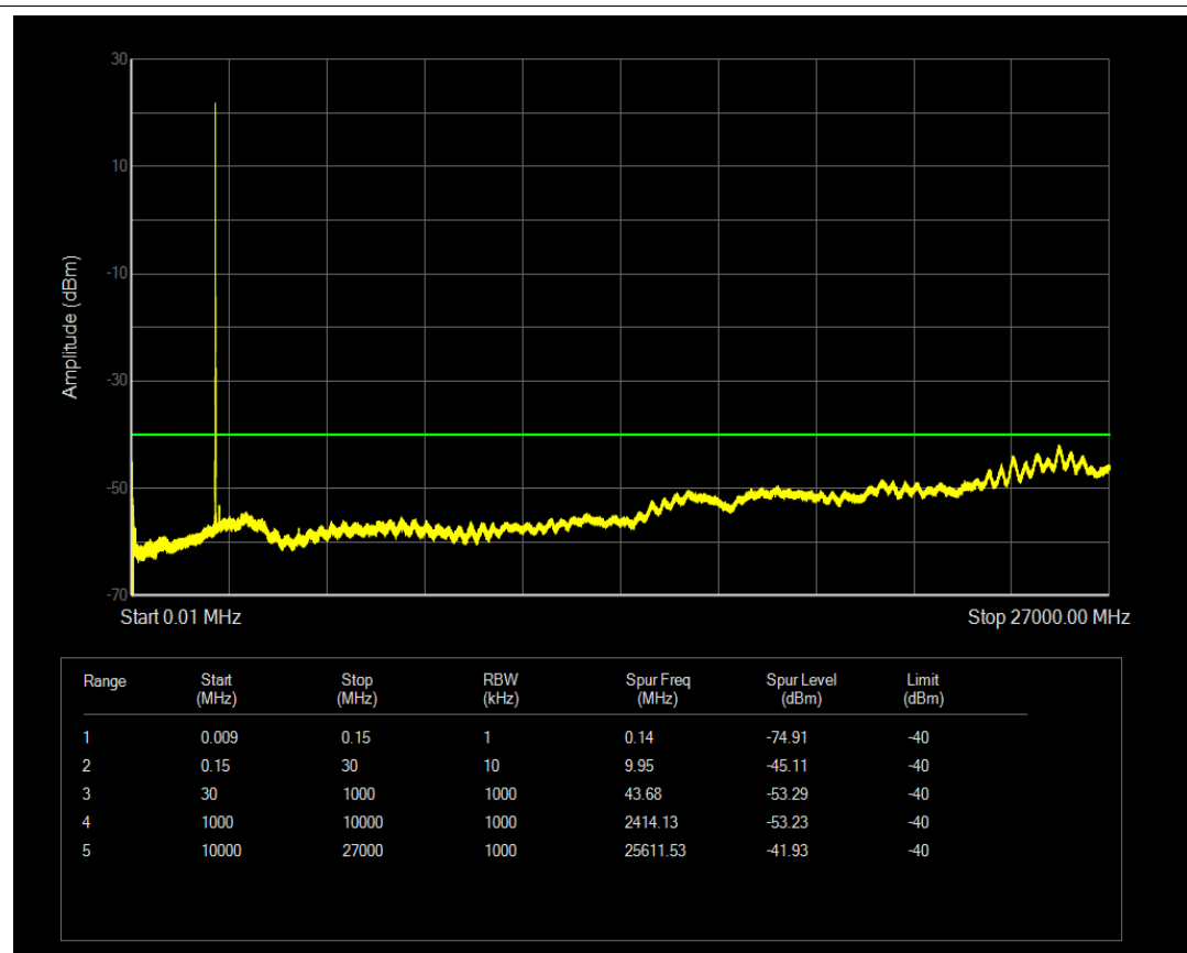
Band30 QPSK BW=5MHz Channel=27685 RB Size=1 Position=#0
