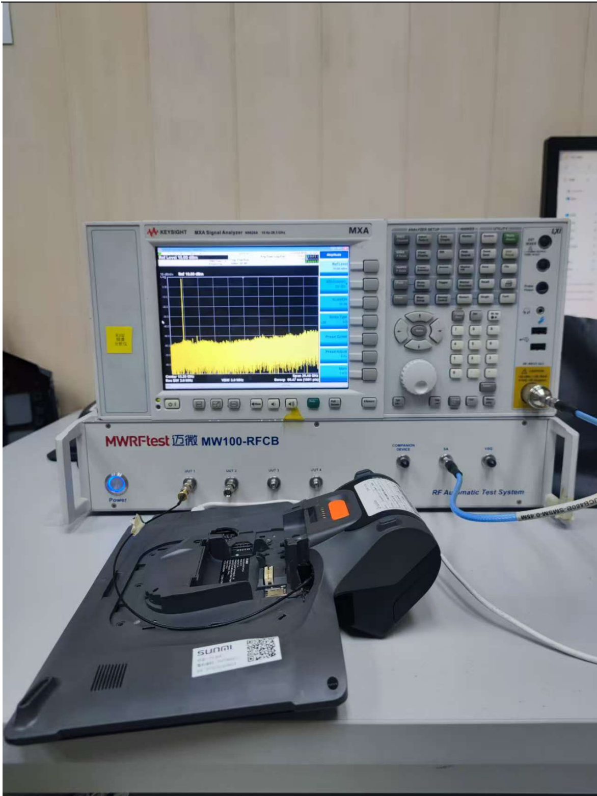
WLAN Test Setup
