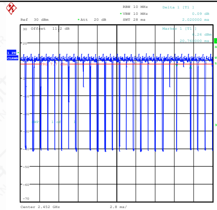
NTNV-11N40SISO-Ant1-2452
