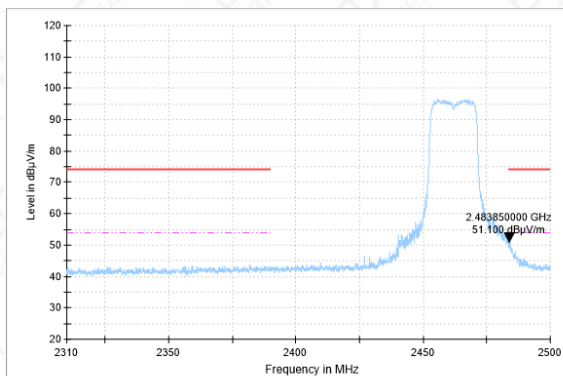
Bandedge-11N-CH11-AV
