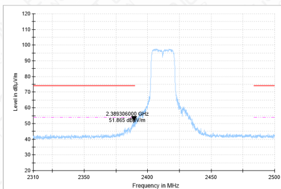
Bandedge-11N-CH1-AV
