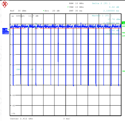
NTNV-11N20SISO-Ant1-2412
