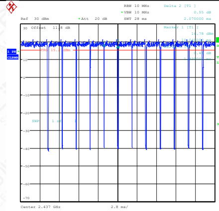
NTNV-11N20SISO-Ant1-2437
