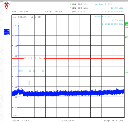
11B-Ant1-2437-1000~26500-PASS
