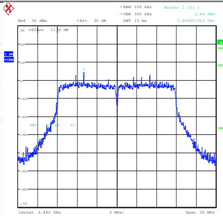
11N20SISO-Ant1-2462-0~Reference-PASS
