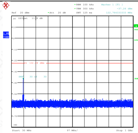
11B-Ant1-2437-30~1000-PASS
