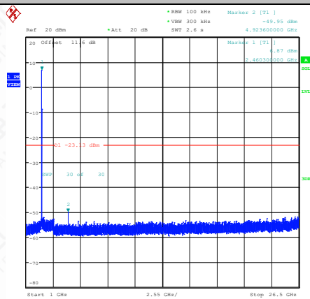
11B-Ant1-2462-1000~26500-PASS
