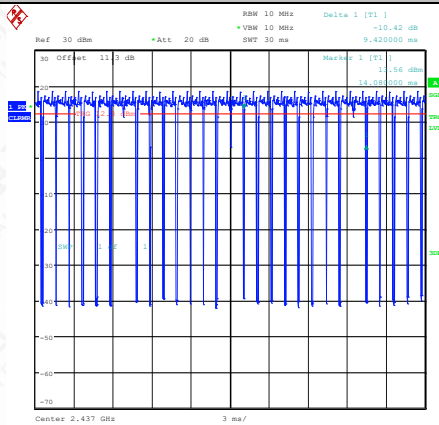
NTNV-11N40SISO-Ant1-2437
