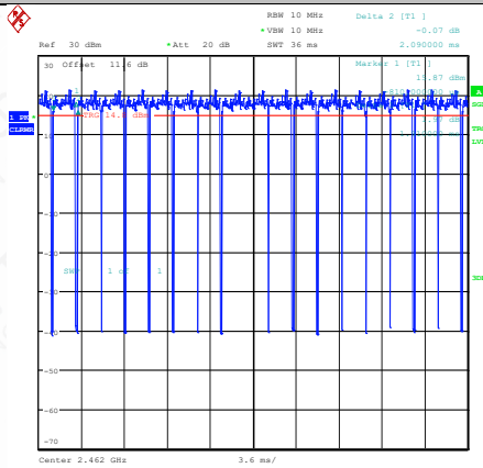
NTNV-11N20SISO-Ant1-2462
