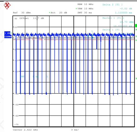
NTNV-11N40SISO-Ant1-2422
