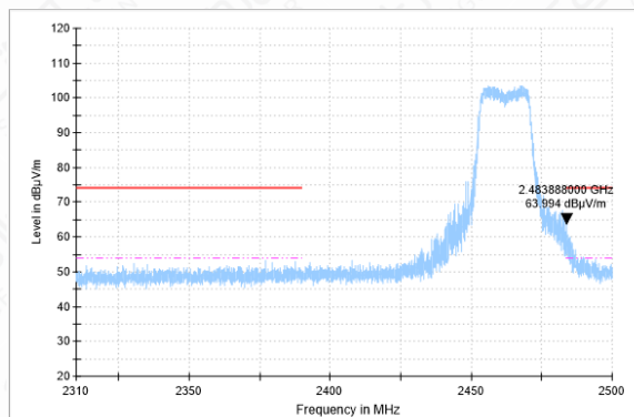
Bandedge-11N-CH11-PK
