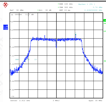
11G-Ant1-2412-0~Reference-PASS
