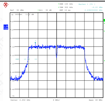
11N40SISO-Ant1-2452-0~Reference-PASS
