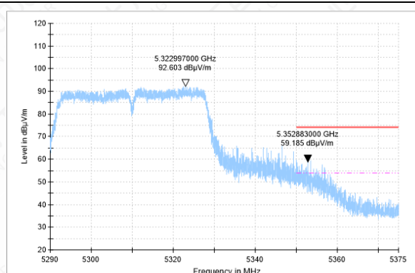
Bandedge-11AC(40M)-CH62-PK
