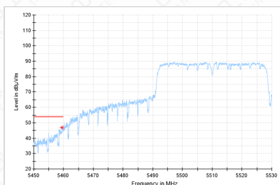
Bandedeg-11N(40M)-CH102-AV
