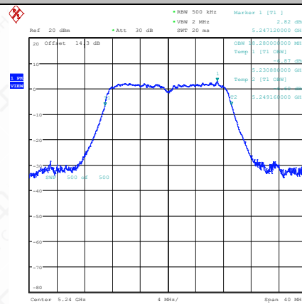
11N20SISO-Ant1-5240
