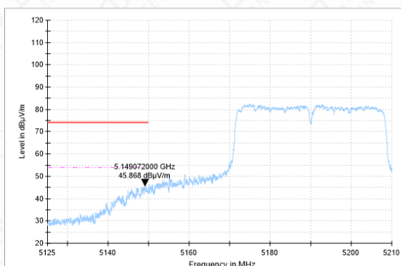
Bandedge-11AC(40M)-CH38-AV
