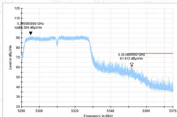
Bandedeg-11N(40M)-CH62-PK
