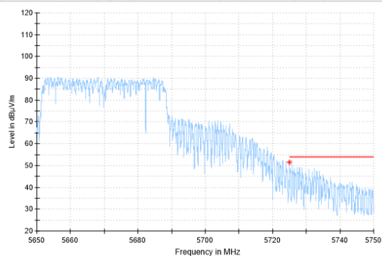
Bandedge-11N(40M)-CH134-AV-38-2.46
