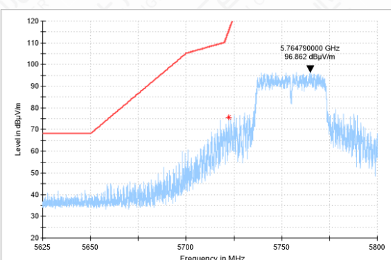
Bandedeg-11N(40M)-CH151-PK
