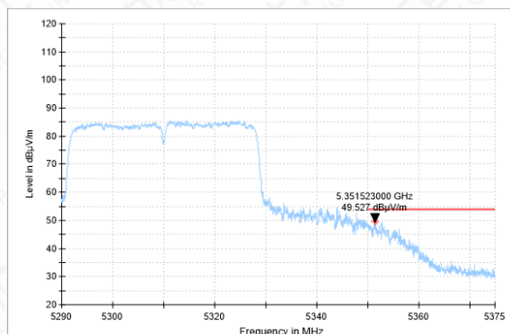
Bandedeg-11N(40M)-CH62-AV
