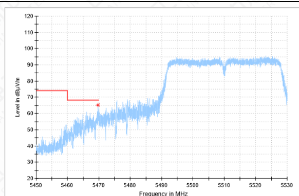
Bandedge-11AC(40M)-CH102-PK
