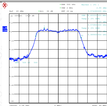
11AC20SISO-Ant1-5580
