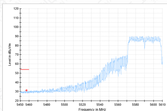
Bandedeg-11N(40M)-CH118-AV
