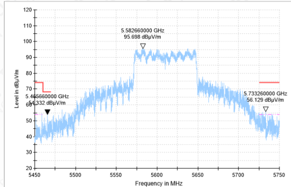
Bandedge-11AC(80M)-CH122-PK
