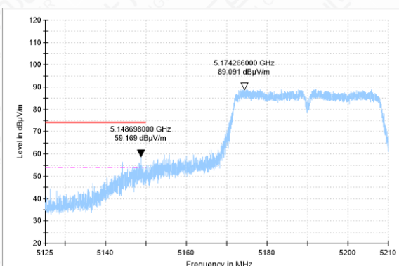
Bandedge-11AC(40M)-CH38-PK
