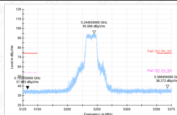
Bandedge-11N-CH48-PK
