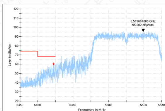
Bandedeg-11N(40M)-CH102-PK
