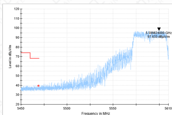
Bandedeg-11N(40M)-CH118-PK
