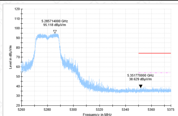
Bandedge-11N-CH56-PK
