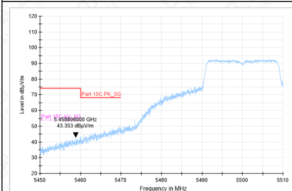
Bandedge-11N-CH100-AV
