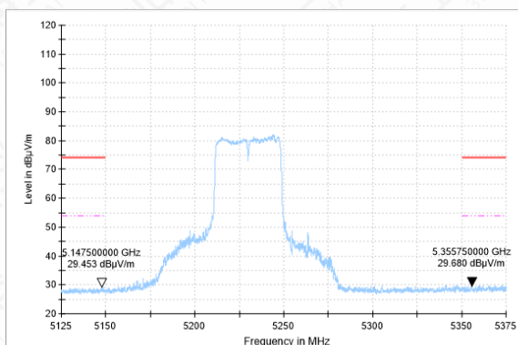
Bandedge-11AC(40M)-CH46-AV
