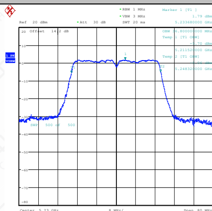
11AC40SISO-Ant1-5230
