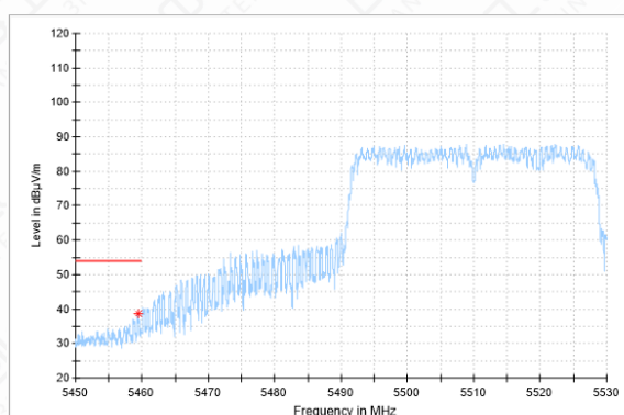
Bandedeg-11N(40M)-CH102-AV
