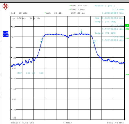
11N20SISO-Ant1-5580
