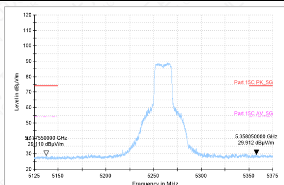
Bandedge-11N-CH52-AV
