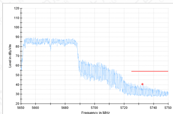
Bandedeg-11N(40M)-CH134-AV
