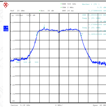
11N20SISO-Ant1-5180
