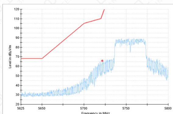
Bandedeg-11N(40M)-CH151-AV
