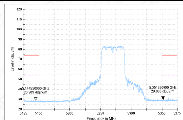
Bandedge-11AC(40M)-CH54-AV
