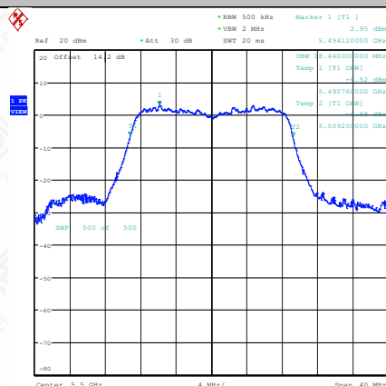
11AC20SISO-Ant1-5500
