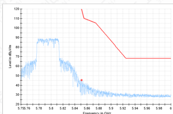
Bandedeg-11N(40M)-CH159-AV
