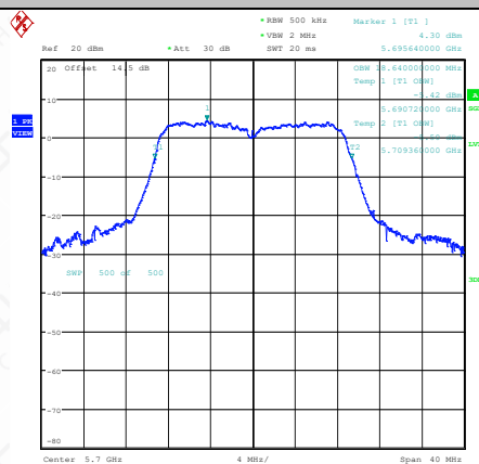
11N20SISO-Ant1-5700
