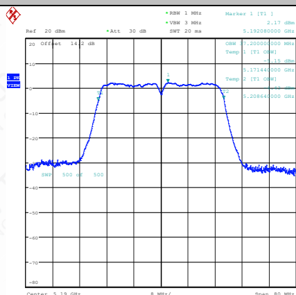
11AC40SISO-Ant1-5190
