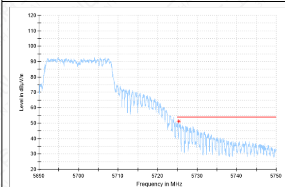
Bandedge-11N-CH140-AV
