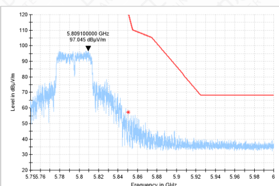
Bandedeg-11N(40M)-CH159-PK
