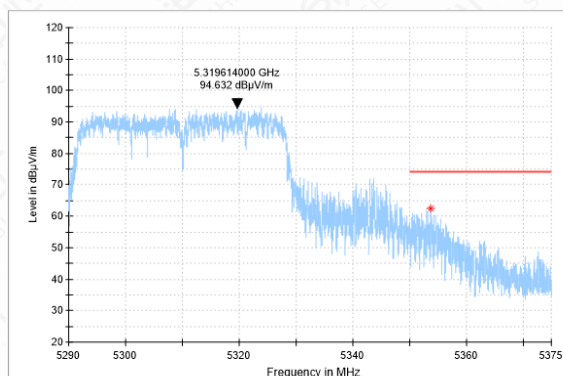
Bandedeg-11N(40M)-CH62-PK
