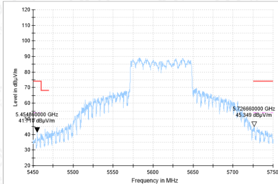
Bandedge-11AC(80M)-CH122-AV
