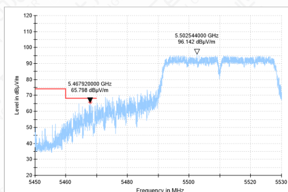
Bandedeg-11N(40M)-CH102-PK
