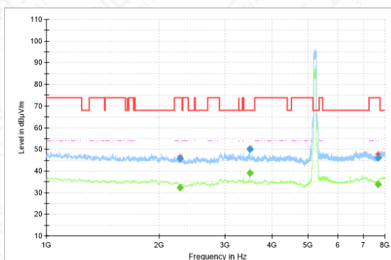
RSE-11AC(80M)-CH42-1GHz-8GHz
