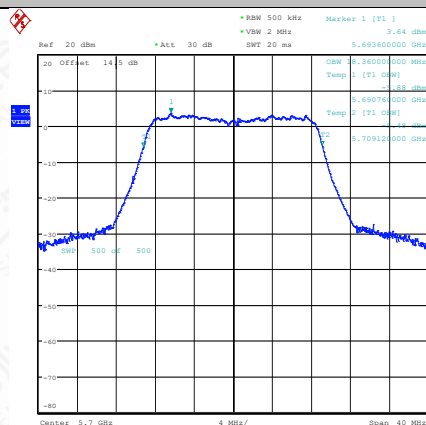
11AC20SISO-Ant1-5700
