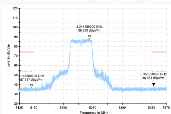
Bandedge-11AC(40M)-CH46-PK
