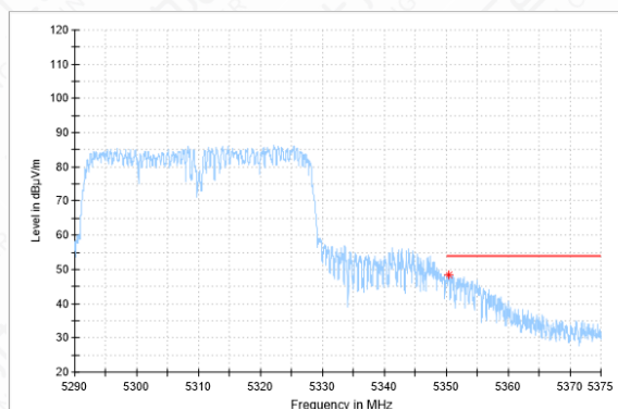
Bandedeg-11N(40M)-CH62-AV
