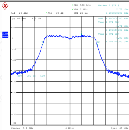
11N20SISO-Ant1-5200
