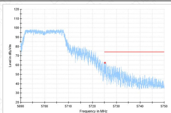
Bandedge-11N-CH140-PK
