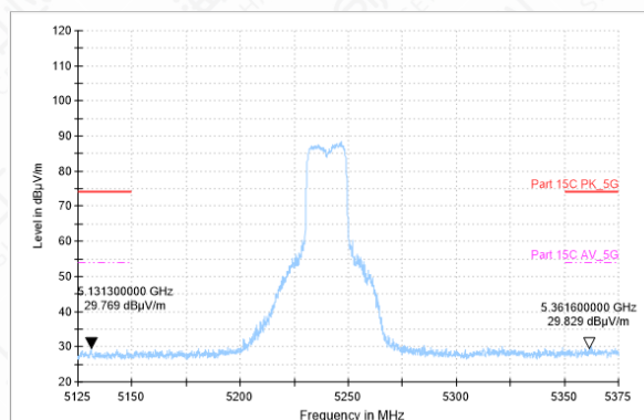
Bandedge-11N-CH48-AV
