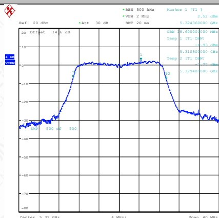
11AC20SISO-Ant1-5320
