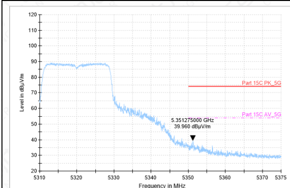
Bandedge-11N-CH64-AV
