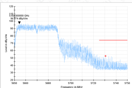
Bandedeg-11N(40M)-CH134-PK
