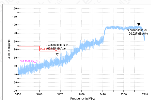
Bandedge-11N-CH100-PK
