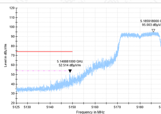
Bandedge-11N-CH36-PK
