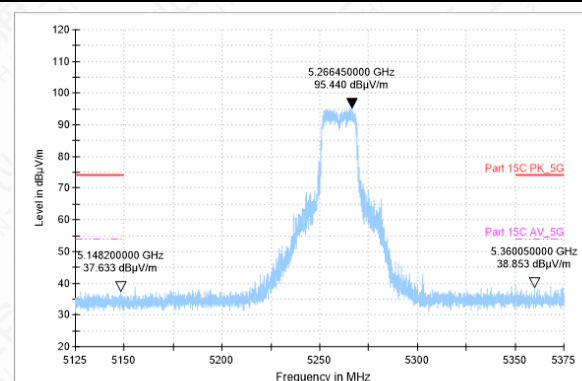
Bandedge-11N-CH52-PK
