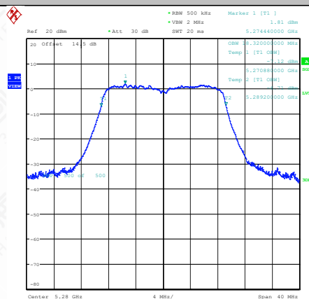
11N20SISO-Ant1-5280
