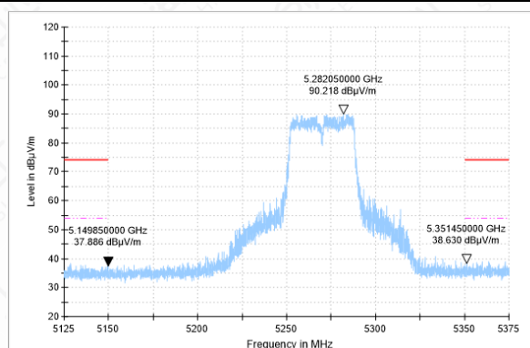
Bandedge-11AC(40M)-CH54-PK
