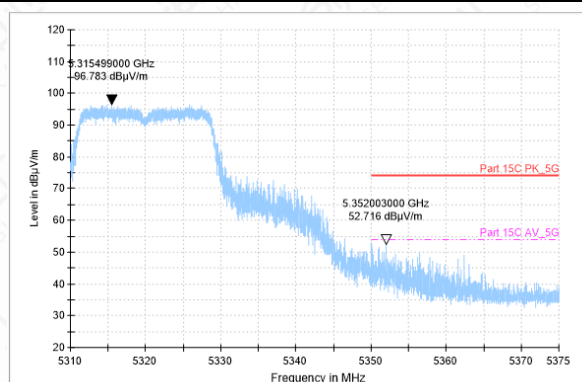
Bandedge-11N-CH64-PK
