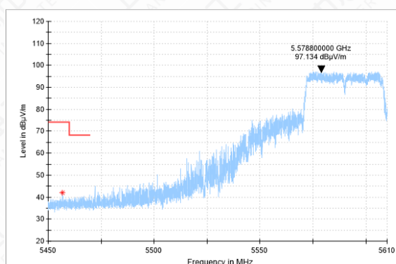
Bandedeg-11N(40M)-CH118-PK
