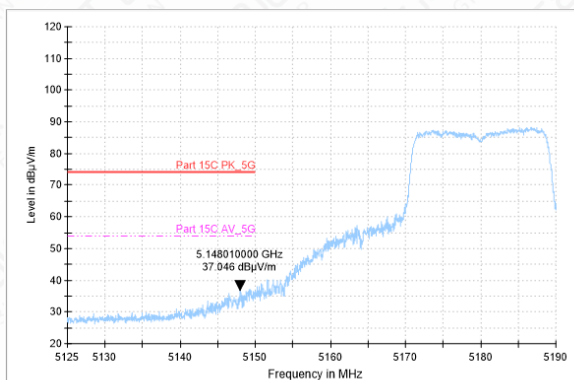
Bandedge-11N-CH36-AV
