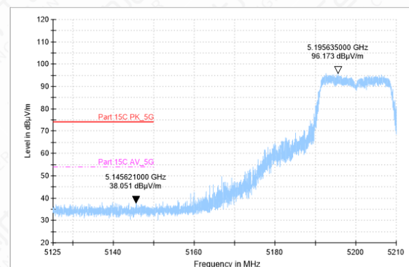
Bandedge-11N-CH40-PK
