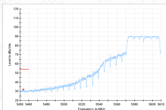
Bandedeg-11N(40M)-CH118-AV
