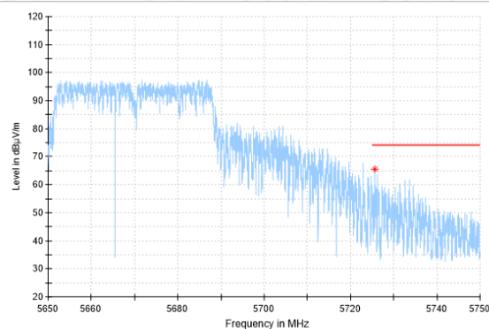
Bandedge-11N(40M)-CH134-PK-38-8.57
