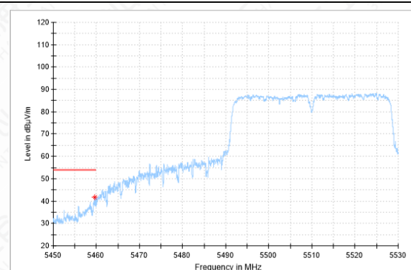
Bandedge-11AC(40M)-CH102-AV
