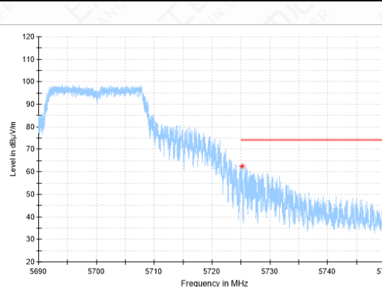
Bandedge-11A-CH140-PK-37
