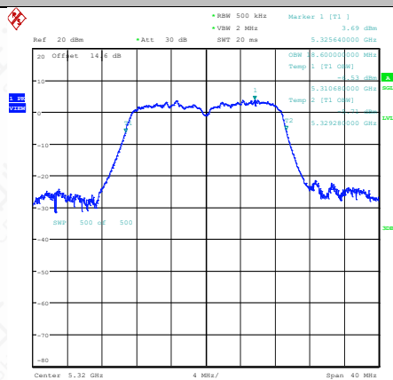
11N20SISO-Ant1-5320
