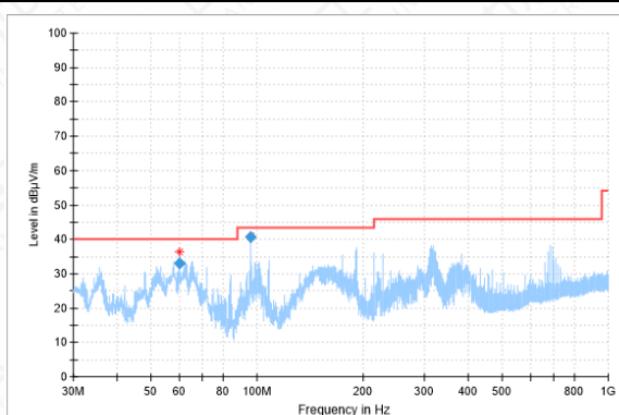
RSE-11N-CH64-30MHz-1GHz
