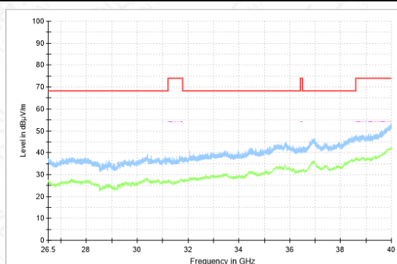
RSE-11N-CH40-26.5GHz-40GHz
