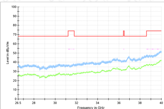
RSE-11N(40M)-CH134-26.5GHz-40GHz
