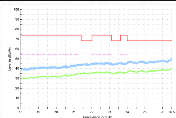
RSE-11N-CH40-18GHz-26.5GHz
