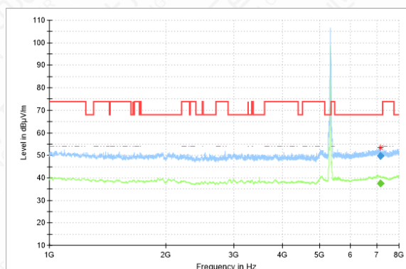
RSE-11N(40M)-CH62-1GHz-8GHz
