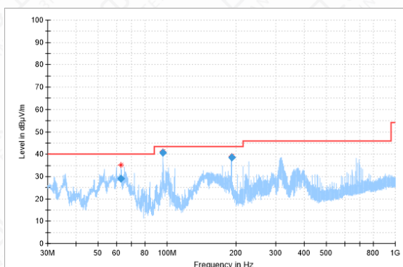
RSE-11N(40M)-CH62-30MHz-1GHz
