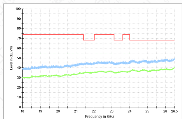
RSE-11AC-CH100-18GHz-26.5GHz
