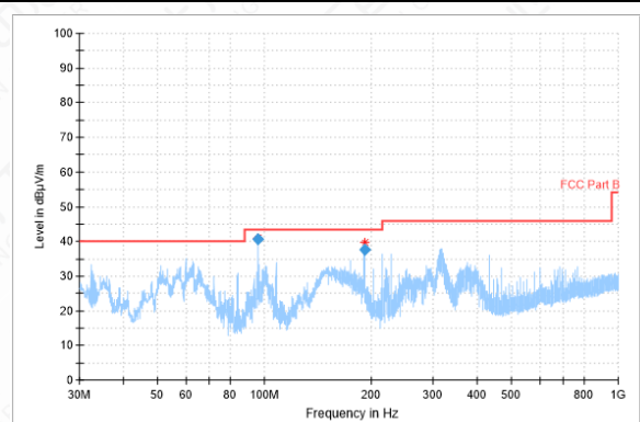
RSE-11A-CH40-30MHz-1GHz
