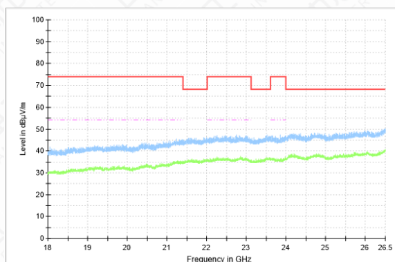
RSE-11N(40M)-CH62-18GHz-26.5GHz
