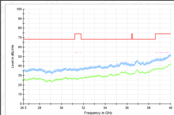
RSE-11AC-CH100-26.5GHz-40GHz
