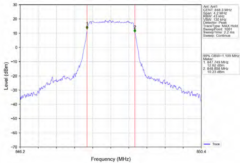
Band5_1.4MHz_16QAM_HCH_848.3MHz_RB_6_0_NTNV
