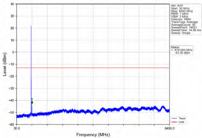
Band5_10MHz_64QAM_MCH_836.5MHz_RB_1_0_NTNV
