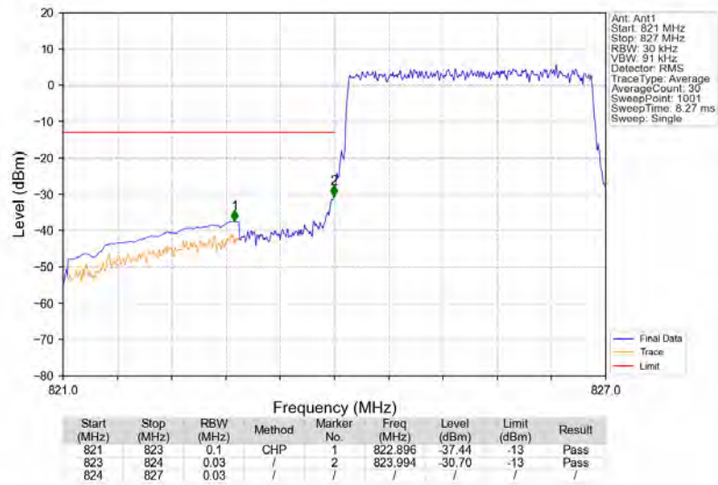
Band5_3MHz_16QAM_LCH_825.5MHz_RB_15_0_NTNV
