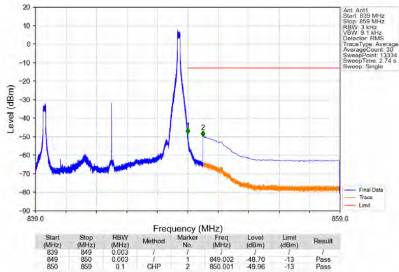
Band5_10MHz_64QAM_HCH_844MHz_RB_1_49_NTNV
