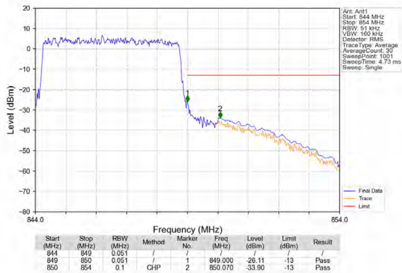
Band5_5MHz_16QAM_HCH_846.5MHz_RB_25_0_NTNV
