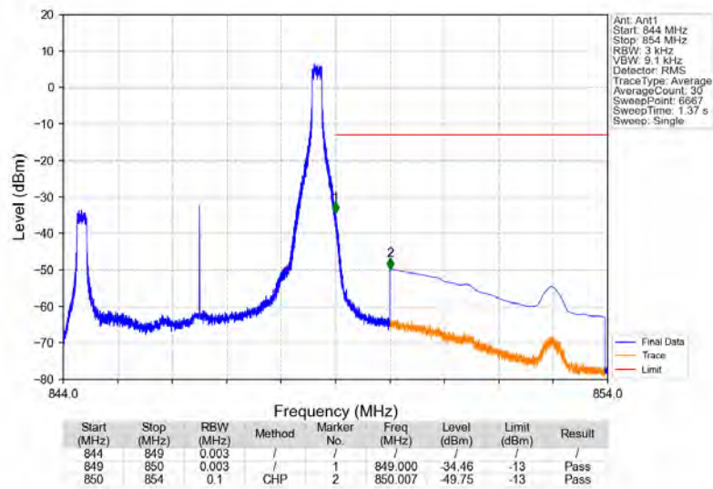
Band5_5MHz_64QAM_HCH_846.5MHz_RB_1_24_NTNV
