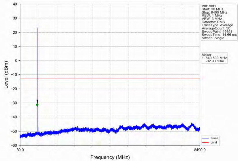
Band5_1.4MHz_16QAM_HCH_848.3MHz_RB_1_0_NTNV
