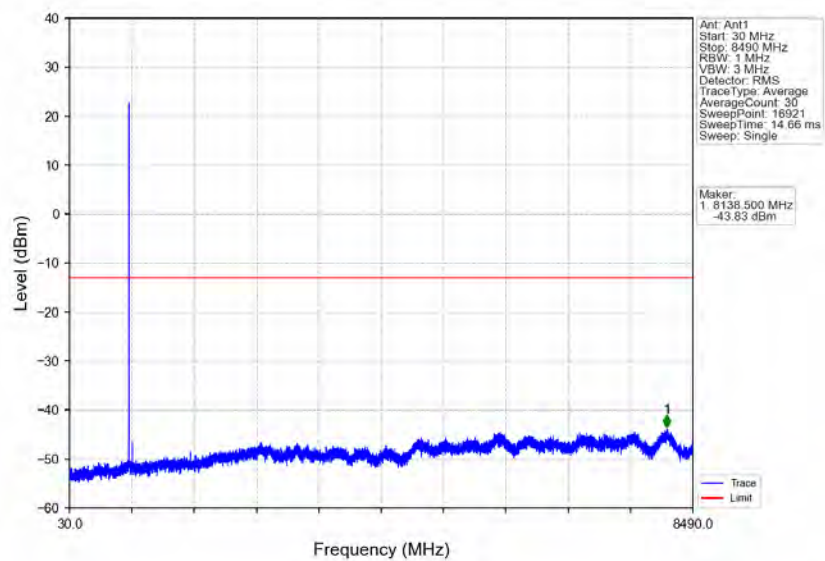
Band5_3MHz_64QAM_MCH_836.5MHz_RB_1_0_NTNV
