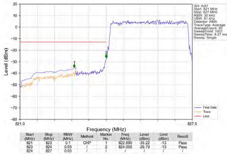
Band5_3MHz_QPSK_LCH_825.5MHz_RB_15_0_NTNV
