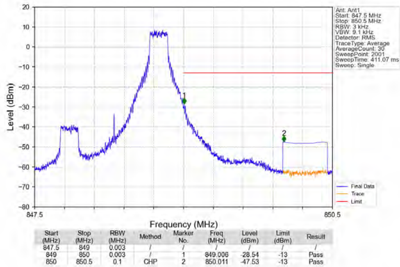
Band5_1.4MHz_16QAM_HCH_848.3MHz_RB_1_5_NTNV
