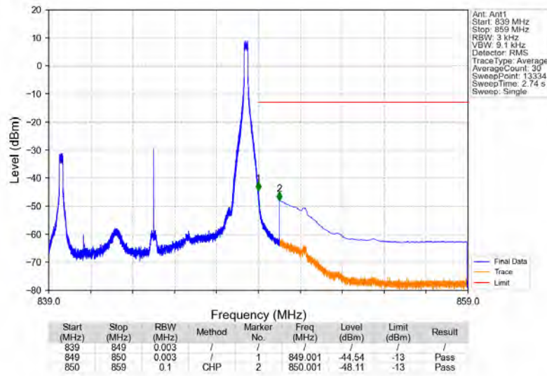
Band5 10MHz 16QAM HCH 844MHz RB 1 49 NTNV
