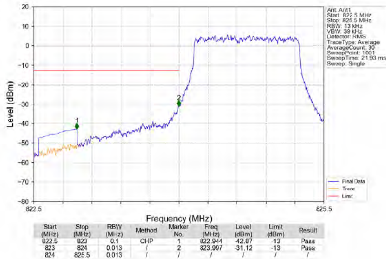
Band5_1.4MHz_16QAM_LCH_824.7MHz_RB_6_0_NTNV
