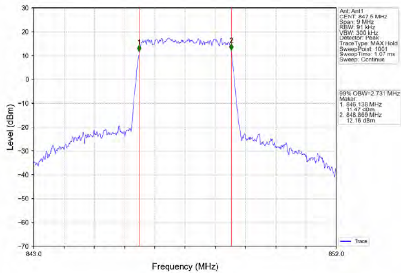
Band5_3MHz_64QAM_HCH_847.5MHz_RB_15_0_NTNV
