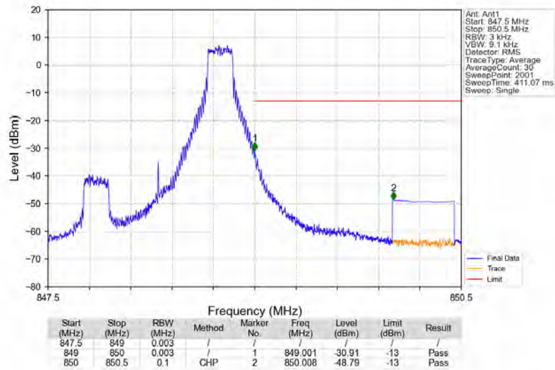
Band5_1.4MHz_64QAM_HCH_848.3MHz_RB_1_5_NTNV
