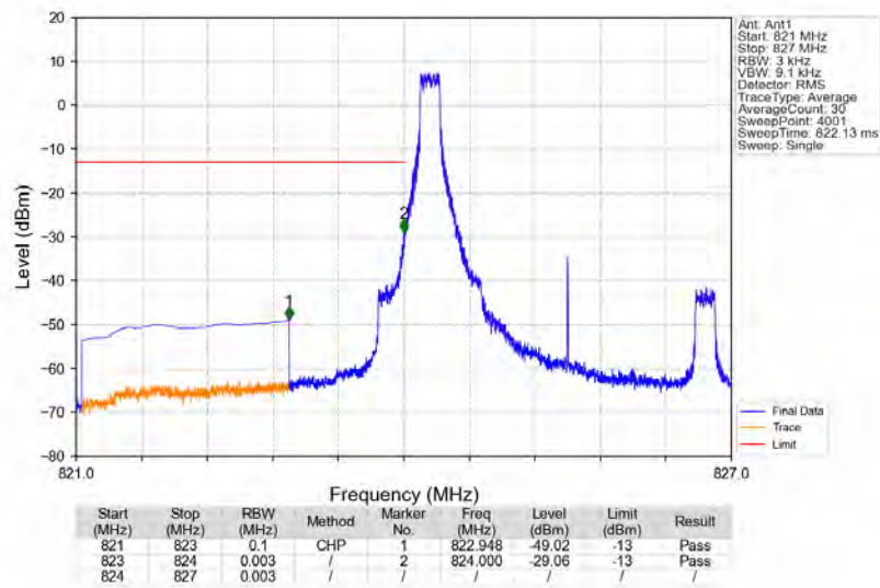
Band5_3MHz_16QAM_LCH_825.5MHz_RB_1_0_NTNV
