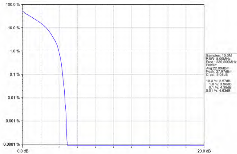
Band5_1.4MHz_QPSK_MCH_836.5MHz_RB_6_0_NTNV
