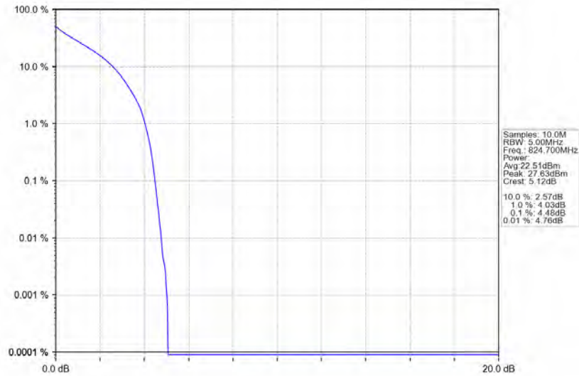
Band5_1.4MHz_QPSK_LCH_824.7MHz_RB_6_0_NTNV
