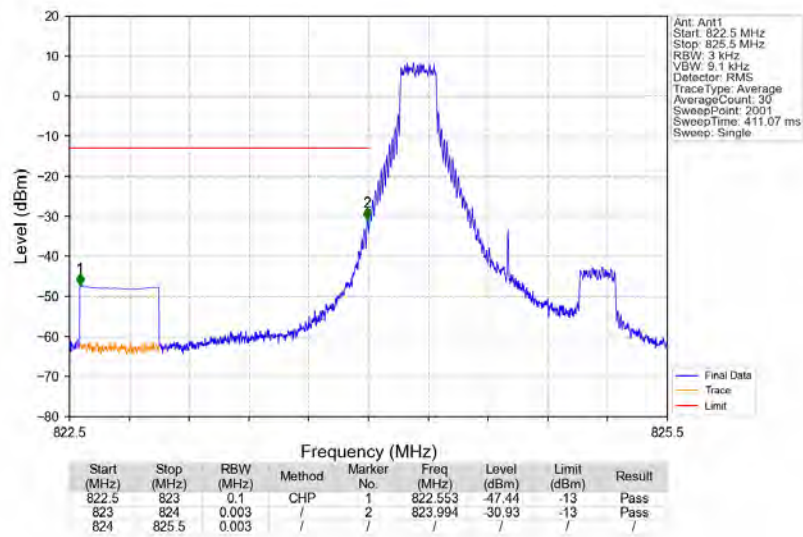
Band5_1.4MHz_16QAM_LCH_824.7MHz_RB_1_0_NTNV
