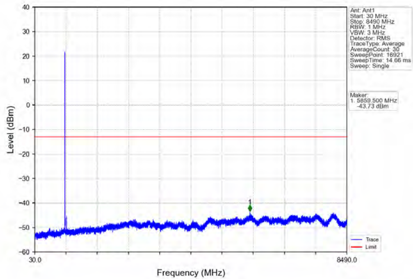
Band5_5MHz_64QAM_HCH_846.5MHz_RB_1_24_NTNV
