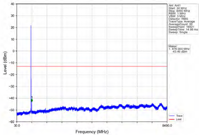
Band5_10MHz_64QAM_LCH_829MHz_RB_1_0_NTNV
