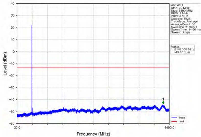
Band5_3MHz_64QAM_HCH_847.5MHz_RB_1_14_NTNV
