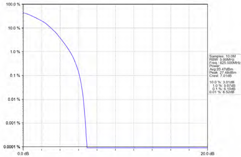
Band5_3MHz_64QAM_LCH_825.5MHz_RB_15_0_NTNV
