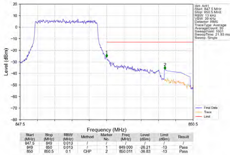
Band5_1.4MHz_QPSK_HCH_848.3MHz_RB_6_0_NTNV
