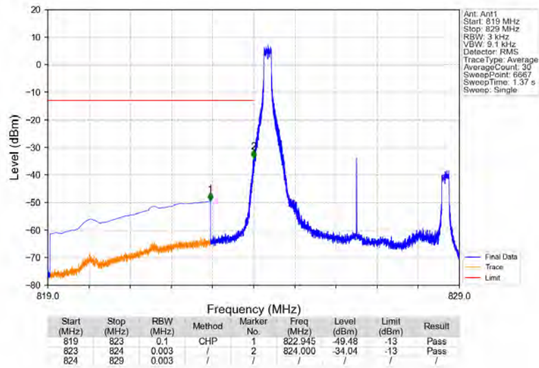
Band5_5MHz_64QAM_LCH_826.5MHz_RB_1_0_NTNV
