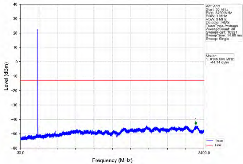
Band5_3MHz_16QAM_LCH_825.5MHz_RB_15_0_NTNV
