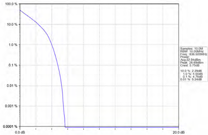
Band5_10MHz_QPSK_MCH_836.5MHz_RB_50_0_NTNV
