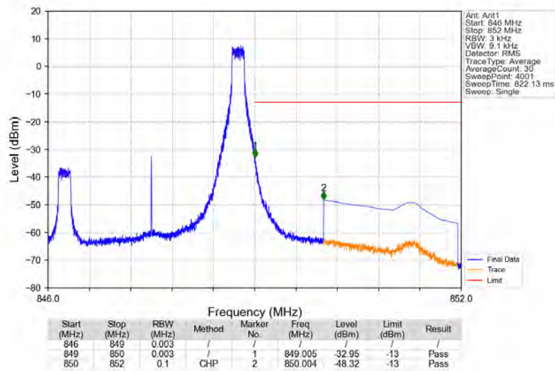
Band5_3MHz_64QAM_HCH_847.5MHz_RB_1_14_NTNV
