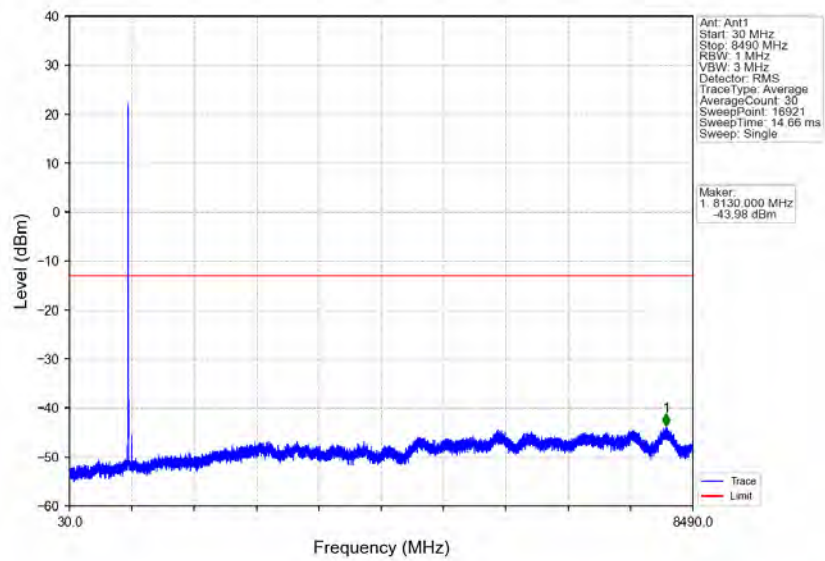
Band5_5MHz_64QAM_LCH_826.5MHz_RB_1_0_NTNV
