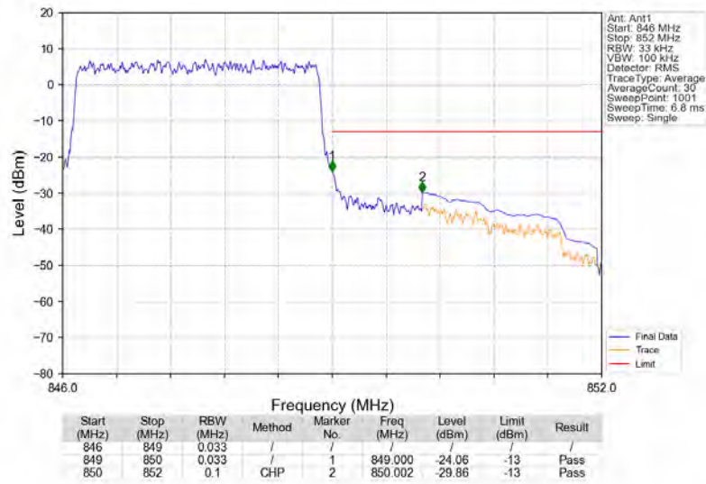
Band5_3MHz_QPSK_HCH_847.5MHz_RB_15_0_NTNV
