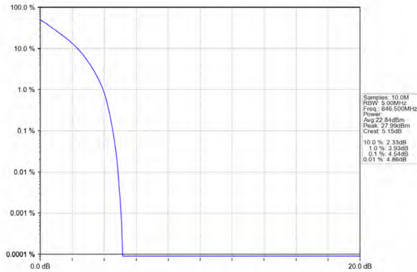
Band5_5MHz_QPSK_HCH_846.5MHz_RB_25_0_NTNV
