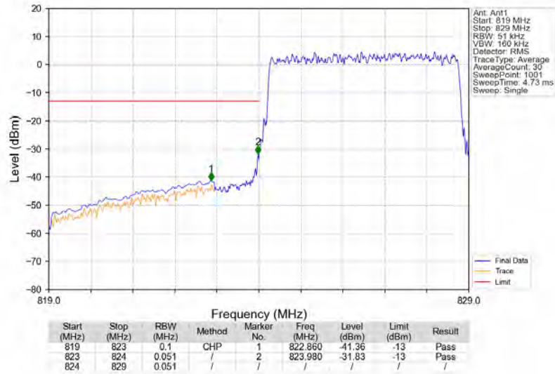
Band5_5MHz_64QAM_LCH_826.5MHz_RB_25_0_NTNV
