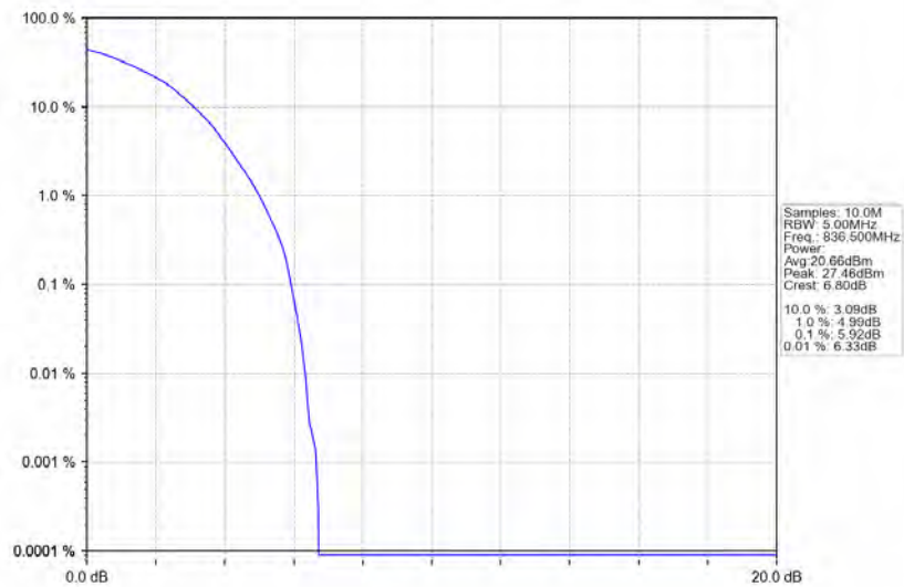
Band5_1.4MHz_64QAM_MCH_836.5MHz_RB_6_0_NTNV
