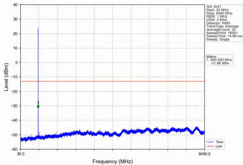
Band5 1.4MHz QPSK MCH 836.5MHz RB 1 0 NTNV
