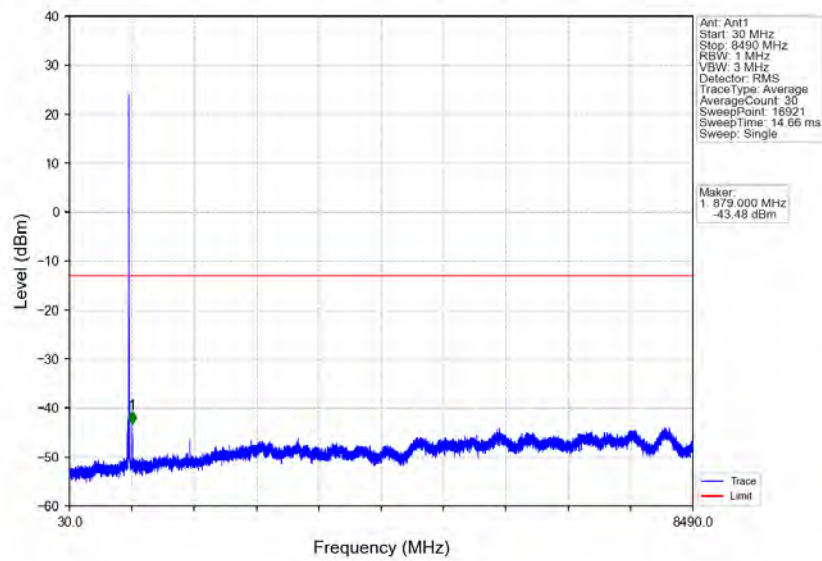
Band5_10MHz_QPSK_MCH_836.5MHz_RB_1_0_NTNV
