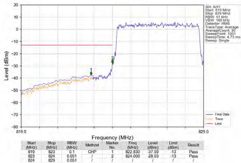
Band5_5MHz_16QAM_LCH_826.5MHz_RB_25_0_NTNV
