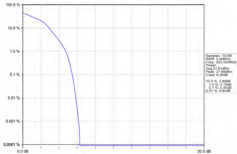
Band5_3MHz_16QAM_LCH_825.5MHz_RB_15_0_NTNV
