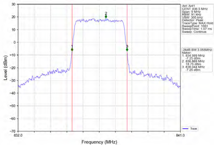
Band5_3MHz_16QAM_MCH_836.5MHz_RB_15_0_NTNV
