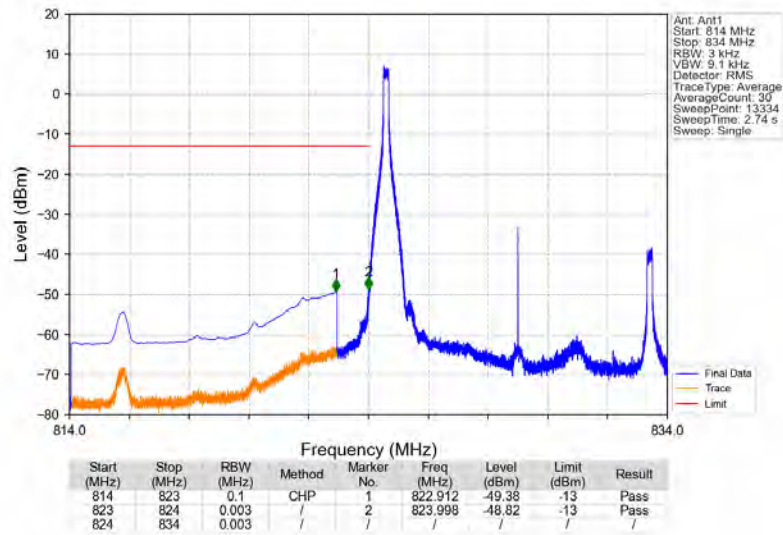
Band5_10MHz_64QAM_LCH_829MHz_RB_1_0_NTNV
