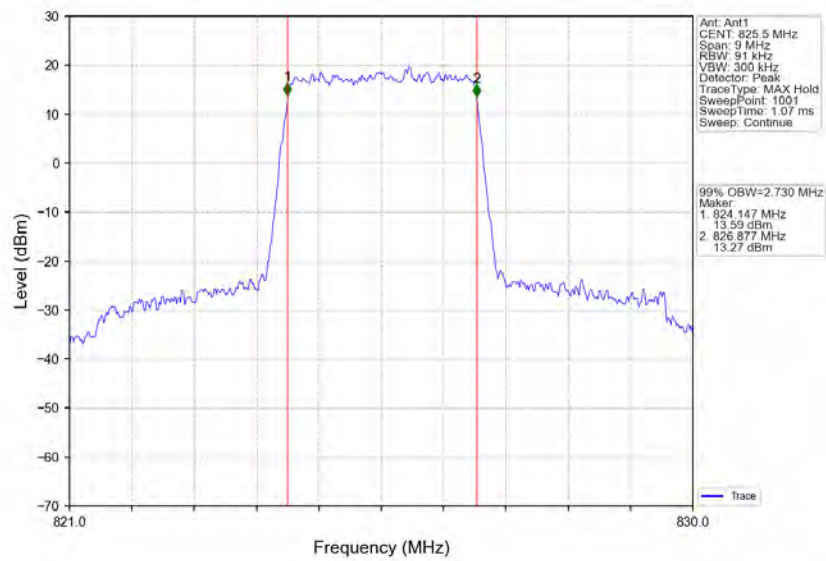
Band5_3MHz_QPSK_LCH_825.5MHz_RB_15_0_NTNV
