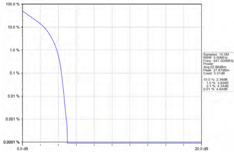
Band5_3MHz_QPSK_HCH_847.5MHz_RB_15_0_NTNV
