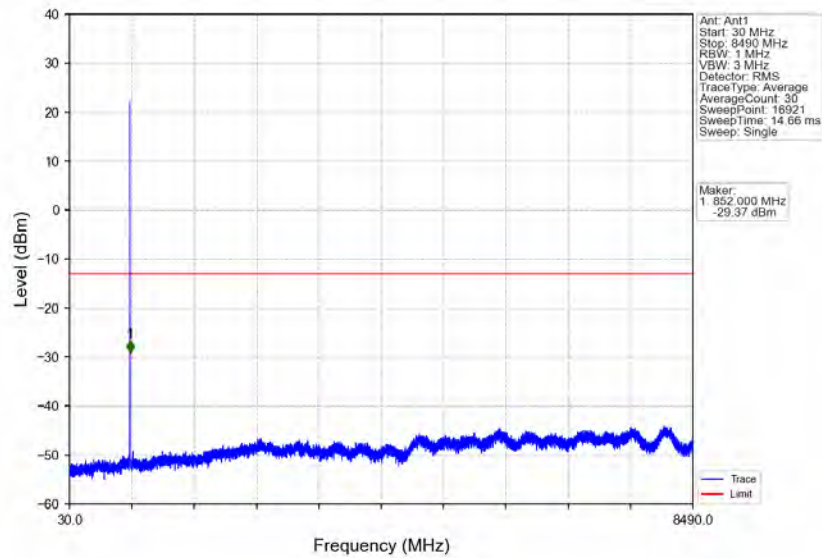
Band5_1.4MHz_64QAM_HCH_848.3MHz_RB_1_5_NTNV
