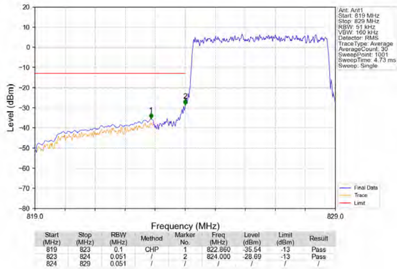
Band5_5MHz_QPSK_LCH_826.5MHz_RB_25_0_NTNV
