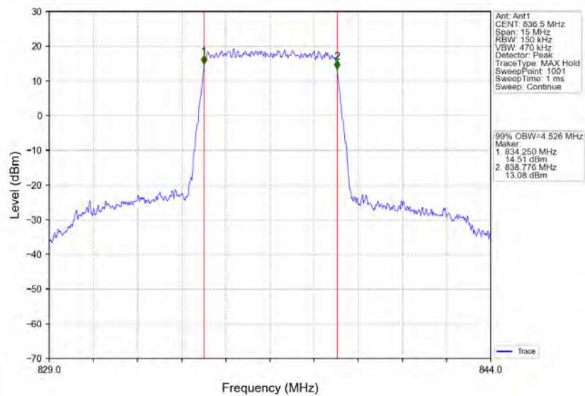
Band5_5MHz_QPSK_MCH_836.5MHz_RB_25_0_NTNV
