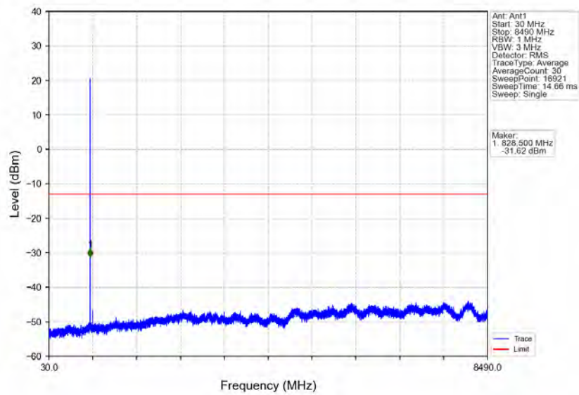
Band5_1.4MHz_64QAM_LCH_824.7MHz_RB_1_0_NTNV
