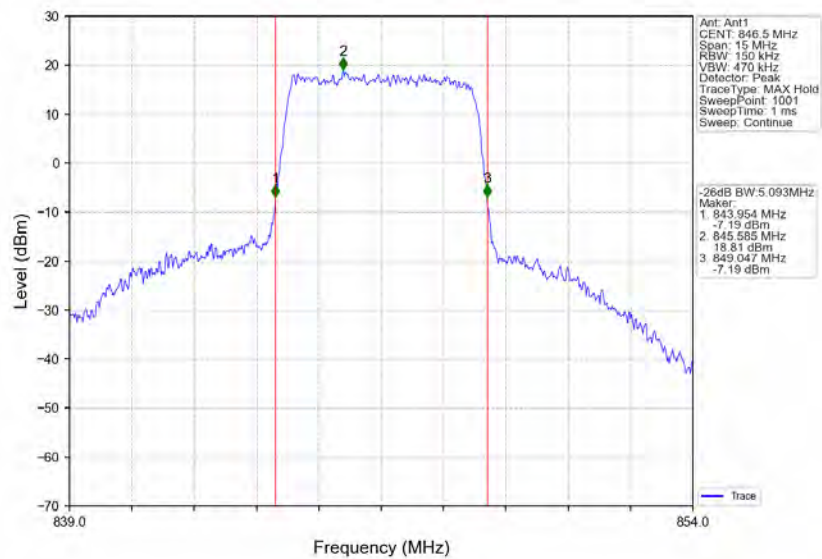
Band5_5MHz_16QAM_HCH_846.5MHz_RB_25_0_NTNV
