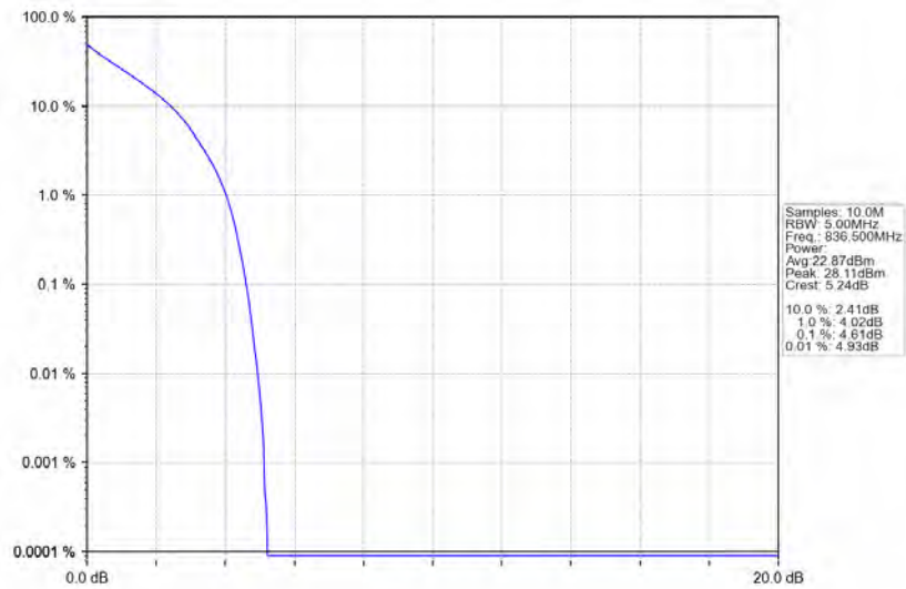
Band5_3MHz_QPSK_MCH_836.5MHz_RB_15_0_NTNV
