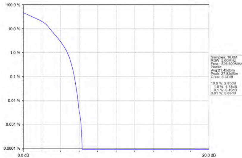
Band5_5MHz_16QAM_LCH_826.5MHz_RB_25_0_NTNV
