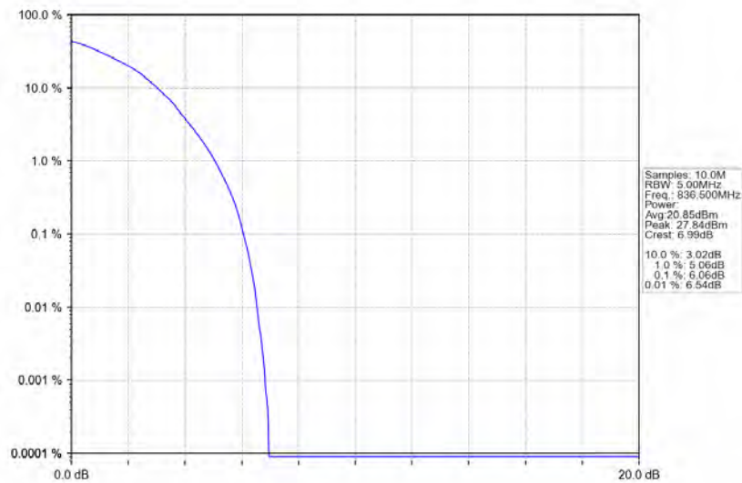
Band5_3MHz_64QAM_MCH_836.5MHz_RB_15_0_NTNV
