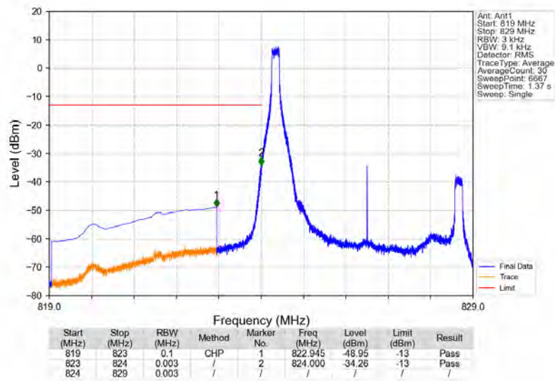
Band5_5MHz_16QAM_LCH_826.5MHz_RB_1_0_NTNV
