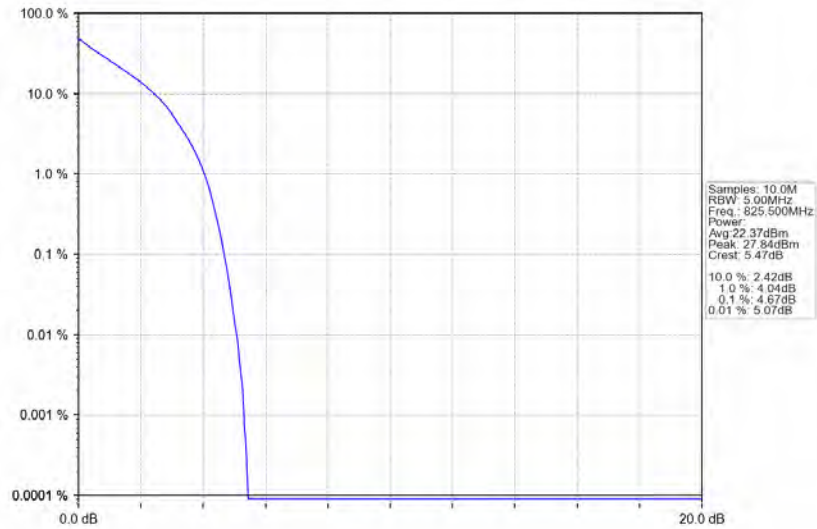
Band5_3MHz_QPSK_LCH_825.5MHz_RB_15_0_NTNV
