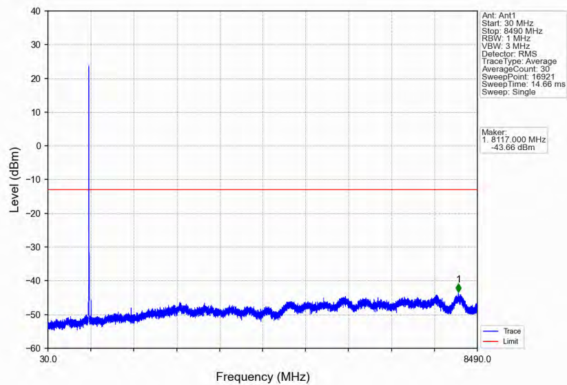
Band5_5MHz_QPSK_MCH_836.5MHz_RB_1_0_NTNV
