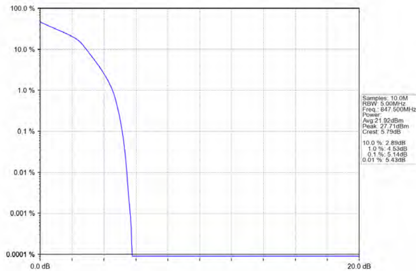
Band5_3MHz_16QAM_HCH_847.5MHz_RB_15_0_NTNV
