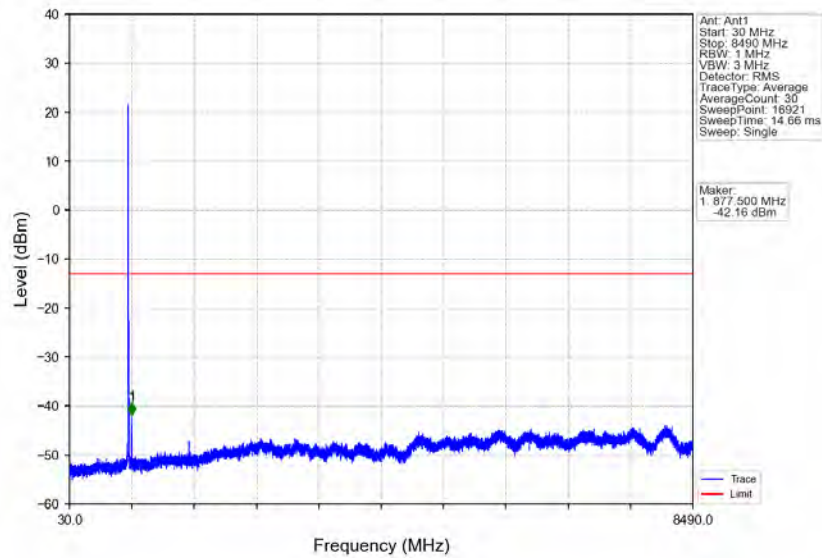
Band5_10MHz_16QAM_LCH_829MHz_RB_50_0_NTNV
