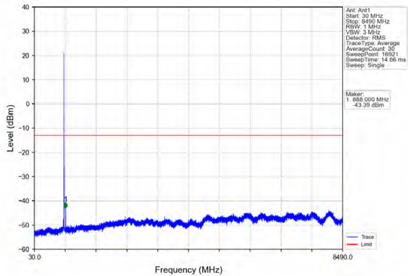
Band5_10MHz_64QAM_HCH_844MHz_RB_1_49_NTNV
