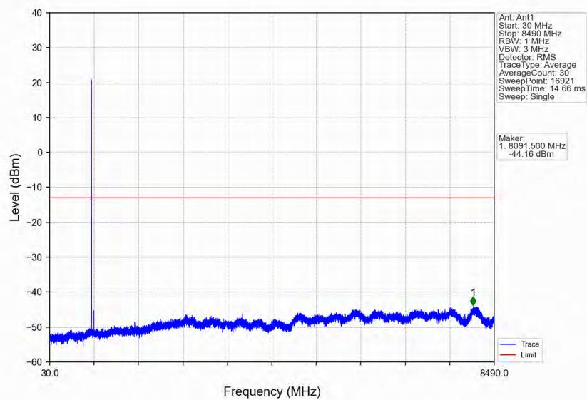
Band5_3MHz_64QAM_LCH_825.5MHz_RB_1_0_NTNV
