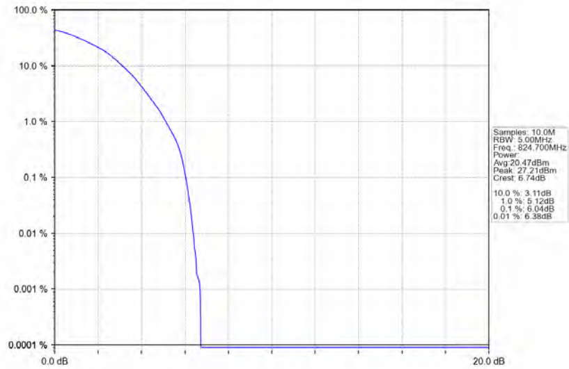
Band5_1.4MHz_64QAM_LCH_824.7MHz_RB_6_0_NTNV
