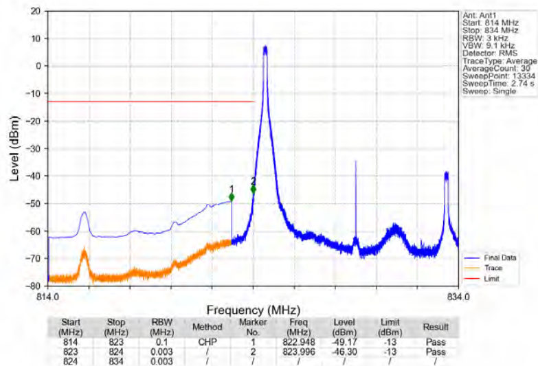
Band5_10MHz_16QAM_LCH_829MHz_RB_1_0_NTNV
