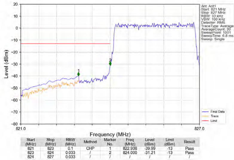
Band5_3MHz_64QAM_LCH_825.5MHz_RB_15_0_NTNV
