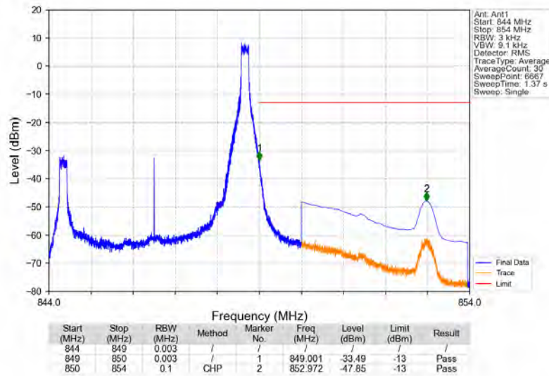
Band5_5MHz_16QAM_HCH_846.5MHz_RB_1_24_NTNV
