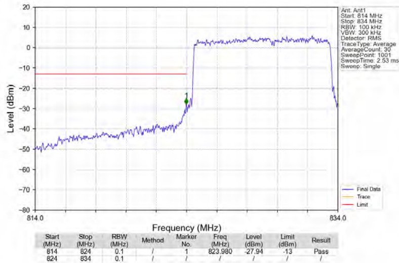
Band5_10MHz_16QAM_LCH_829MHz_RB_50_0_NTNV
