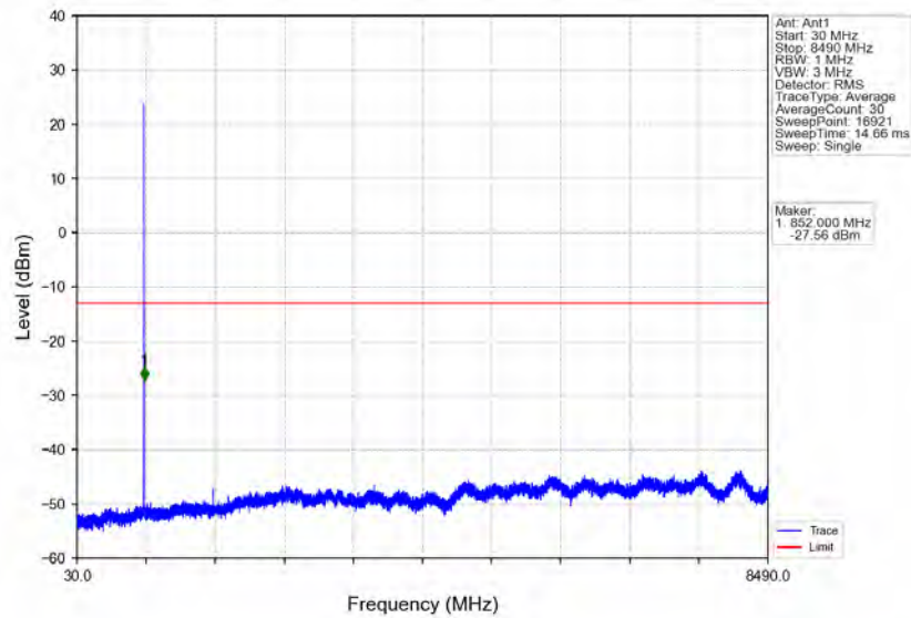
Band5_1.4MHz_QPSK_HCH_848.3MHz_RB_1_5_NTNV
