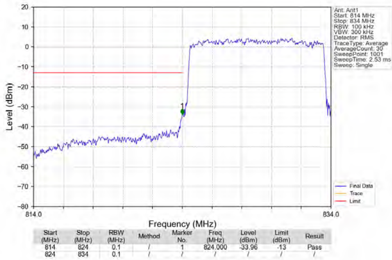
Band5_10MHz_64QAM_LCH_829MHz_RB_50_0_NTNV
