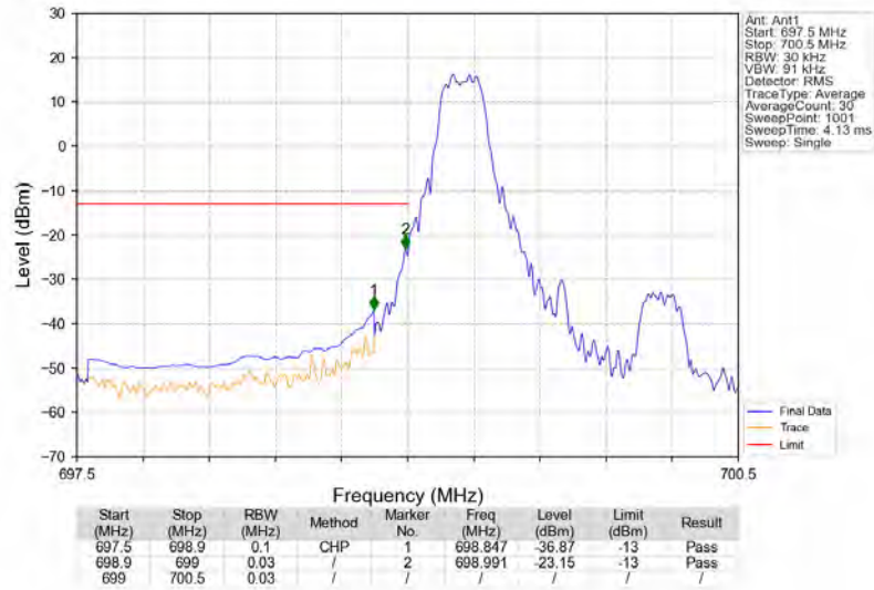
Band12_1.4MHz_64QAM_LCH_699.7MHz_RB_1_0_NTNV
