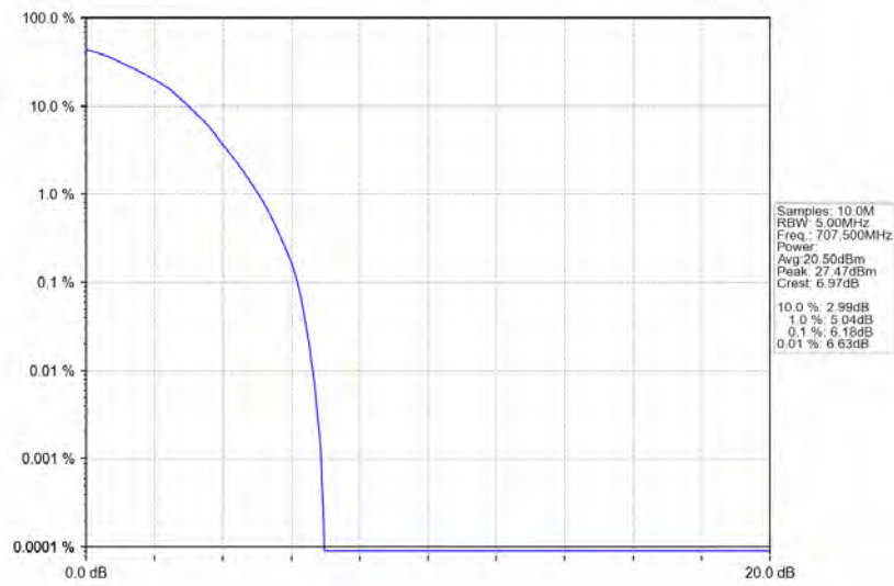
Band12_3MHz_64QAM_MCH_707.5MHz_RB_15_0_NTNV
