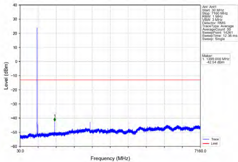
Band12_3MHz_QPSK_LCH_700.5MHz_RB_1_0_NTNV
