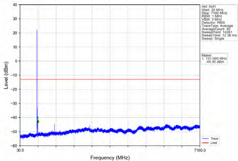
Band12_5MHz_64QAM_LCH_701.5MHz_RB_1_0_NTNV
