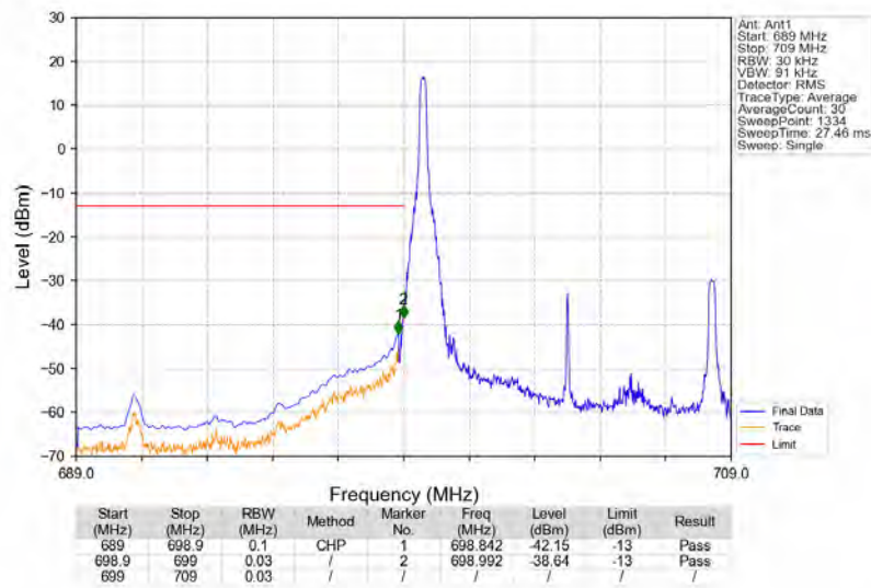
Band12_10MHz_16QAM_LCH_704MHz_RB_1_0_NTNV
