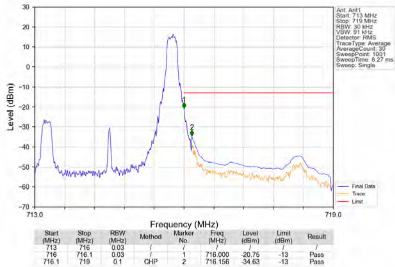
Band12_3MHz_64QAM_HCH_714.5MHz_RB_1_14_NTNV
