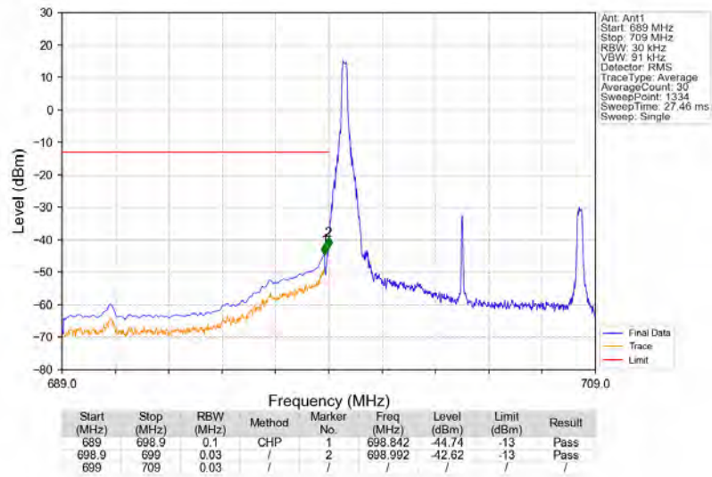
Band12_10MHz_64QAM_LCH_704MHz_RB_1_0_NTNV
