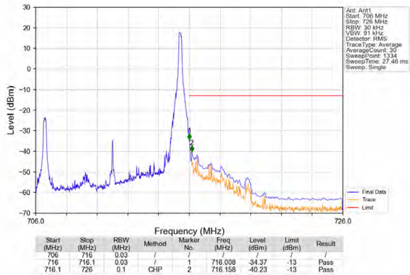
Band12_10MHz_QPSK_HCH_711MHz_RB_1_49_NTNV
