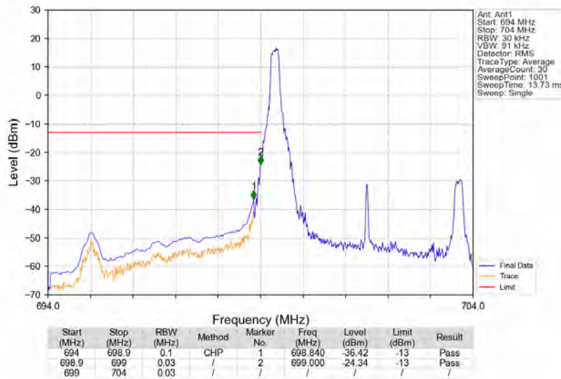
Band12_5MHz_16QAM_LCH_701.5MHz_RB_1_0_NTNV
