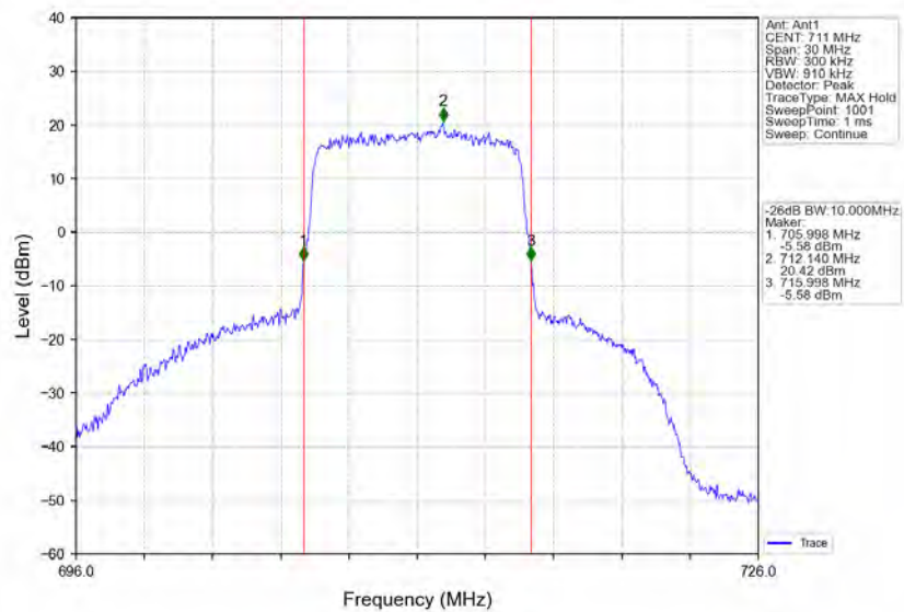
Band12_10MHz_QPSK_HCH_711MHz_RB_50_0_NTNV
