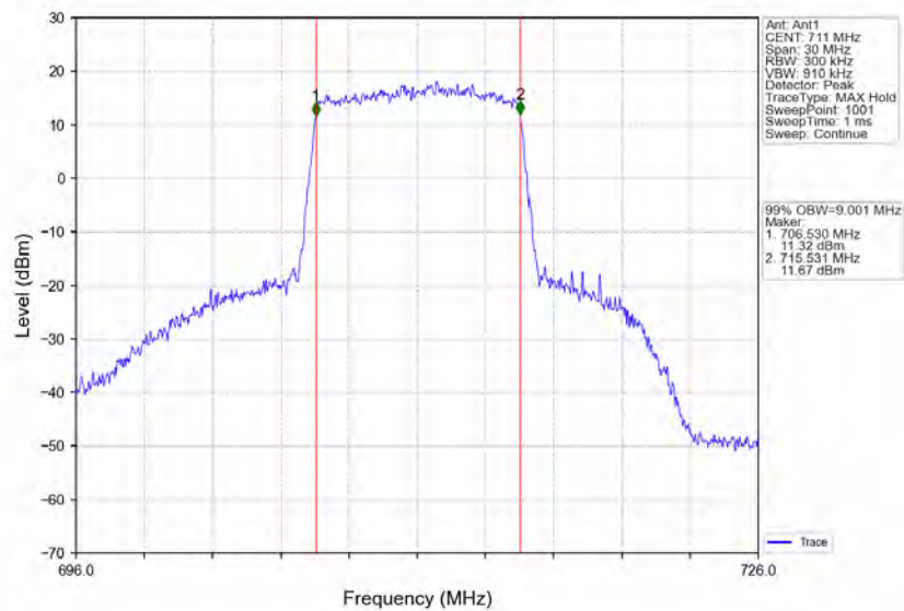
Band12_10MHz_64QAM_HCH_711MHz_RB_50_0_NTNV
