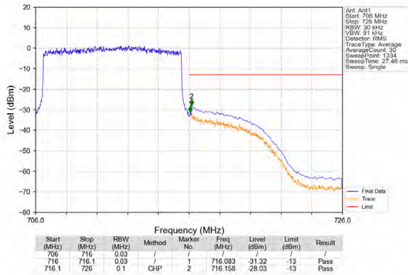
Band12_10MHz_QPSK_HCH_711MHz_RB_50_0_NTNV
