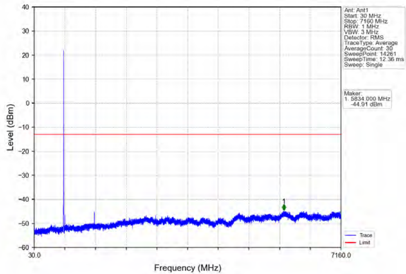
Band12_3MHz_64QAM_HCH_714.5MHz_RB_1_14_NTNV
