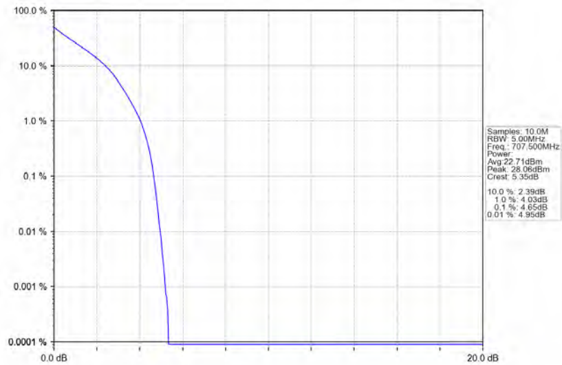
Band12_3MHz_QPSK_MCH_707.5MHz_RB_15_0_NTNV
