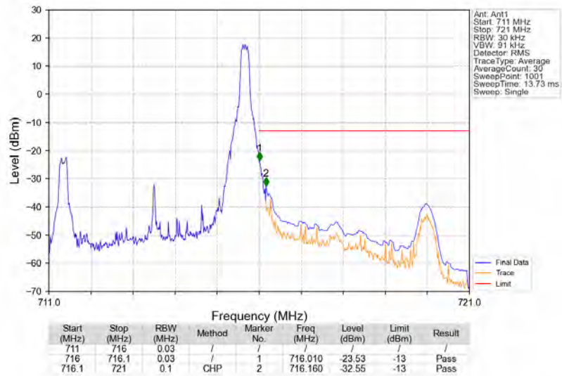
Band12_5MHz_QPSK_HCH_713.5MHz_RB_1_24_NTNV
