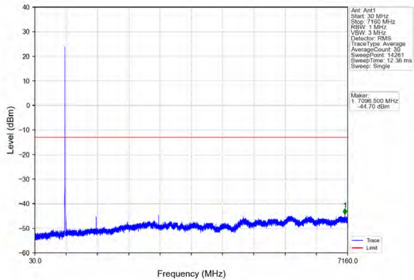
Band12_3MHz_QPSK_HCH_714.5MHz_RB_1_14_NTNV
