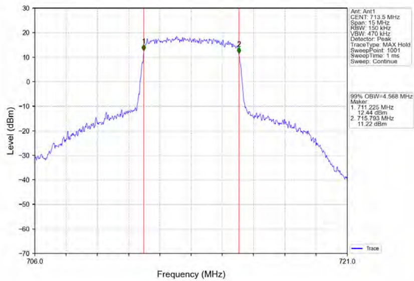
Band12_5MHz_16QAM_HCH_713.5MHz_RB_25_0_NTNV
