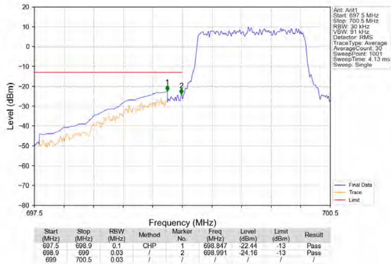
Band12_1.4MHz_16QAM_LCH_699.7MHz_RB_6_0_NTNV
