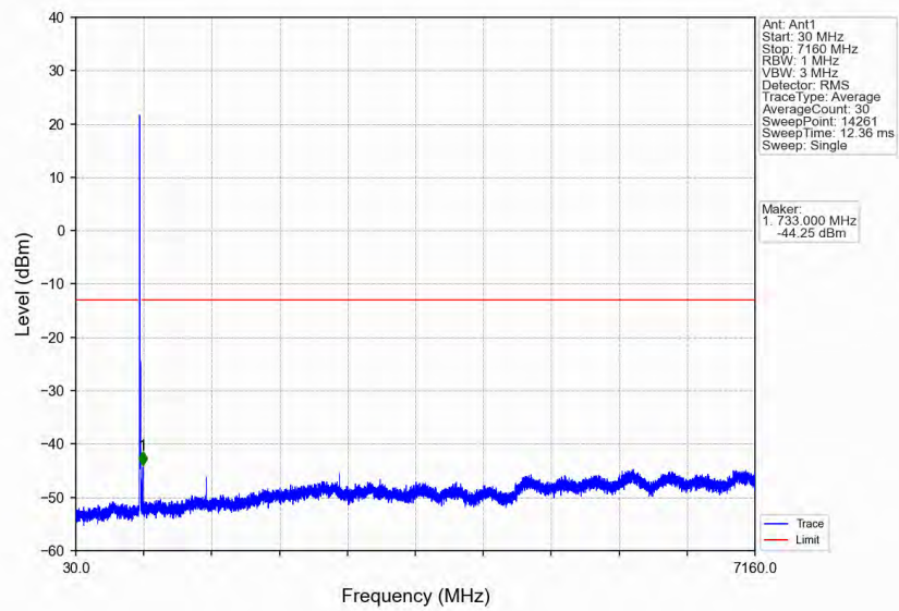
Band12_10MHz_64QAM_LCH_704MHz_RB_1_0_NTNV
