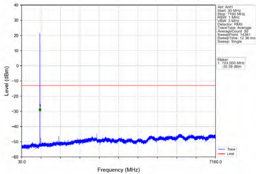
Band12_1.4MHz_64QAM_LCH_699.7MHz_RB_1_0_NTNV
