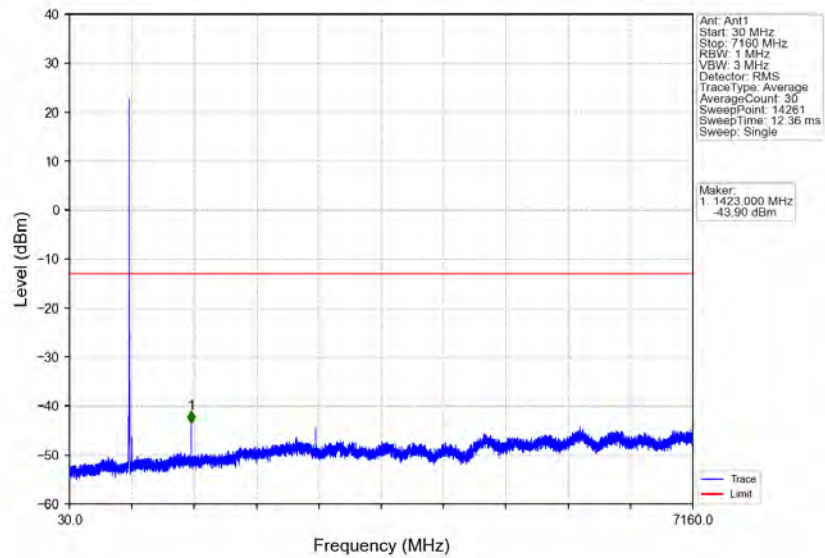
Band12_5MHz_QPSK_HCH_713.5MHz_RB_1_24_NTNV
