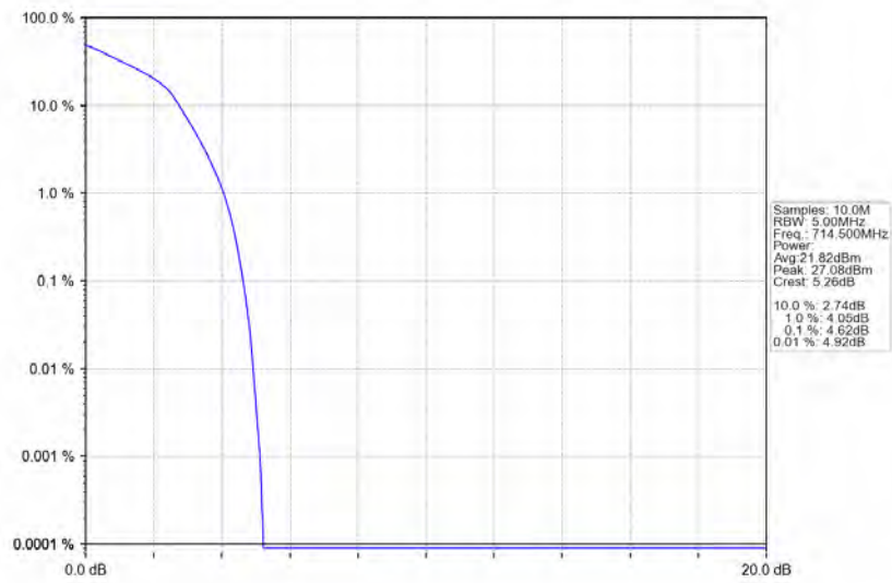
Band12_3MHz_16QAM_HCH_714.5MHz_RB_15_0_NTNV
