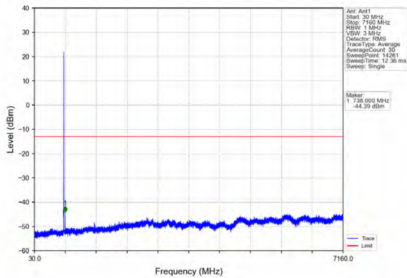
Band12_3MHz_64QAM_MCH_707.5MHz_RB_1_0_NTNV
