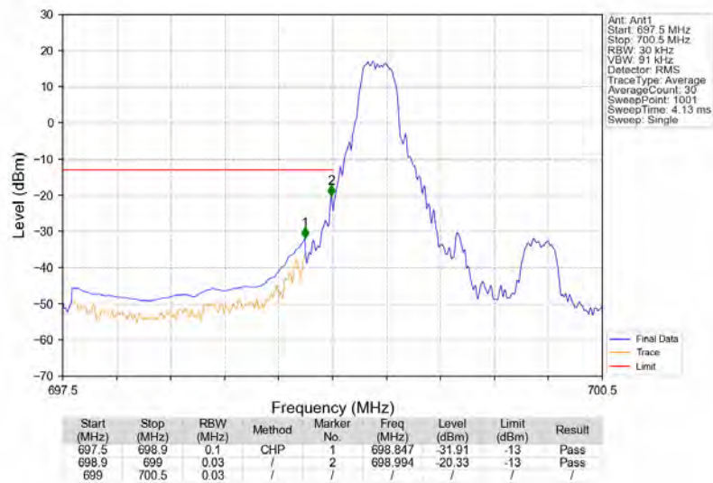
Band12_1.4MHz_16QAM_LCH_699.7MHz_RB_1_0_NTNV
