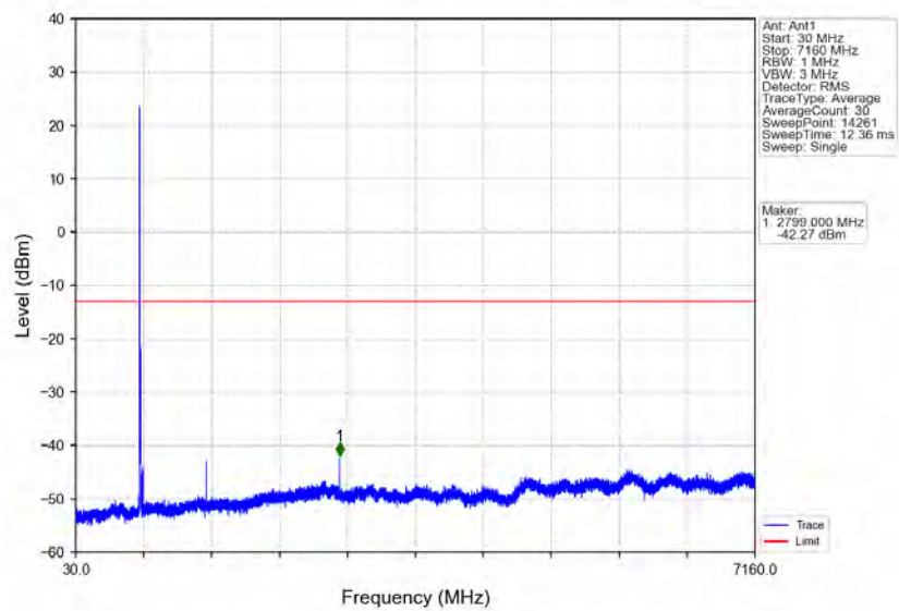
Band12_10MHz_QPSK_LCH_704MHz_RB_1_0_NTNV
