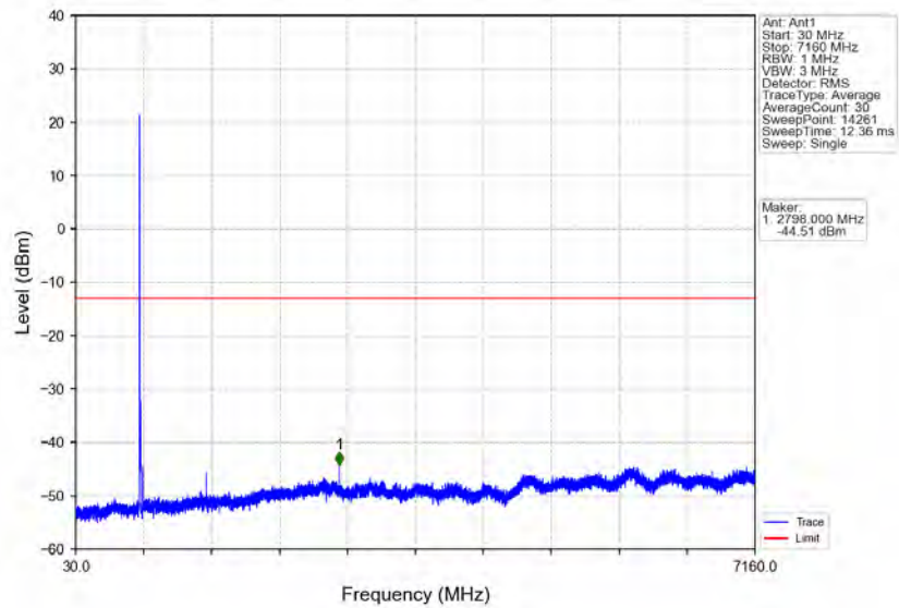
Band12_5MHz_16QAM_LCH_701.5MHz_RB_25_0_NTV
