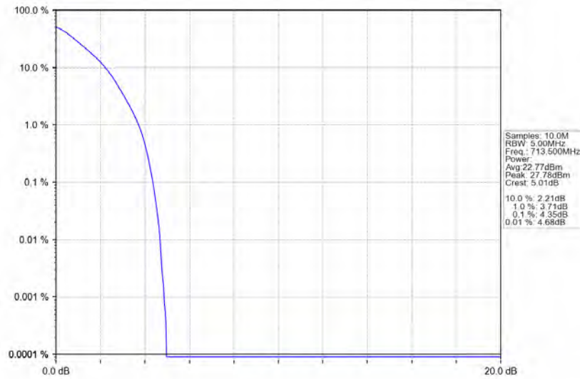
Band12_5MHz_QPSK_HCH_713.5MHz_RB_25_0_NTNV
