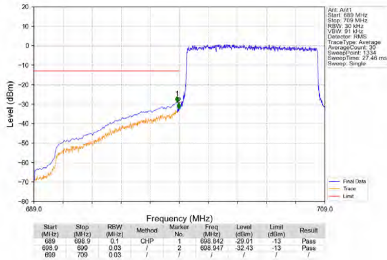
Band12_10MHz_QPSK_LCH_704MHz_RB_50_0_NTNV
