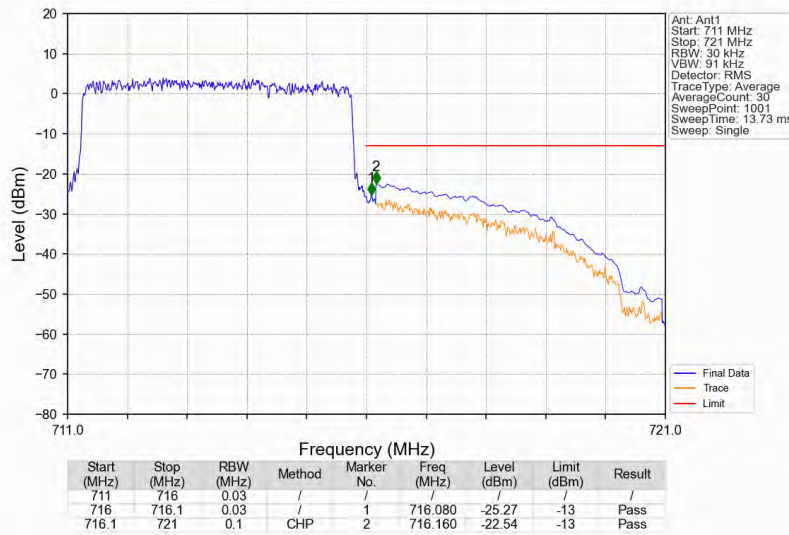
Band12_5MHz_QPSK_HCH_713.5MHz_RB_25_0_NTNV
