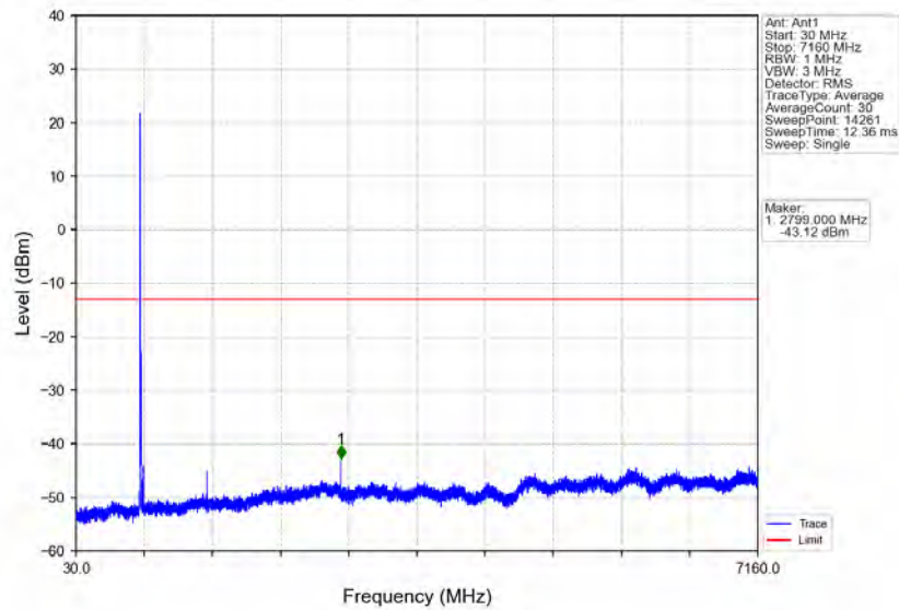
Band12_10MHz_16QAM_LCH_704MHz_RB_50_0_NTNV
