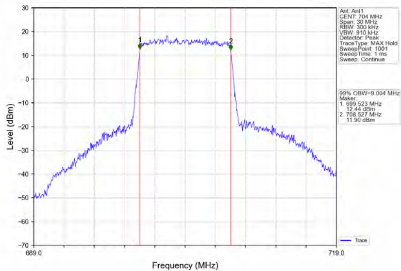
Band12_10MHz_64QAM_LCH_704MHz_RB_50_0_NTNV
