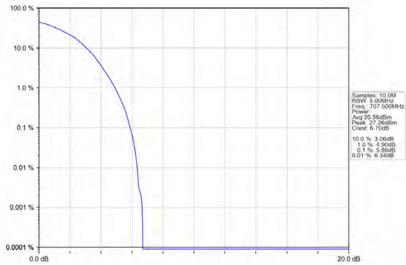
Band12_1.4MHz_64QAM_MCH_707.5MHz_RB_6_0_NTNV
