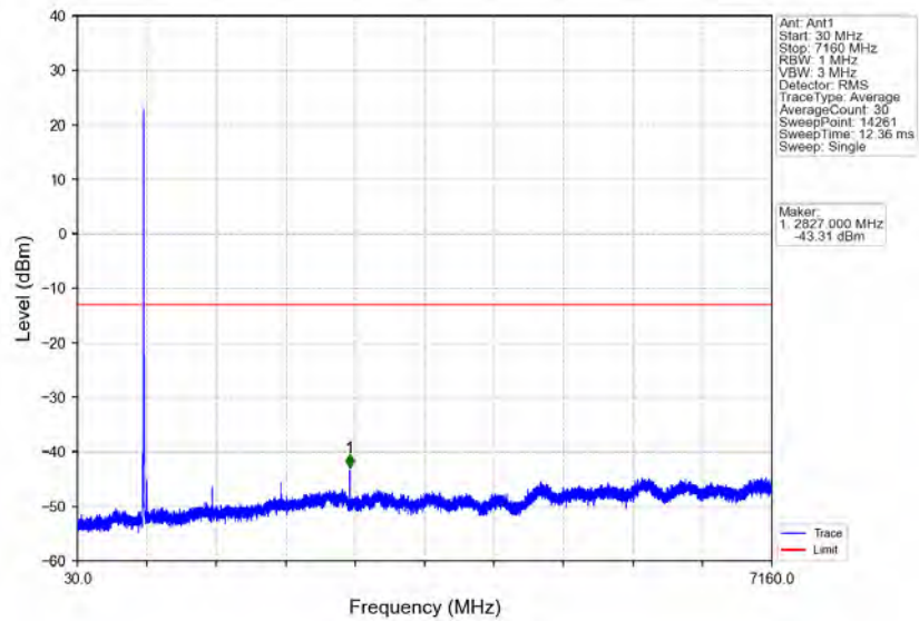
Band12_10MHz_QPSK_HCH_711MHz_RB_1_49_NTNV
