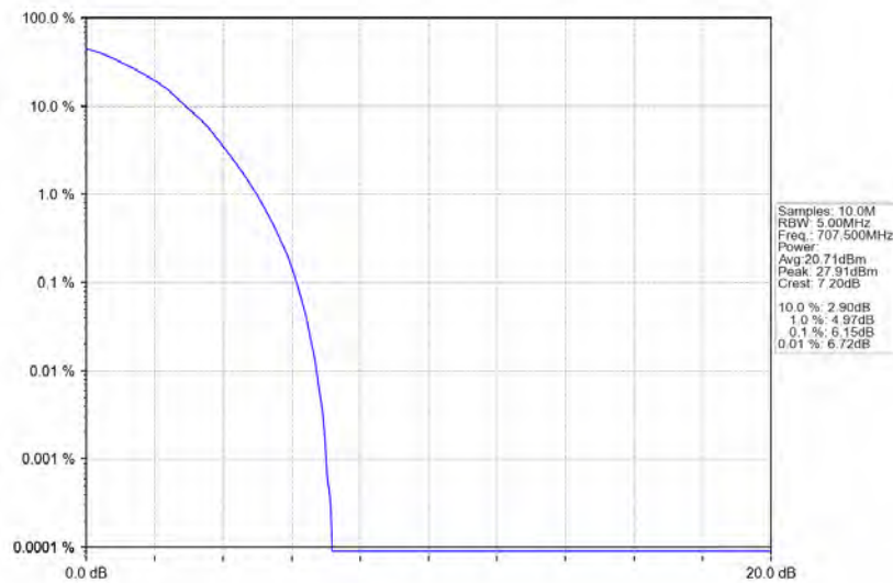
Band12_5MHz_64QAM_MCH_707.5MHz_RB_25_0_NTNV
