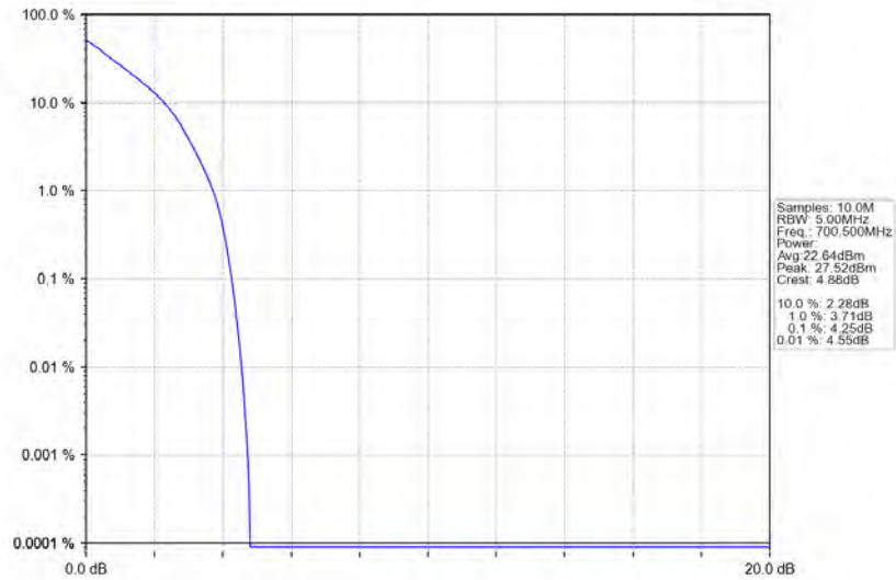
Band12_3MHz_QPSK_LCH_700.5MHz_RB_15_0_NTNV
