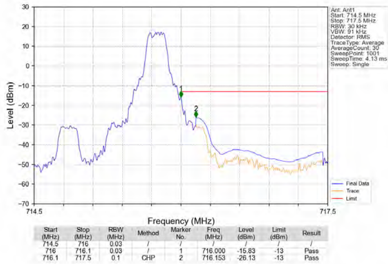
Band12_1.4MHz_16QAM_HCH_715.3MHz_RB_1_5_NTNV
