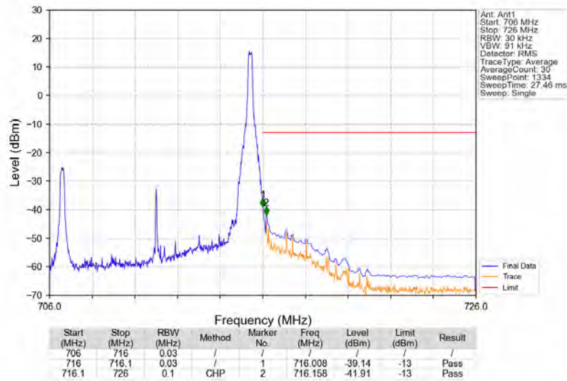
Band12_10MHz_64QAM_HCH_711MHz_RB_1_49_NTNV
