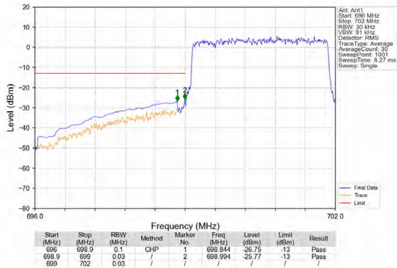
Band12_3MHz_16QAM_LCH_700.5MHz_RB_15_0_NTNV
