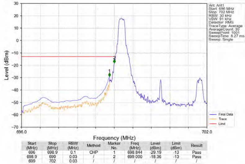
Band12_3MHz_QPSK_LCH_700.5MHz_RB_1_0_NTNV
