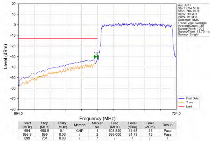
Band12_5MHz_64QAM_LCH_701.5MHz_RB_25_0_NTNV
