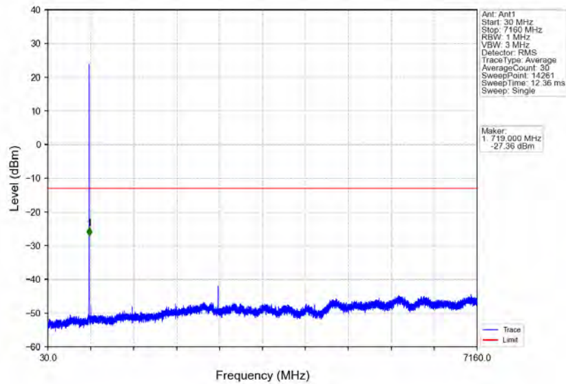
Band12_1.4MHz_QPSK_HCH_715.3MHz_RB_1_5_NTNV
