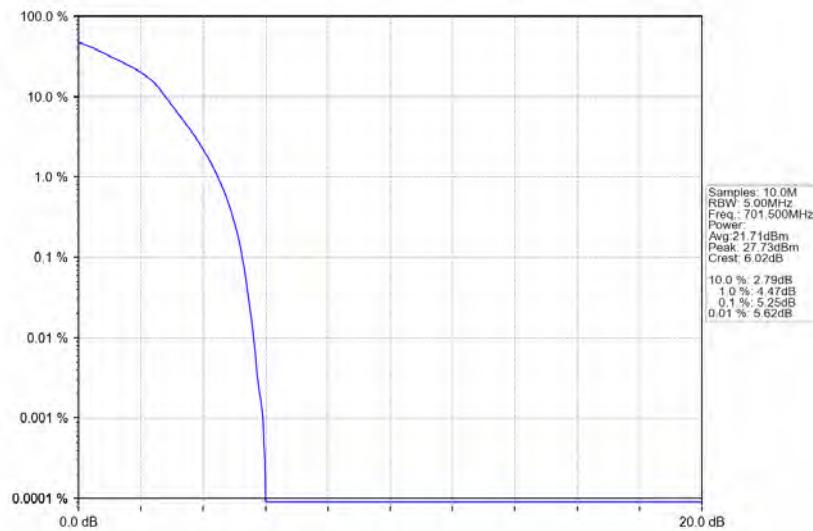
Band12_5MHz_16QAM_LCH_701.5MHz_RB_25_0_NTNV
