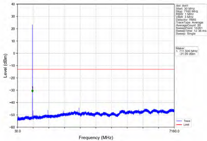
Band12_1.4MHz_QPSK_MCH_707.5MHz_RB_1_0_NTNV
