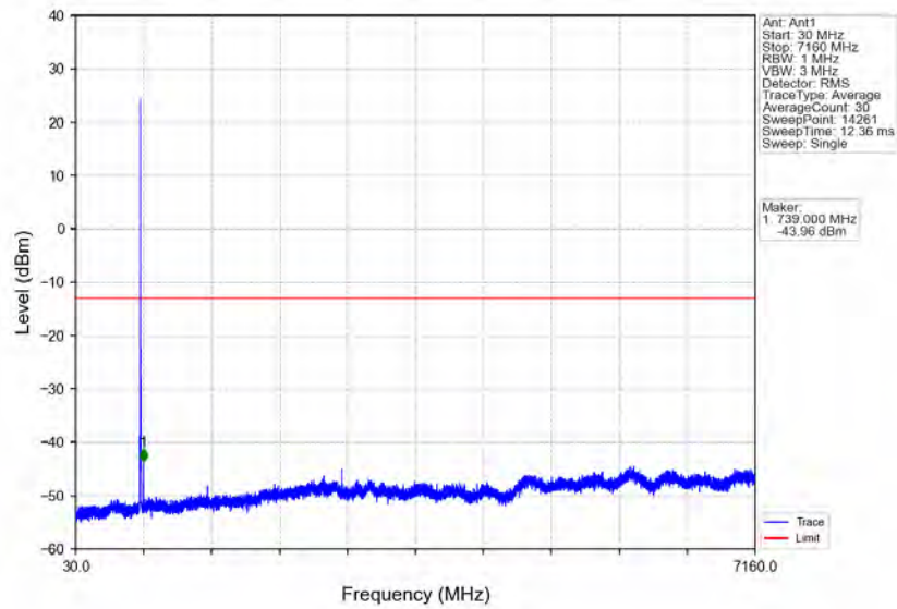
Band12_5MHz_QPSK_MCH_707.5MHz_RB_1_0_NTNV
