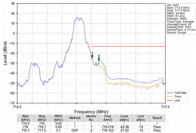
Band12_1.4MHz_64QAM_HCH_715.3MHz_RB_1_5_NTNV
