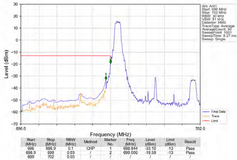
Band12_3MHz_64QAM_LCH_700.5MHz_RB_1_0_NTV
