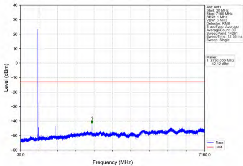
Band12_5MHz_QPSK_LCH_701.5MHz_RB_1_0_NTNV
