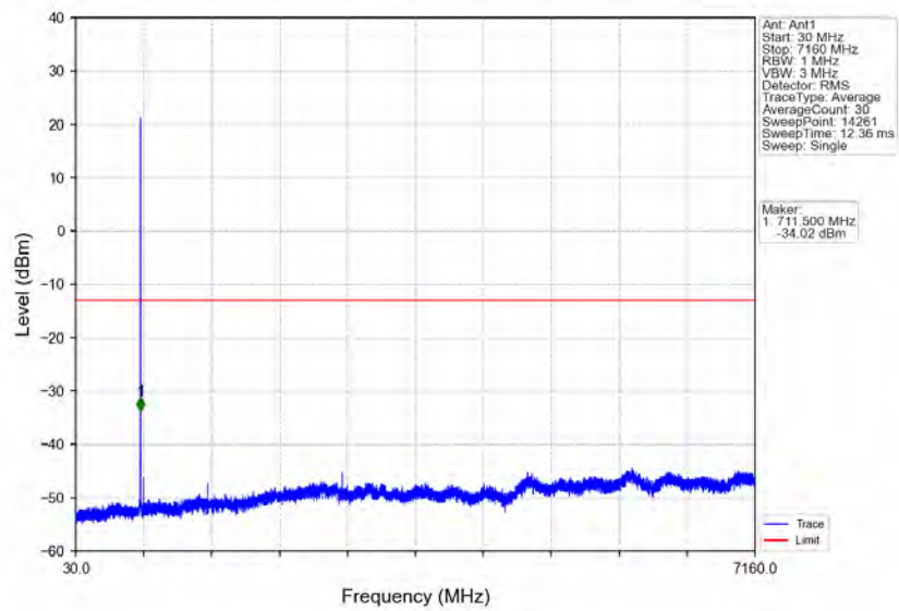
Band12_1.4MHz_64QAM_MCH_707.5MHz_RB_1_0_NTNV
