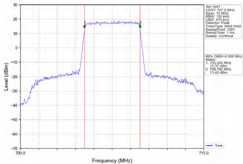
Band12_5MHz_QPSK_MCH_707.5MHz_RB_25_0_NTNV
