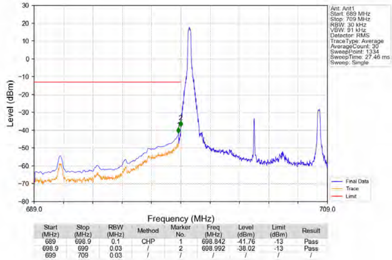
Band12_10MHz_QPSK_LCH_704MHz_RB_1_0_NTNV
