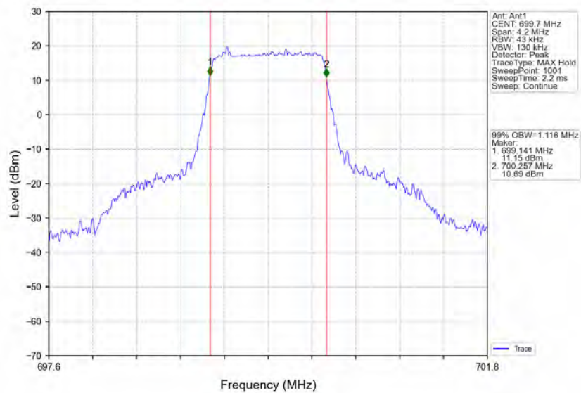
Band12_1.4MHz_16QAM_LCH_699.7MHz_RB_6_0_NTNV
