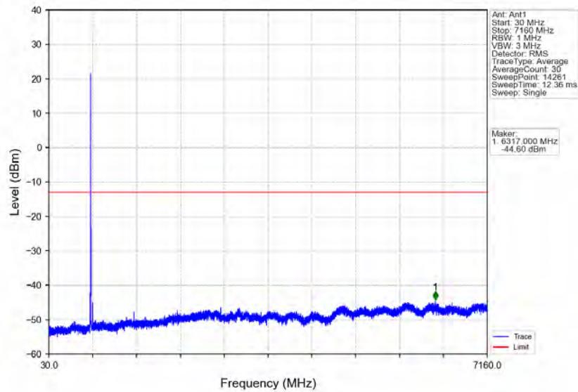
Band12_10MHz_64QAM_HCH_711MHz_RB_1_49_NTNV
