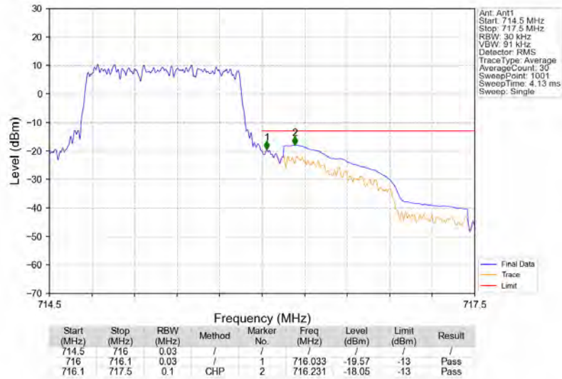
Band12_1.4MHz_QPSK_HCH_715.3MHz_RB_6_0_NTNV
