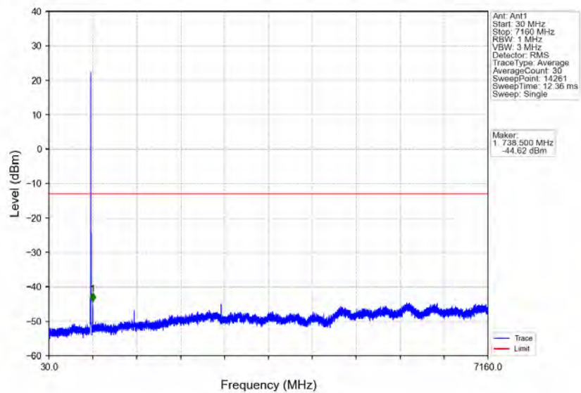
Band12_10MHz_16QAM_HCH_711MHz_RB_1_0_NTNV
