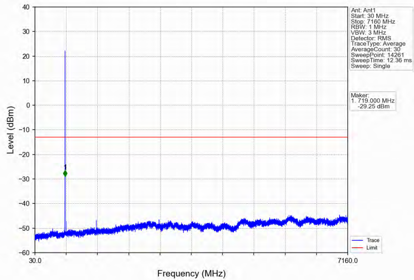
Band12_1.4MHz_64QAM_HCH_715.3MHz_RB_1_5_NTNV
