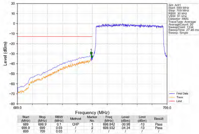
Band12_10MHz_16QAM_LCH_704MHz_RB_50_0_NTNV
