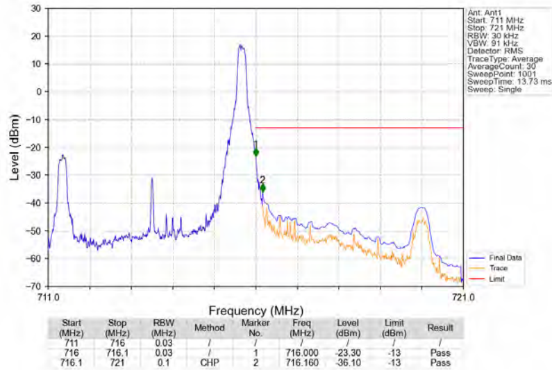
Band12_5MHz_16QAM_HCH_713.5MHz_RB_1_24_NTNV
