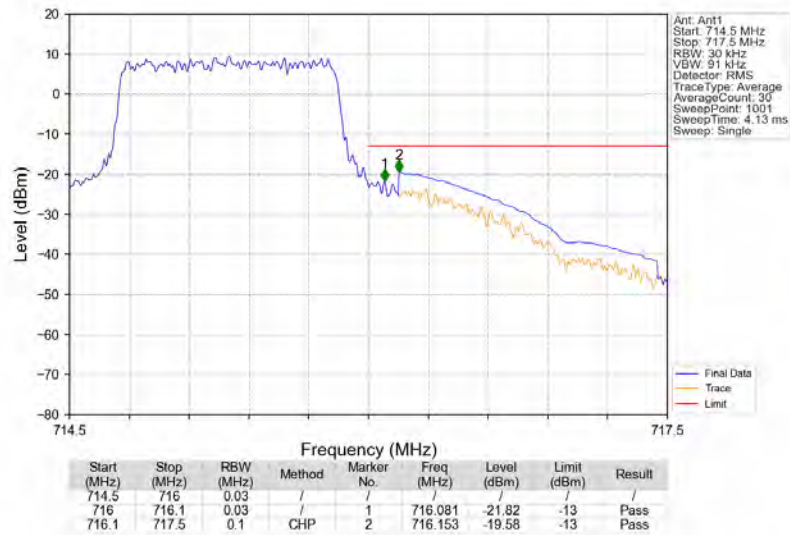
Band12_1.4MHz_16QAM_HCH_715.3MHz_RB_6_0_NTNV
