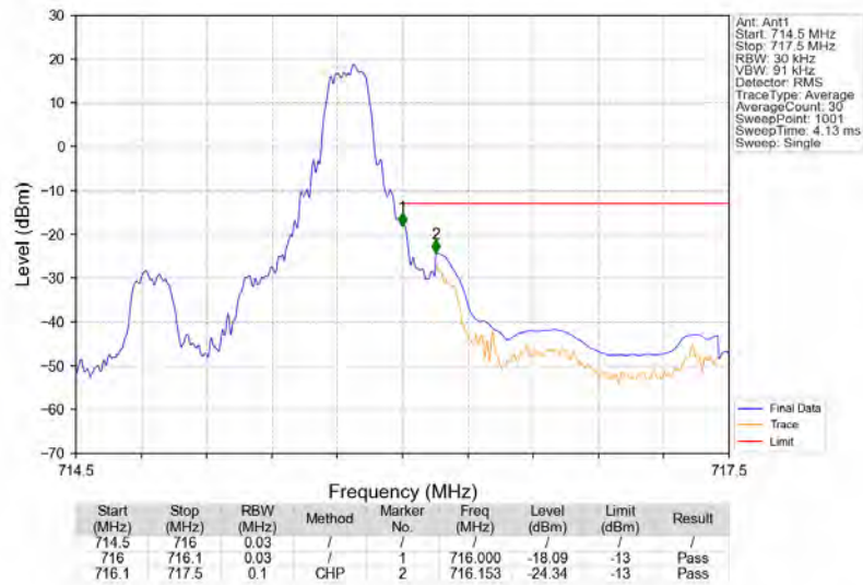
Band12_1.4MHz_QPSK_HCH_715.3MHz_RB_1_5_NTNV
