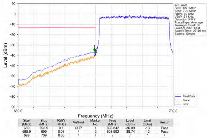
Band12_10MHz_64QAM_LCH_704MHz_RB_50_0_NTNV
