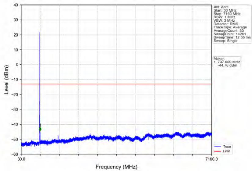
Band12_5MHz_64QAM_MCH_707.5MHz_RB_1_0_NTNV
