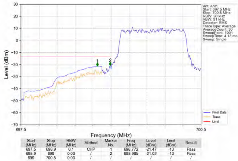
Band12_1.4MHz_QPSK_LCH_699.7MHz_RB_6_0_NTNV
