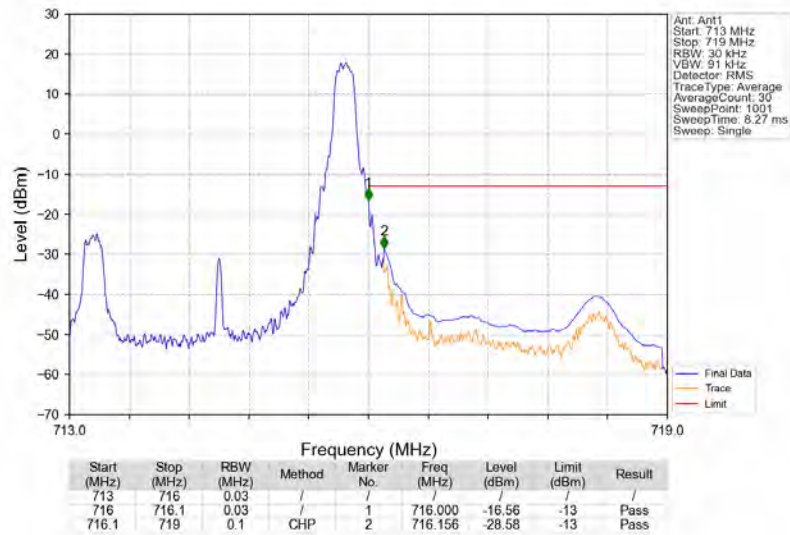
Band12_3MHz_QPSK_HCH_714.5MHz_RB_1_14_NTNV
