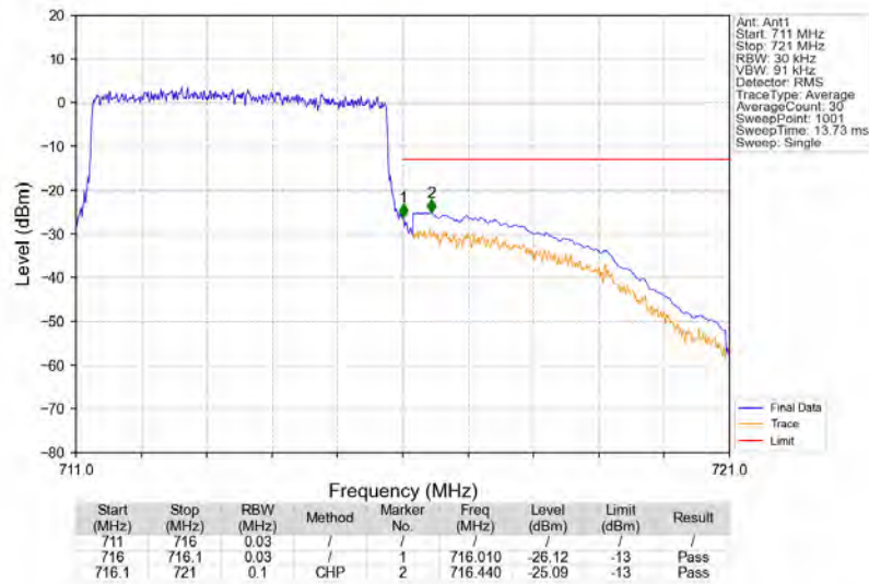
Band12_5MHz_16QAM_HCH_713.5MHz_RB_25_0_NTNV
