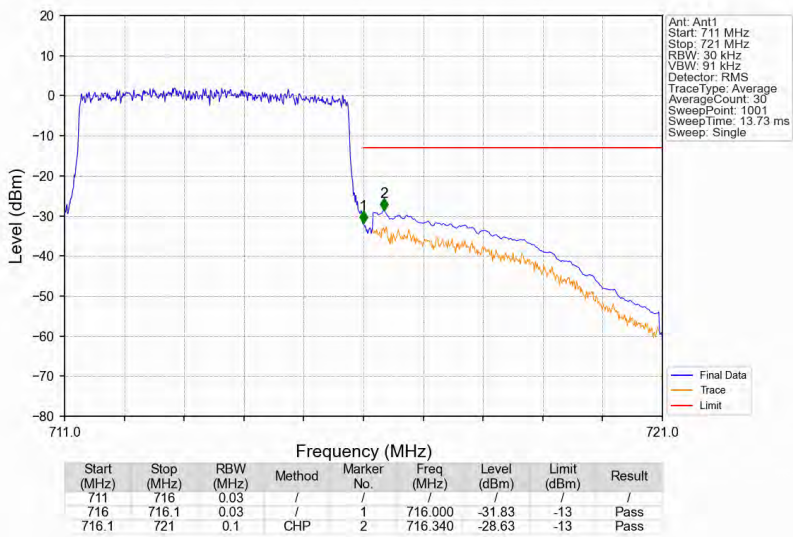
Band12_5MHz_64QAM_HCH_713.5MHz_RB_25_0_NTNV
