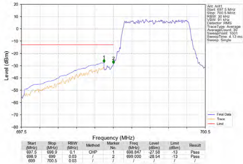
Band12_1.4MHz_64QAM_LCH_699.7MHz_RB_6_0_NTNV
