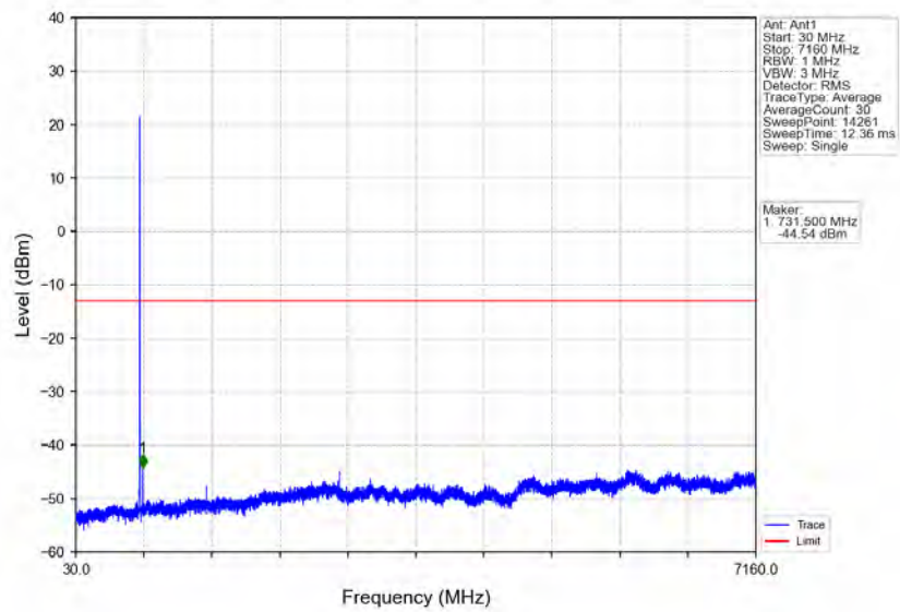
Band12_3MHz_64QAM_LCH_700.5MHz_RB_1_0_NTV
