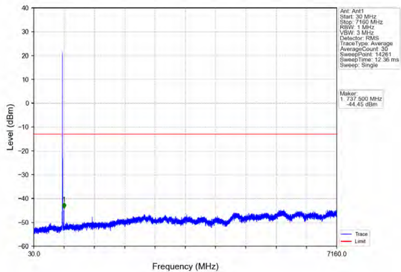
Band12_10MHz_64QAM_MCH_707.5MHz_RB_1_0_NTNV
