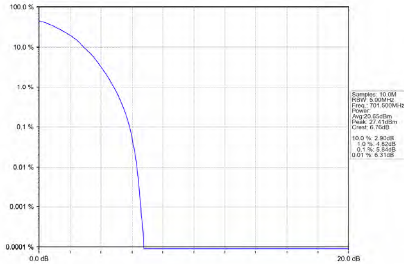
Band12_5MHz_64QAM_LCH_701.5MHz_RB_25_0_NTNV
