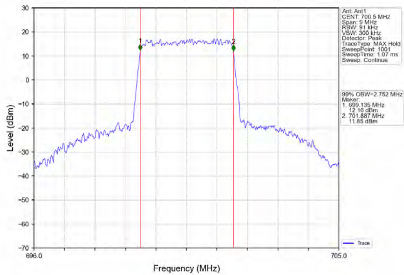
Band12_3MHz_64QAM_LCH_700.5MHz_RB_15_0_NTNV
