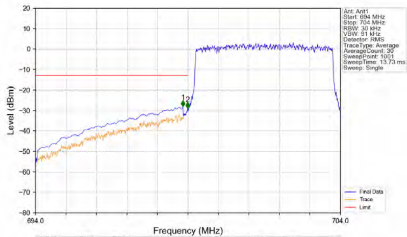
Band12_5MHz_16QAM_LCH_701.5MHz_RB_25_0_NTV
