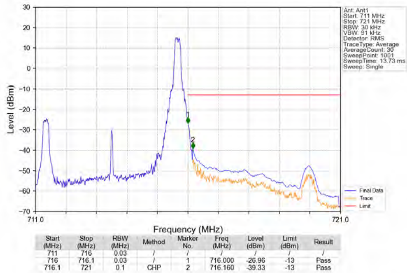
Band12_5MHz_64QAM_HCH_713.5MHz_RB_1_24_NTNV
