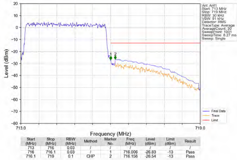
Band12_3MHz_64QAM_HCH_714.5MHz_RB_15_0_NTNV
