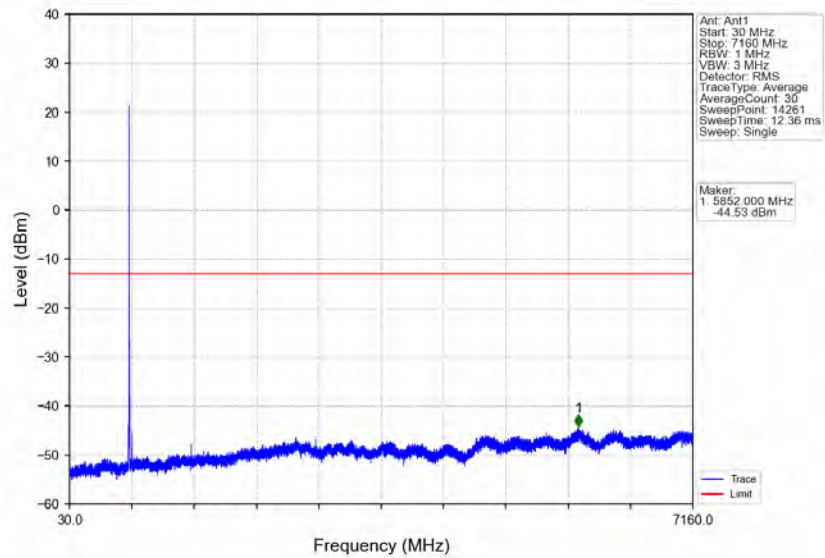
Band12_5MHz_64QAM_HCH_713.5MHz_RB_1_24_NTNV
