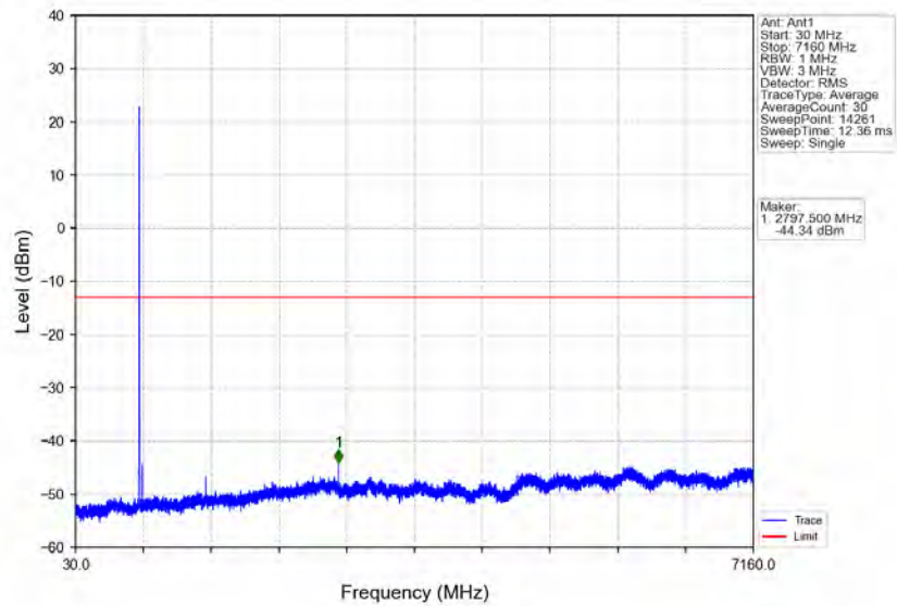
Band12_3MHz_16QAM_LCH_700.5MHz_RB_15_0_NTNV
