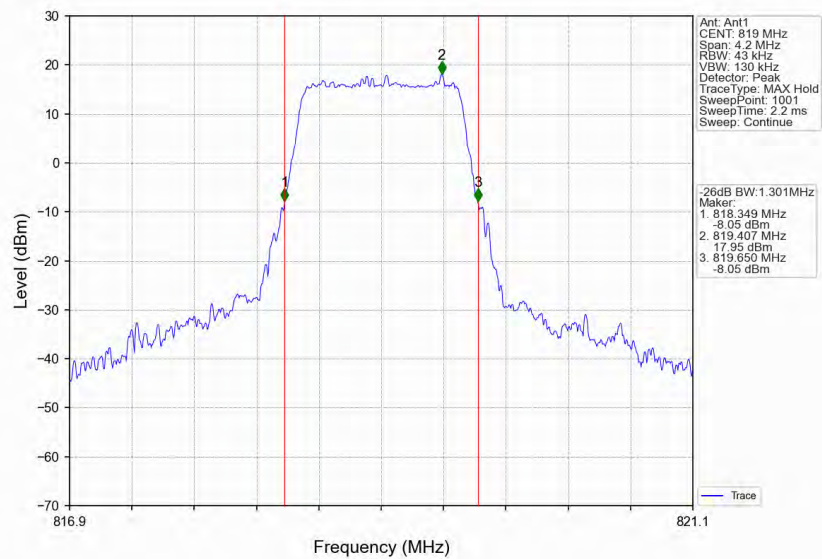
Band26a_1.4MHz_64QAM_MCH_819MHz_RB_6_0_NTNV
