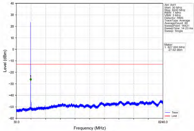
Band26a_1.4MHz_QPSK_HCH_823.3MHz_RB_1_5_NTNV
