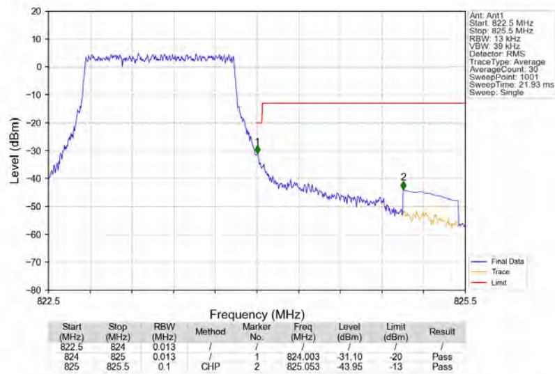
Band26a_1.4MHz_16QAM_HCH_823.3MHz_RB_6_0_NTNV
