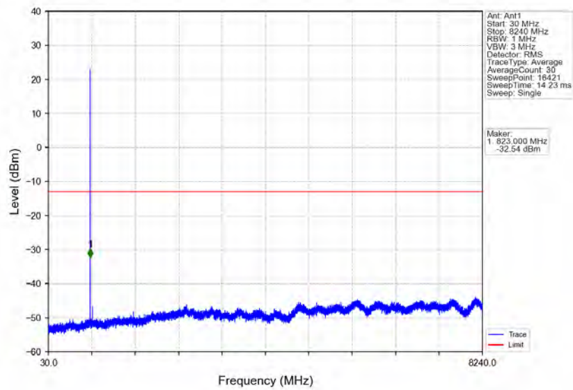
Band26a_1.4MHz_QPSK_MCH_819MHz_RB_1_0_NTNV
