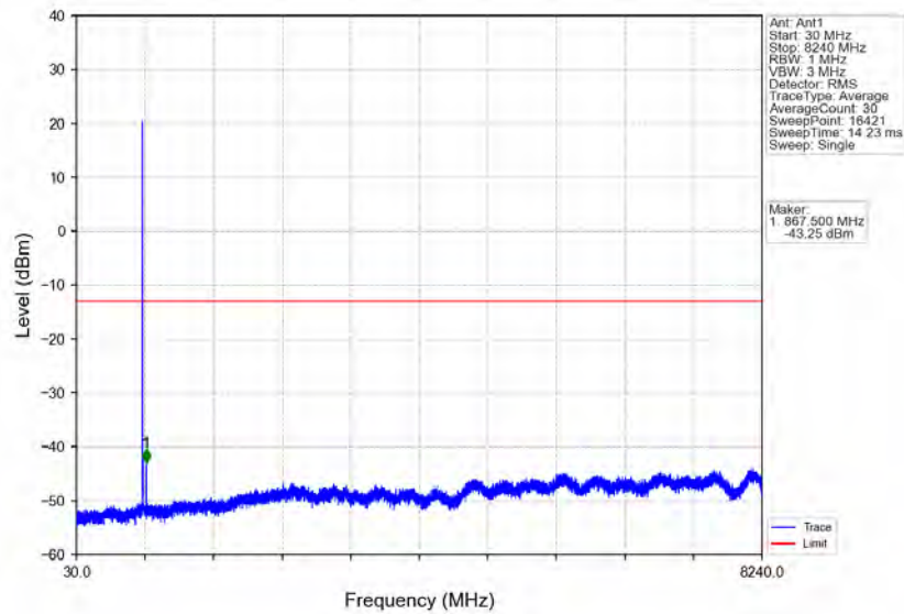
Band26a_5MHz_64QAM_HCH_821.5MHz_RB_1_24_NTNV
