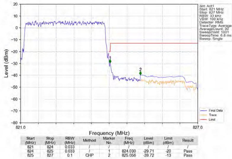
Band26a_3MHz_QPSK_HCH_822.5MHz_RB_15_0_NTNV
