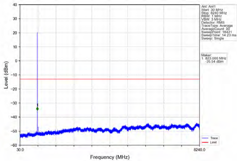
Band26a_1.4MHz_64QAM_MCH_819MHz_RB_1_0_NTNV
