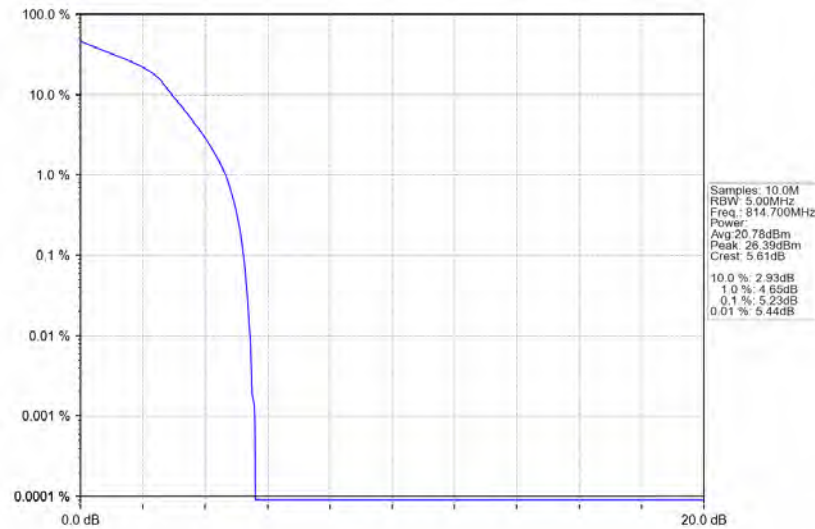
Band26a_1.4MHz_16QAM_LCH_814.7MHz_RB_6_0_NTNV
