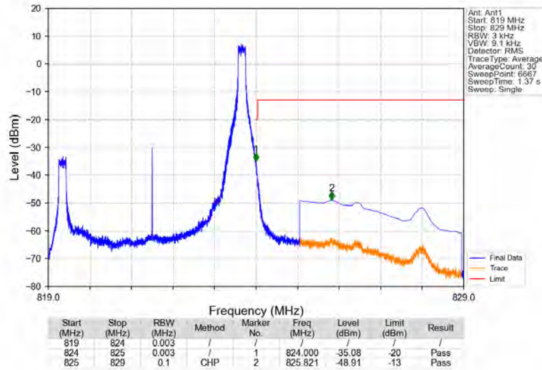
Band26a_5MHz_16QAM_HCH_821.5MHz_RB_1_24_NTNV
