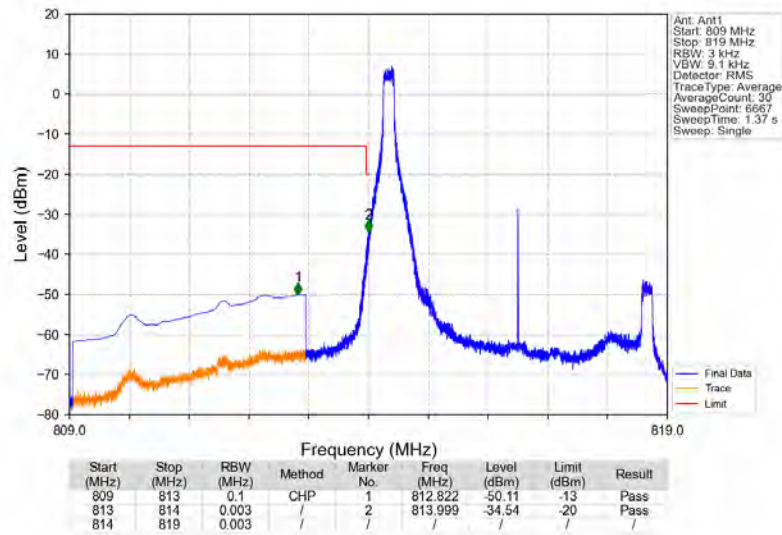
Band26a_5MHz_16QAM_LCH_816.5MHz_RB_1_0_NTNV
