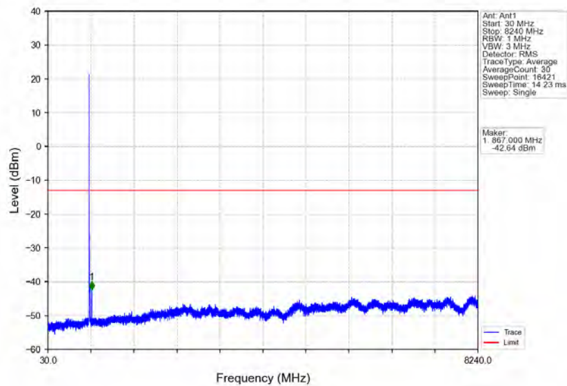
Band26a_10MHz_16QAM_MCH_819MHz_RB_1_0_NTNV
