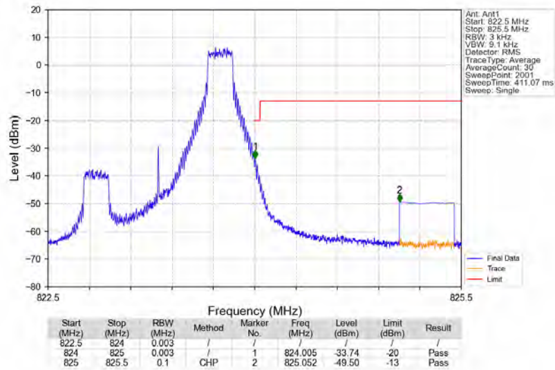
Band26a_1.4MHz_64QAM_HCH_823.3MHz_RB_1_5_NTNV
