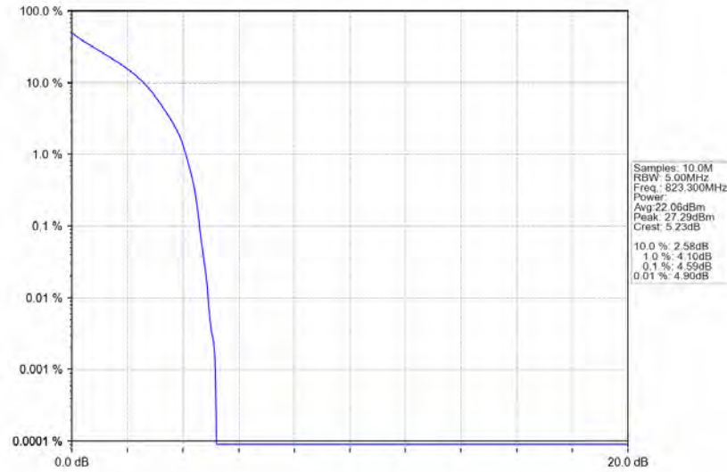
Band26a_1.4MHz_QPSK_HCH_823.3MHz_RB_6_0_NTNV
