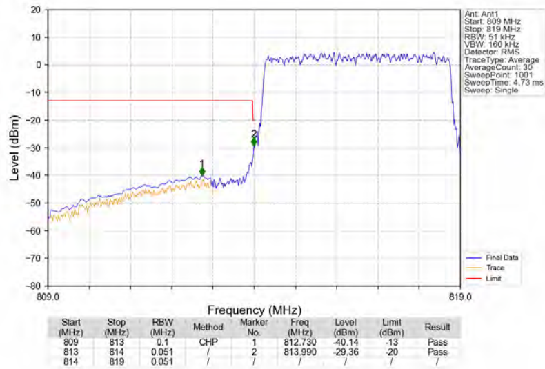
Band26a_5MHz_16QAM_LCH_816.5MHz_RB_25_0_NTNV
