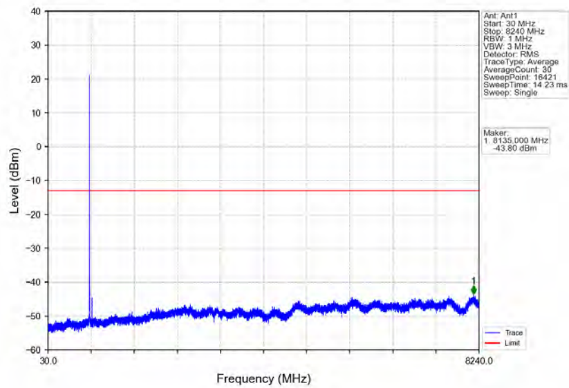
Band26a_5MHz_64QAM_MCH_819MHz_RB_1_0_NTNV
