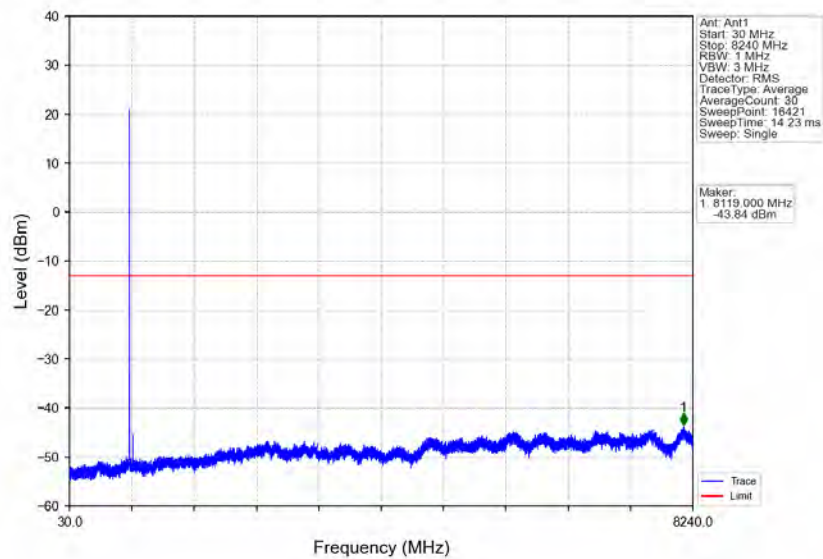
Band26a_3MHz_64QAM_MCH_819MHz_RB_1_0_NTNV
