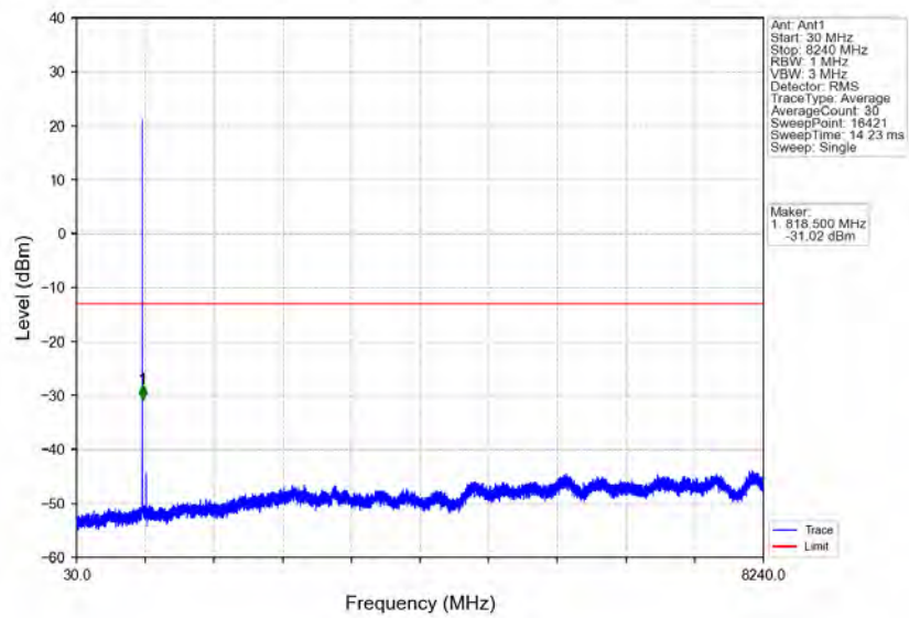
Band26a_1.4MHz_64QAM_LCH_814.7MHz_RB_1_0_NTNV
