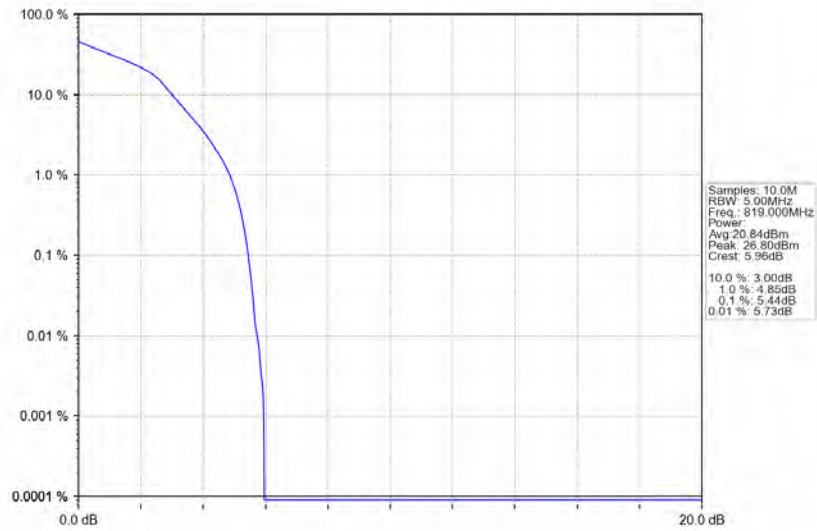
Band26a_1.4MHz_16QAM_MCH_819MHz_RB_6_0_NTNV
