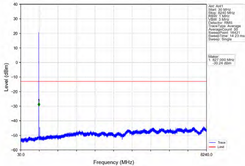
Band26a_1.4MHz_64QAM_HCH_823.3MHz_RB_1_5_NTNV
