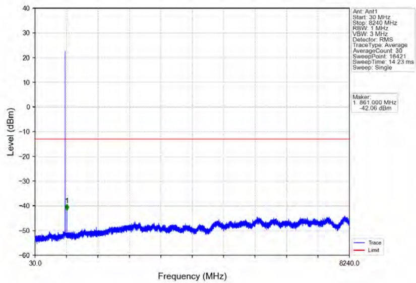
Band26a_3MHz_64QAM_LCH_815.5MHz_RB_1_0_NTNV
