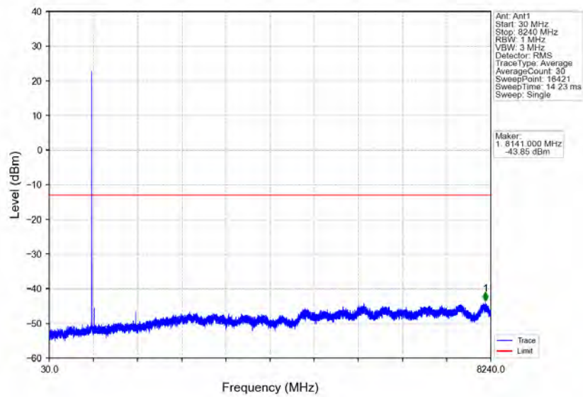
Band26a_3MHz_QPSK_MCH_819MHz_RB_1_0_NTNV
