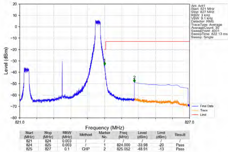
Band26a_3MHz_64QAM_HCH_822.5MHz_RB_1_14_NTNV
