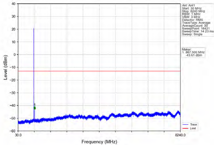
Band26a_3MHz_64QAM_HCH_822.5MHz_RB_1_14_NTNV
