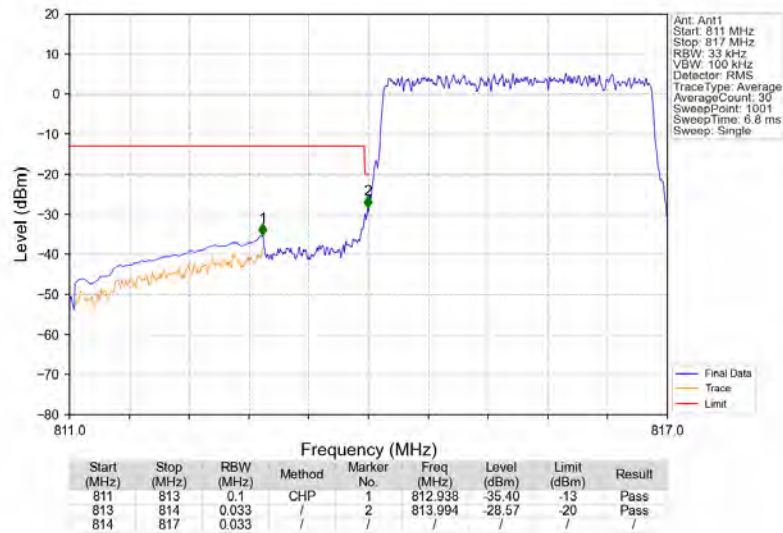
Band26a_3MHz_16QAM_LCH_815.5MHz_RB_15_0_NTNV
