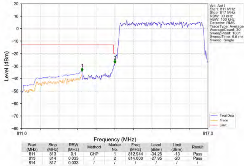
Band26a_3MHz_QPSK_LCH_815.5MHz_RB_15_0_NTNV
