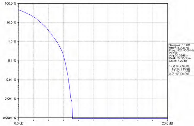
Band26a_5MHz_64QAM_HCH_821.5MHz_RB_25_0_NTNV
