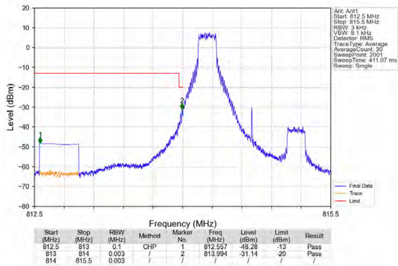
Band26a_1.4MHz_16QAM_LCH_814.7MHz_RB_1_0_NTNV
