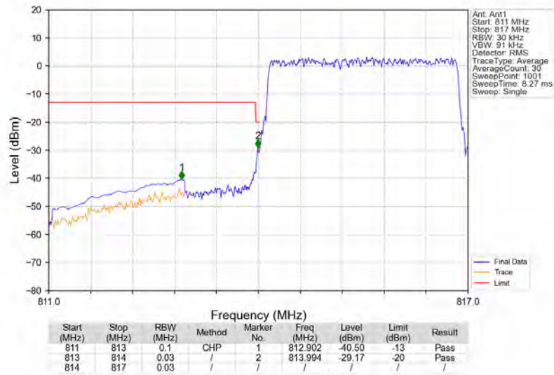
Band26a_3MHz_64QAM_LCH_815.5MHz_RB_15_0_NTNV
