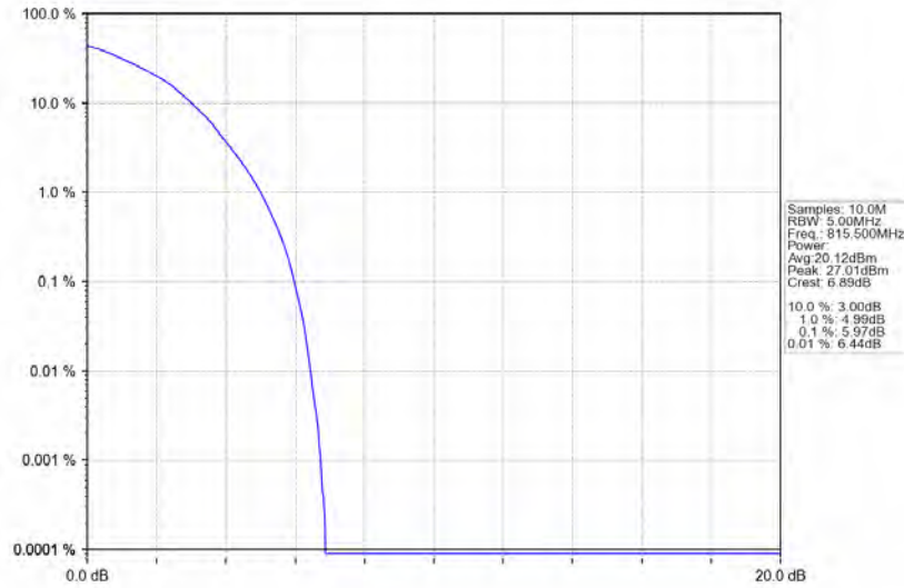
Band26a_3MHz_64QAM_LCH_815.5MHz_RB_15_0_NTNV
