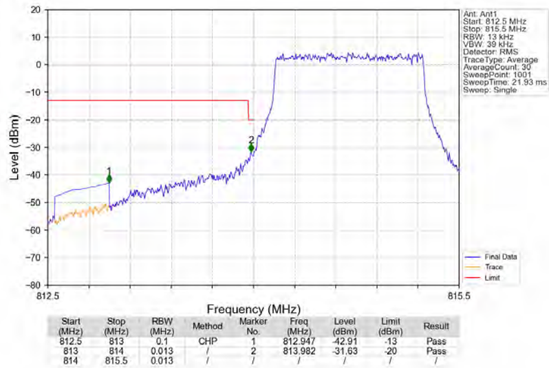
Band26a_1.4MHz_16QAM_LCH_814.7MHz_RB_6_0_NTNV
