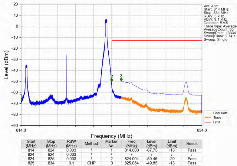
Band26a_10MHz_64QAM_MCH_819MHz_RB_50_0_NTNV
