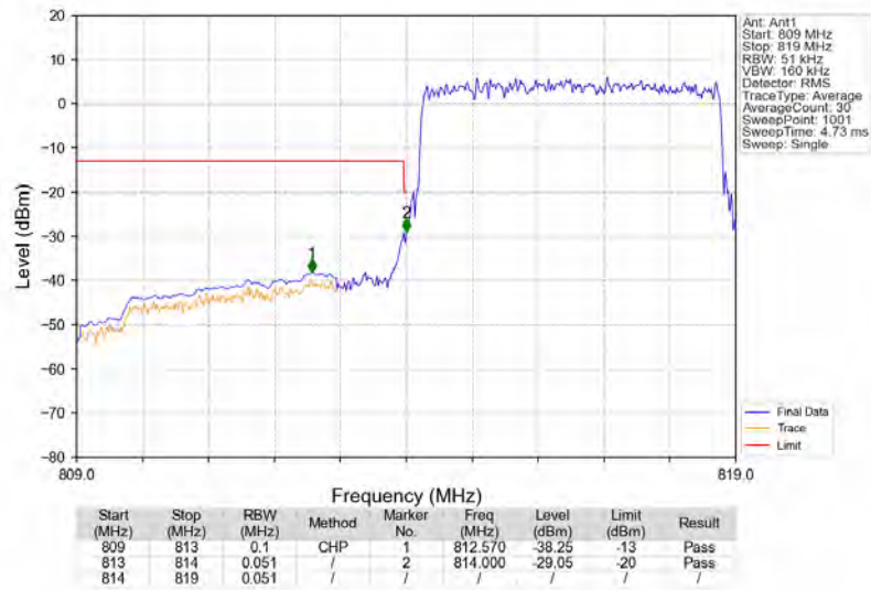
Band26a_5MHz_QPSK_LCH_816.5MHz_RB_25_0_NTNV
