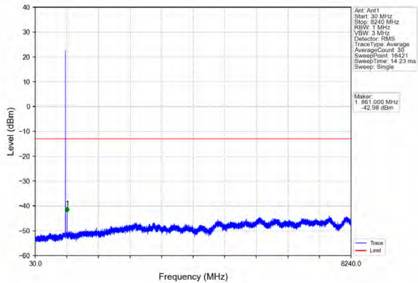
Band26a_3MHz_16QAM_LCH_815.5MHz_RB_15_0_NTNV
