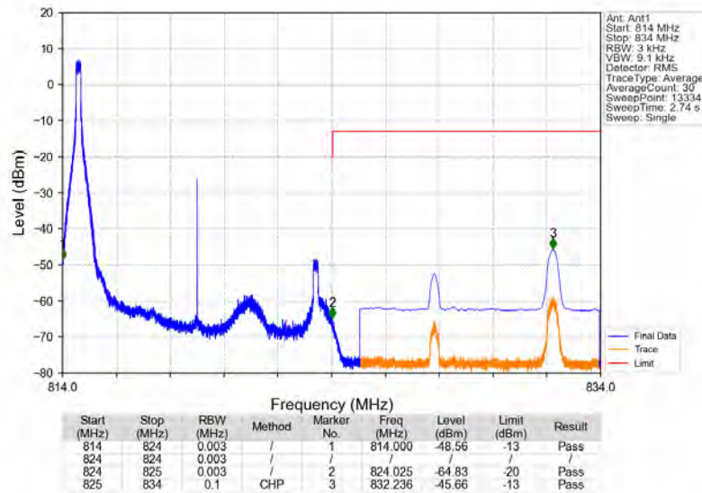
Band26a_10MHz_16QAM_MCH_819MHz_RB_1_0_NTNV
