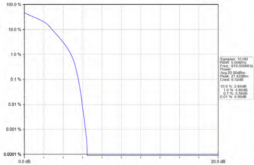
Band26a_5MHz_16QAM_MCH_819MHz_RB_25_0_NTNV
