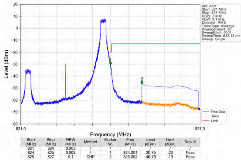
Band26a_3MHz_QPSK_HCH_822.5MHz_RB_1_14_NTNV
