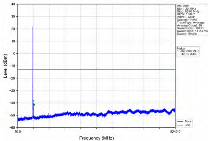
Band26a_10MHz_64QAM_MCH_819MHz_RB_1_0_NTNV
