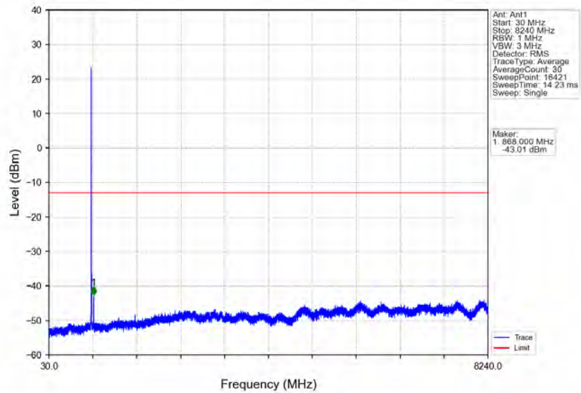
Band26a_5MHz_QPSK_HCH_821.5MHz_RB_1_24_NTNV
