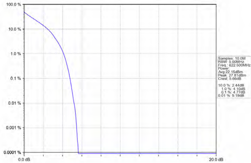
Band26a_3MHz_QPSK_HCH_822.5MHz_RB_15_0_NTNV
