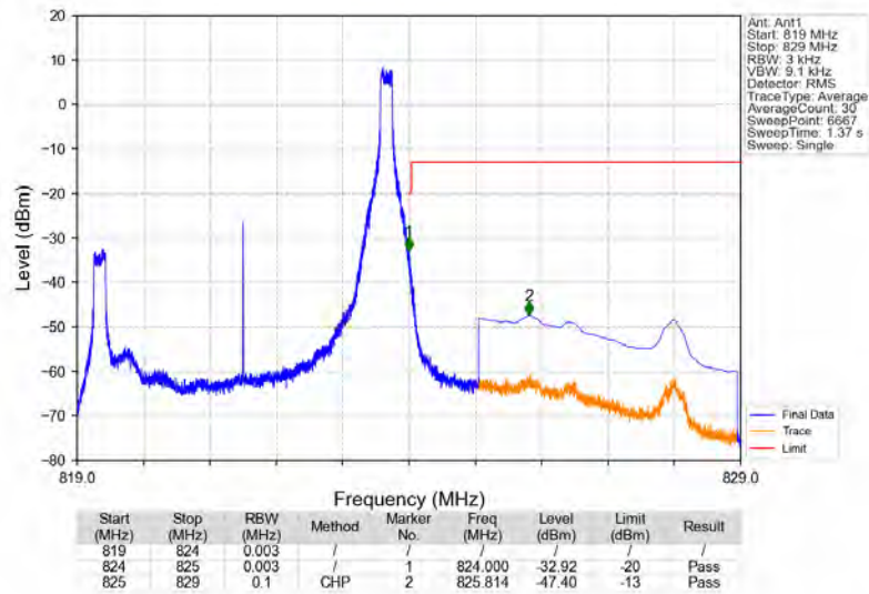
Band26a_5MHz_QPSK_HCH_821.5MHz_RB_1_24_NTNV
