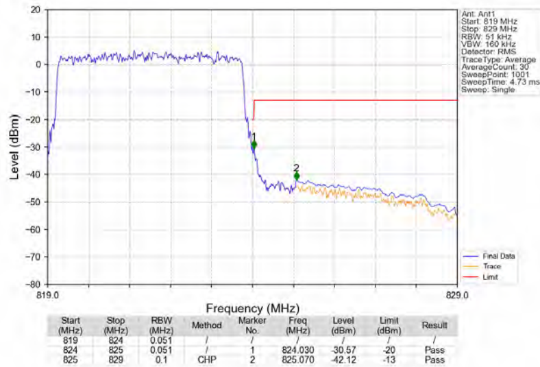
Band26a_5MHz_16QAM_HCH_821.5MHz_RB_25_0_NTNV
