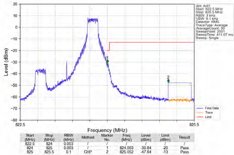
Band26a_1.4MHz_QPSK_HCH_823.3MHz_RB_1_5_NTNV
