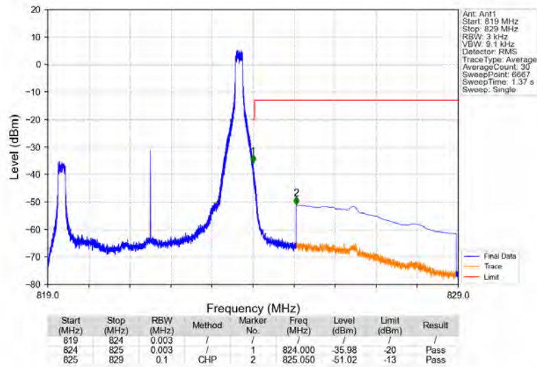
Band26a_5MHz_64QAM_HCH_821.5MHz_RB_1_24_NTNV
