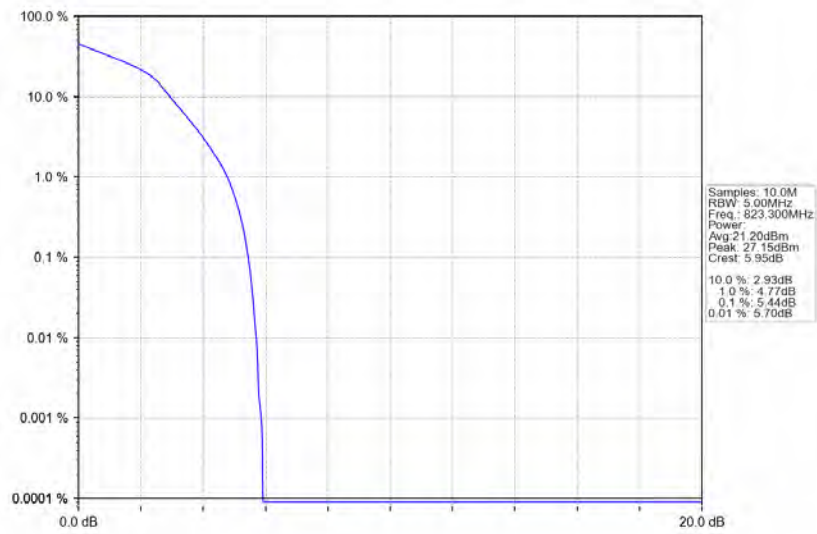
Band26a_1.4MHz_16QAM_HCH_823.3MHz_RB_6_0_NTNV
