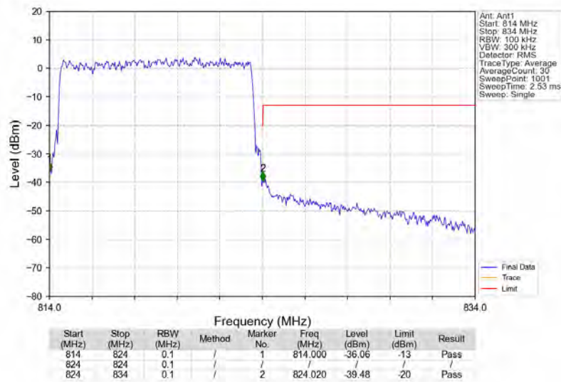
Band26a_10MHz_64QAM_MCH_819MHz_RB_50_0_NTNV
