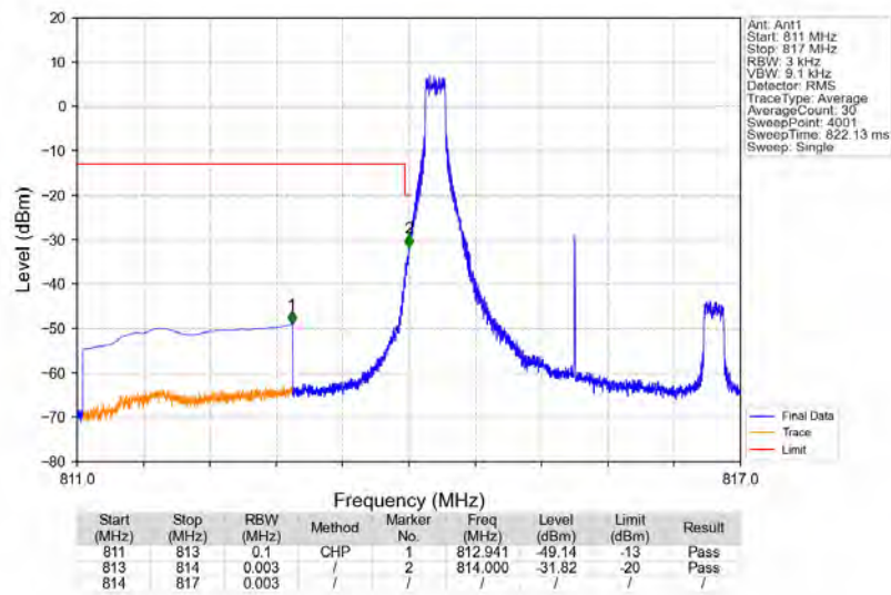
Band26a_3MHz_16QAM_LCH_815.5MHz_RB_1_0_NTNV
