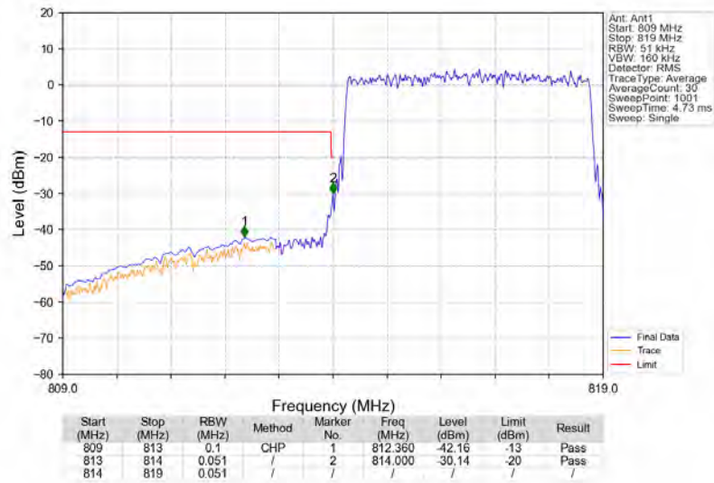
Band26a_5MHz_64QAM_LCH_816.5MHz_RB_25_0_NTNV
