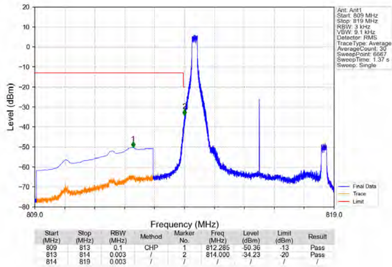
Band26a_5MHz_64QAM_LCH_816.5MHz_RB_1_0_NTNV
