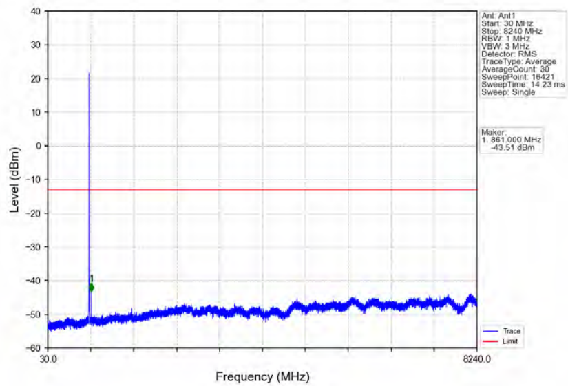
Band26a_5MHz_64QAM_LCH_816.5MHz_RB_1_0_NTNV
