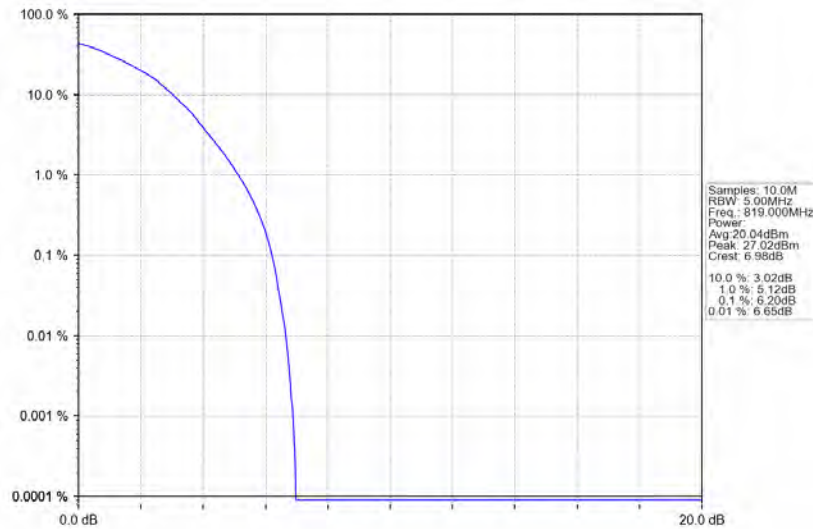
Band26a_3MHz_64QAM_MCH_819MHz_RB_15_0_NTNV
