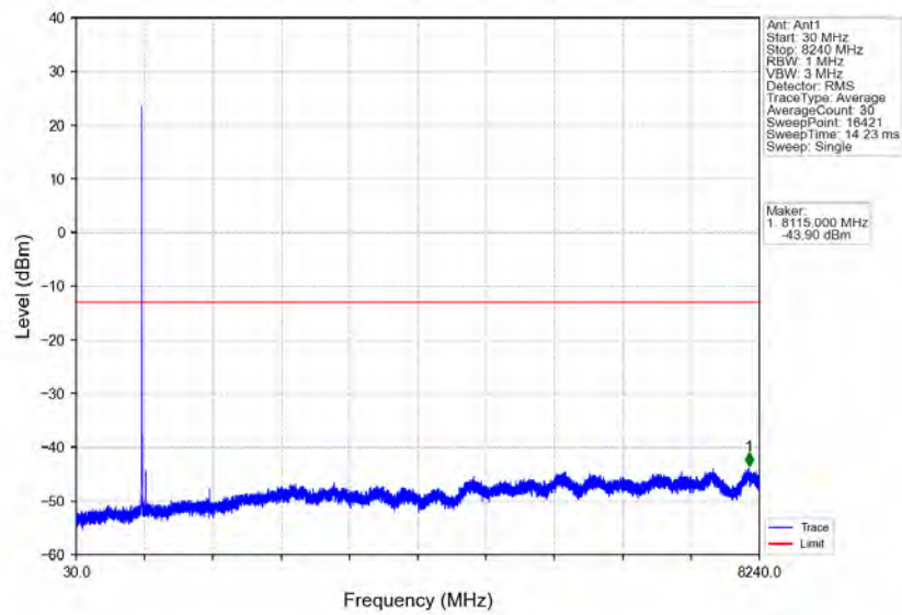
Band26a_5MHz_QPSK_MCH_819MHz_RB_1_0_NTNV
