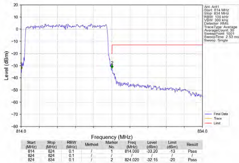
Band26a_10MHz_16QAM_MCH_819MHz_RB_50_0_NTNV
