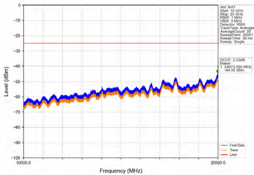
Band38_15MHz_64QAM_HCH_2612.5MHz_RB_1_0_NTNV
