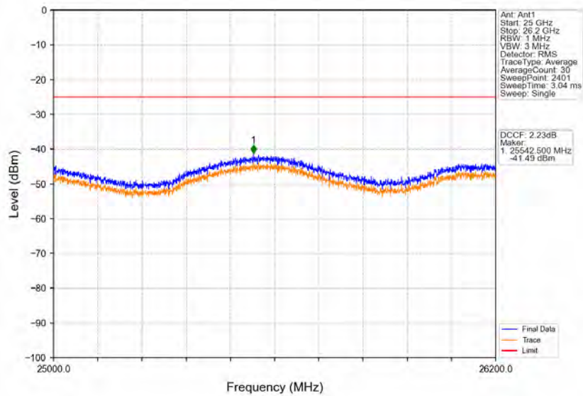
Band38_10MHz_64QAM_HCH_2615MHz_RB_1_49_NTNV
