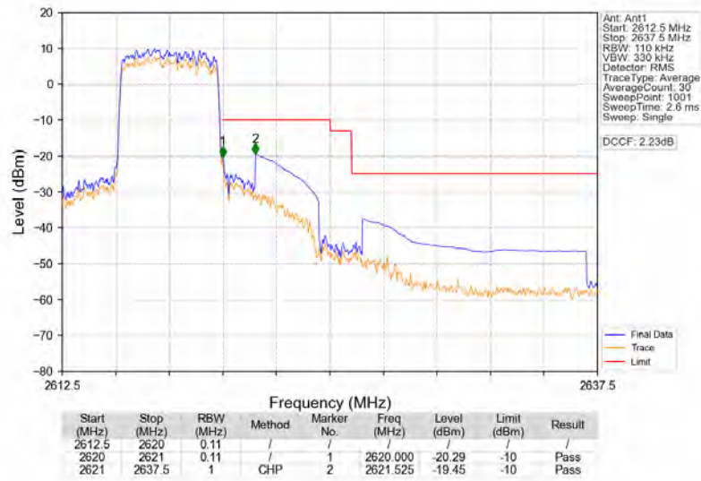
Band38_5MHz_QPSK_HCH_2617.5MHz_RB_25_0_NTNV
