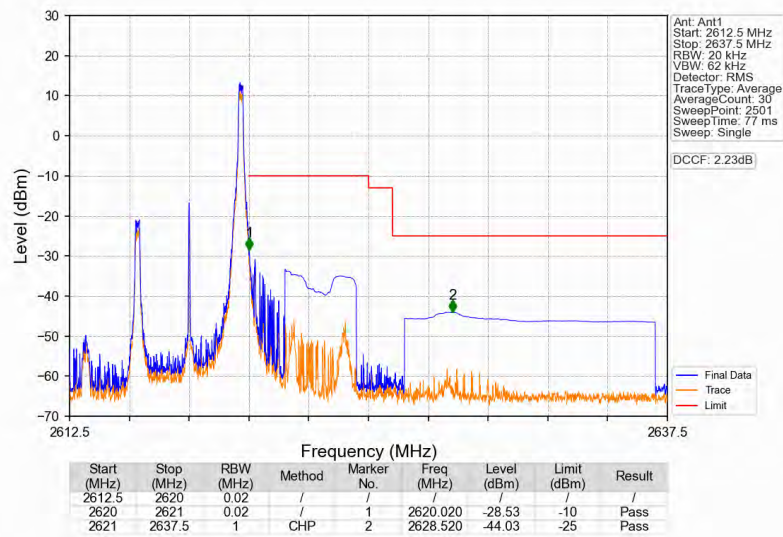
Band38_5MHz_64QAM_HCH_2617.5MHz_RB_1_24_NTNV
