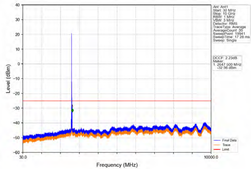
Band38_10MHz_16QAM_HCH_2615MHz_RB_1_0_NTNV
