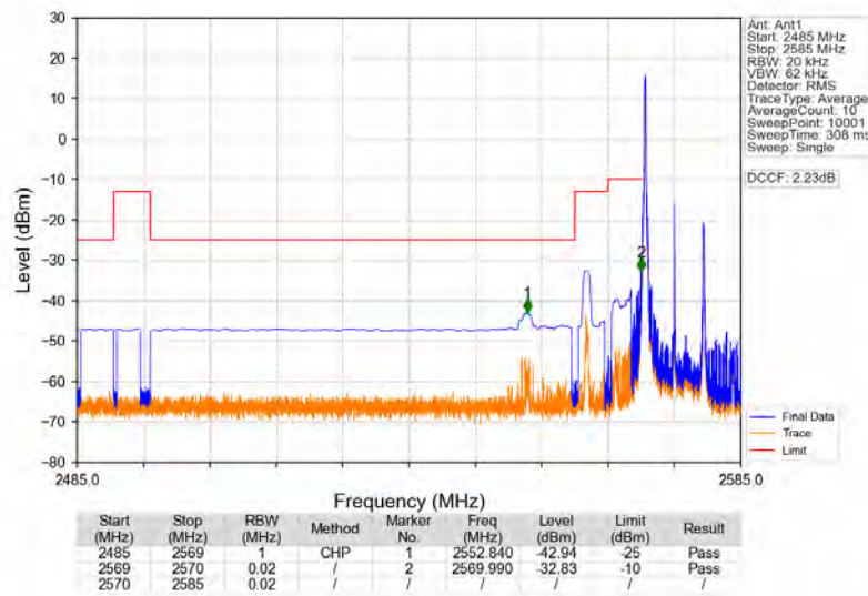
Band38_10MHz_16QAM_LCH_2575MHz_RB_1_0_NTNV
