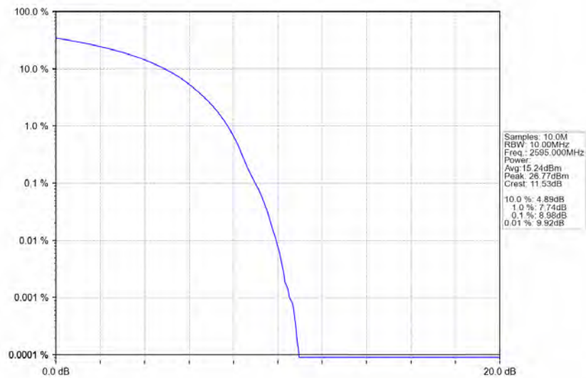
Band38_20MHz_64QAM_MCH_2595MHz_RB_100_0_NTNV
