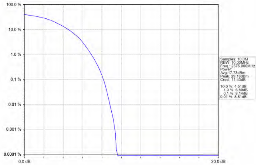
Band38_10MHz_64QAM_LCH_2575MHz_RB_50_0_NTNV
