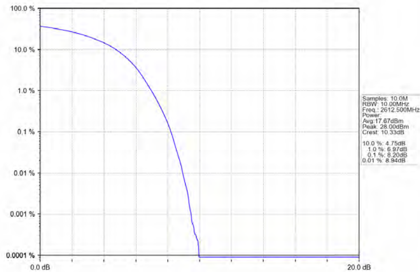
Band38_15MHz_16QAM_HCH_2612.5MHz_RB_75_0_NTNV
