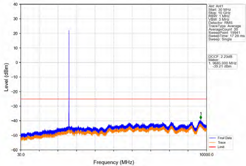
Band38_5MHz_QPSK_HCH_2617.5MHz_RB_1_0_NTNV
