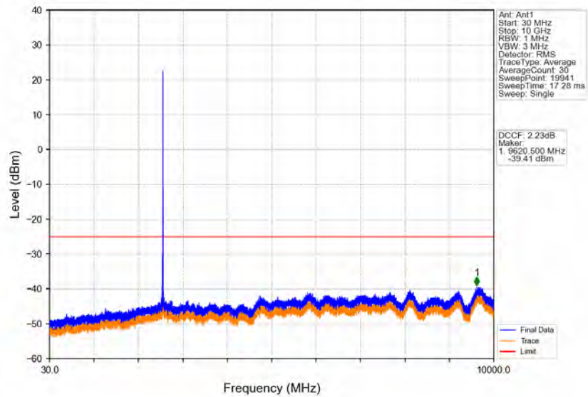
Band38_10MHz_16QAM_LCH_2575MHz_RB_1_0_NTNV
