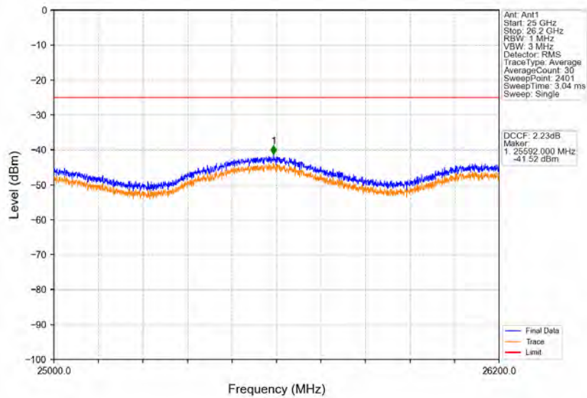
Band38_15MHz_QPSK_HCH_2612.5MHz_RB_1_74_NTNV
