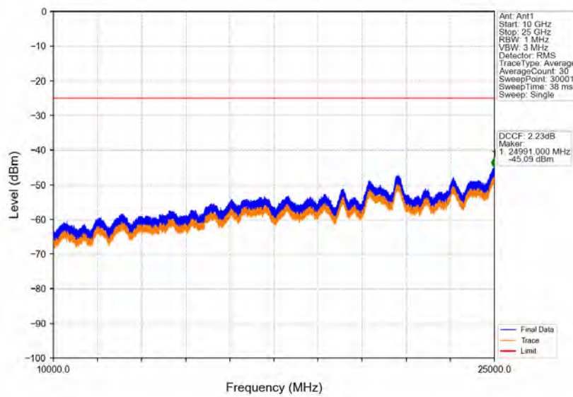
Band38_5MHz_16QAM_MCH_2595MHz_RB_1_0_NTNV
