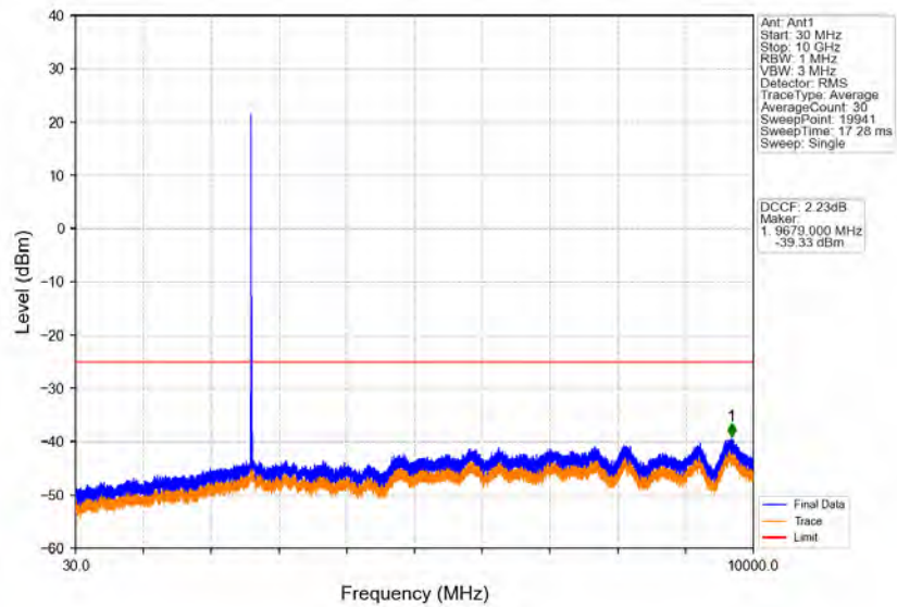
Band38_10MHz_64QAM_HCH_2615MHz_RB_1_0_NTNV
