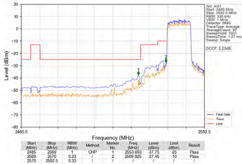
Band38_15MHz_QPSK_LCH_2577.5MHz_RB_75_0_NTNV
