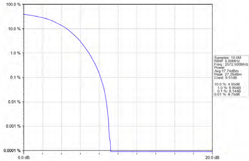
Band38_5MHz_64QAM_LCH_2572.5MHz_RB_25_0_NTNV
