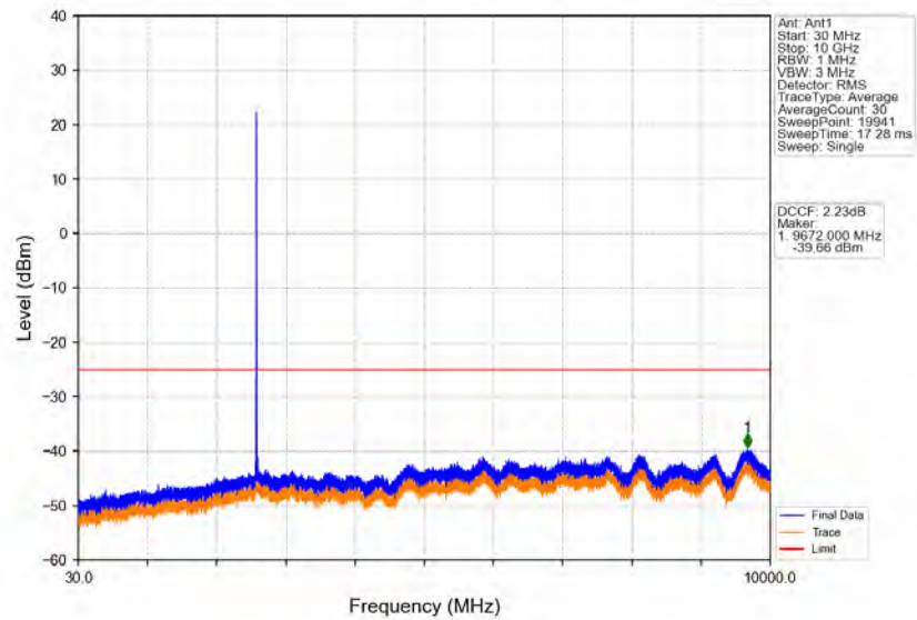
Band38_5MHz_16QAM_MCH_2595MHz_RB_1_0_NTNV
