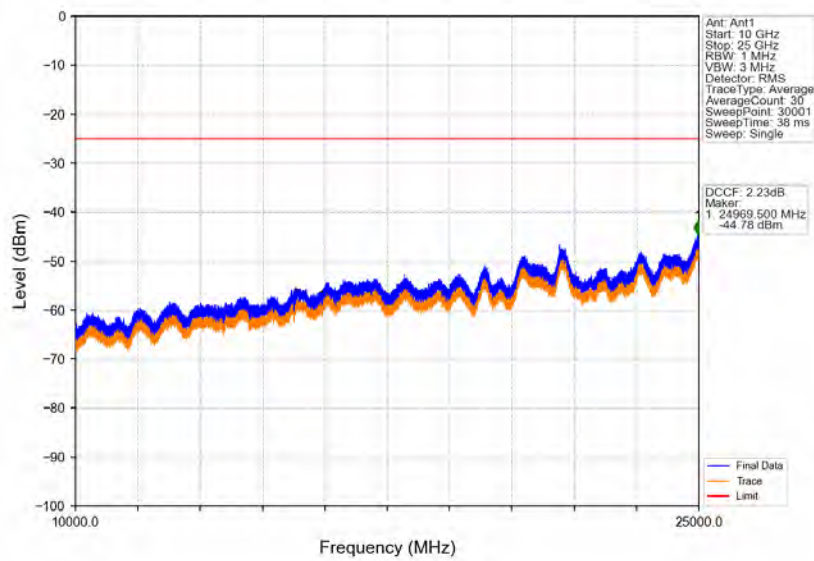
Band38_15MHz_QPSK_HCH_2612.5MHz_RB_1_0_NTNV
