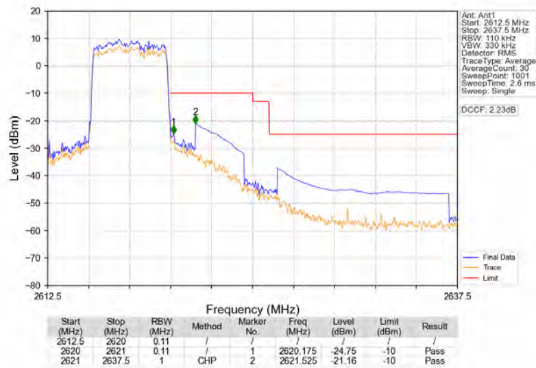
Band38_5MHz_16QAM_HCH_2617.5MHz_RB_25_0_NTNV
