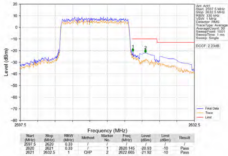
Band38_15MHz_QPSK_HCH_2612.5MHz_RB_75_0_NTNV
