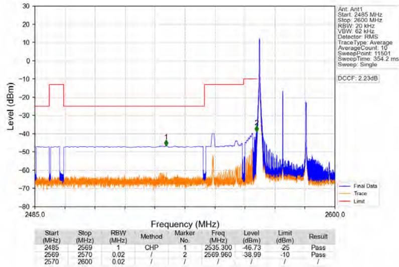
Band38_20MHz_64QAM_LCH_2580MHz_RB_1_0_NTNV
