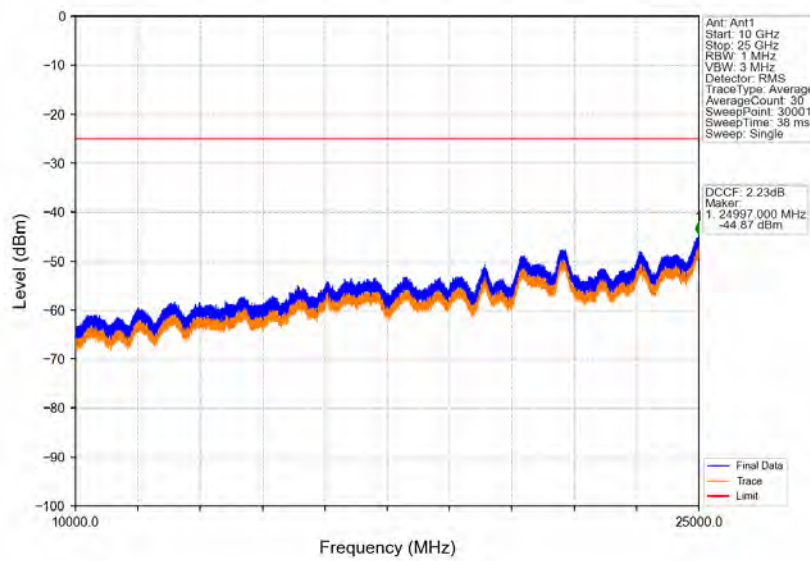
Band38_5MHz_64QAM_HCH_2617.5MHz_RB_1_0_NTNV
