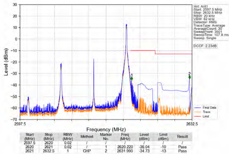
Band38_15MHz_64QAM_HCH_2612.5MHz_RB_1_74_NTNV
