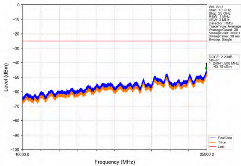
Band38_20MHz_64QAM_HCH_2610MHz_RB_1_0_NTNV
