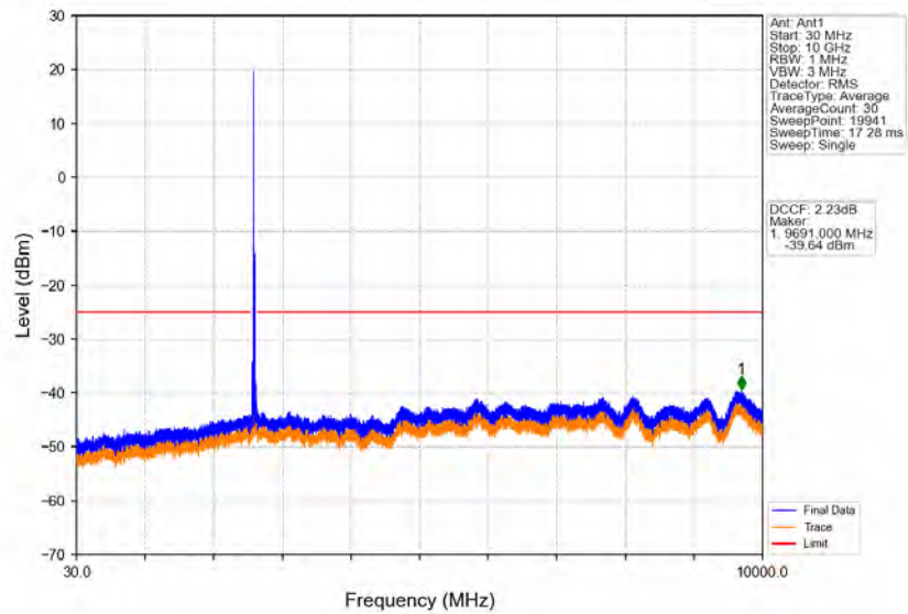
Band38_20MHz_64QAM_HCH_2610MHz_RB_1_0_NTNV
