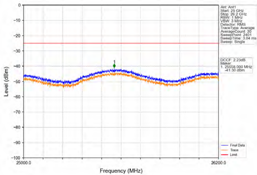
Band38_15MHz_16QAM_HCH_2612.5MHz_RB_1_0_NTNV
