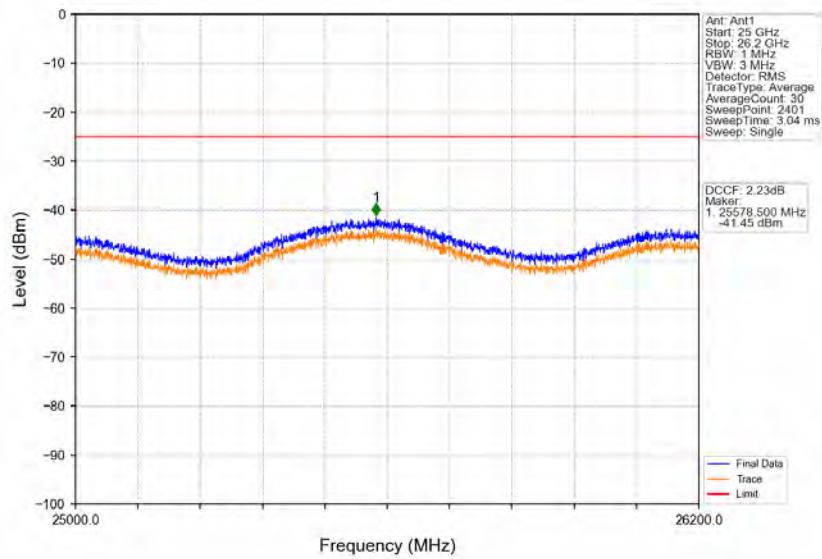
Band38_15MHz_QPSK_LCH_2577.5MHz_RB_1_0_NTNV
