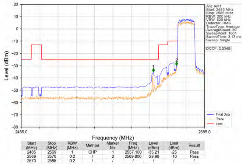
Band38_10MHz_16QAM_LCH_2575MHz_RB_50_0_NTNV
