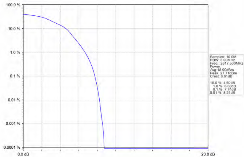
Band38_5MHz_16QAM_HCH_2617.5MHz_RB_25_0_NTNV
