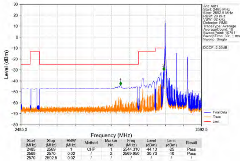
Band38_15MHz_64QAM_LCH_2577.5MHz_RB_1_0_NTNV
