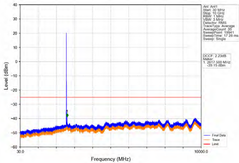
Band38_15MHz_64QAM_LCH_2577.5MHz_RB_1_0_NTNV
