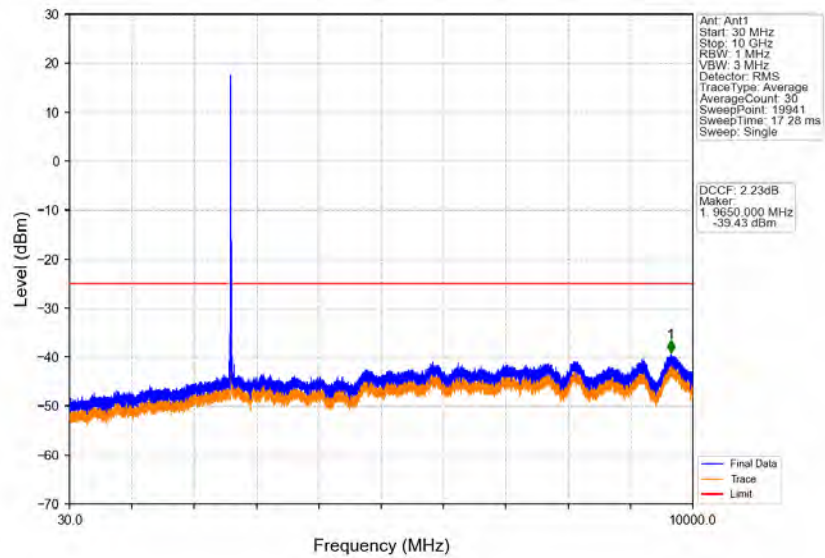
Band38_15MHz_64QAM_HCH_2612.5MHz_RB_1_0_NTNV
