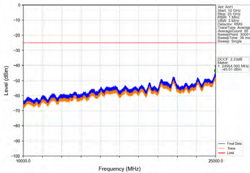
Band38_10MHz_16QAM_MCH_2595MHz_RB_1_0_NTNV
