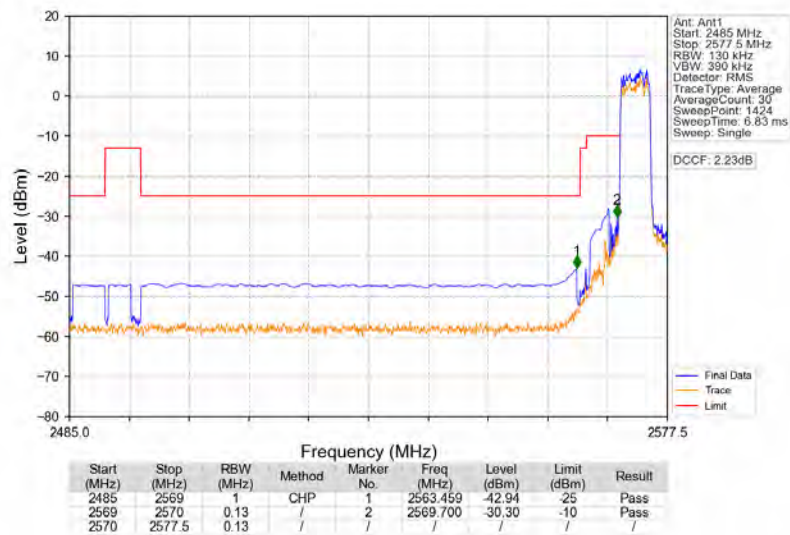
Band38_5MHz_16QAM_LCH_2572.5MHz_RB_25_0_NTNV
