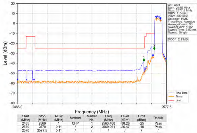
Band38_5MHz_QPSK_LCH_2572.5MHz_RB_25_0_NTNV
