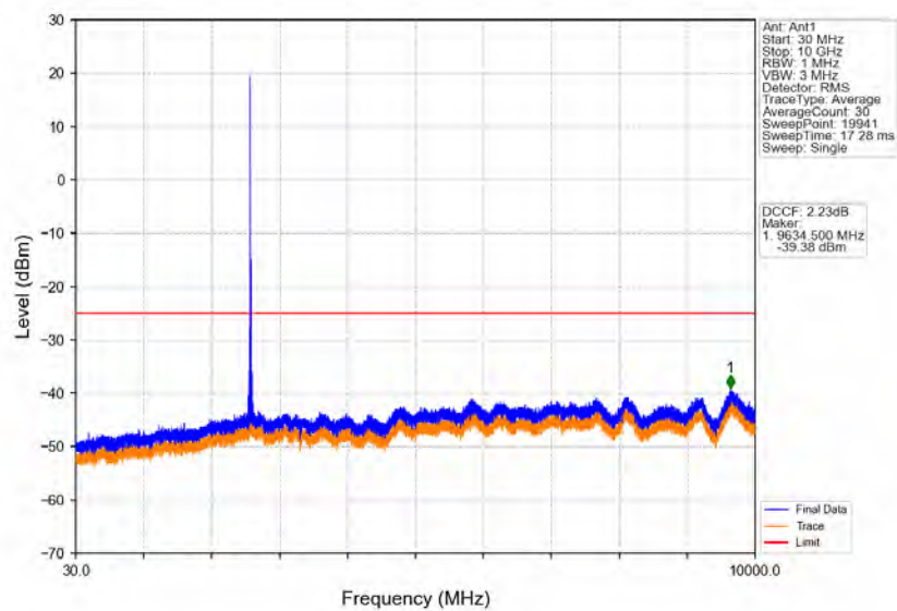
Band38_15MHz_64QAM_MCH_2595MHz_RB_1_0_NTNV
