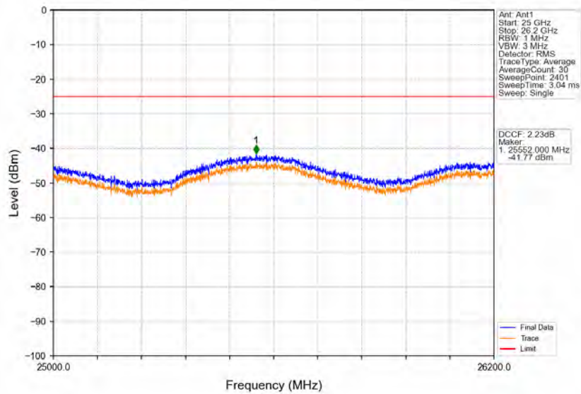
Band38_10MHz_16QAM_HCH_2615MHz_RB_1_0_NTNV
