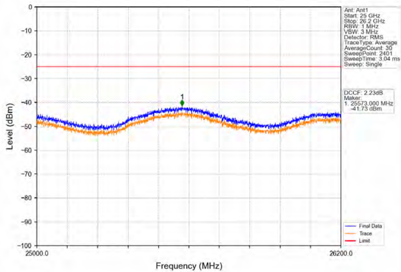
Band38_5MHz_16QAM_HCH_2617.5MHz_RB_1_0_NTNV
