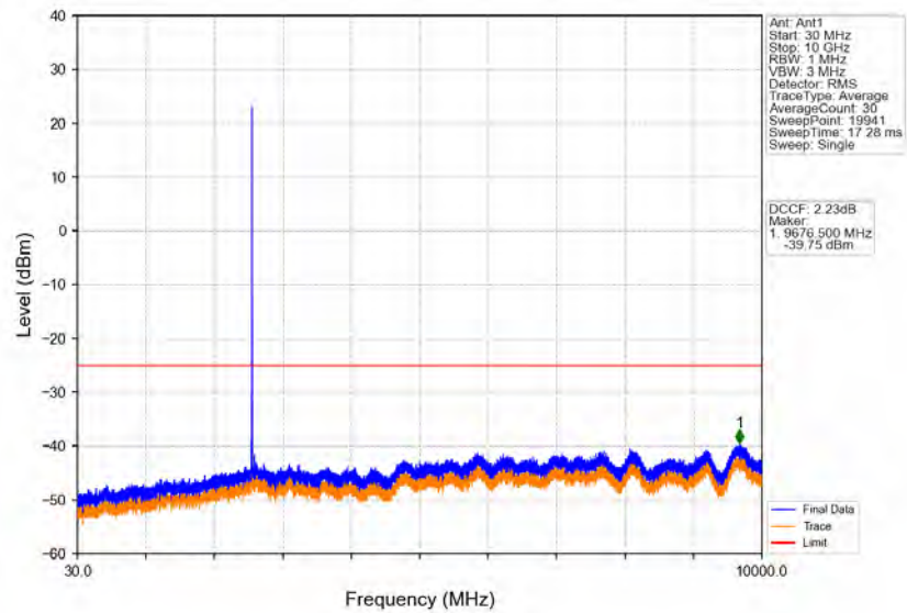
Band38_5MHz_16QAM_LCH_2572.5MHz_RB_1_0_NTNV
