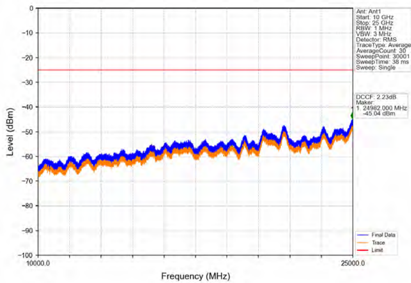
Band38_5MHz_QPSK_HCH_2617.5MHz_RB_1_0_NTNV
