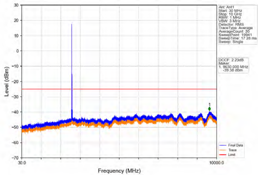
Band38_20MHz_64QAM_MCH_2595MHz_RB_1_0_NTNV
