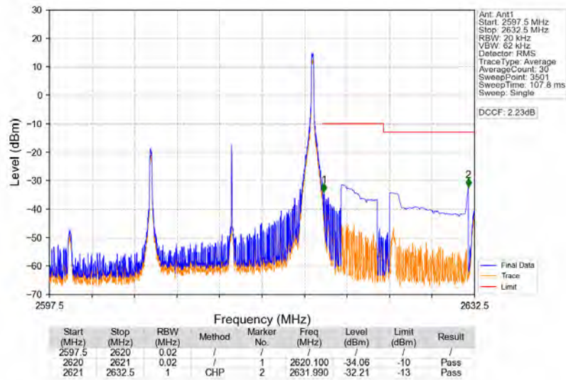
Band38_15MHz_QPSK_HCH_2612.5MHz_RB_1_74_NTNV
