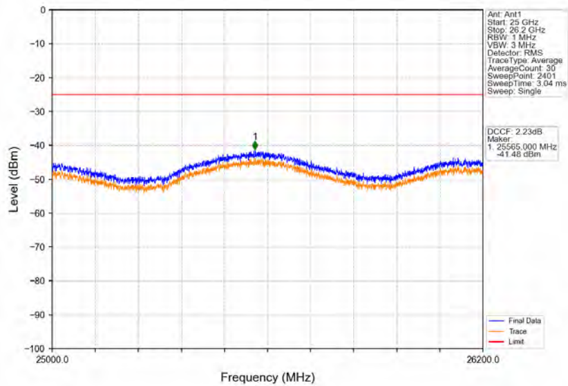
Band38_15MHz_64QAM_HCH_2612.5MHz_RB_1_74_NTNV
