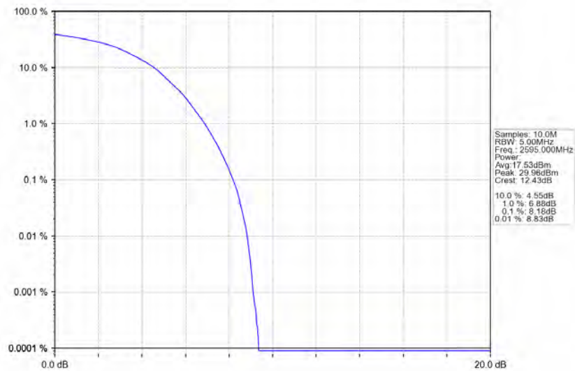
Band38_5MHz_64QAM_MCH_2595MHz_RB_25_0_NTNV
