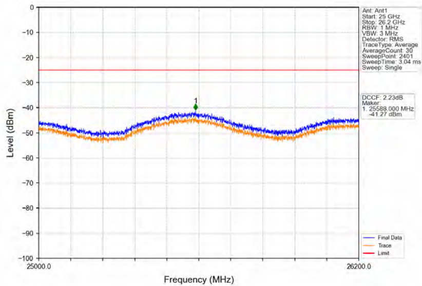
Band38_5MHz_64QAM_HCH_2617.5MHz_RB_1_24_NTNV
