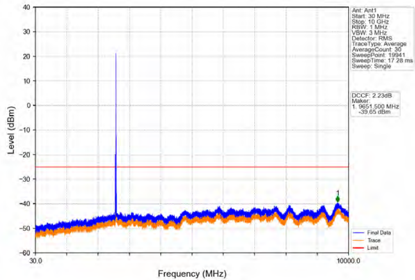
Band38_10MHz_16QAM_MCH_2595MHz_RB_1_0_NTNV
