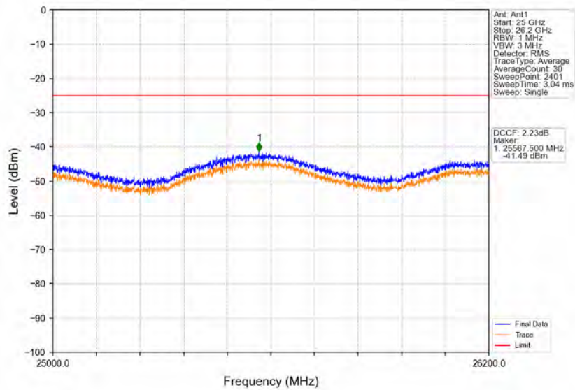
Band38_10MHz_16QAM_LCH_2575MHz_RB_50_0_NTNV
