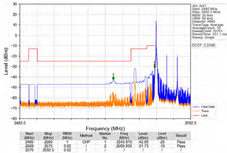
Band38_15MHz_16QAM_LCH_2577.5MHz_RB_1_0_NTNV
