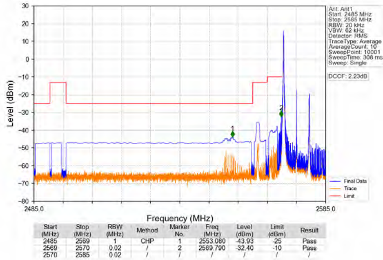
Band38_10MHz_64QAM_LCH_2575MHz_RB_1_0_NTNV
