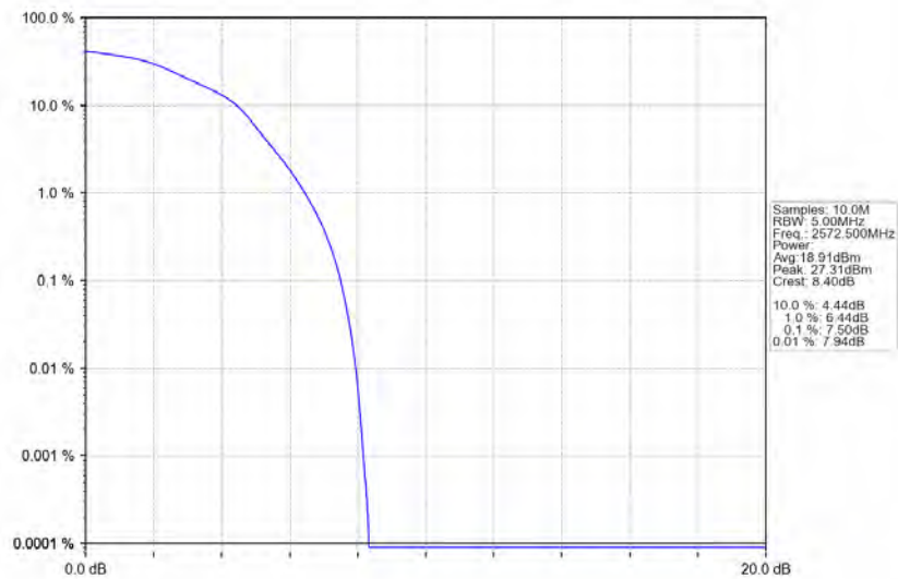
Band38_5MHz_16QAM_LCH_2572.5MHz_RB_25_0_NTNV
