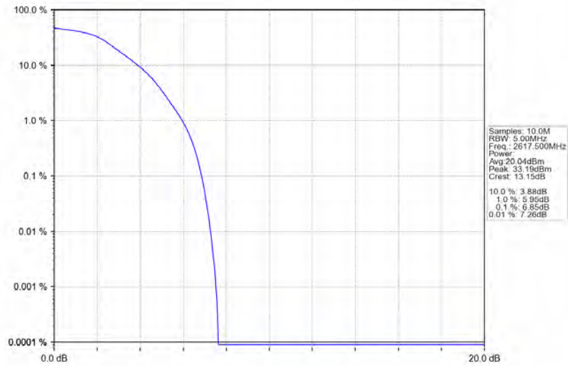
Band38_5MHz_QPSK_HCH_2617.5MHz_RB_25_0_NTNV
