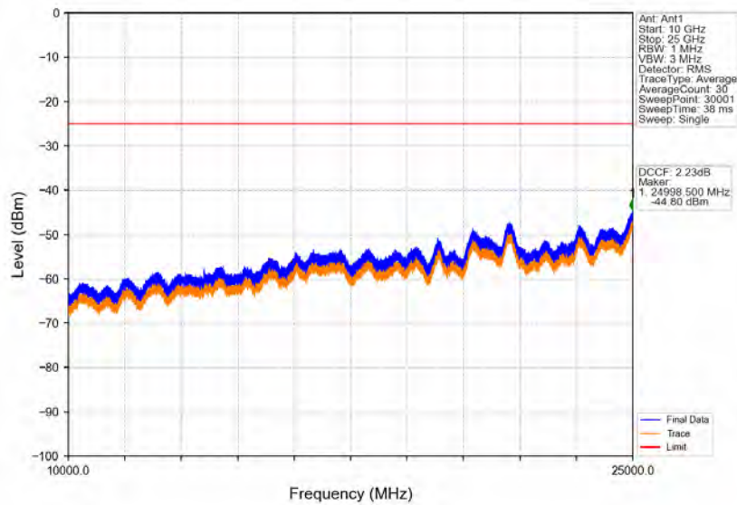
Band38_10MHz_64QAM_MCH_2595MHz_RB_1_0_NTNV
