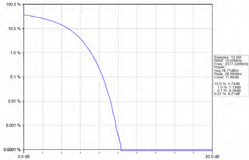
Band38_15MHz_64QAM_LCH_2577.5MHz_RB_75_0_NTNV
