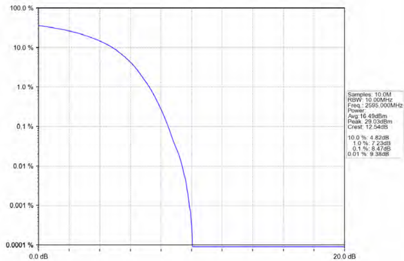
Band38_15MHz_64QAM_MCH_2595MHz_RB_75_0_NTNV
