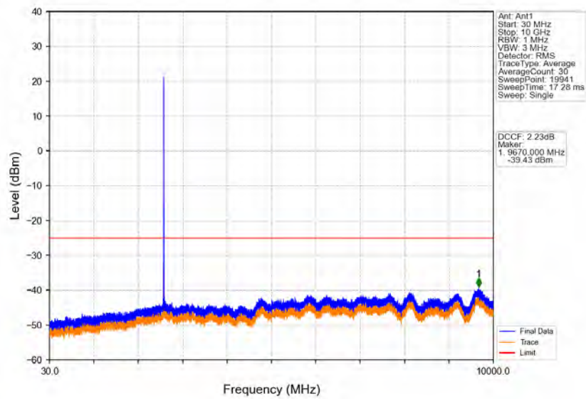
Band38_5MHz_64QAM_MCH_2595MHz_RB_1_0_NTNV
