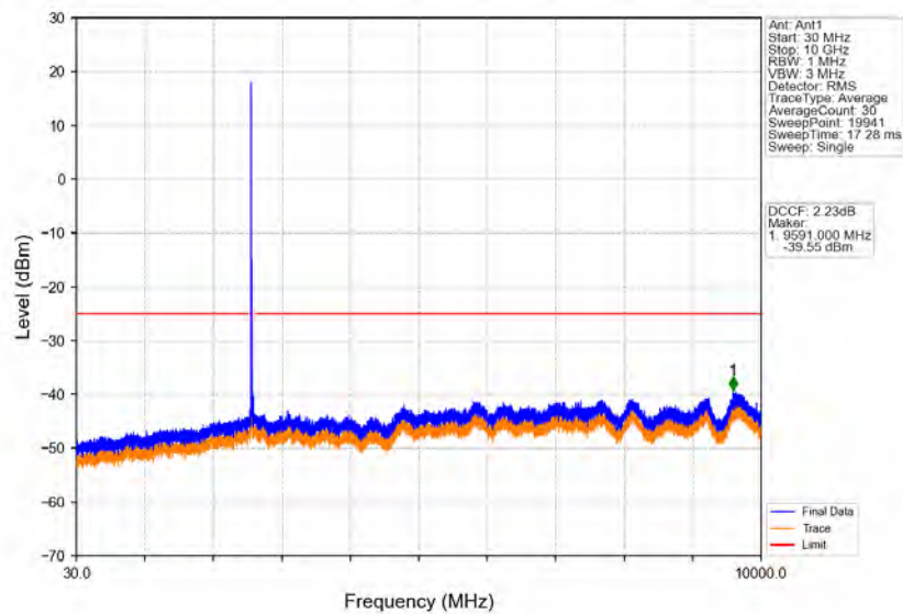
Band38_20MHz_64QAM_LCH_2580MHz_RB_1_0_NTNV
