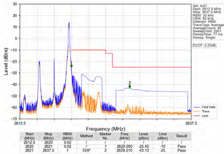
Band38_5MHz_16QAM_HCH_2617.5MHz_RB_1_24_NTNV
