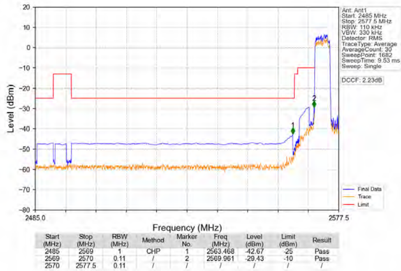
Band38_5MHz_64QAM_LCH_2572.5MHz_RB_25_0_NTNV
