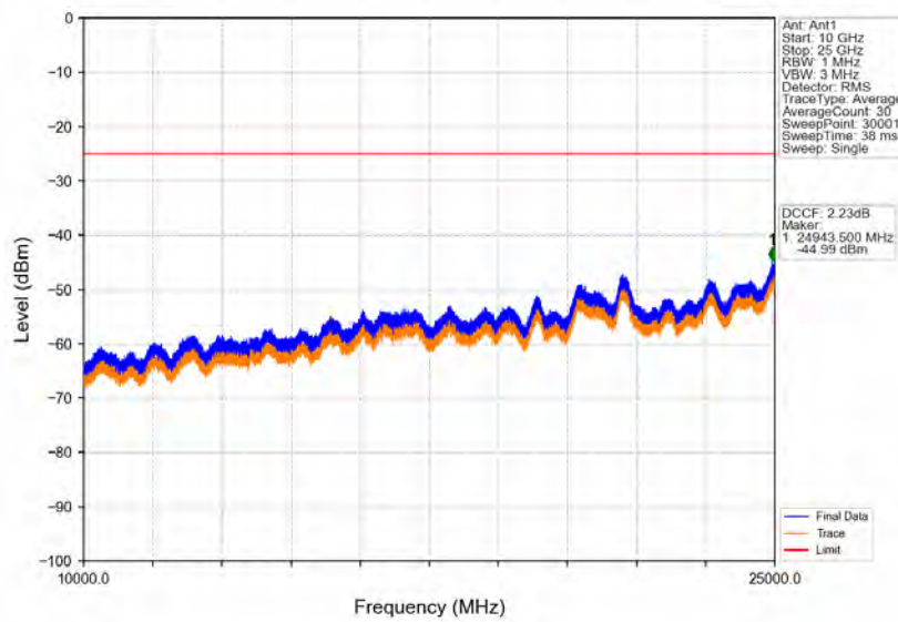
Band38_5MHz_16QAM_LCH_2572.5MHz_RB_1_0_NTNV
