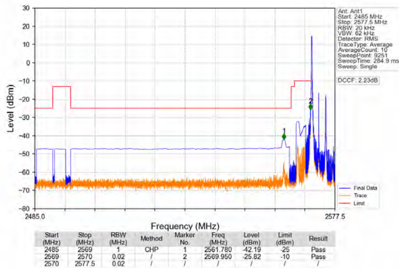
Band38_5MHz_16QAM_LCH_2572.5MHz_RB_1_0_NTNV
