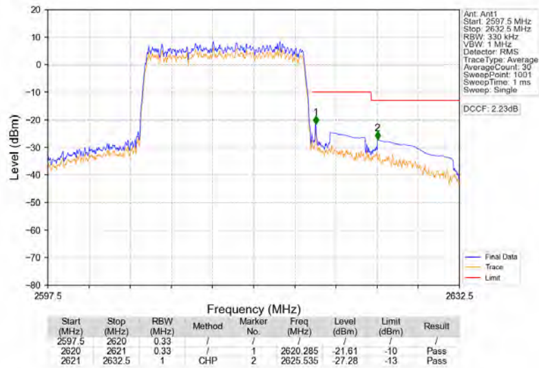
Band38_15MHz_16QAM_HCH_2612.5MHz_RB_75_0_NTNV
