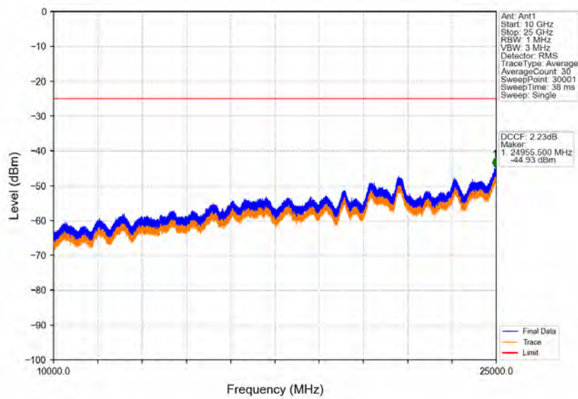
Band38_15MHz_16QAM_MCH_2595MHz_RB_1_0_NTNV
