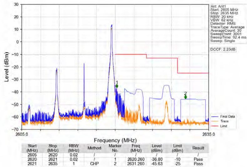
Band38_10MHz_64QAM_HCH_2615MHz_RB_1_49_NTNV
