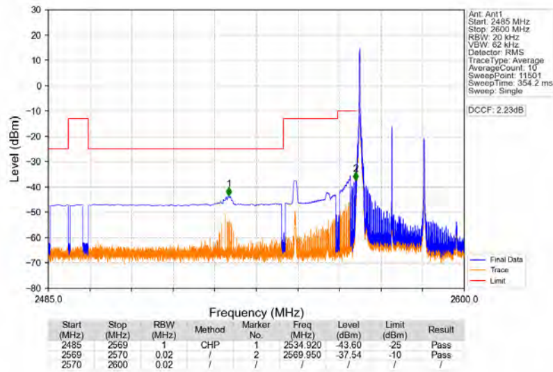
Band38 20MHz 16QAM LCH 2580MHz RB 1 0 NTN
