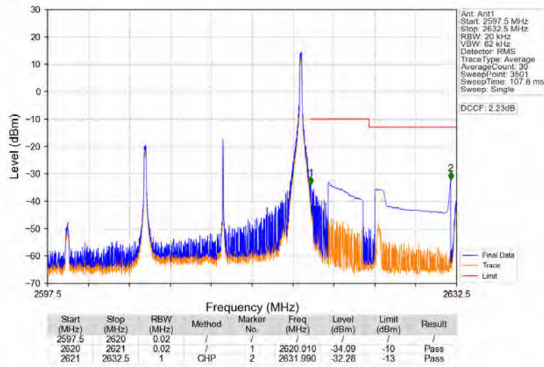
Band38_15MHz_16QAM_HCH_2612.5MHz_RB_1_74_NTNV
