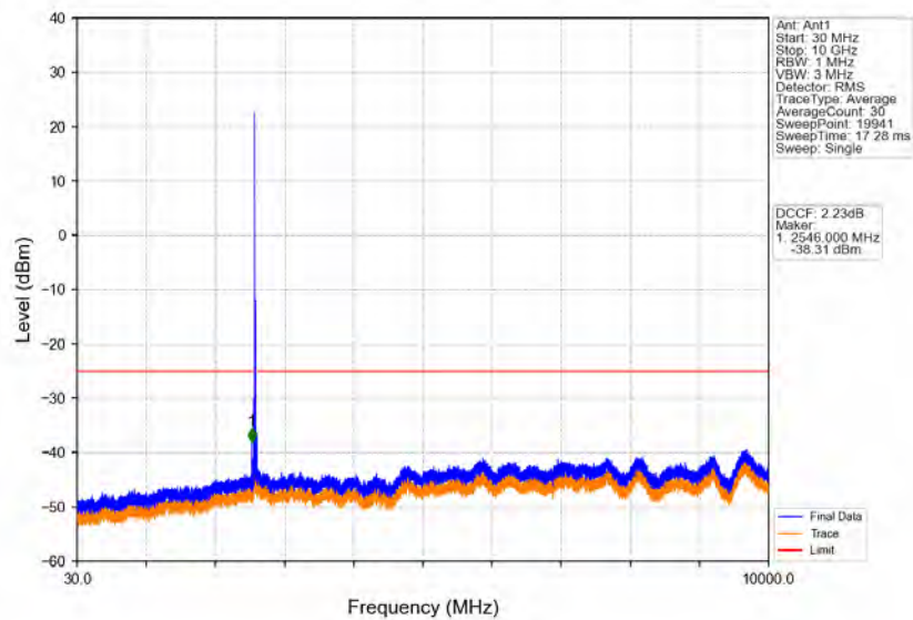
Band38_15MHz_QPSK_MCH_2595MHz_RB_1_0_NTNV
