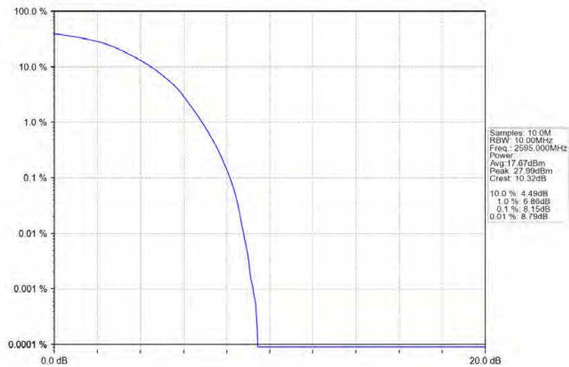
Band38_10MHz_64QAM_MCH_2595MHz_RB_50_0_NTNV
