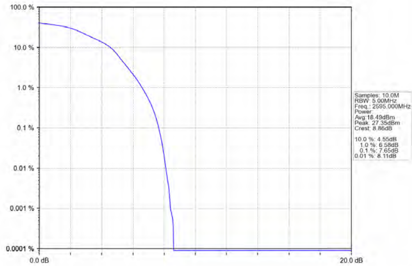
Band38_5MHz_16QAM_MCH_2595MHz_RB_25_0_NTNV
