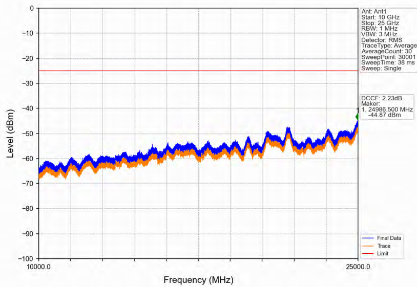
Band38_10MHz_64QAM_HCH_2615MHz_RB_1_0_NTNV
