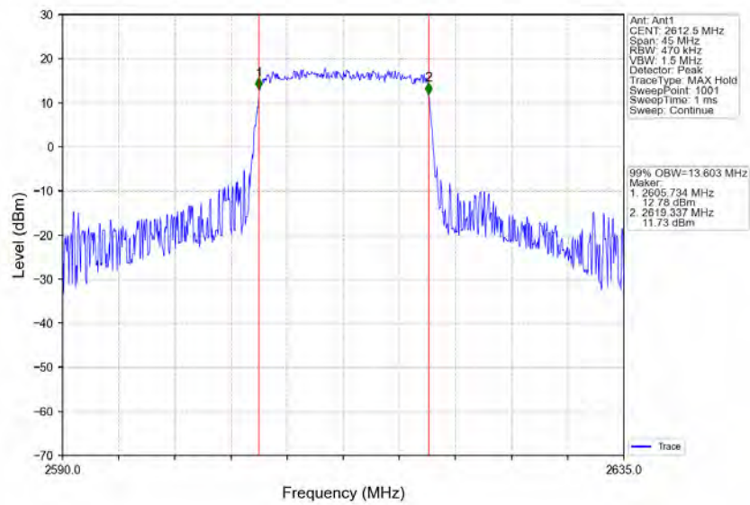
Band38_15MHz_16QAM_HCH_2612.5MHz_RB_75_0_NTNV
