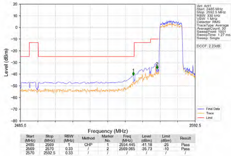
Band38_15MHz_64QAM_LCH_2577.5MHz_RB_75_0_NTNV
