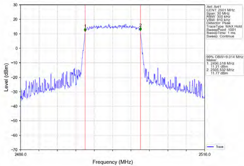
Band41_10MHz_64QAM_LCH_2501MHz_RB_50_0_NTNV
