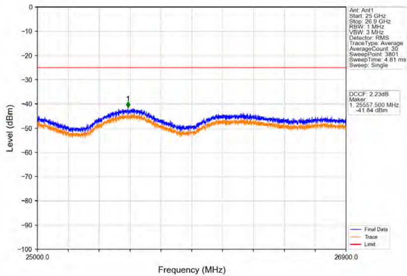
Band41_20MHz_16QAM_LCH_2506MHz_RB_100_0_NTNV
