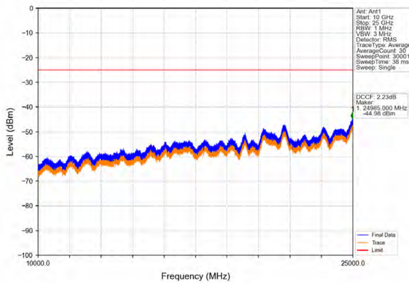
Band41_10MHz_64QAM_HCH_2685MHz_RB_1_0_NTNV
