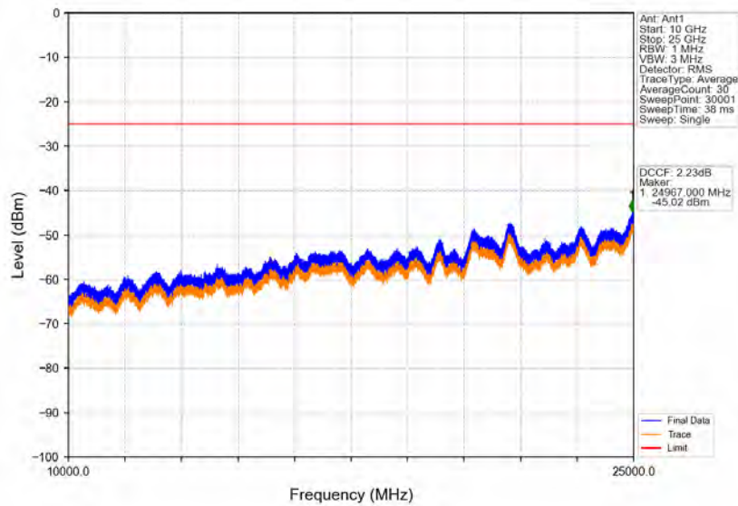
Band41_5MHz_16QAM_HCH_2687.5MHz_RB_1_0_NTNV
