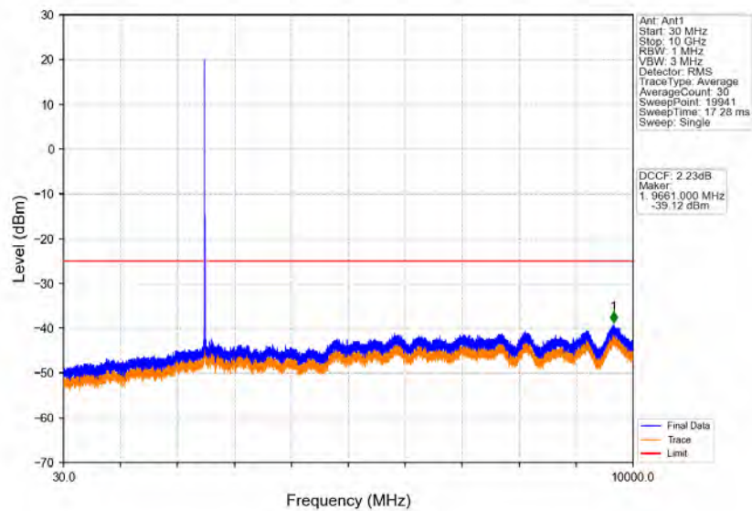
Band41_15MHz_64QAM_LCH_2503.5MHz_RB_1_0_NTNV
