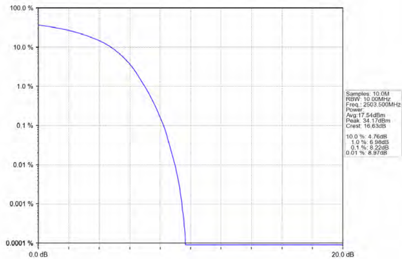
Band41_15MHz_16QAM_LCH_2503.5MHz_RB_75_0_NTNV
