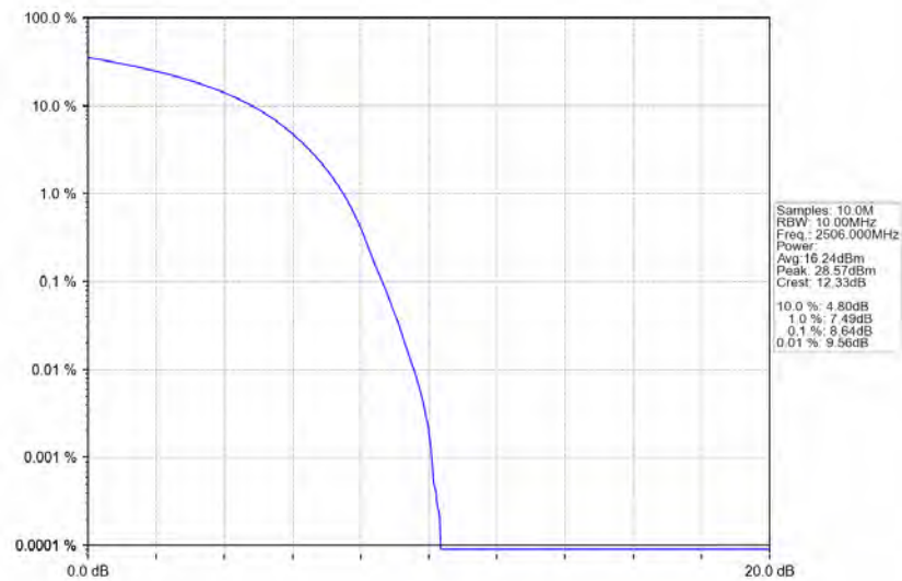
Band41_20MHz_16QAM_LCH_2506MHz_RB_100_0_NTNV
