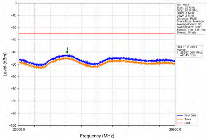
Band41_20MHz_64QAM_HCH_2680MHz_RB_1_99_NTNV
