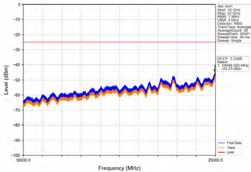
Band41_15MHz_64QAM_LCH_2503.5MHz_RB_1_0_NTNV
