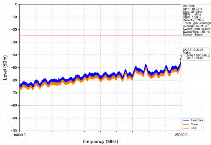
Band41_20MHz_16QAM_LCH_2506MHz_RB_1_0_NTNV
