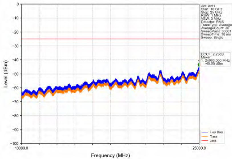
Band41_10MHz_64QAM_LCH_2501MHz_RB_1_0_NTNV
