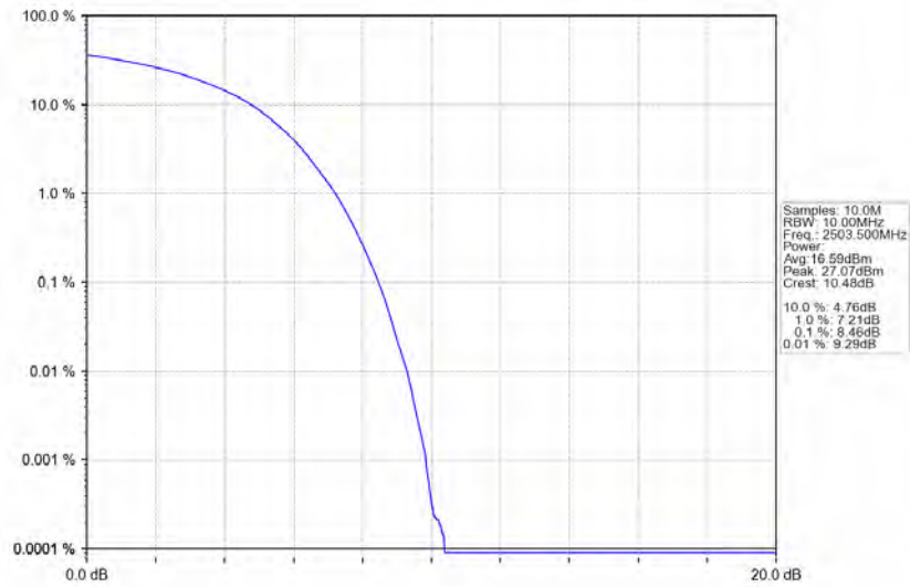
Band41_15MHz_64QAM_LCH_2503.5MHz_RB_75_0_NTNV
