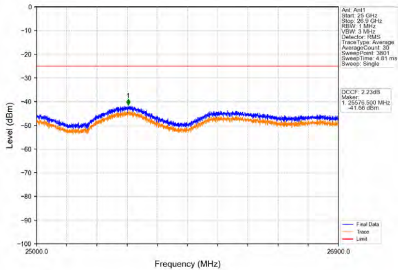
Band41_5MHz_64QAM_HCH_2687.5MHz_RB_1_24_NTNV
