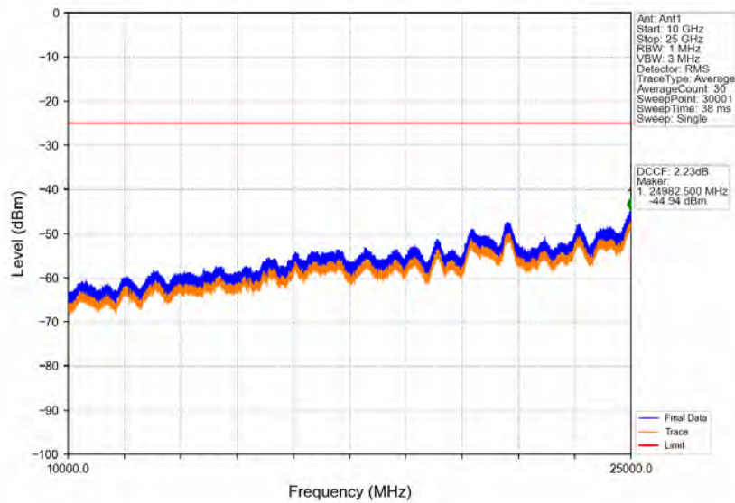
Band41_20MHz_64QAM_LCH_2506MHz_RB_1_0_NTNV
