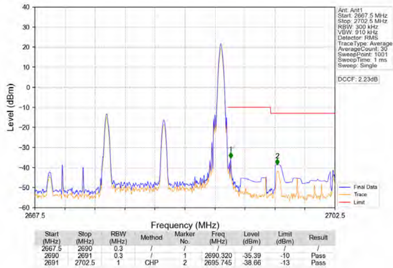
Band41_15MHz_64QAM_HCH_2682.5MHz_RB_1_74_NTNV
