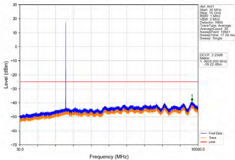
Band41_5MHz_64QAM_MCH_2593MHz_RB_1_0_NTNV
