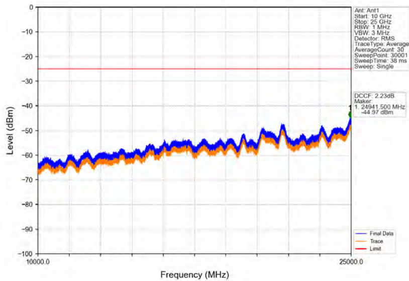
Band41_20MHz_64QAM_MCH_2593MHz_RB_1_0_NTNV
