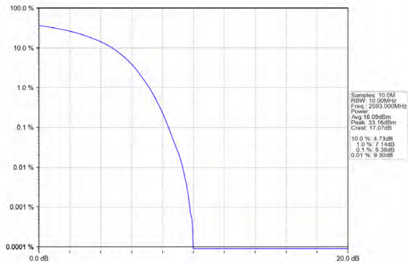
Band41_15MHz_64QAM_MCH_2593MHz_RB_75_0_NTNV
