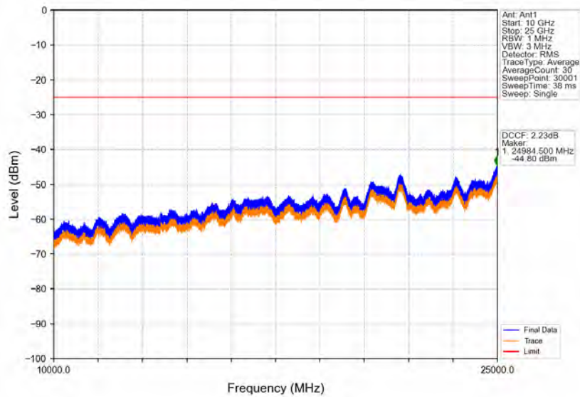
Band41_15MHz_64QAM_MCH_2593MHz_RB_1_0_NTNV
