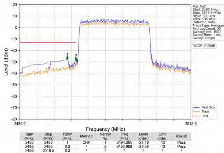
Band41_15MHz_16QAM_LCH_2503.5MHz_RB_75_0_NTNV
