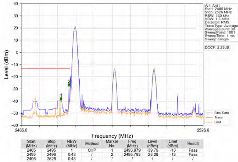
Band41_20MHz_64QAM_LCH_2506MHz_RB_1_0_NTNV
