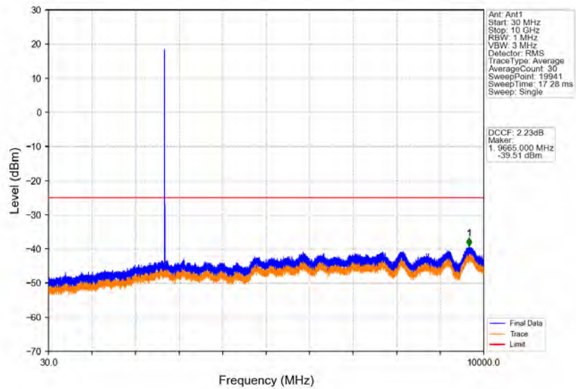
Band41_5MHz_64QAM_HCH_2687.5MHz_RB_1_0_NTNV
