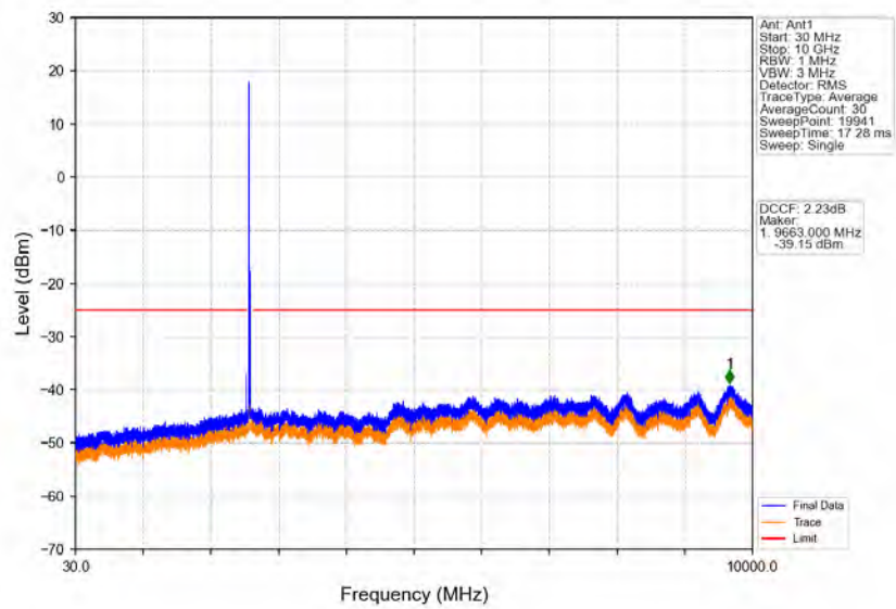
Band41_20MHz_64QAM_MCH_2593MHz_RB_1_0_NTNV
