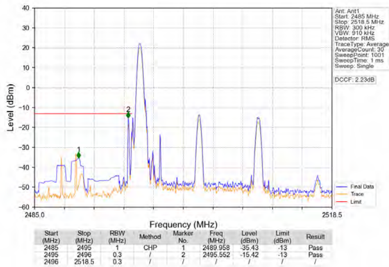
Band41_15MHz_16QAM_LCH_2503.5MHz_RB_1_0_NTNV
