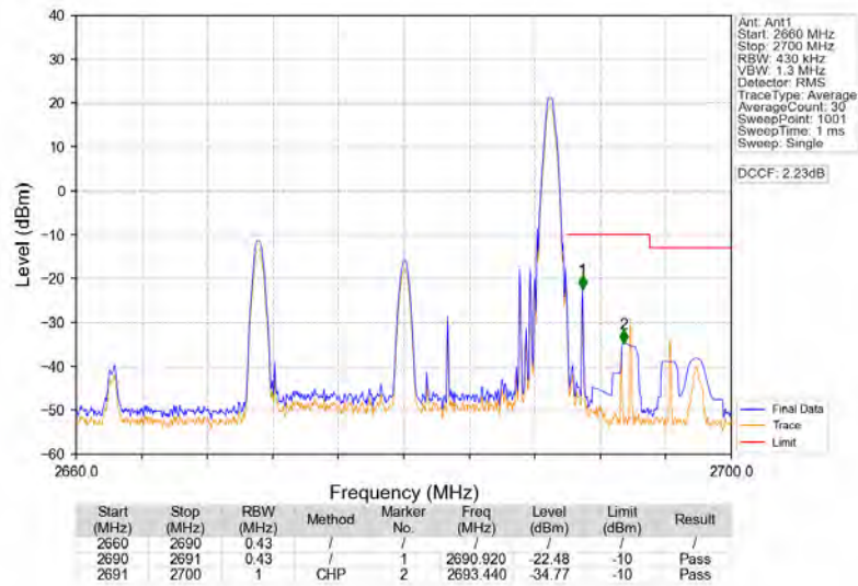
Band41_20MHz_64QAM_HCH_2680MHz_RB_1_99_NTNV
