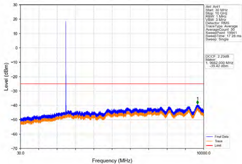
Band41_10MHz_64QAM_LCH_2501MHz_RB_1_0_NTNV
