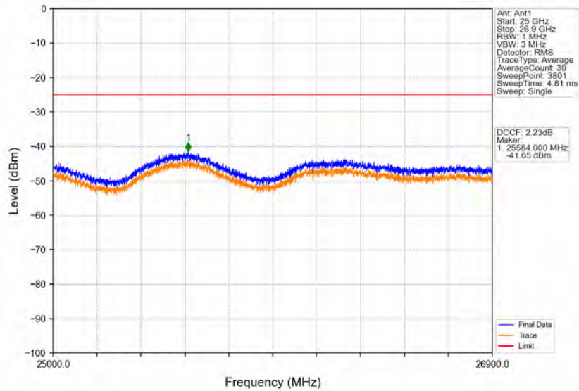
Band41_15MHz_64QAM_HCH_2682.5MHz_RB_1_74_NTNV
