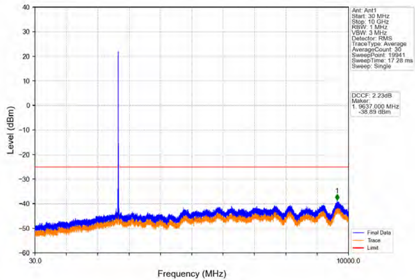
Band41_15MHz_64QAM_HCH_2682.5MHz_RB_1_0_NTNV
