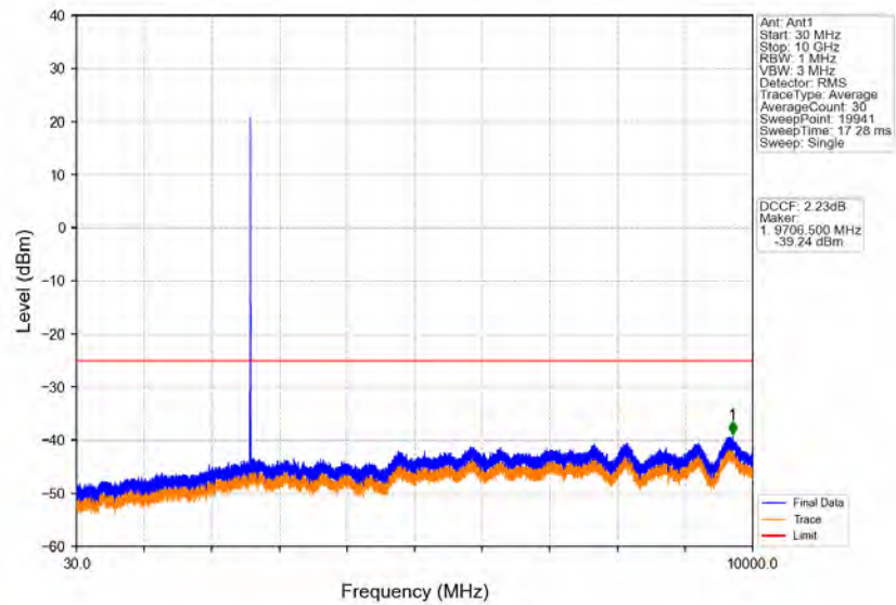
Band41_5MHz_16QAM_MCH_2593MHz_RB_1_0_NTNV
