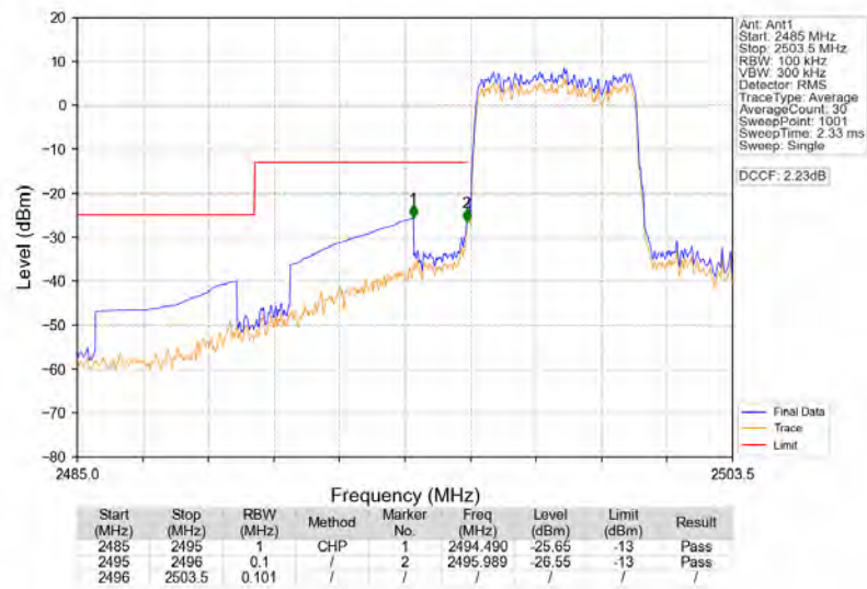
Band41_5MHz_16QAM_LCH_2498.5MHz_RB_25_0_NTNV
