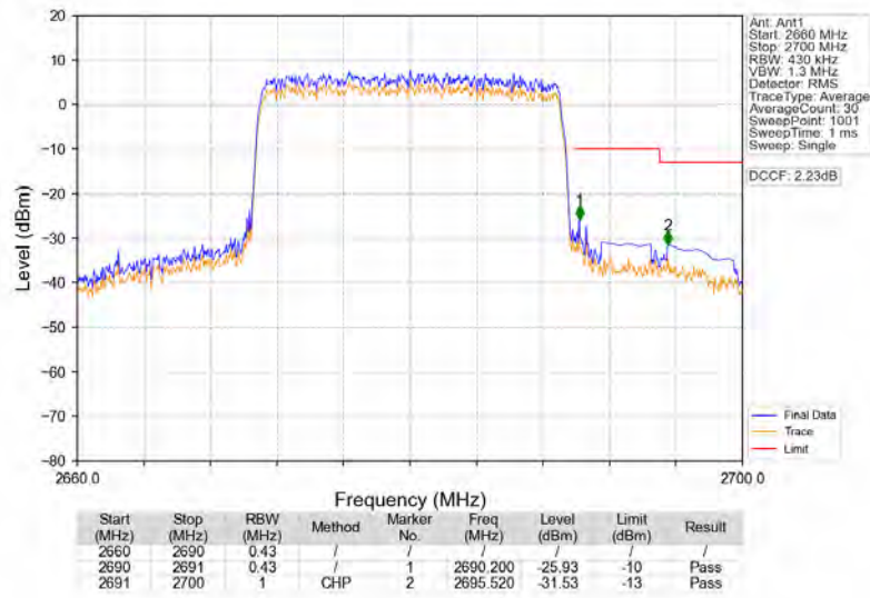
Band41_20MHz_16QAM_HCH_2680MHz_RB_100_0_NTNV
