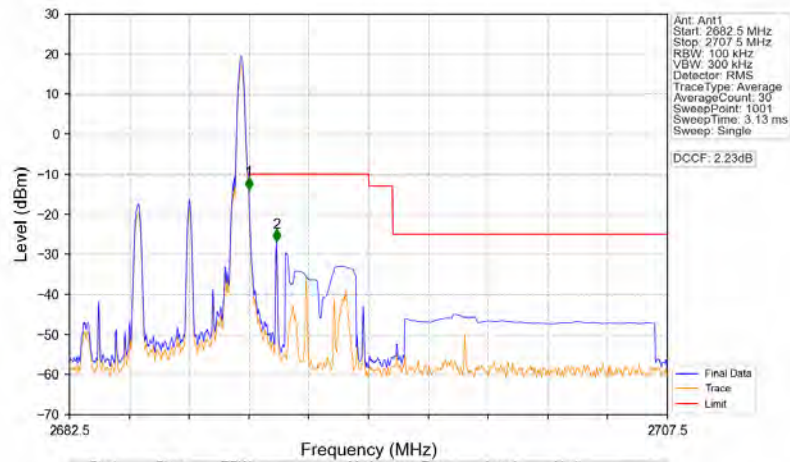
Band41_5MHz_64QAM_HCH_2687.5MHz_RB_1_24_NTNV
