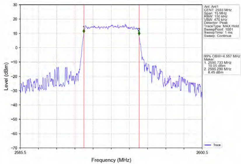
Band41_5MHz_64QAM_MCH_2593MHz_RB_25_0_NTNV
