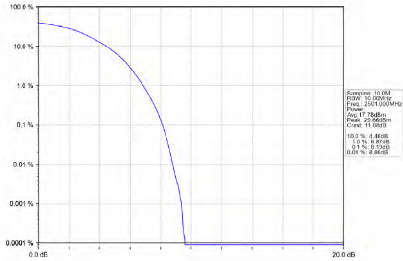
Band41_10MHz_64QAM_LCH_2501MHz_RB_50_0_NTNV
