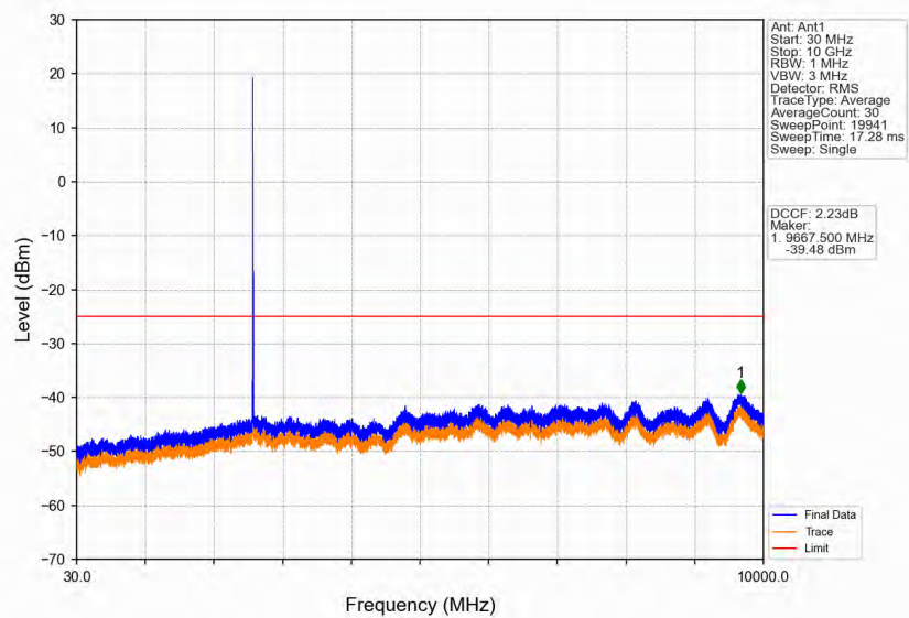
Band41_10MHz_64QAM_MCH_2593MHz_RB_1_0_NTNV
