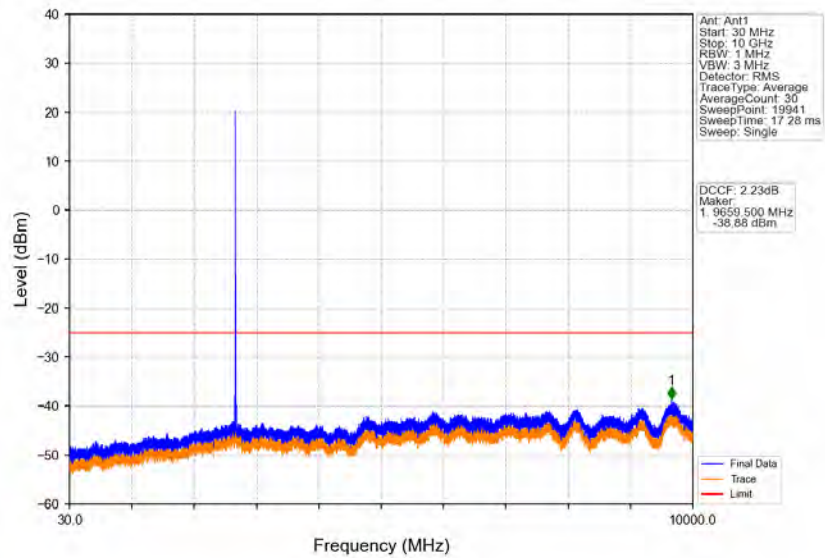
Band41_10MHz_64QAM_HCH_2685MHz_RB_1_0_NTNV
