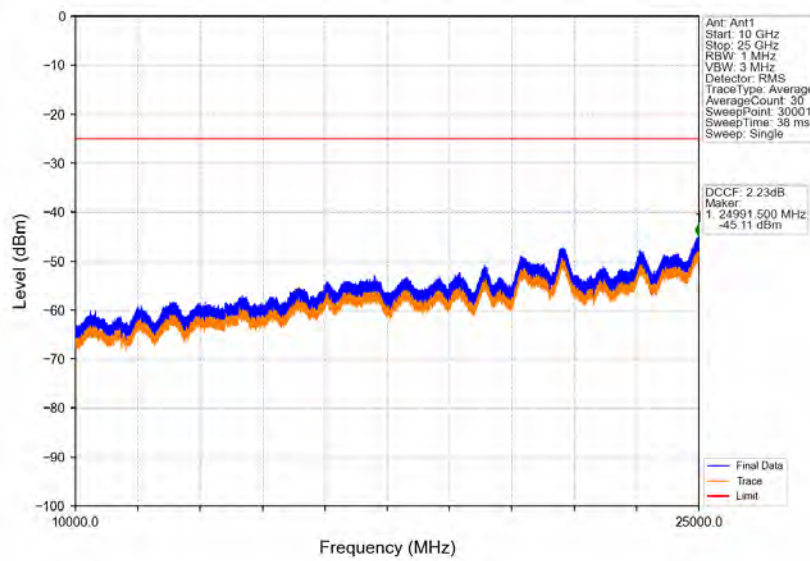
Band41_5MHz_16QAM_MCH_2593MHz_RB_1_0_NTNV
