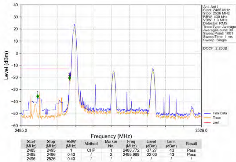
Band41_20MHz_16QAM_LCH_2506MHz_RB_1_0_NTNV
