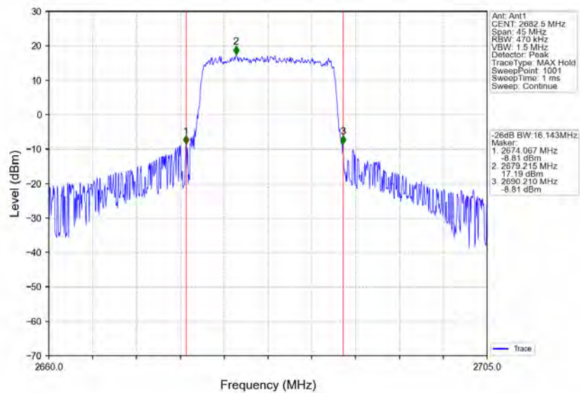
Band41_15MHz_16QAM_HCH_2682.5MHz_RB_75_0_NTNV
