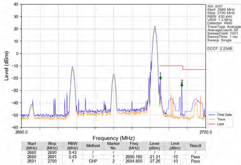
Band41_20MHz_16QAM_HCH_2680MHz_RB_1_99_NTNV
