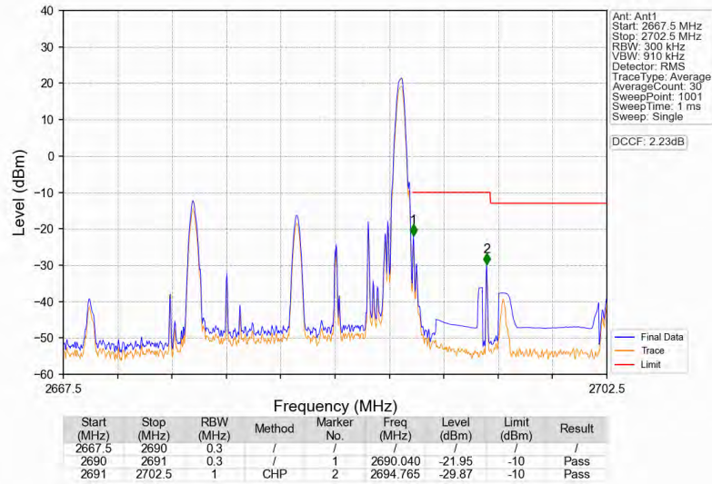
Band41_15MHz_16QAM_HCH_2682.5MHz_RB_1_74_NTNV
