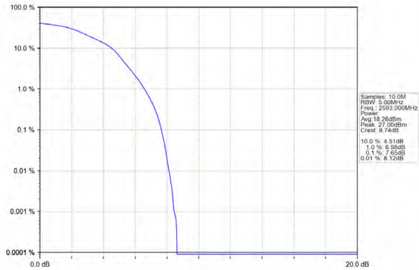
Band41_5MHz_16QAM_MCH_2593MHz_RB_25_0_NTNV
