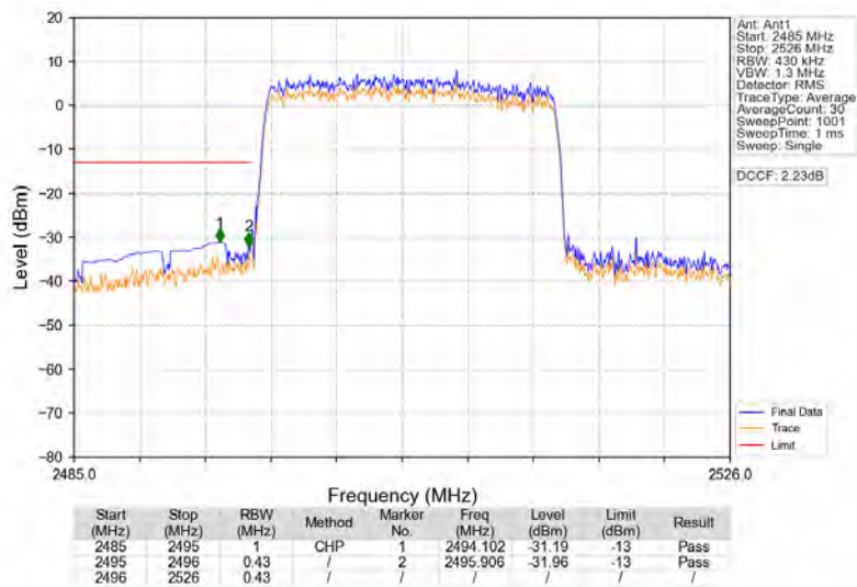
Band41_20MHz_16QAM_LCH_2506MHz_RB_100_0_NTNV
