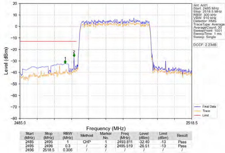
Band41_15MHz_64QAM_LCH_2503.5MHz_RB_75_0_NTNV
