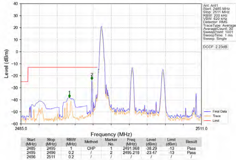
Band41_10MHz_64QAM_LCH_2501MHz_RB_1_0_NTNV
