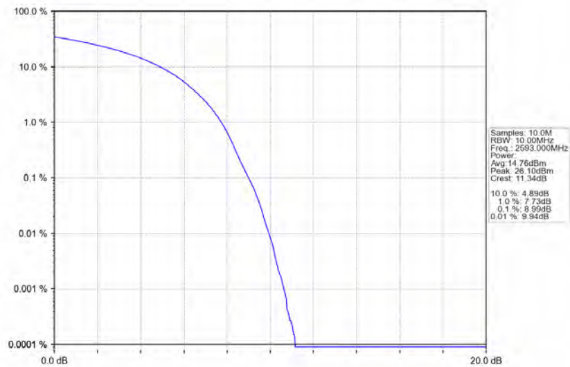
Band41_20MHz_64QAM_MCH_2593MHz_RB_100_0_NTNV
