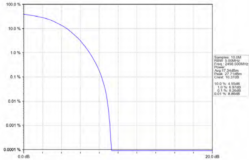
Band41_5MHz_64QAM_LCH_2498.5MHz_RB_25_0_NTNV
