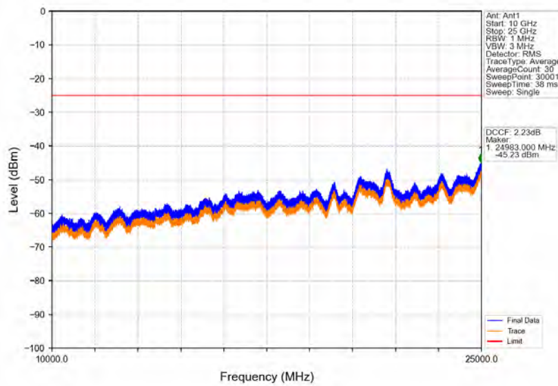
Band41_15MHz_16QAM_LCH_2503.5MHz_RB_1_0_NTNV
