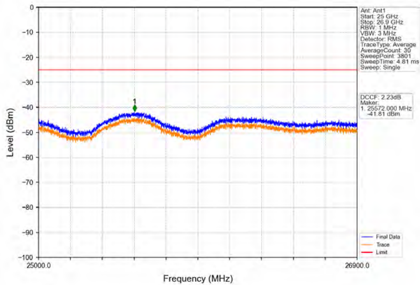
Band41_20MHz_16QAM_HCH_2680MHz_RB_1_0_NTNV
