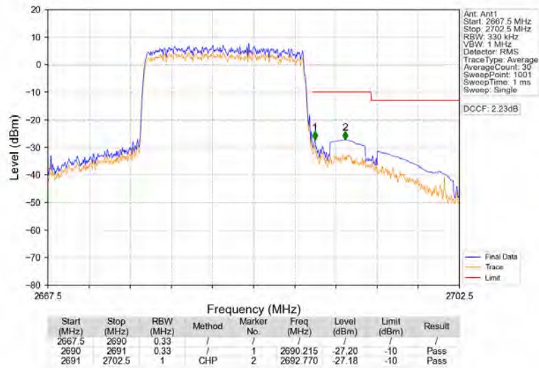
Band41_15MHz_16QAM_HCH_2682.5MHz_RB_75_0_NTNV
