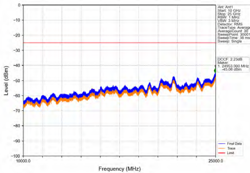
Band41_5MHz_64QAM_HCH_2687.5MHz_RB_1_0_NTNV
