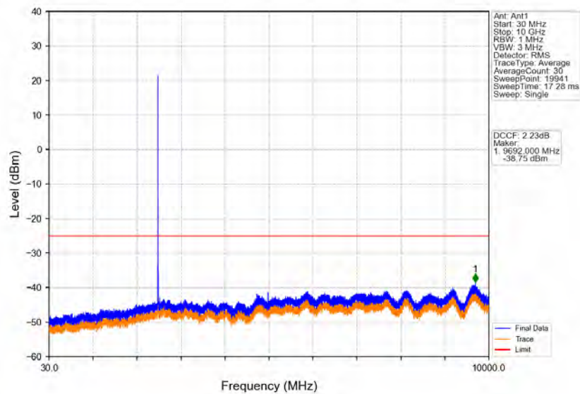
Band41_5MHz_64QAM_LCH_2498.5MHz_RB_1_0_NTNV
