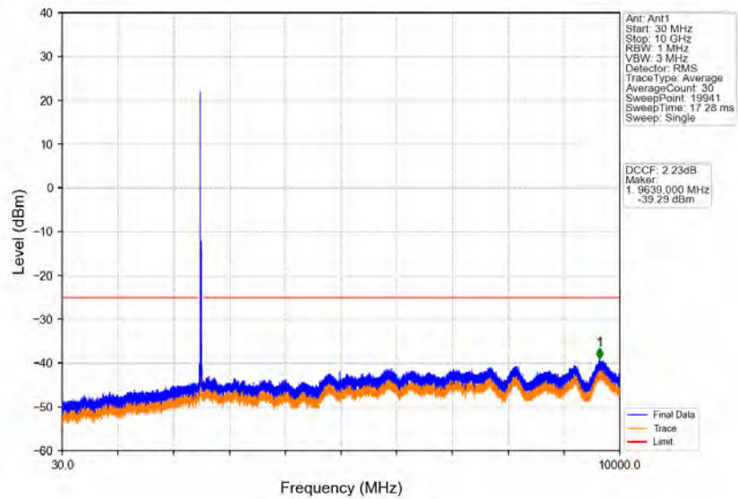
Band41_20MHz_16QAM_LCH_2506MHz_RB_1_0_NTNV
