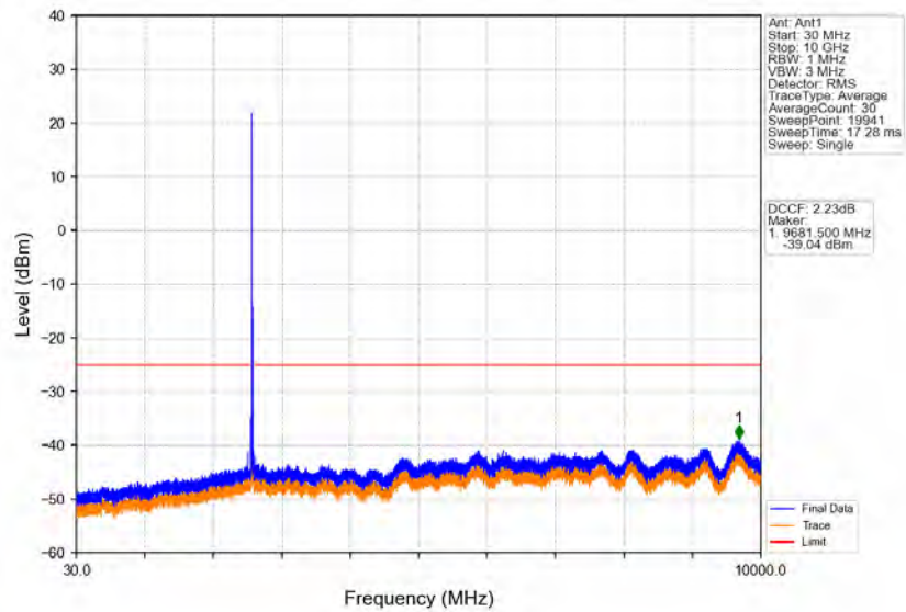
Band41_15MHz_16QAM_MCH_2593MHz_RB_1_0_NTNV
