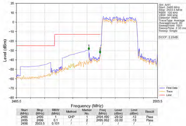
Band41_5MHz_64QAM_LCH_2498.5MHz_RB_25_0_NTNV
