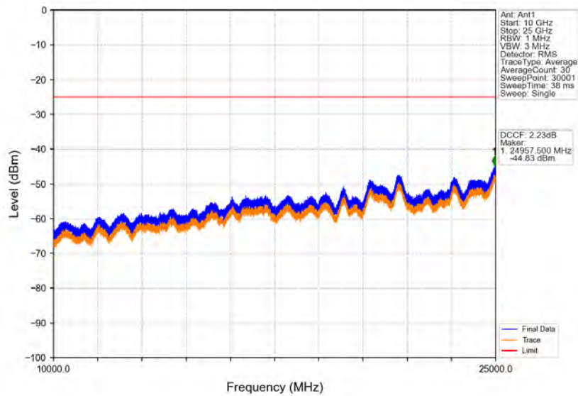
Band41_15MHz_16QAM_HCH_2682.5MHz_RB_1_0_NTNV
