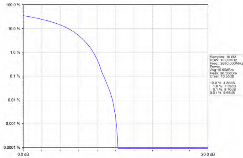
Band41_20MHz_16QAM_HCH_2680MHz_RB_100_0_NTNV
