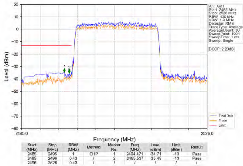
Band41_20MHz_64QAM_LCH_2506MHz_RB_100_0_NTNV
