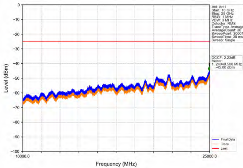
Band41_15MHz_16QAM_MCH_2593MHz_RB_1_0_NTNV
