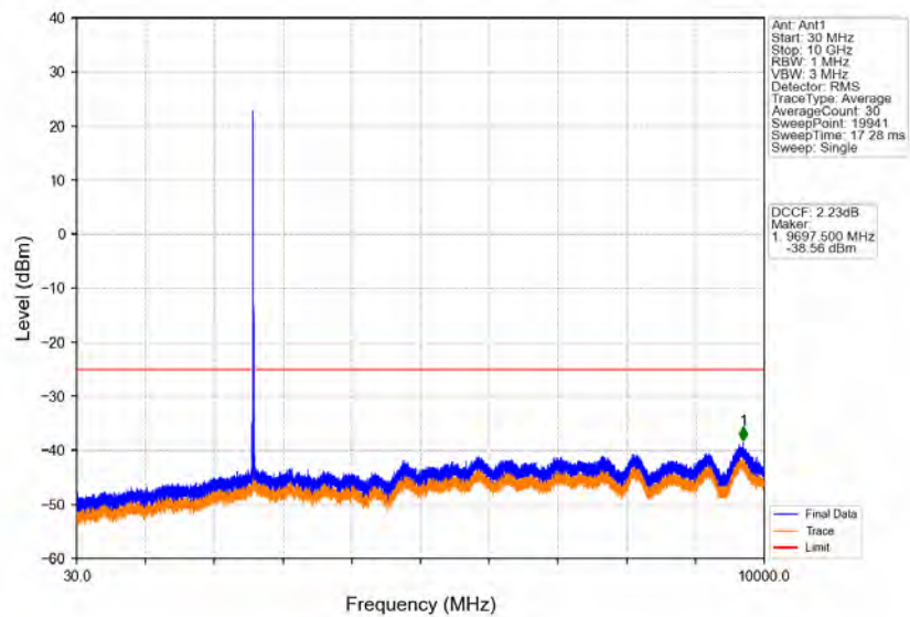
Band41_15MHz_64QAM_MCH_2593MHz_RB_1_0_NTNV
