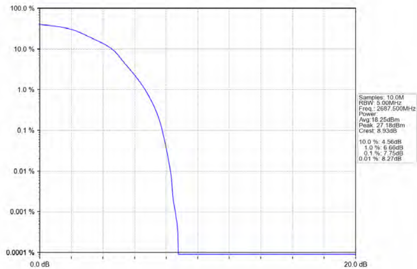
Band41_5MHz_16QAM_HCH_2687.5MHz_RB_25_0_NTNV
