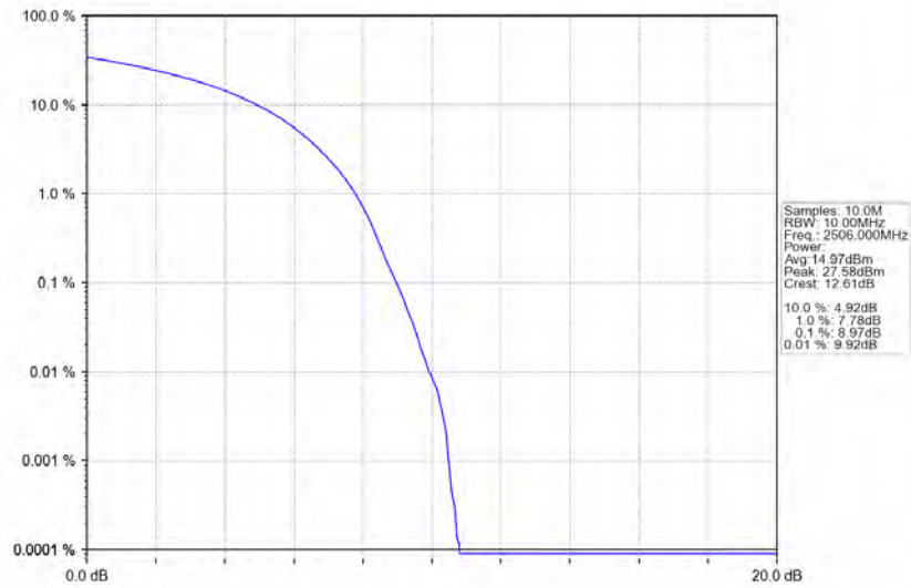
Band41_20MHz_64QAM_LCH_2506MHz_RB_100_0_NTNV
