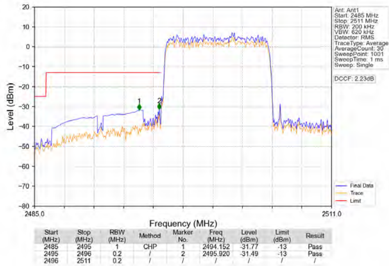
Band41_10MHz_64QAM_LCH_2501MHz_RB_50_0_NTNV
