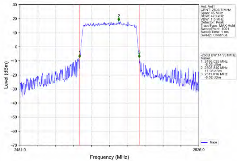
Band41_15MHz_16QAM_LCH_2503.5MHz_RB_75_0_NTNV
