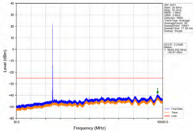
Band41_15MHz_16QAM_LCH_2503.5MHz_RB_1_0_NTNV
