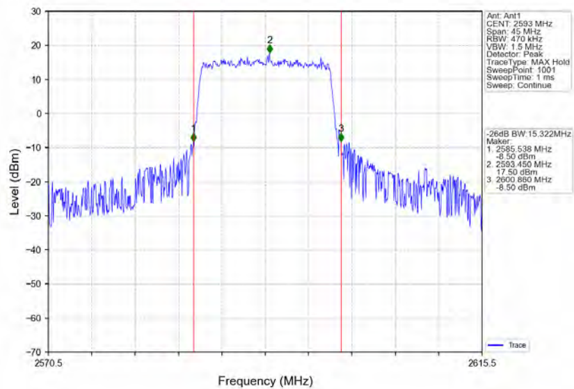
Band41_15MHz_64QAM_MCH_2593MHz_RB_75_0_NTNV
