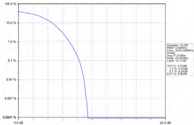
Band41_5MHz_64QAM_MCH_2593MHz_RB_25_0_NTNV
