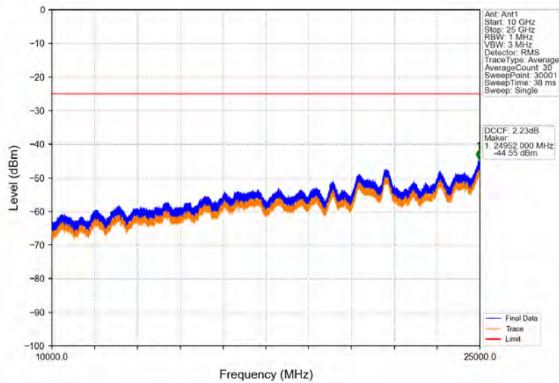
Band41_5MHz_64QAM_LCH_2498.5MHz_RB_1_0_NTNV
