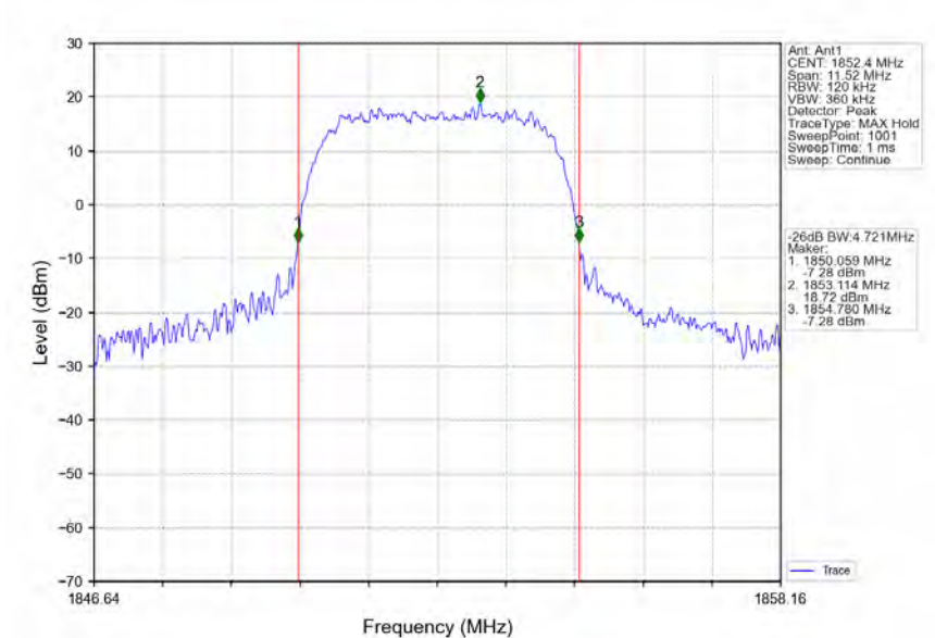
Band2_HSDPA_LCH_1852.4MHz_Subtest 1_NTNV
