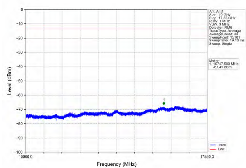
Band4_RMC_MCH_1732.6MHz_12.2kbps_RMC_NTNV
