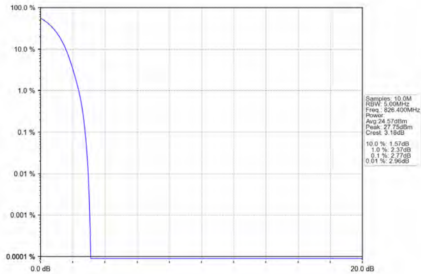
Band5_RMC_LCH_826.4MHz_12.2kbps_RMC_NTNV
