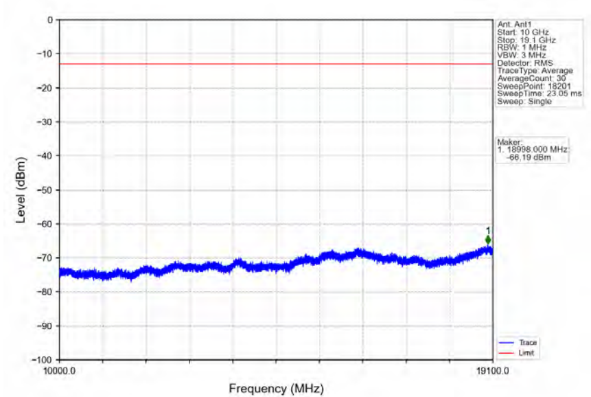
Band2_RMC_HCH_1907.6MHz_12.2kbps_RMC_NTNV
