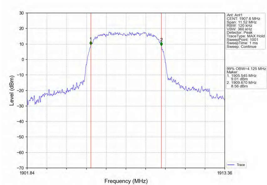
Band2 HSDPA HCH 1907.6MHz Subtest 1 NTN
