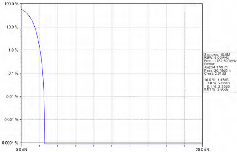
Band4_RMC_HCH_1752.6MHz_12.2kbps_RMC_NTNV
