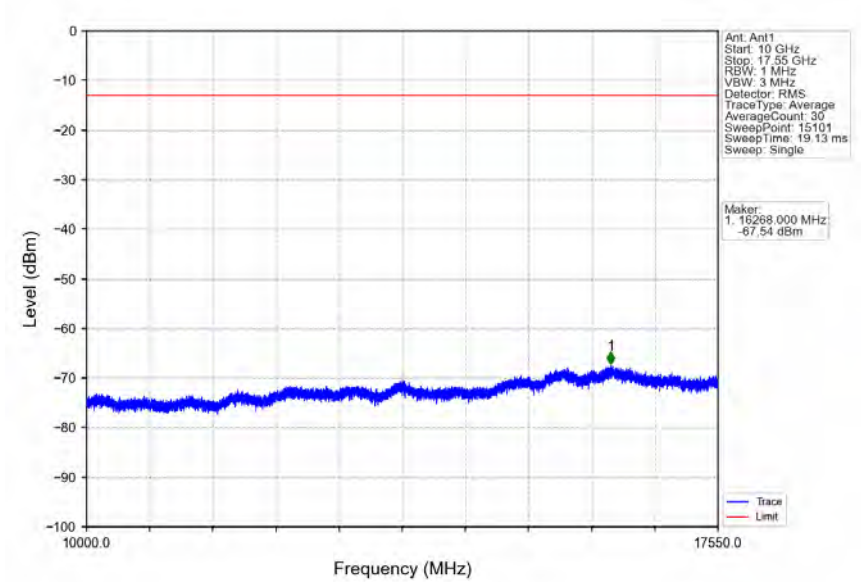
Band4_HSUPA_MCH_1732.6MHz_Subtest 1_NTNV
