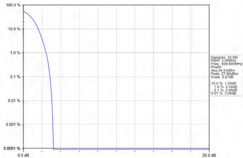
Band5_RMC_MCH_836.6MHz_12.2kbps_RMC_NTNV
