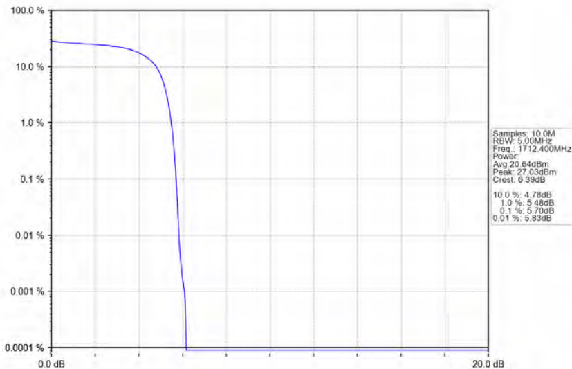
Band4_HSDPA_LCH_1712.4MHz_Subtest 1_NTNV
