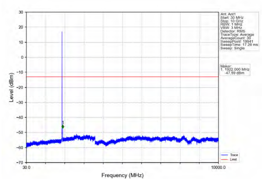
Band2 HSUPA MCH 1880MHz Subtest 1 NTN
