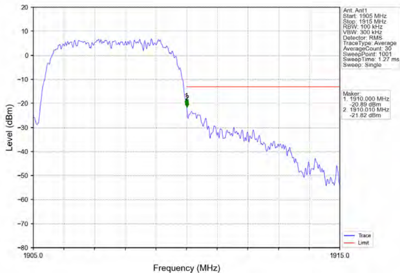
Band2 HSUPA HCH 1907.6MHz Subtest 1 NTNV
