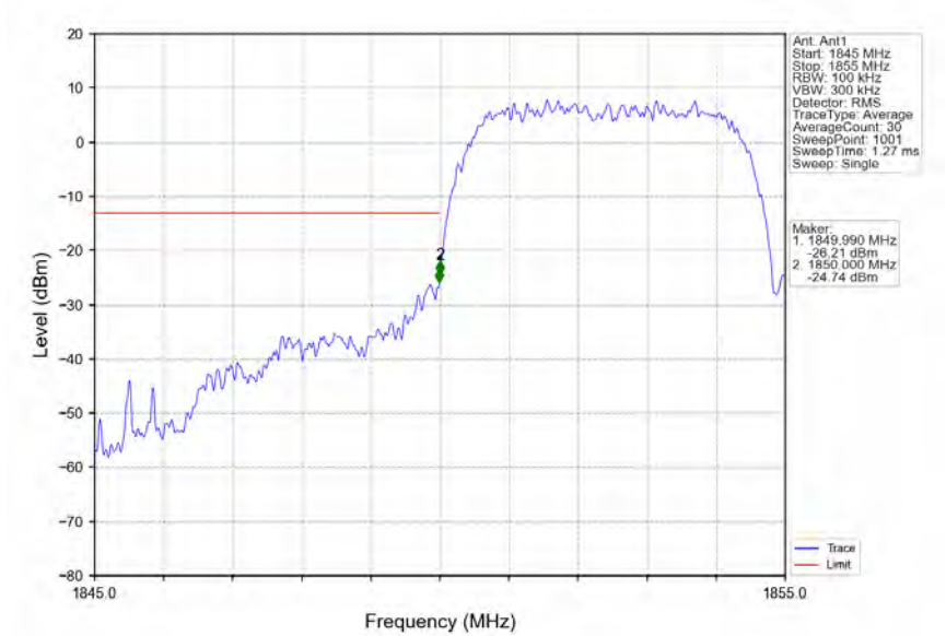
Band2_HSDPA_LCH_1852.4MHz_Subtest 1_NTNV
