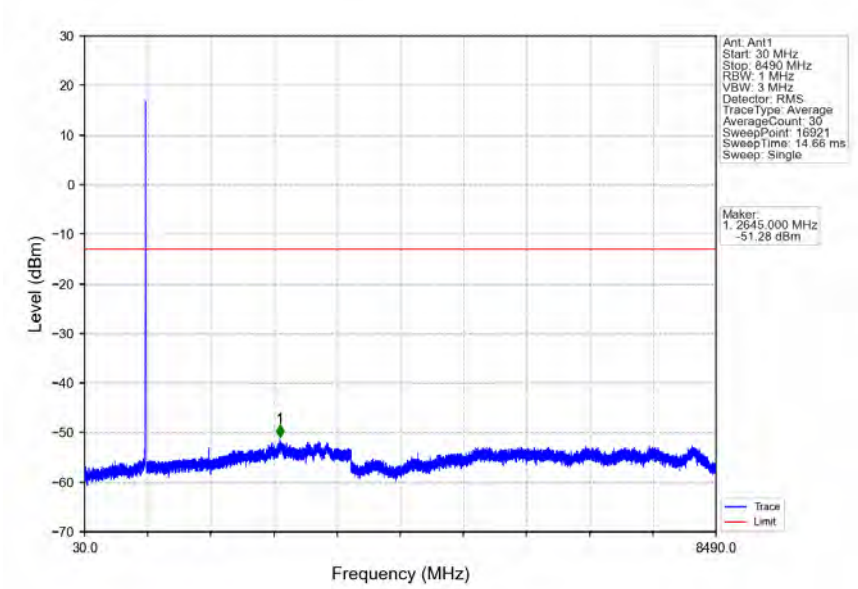
Band5 HSUPA HCH 846.6MHz Subtest 1 NTV
