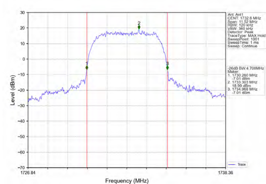
Band4_HSUPA_MCH_1732.6MHz_Subtest 1_NTNV
