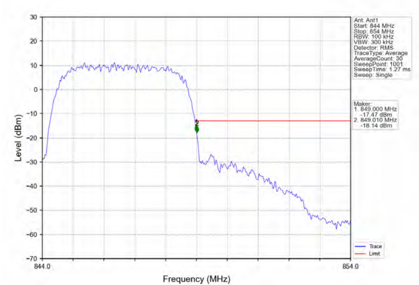
Band5 RMC HCH 846.6MHz 12.2kbps RMC NTN
