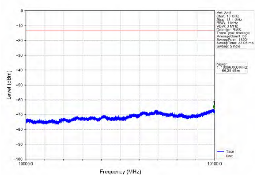
Band2_RMC_MCH_1880MHz_12.2kbps_RMC_NTNV
