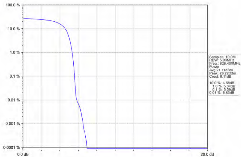
Band5 HSDPA LCH 826.4MHz Subtest 1 NTN
