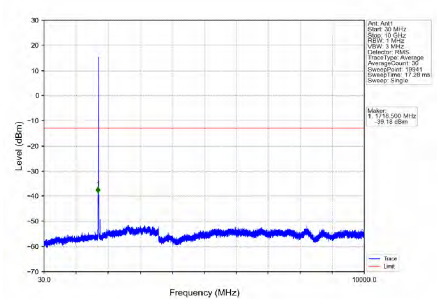
Band4_HSDPA_MCH_1732.6MHz_Subtest 1_NTNV
