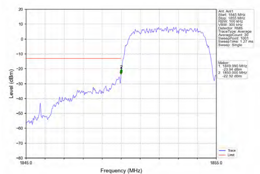
Band2 HSUPA LCH 1852.4MHz Subtest 1 NTN
