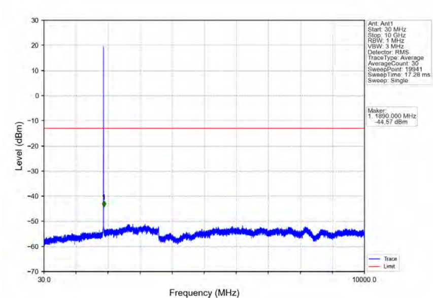
Band2_RMC_MCH_1880MHz_12.2kbps_RMC_NTNV
