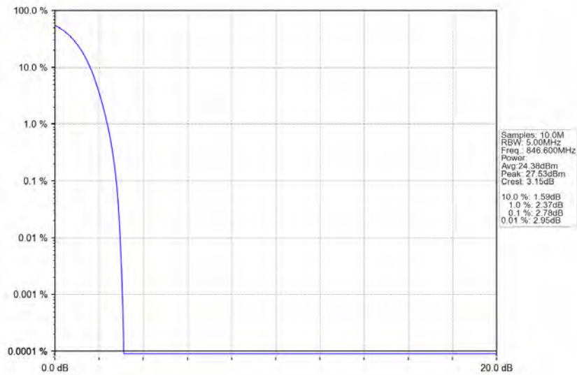
Band5 RMC HCH 846.6MHz 12.2kbps RMC NTN
