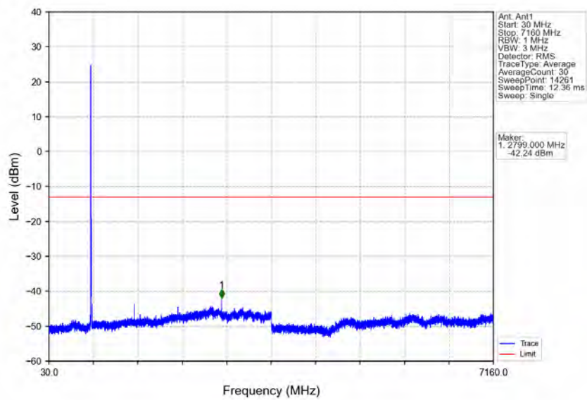
Band12_10MHz_QPSK_LCH_704MHz_RB_1_0_NTNV
