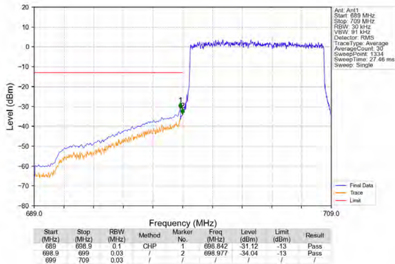
Band12_10MHz_QPSK_LCH_704MHz_RB_50_0_NTNV
