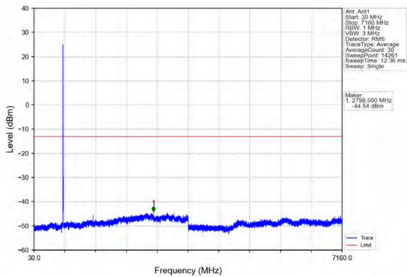
Band12_5MHz_QPSK_LCH_701.5MHz_RB_1_0_NTNV
