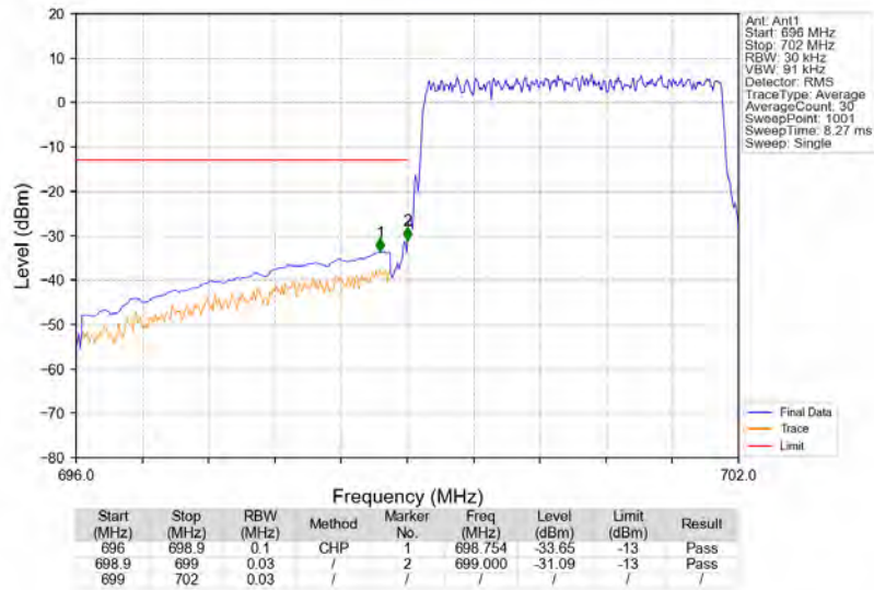
Band12_3MHz_64QAM_LCH_700.5MHz_RB_15_0_NTNV
