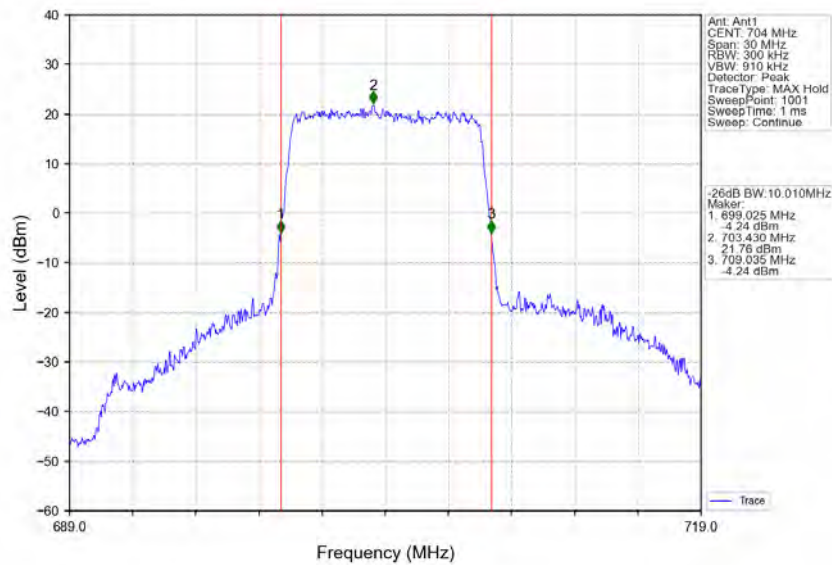
Band12_10MHz_QPSK_LCH_704MHz_RB_50_0_NTNV
