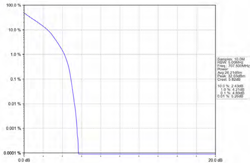
Band12_3MHz_QPSK_MCH_707.5MHz_RB_15_0_NTNV
