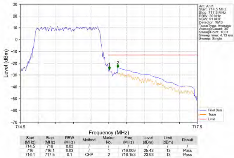
Band12_1.4MHz_16QAM_HCH_715.3MHz_RB_6_0_NTNV
