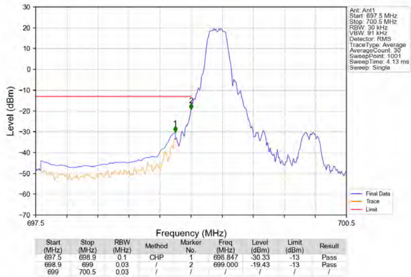
Band12_1.4MHz_QPSK_LCH_699.7MHz_RB_1_0_NTNV
