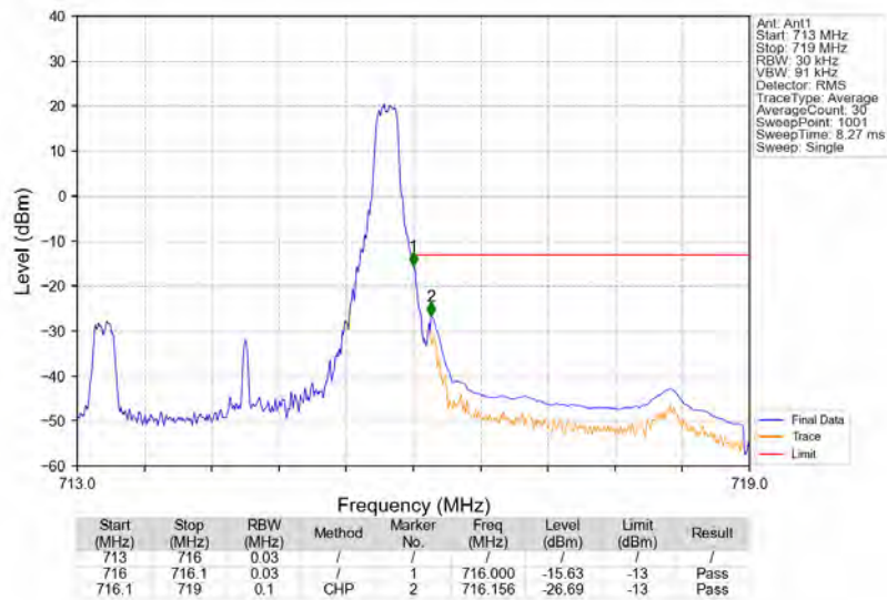
Band12_3MHz_QPSK_HCH_714.5MHz_RB_1_14_NTNV
