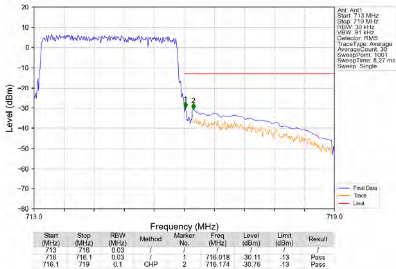
Band12_3MHz_64QAM_HCH_714.5MHz_RB_15_0_NTNV
