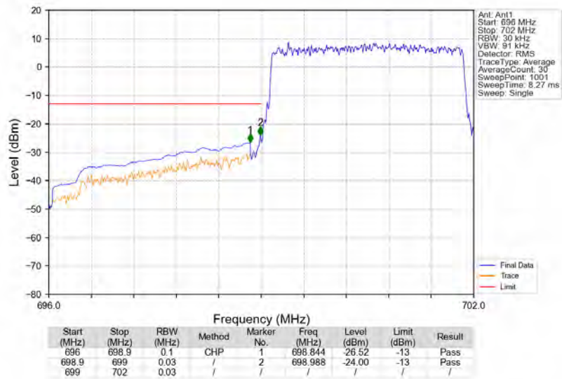
Band12_3MHz_QPSK_LCH_700.5MHz_RB_15_0_NTNV
