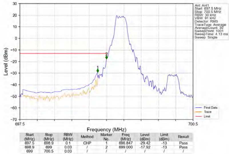
Band12_1.4MHz_16QAM_LCH_699.7MHz_RB_1_0_NTNV
