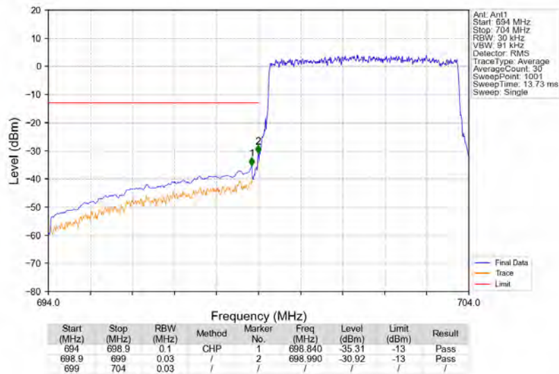
Band12_5MHz_64QAM_LCH_701.5MHz_RB_25_0_NTNV
