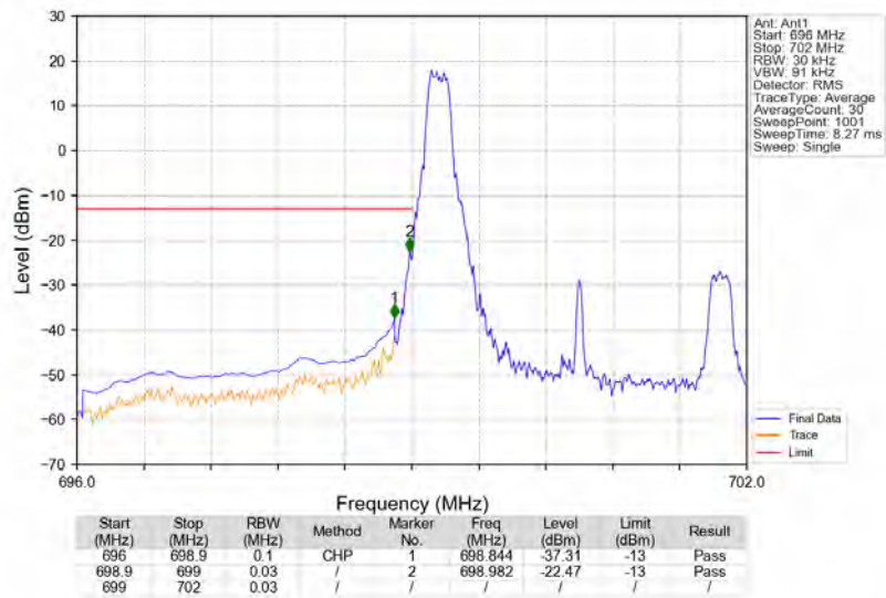
Band12_3MHz_64QAM_LCH_700.5MHz_RB_1_0_NTNV
