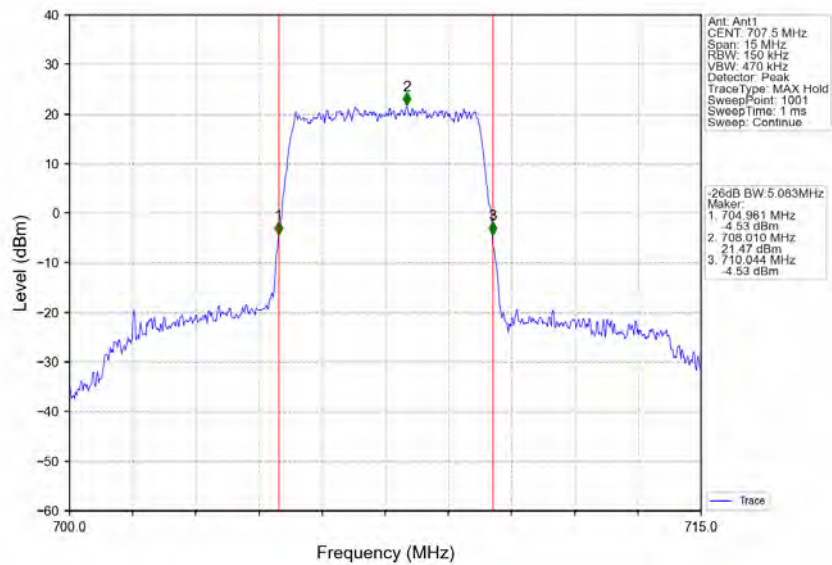
Band12_5MHz_QPSK_MCH_707.5MHz_RB_25_0_NTNV
