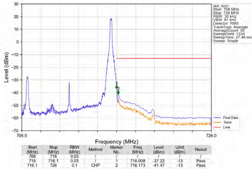
Band12_10MHz_16QAM_HCH_711MHz_RB_1_49_NTNV
