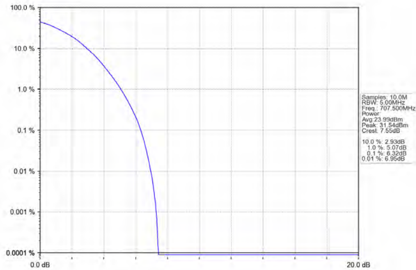
Band12_5MHz_64QAM_MCH_707.5MHz_RB_25_0_NTNV
