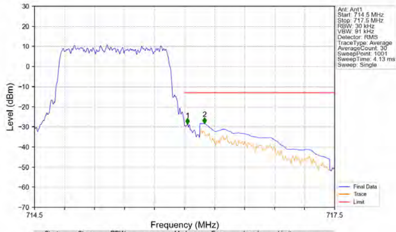
Band12_1.4MHz_64QAM_HCH_715.3MHz_RB_6_0_NTNV
