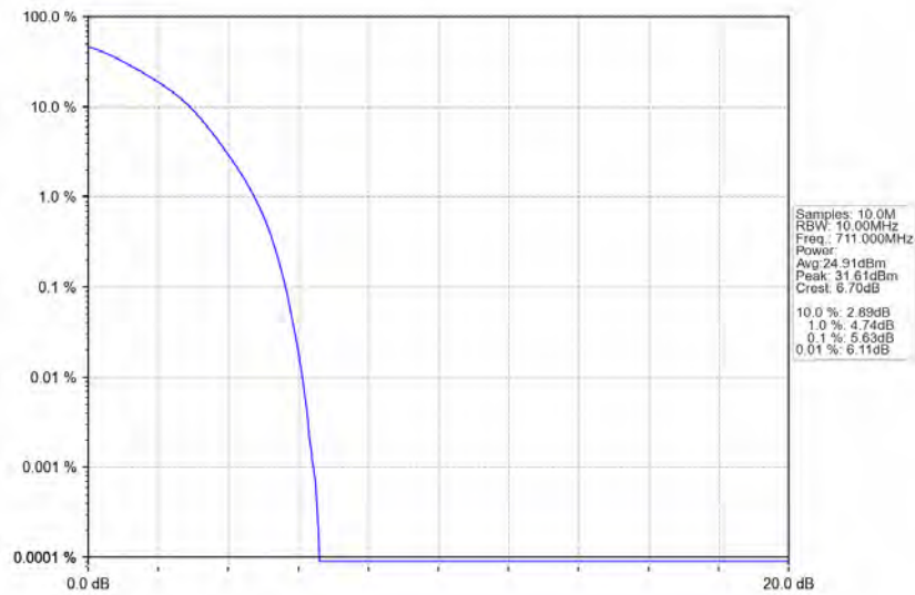
Band12_10MHz_16QAM_HCH_711MHz_RB_50_0_NTNV
