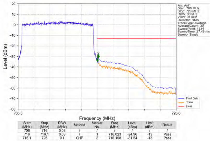
Band12_10MHz_QPSK_HCH_711MHz_RB_50_0_NTNV
