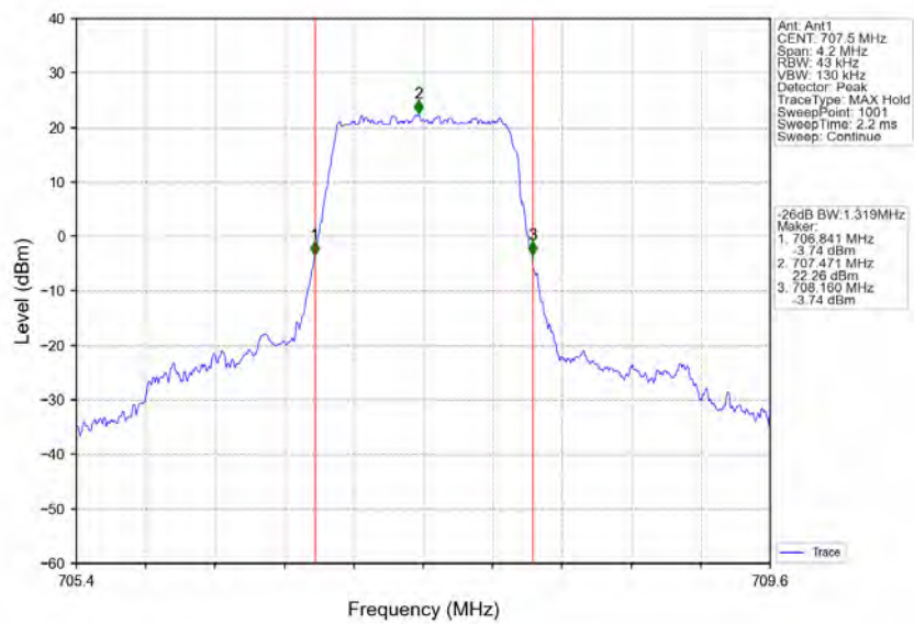
Band12_1.4MHz_QPSK_MCH_707.5MHz_RB_6_0_NTNV
