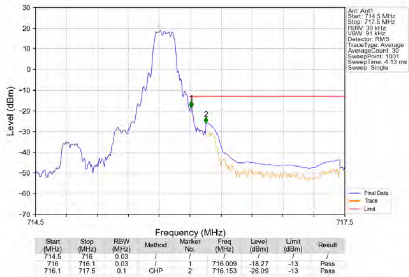
Band12_1.4MHz_16QAM_HCH_715.3MHz_RB_1_5_NTNV
