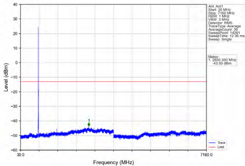
Band12_5MHz_16QAM_HCH_713.5MHz_RB_1_0_NTNV
