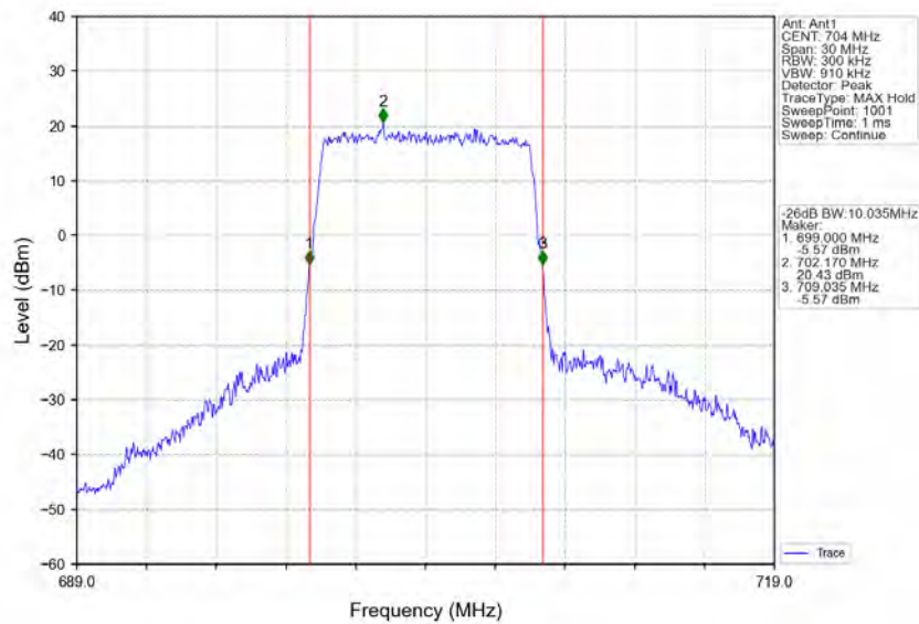
Band12_10MHz_64QAM_LCH_704MHz_RB_50_0_NTNV
