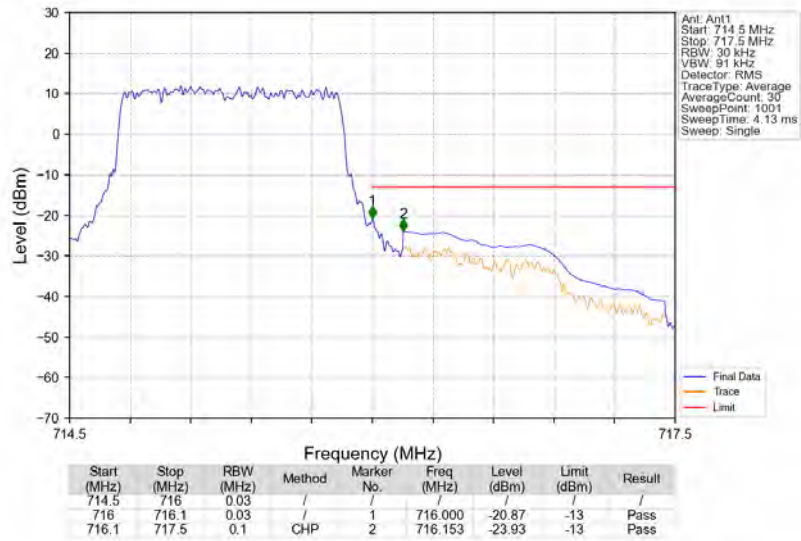
Band12_1.4MHz_QPSK_HCH_715.3MHz_RB_6_0_NTNV
