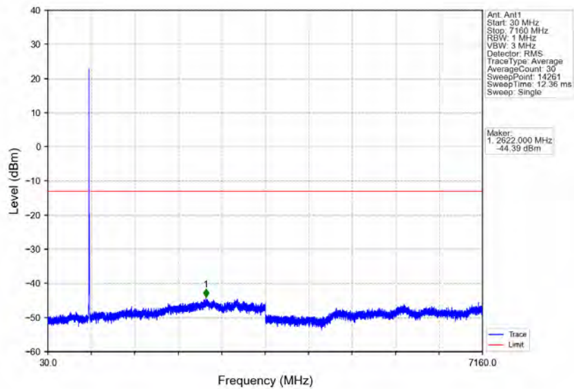
Band12_10MHz_64QAM_MCH_707.5MHz_RB_1_0_NTNV
