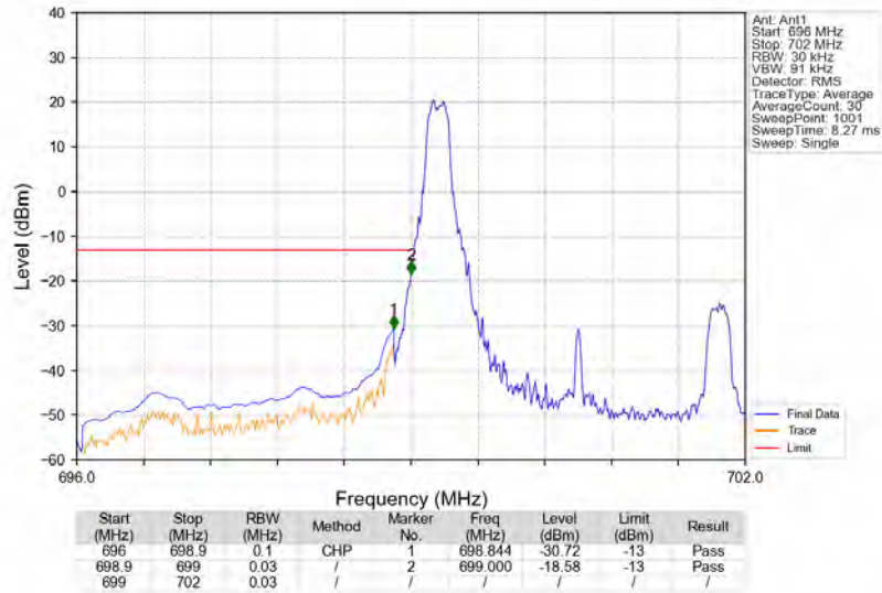
Band12_3MHz_QPSK_LCH_700.5MHz_RB_1_0_NTNV
