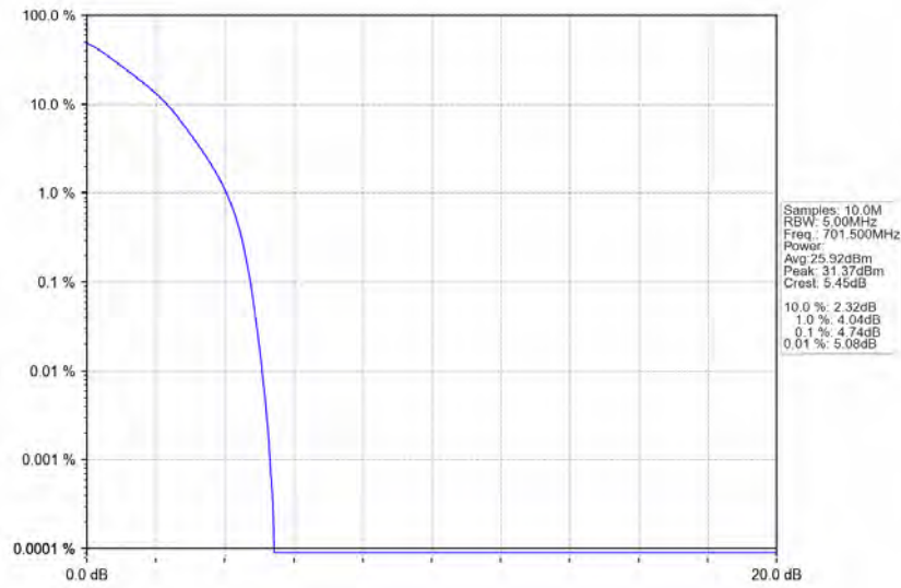
Band12_5MHz_QPSK_LCH_701.5MHz_RB_25_0_NTNV
