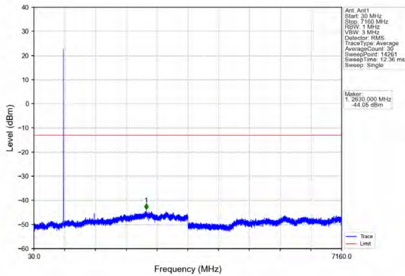
Band12_3MHz_64QAM_HCH_714.5MHz_RB_1_14_NTNV
