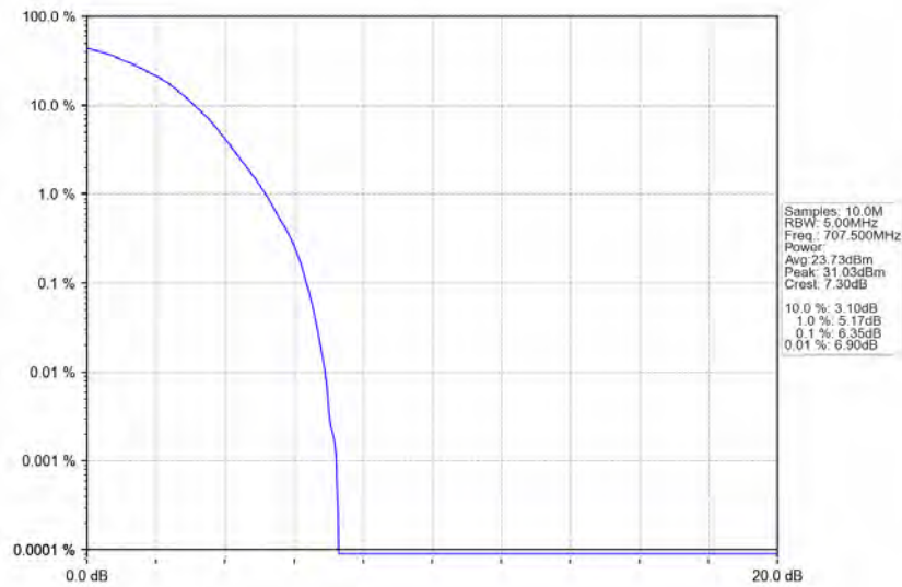
Band12_1.4MHz_64QAM_MCH_707.5MHz_RB_6_0_NTNV
