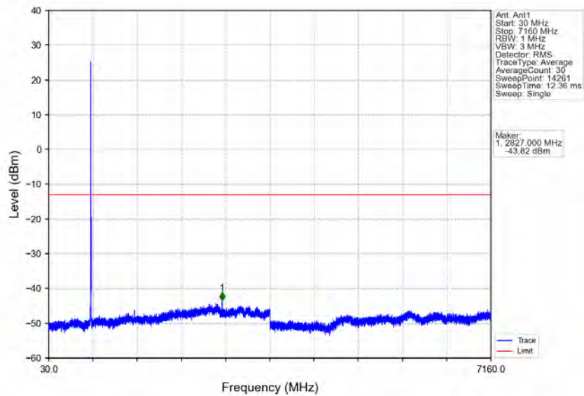
Band12_10MHz_16QAM_HCH_711MHz_RB_1_0_NTNV
