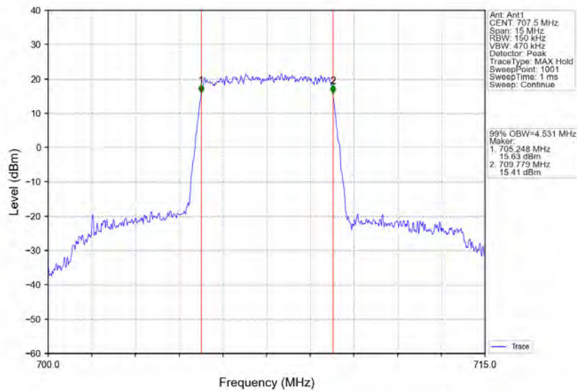
Band12_5MHz_QPSK_MCH_707.5MHz_RB_25_0_NTNV
