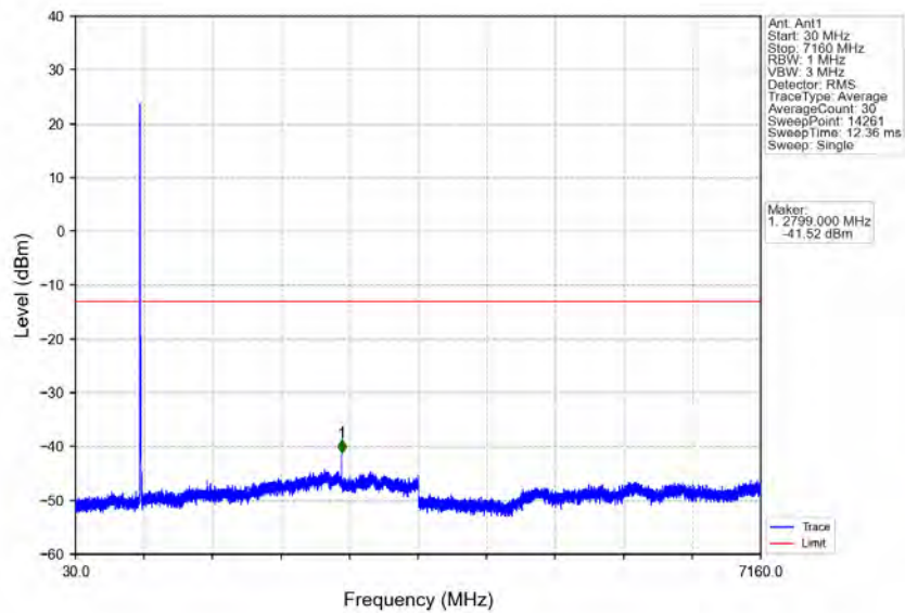
Band12_10MHz_64QAM_LCH_704MHz_RB_1_0_NTNV
