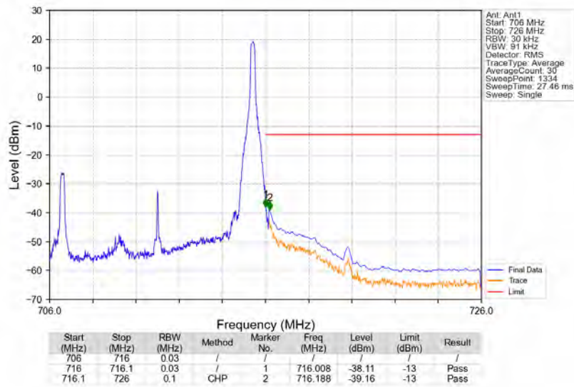
Band12_10MHz_QPSK_HCH_711MHz_RB_1_49_NTNV
