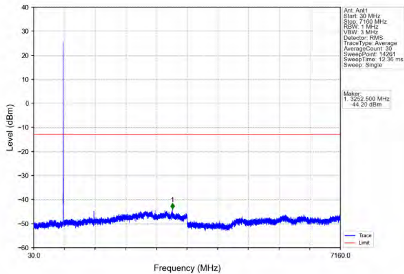
Band12_3MHz_QPSK_HCH_714.5MHz_RB_1_14_NTNV
