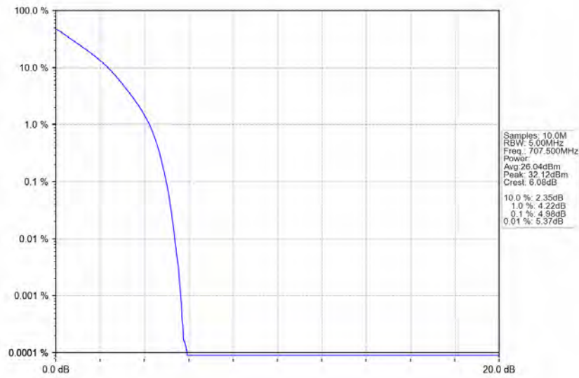
Band12_5MHz_QPSK_MCH_707.5MHz_RB_25_0_NTNV
