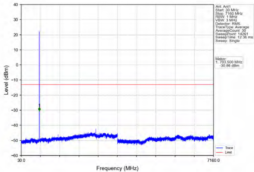
Band12_1.4MHz_64QAM_LCH_699.7MHz_RB_1_0_NTNV
