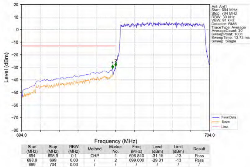
Band12_5MHz_QPSK_LCH_701.5MHz_RB_25_0_NTNV
