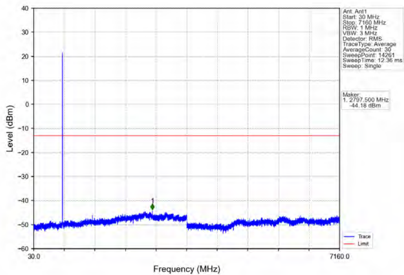
Band12_3MHz_64QAM_LCH_700.5MHz_RB_1_0_NTNV
