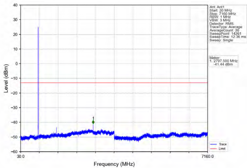
Band12_3MHz_QPSK_LCH_700.5MHz_RB_1_0_NTNV
