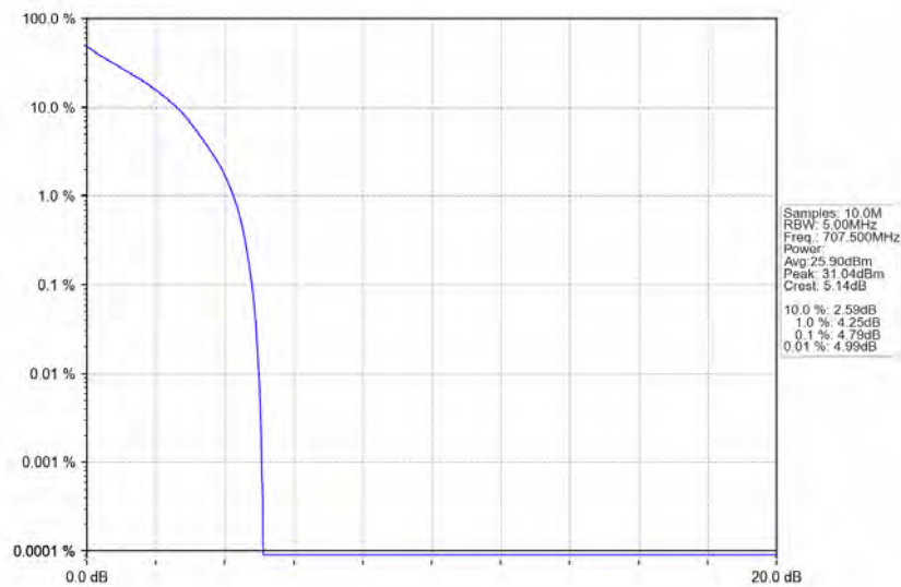
Band12_1.4MHz_QPSK_MCH_707.5MHz_RB_6_0_NTNV
