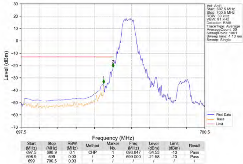
Band12_1.4MHz_64QAM_LCH_699.7MHz_RB_1_0_NTNV
