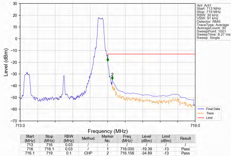
Band12_3MHz_64QAM_HCH_714.5MHz_RB_1_14_NTNV
