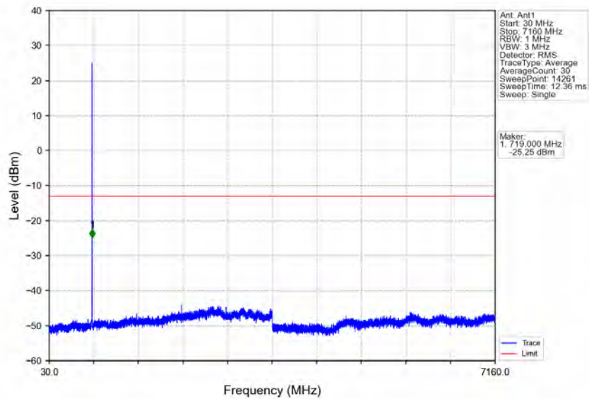
Band12_1.4MHz_QPSK_HCH_715.3MHz_RB_1_5_NTNV
