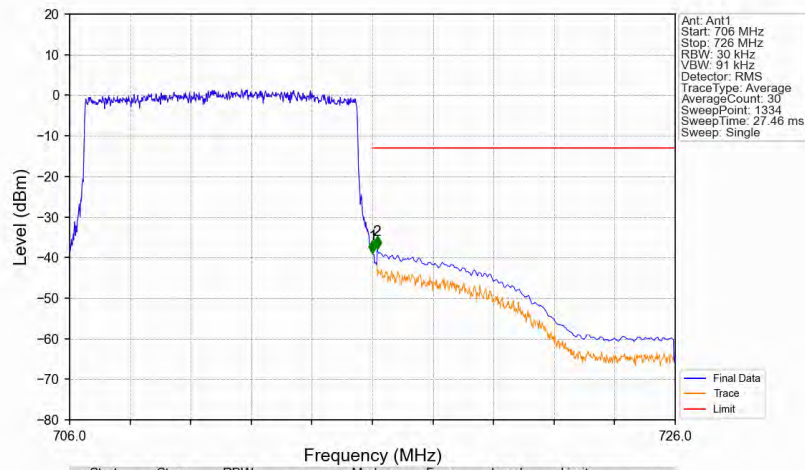
Band12_10MHz_64QAM_HCH_711MHz_RB_50_0_NTNV
