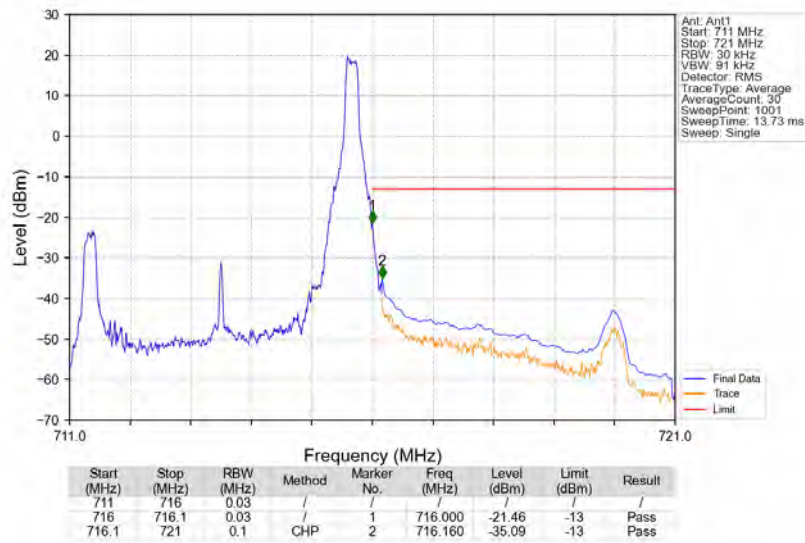
Band12_5MHz_QPSK_HCH_713.5MHz_RB_1_24_NTNV
