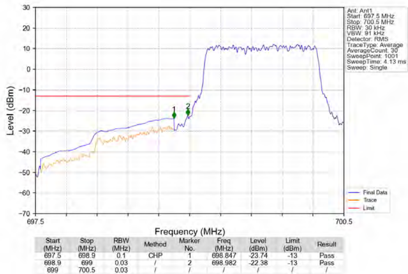
Band12_1.4MHz_QPSK_LCH_699.7MHz_RB_6_0_NTNV
