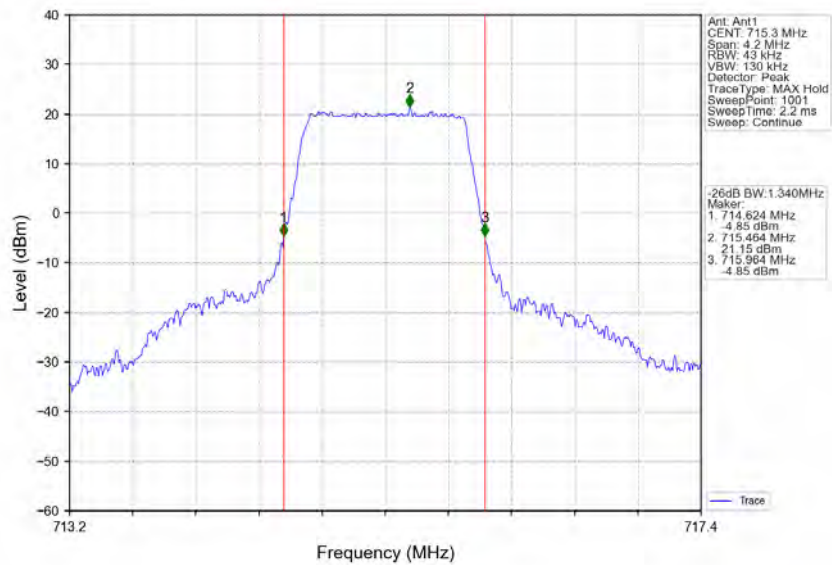
Band12_1.4MHz_16QAM_HCH_715.3MHz_RB_6_0_NTNV
