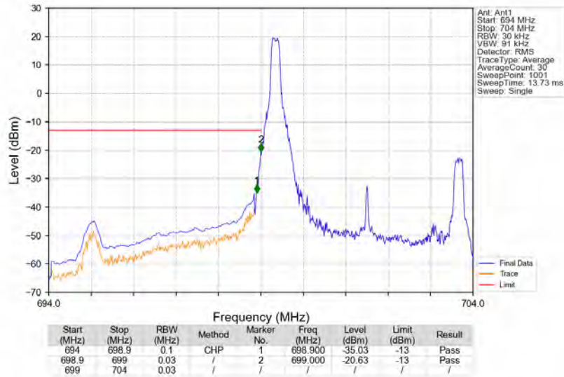
Band12_5MHz_QPSK_LCH_701.5MHz_RB_1_0_NTNV
