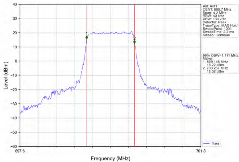
Band12_1.4MHz_16QAM_LCH_699.7MHz_RB_6_0_NTNV
