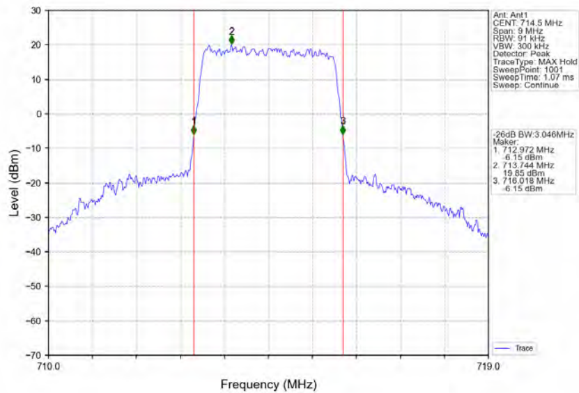
Band12_3MHz_64QAM_HCH_714.5MHz_RB_15_0_NTNV
