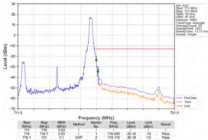
Band12_5MHz_64QAM_HCH_713.5MHz_RB_1_24_NTNV
