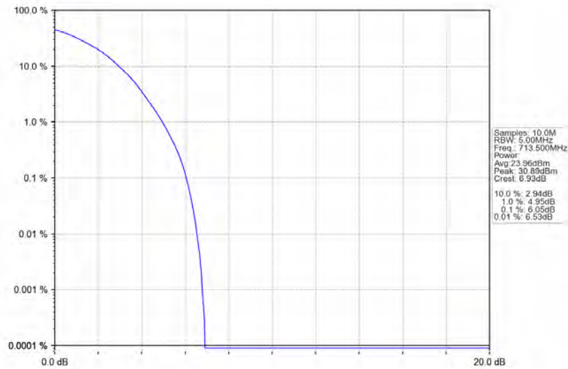
Band12_5MHz_64QAM_HCH_713.5MHz_RB_25_0_NTNV
