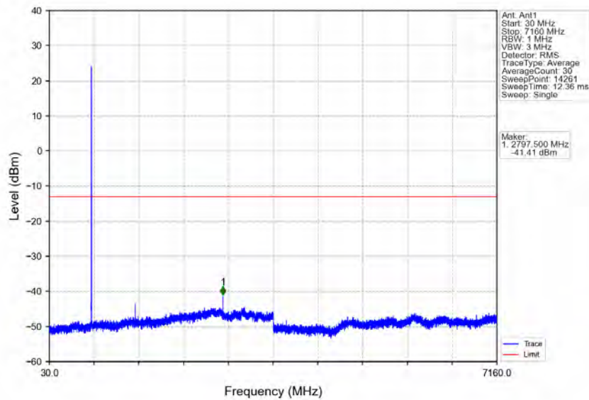
Band12_3MHz_16QAM_LCH_700.5MHz_RB_15_0_NTNV
