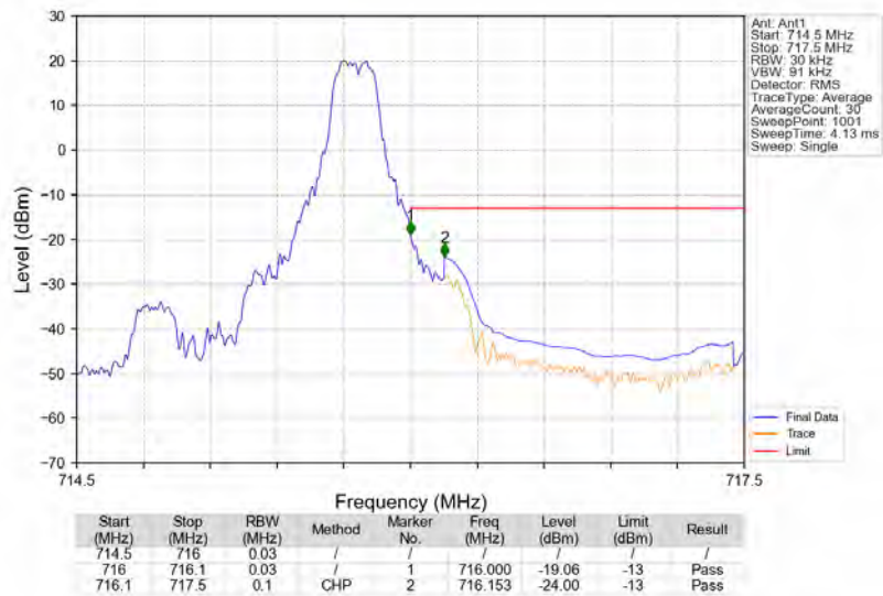
Band12_1.4MHz_QPSK_HCH_715.3MHz_RB_1_5_NTNV
