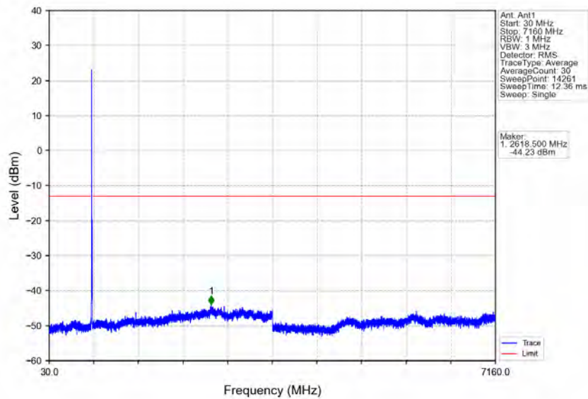
Band12_10MHz_64QAM_HCH_711MHz_RB_1_49_NTNV
