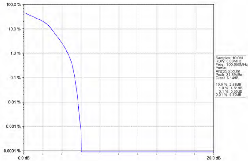
Band12_3MHz_16QAM_LCH_700.5MHz_RB_15_0_NTNV
