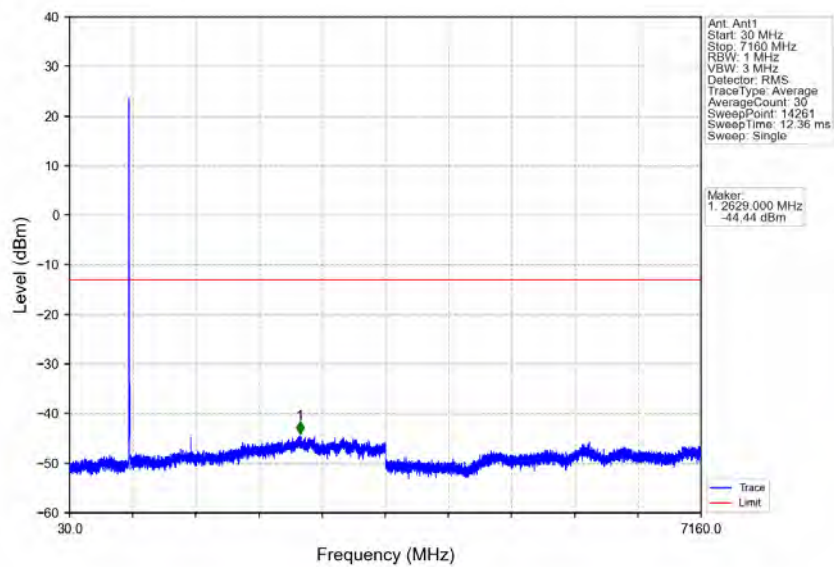
Band12_5MHz_64QAM_LCH_701.5MHz_RB_1_0_NTNV
