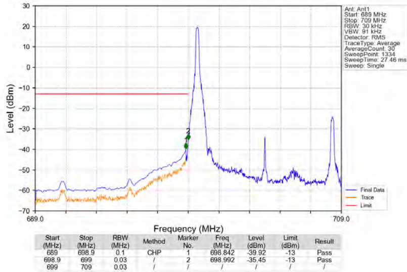
Band12_10MHz_QPSK_LCH_704MHz_RB_1_0_NTNV
