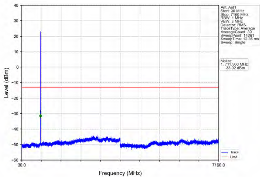
Band12_1.4MHz_64QAM_MCH_707.5MHz_RB_1_0_NTNV
