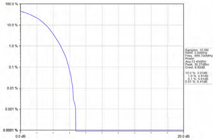
Band12_1.4MHz_64QAM_LCH_699.7MHz_RB_6_0_NTNV
