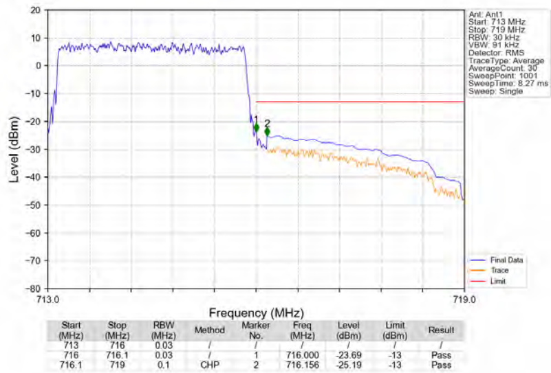
Band12_3MHz_QPSK_HCH_714.5MHz_RB_15_0_NTNV
