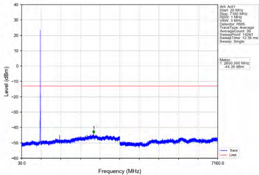
Band12_5MHz_64QAM_MCH_707.5MHz_RB_1_0_NTNV
