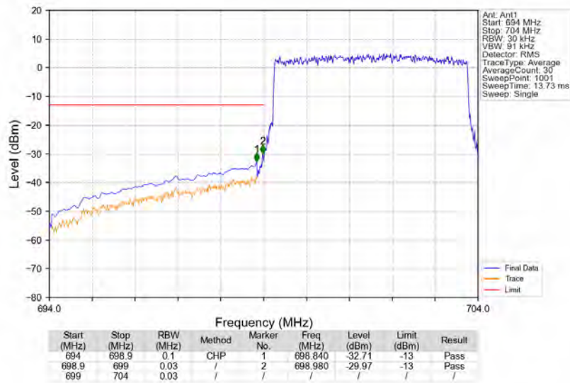
Band12_5MHz_16QAM_LCH_701.5MHz_RB_25_0_NTNV
