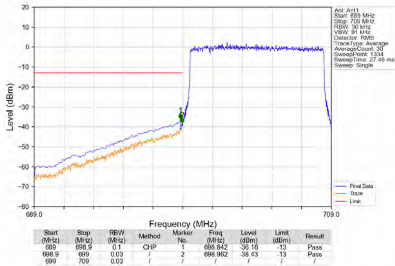
Band12_10MHz_64QAM_LCH_704MHz_RB_50_0_NTNV
