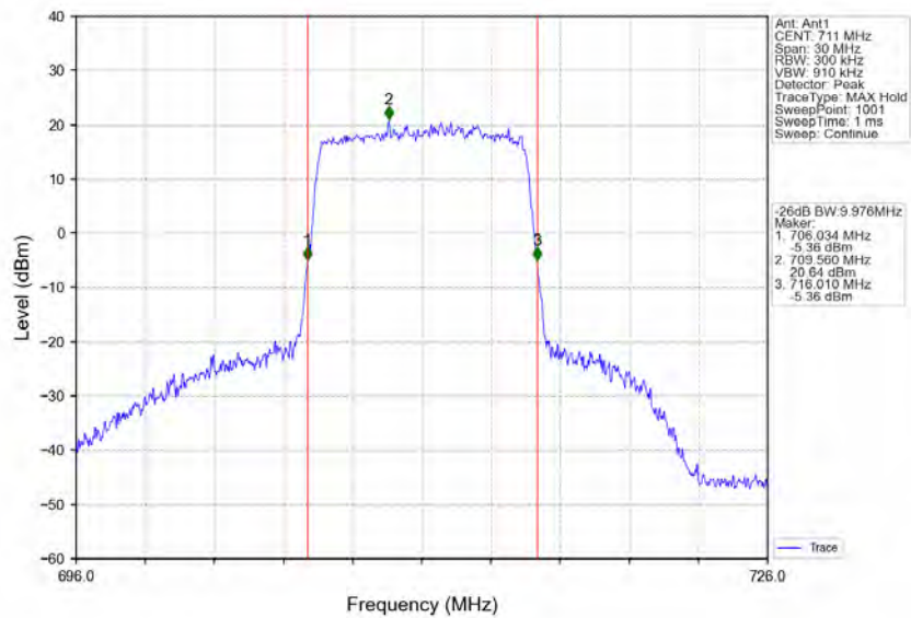
Band12_10MHz_64QAM_HCH_711MHz_RB_50_0_NTNV
