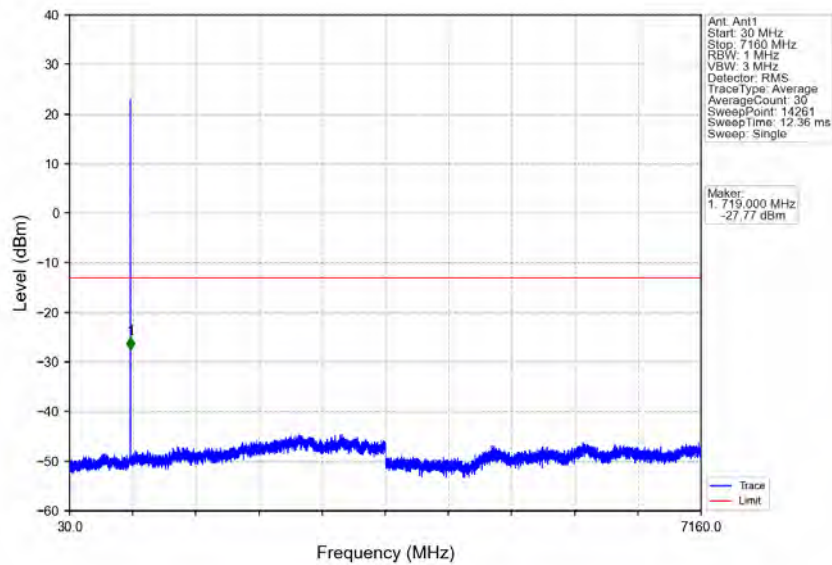
Band12_1.4MHz_64QAM_HCH_715.3MHz_RB_1_5_NTNV
