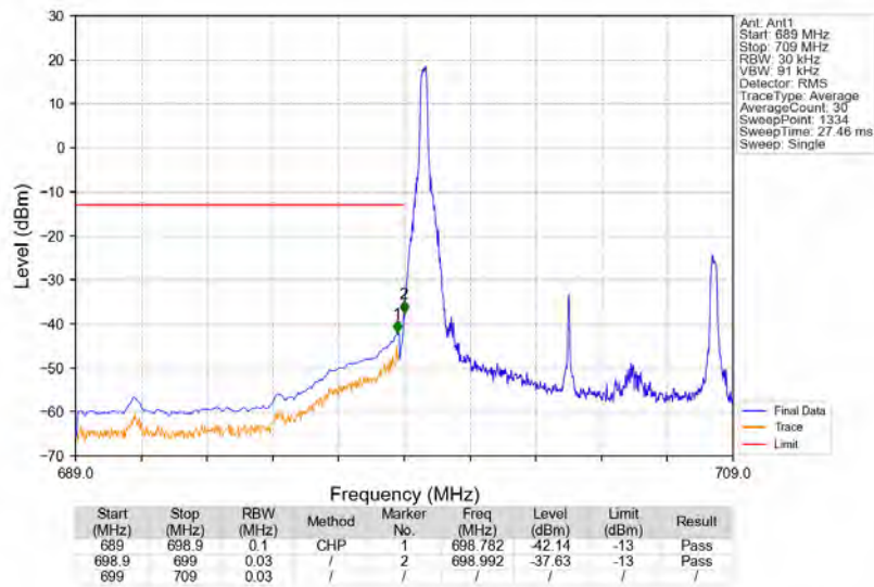
Band12_10MHz_16QAM_LCH_704MHz_RB_1_0_NTNV
