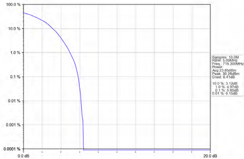
Band12_1.4MHz_64QAM_HCH_715.3MHz_RB_6_0_NTNV
