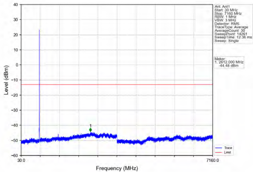
Band12_3MHz_64QAM_MCH_707.5MHz_RB_1_0_NTNV
