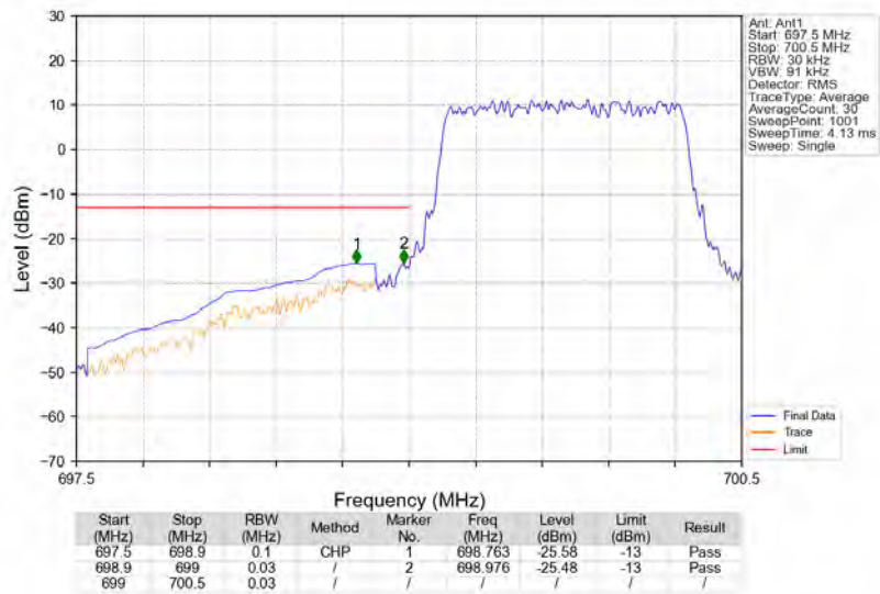
Band12_1.4MHz_16QAM_LCH_699.7MHz_RB_6_0_NTNV
