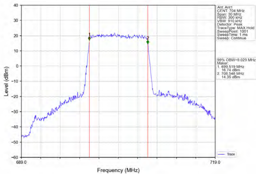
Band12_10MHz_QPSK_LCH_704MHz_RB_50_0_NTNV
