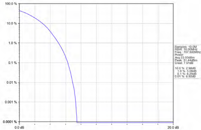
Band12_10MHz_64QAM_MCH_707.5MHz_RB_50_0_NTNV
