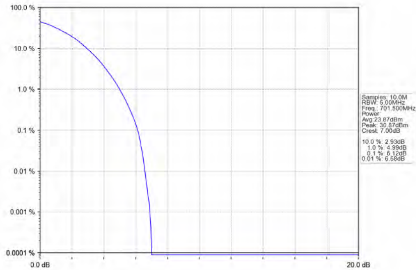
Band12_5MHz_64QAM_LCH_701.5MHz_RB_25_0_NTNV
