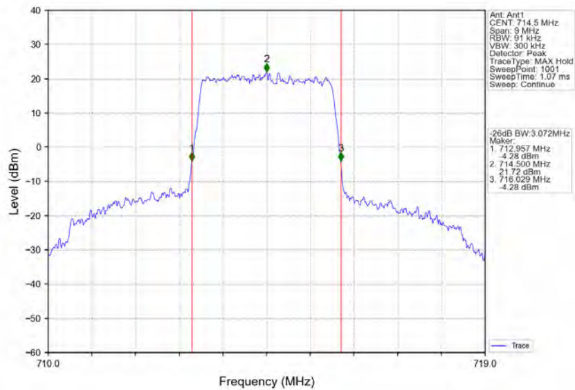
Band12_3MHz_QPSK_HCH_714.5MHz_RB_15_0_NTNV
