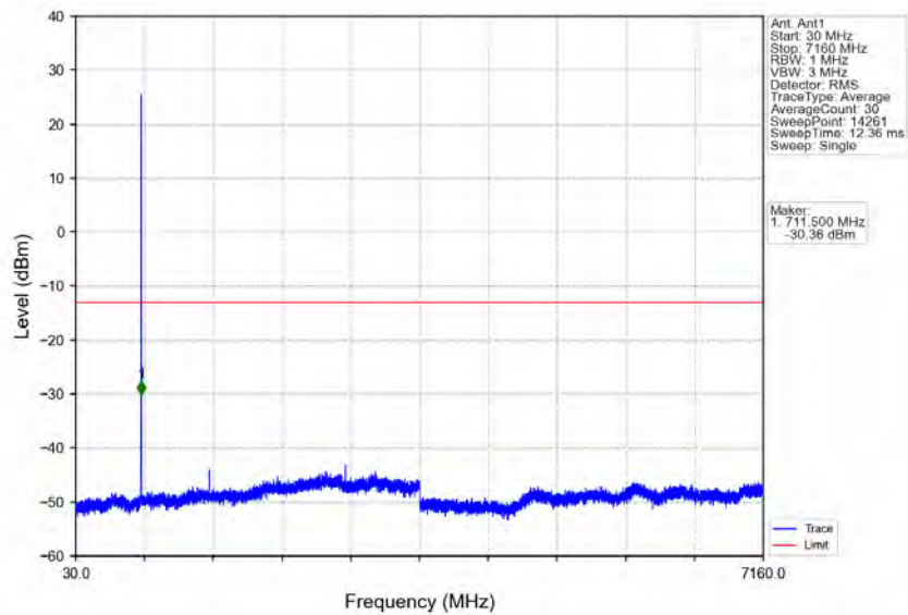
Band12_1.4MHz_QPSK_MCH_707.5MHz_RB_1_0_NTNV
