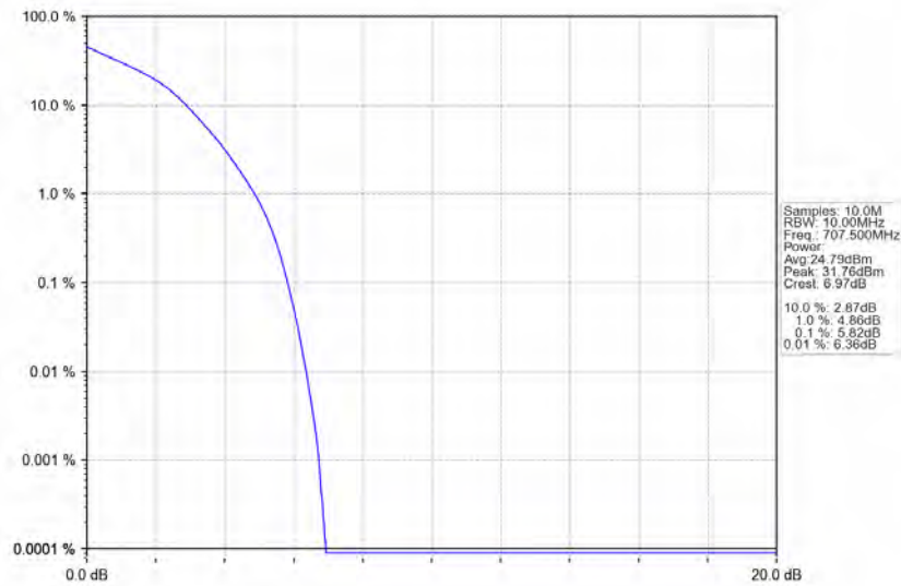
Band12_10MHz_16QAM_MCH_707.5MHz_RB_50_0_NTNV
