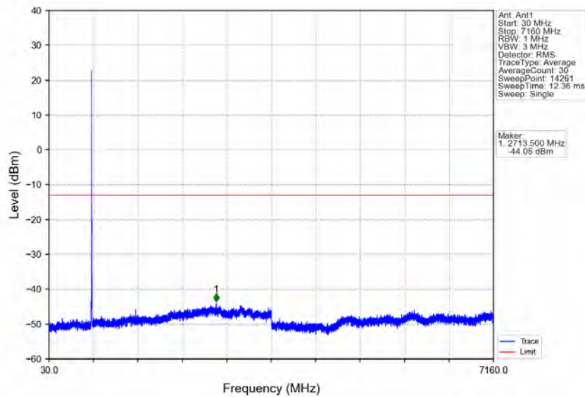
Band12_5MHz_64QAM_HCH_713.5MHz_RB_1_24_NTNV
