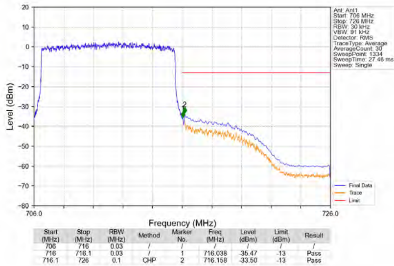
Band12_10MHz_16QAM_HCH_711MHz_RB_50_0_NTNV
