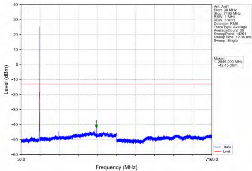
Band12_5MHz_QPSK_HCH_713.5MHz_RB_1_24_NTNV
