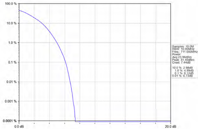
Band12_10MHz_64QAM_HCH_711MHz_RB_50_0_NTNV
