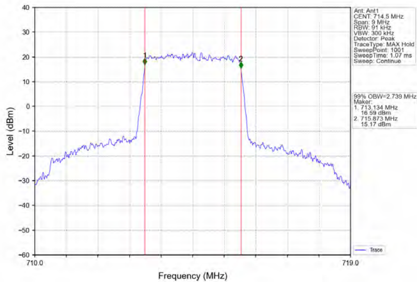
Band12_3MHz_QPSK_HCH_714.5MHz_RB_15_0_NTNV
