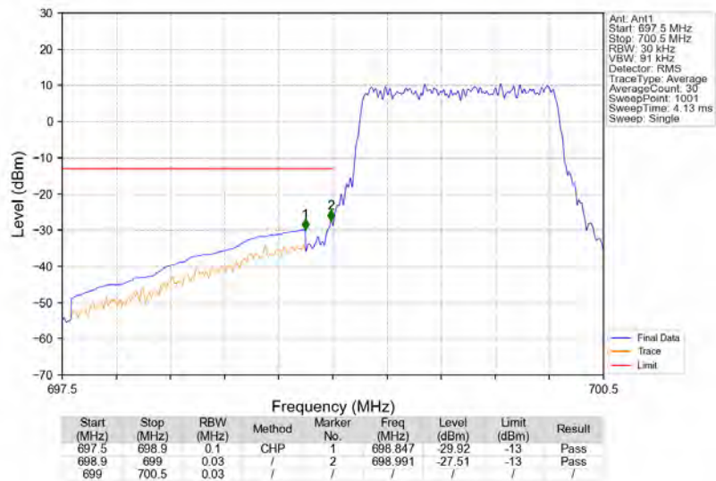
Band12_1.4MHz_64QAM_LCH_699.7MHz_RB_6_0_NTNV
