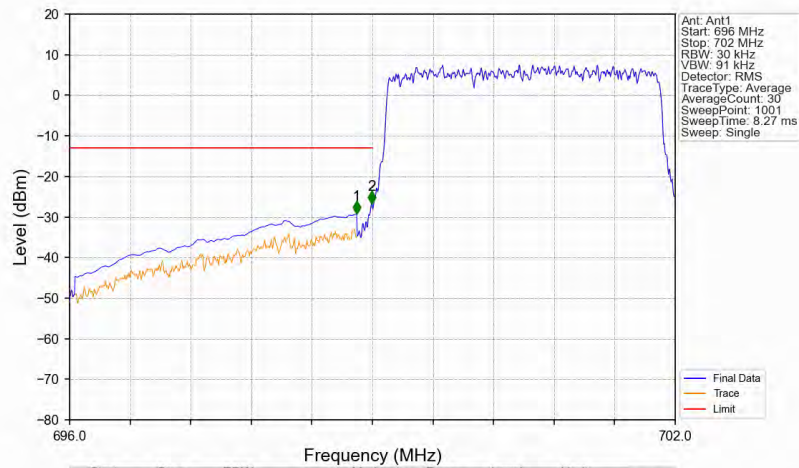
Band12_3MHz_16QAM_LCH_700.5MHz_RB_15_0_NTNV
