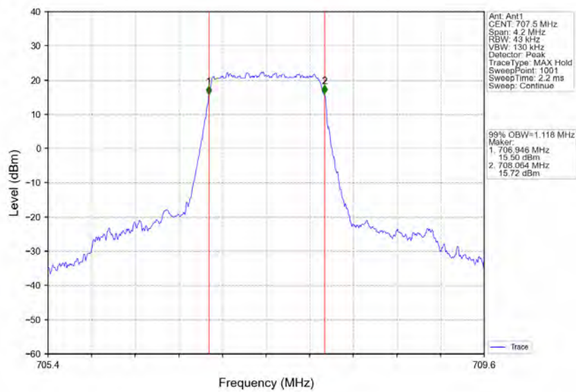
Band12_1.4MHz_QPSK_MCH_707.5MHz_RB_6_0_NTNV
