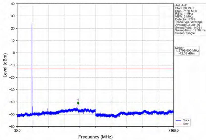
Band12_10MHz_16QAM_LCH_704MHz_RB_50_0_NTNV
