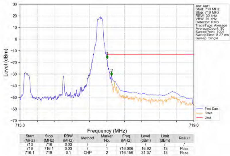
Band12_3MHz_16QAM_HCH_714.5MHz_RB_1_14_NTNV
