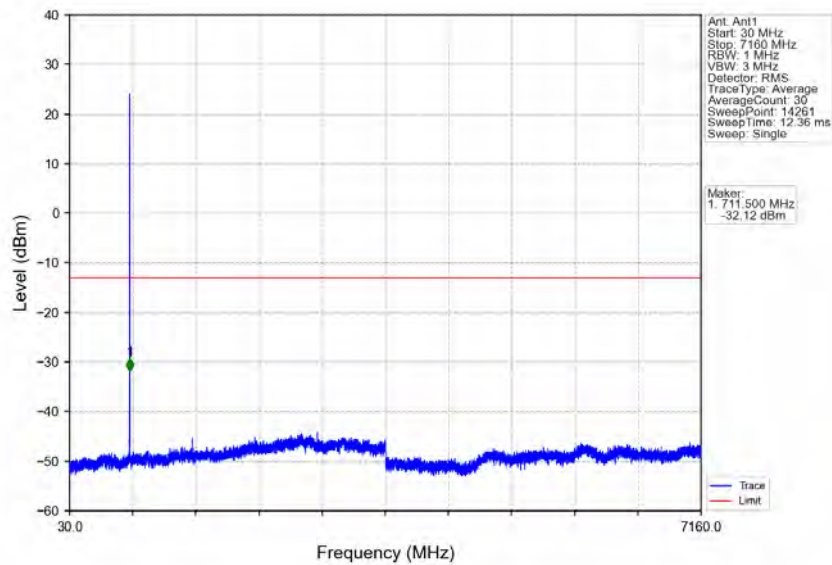
Band12_1.4MHz_16QAM_HCH_715.3MHz_RB_1_0_NTNV
