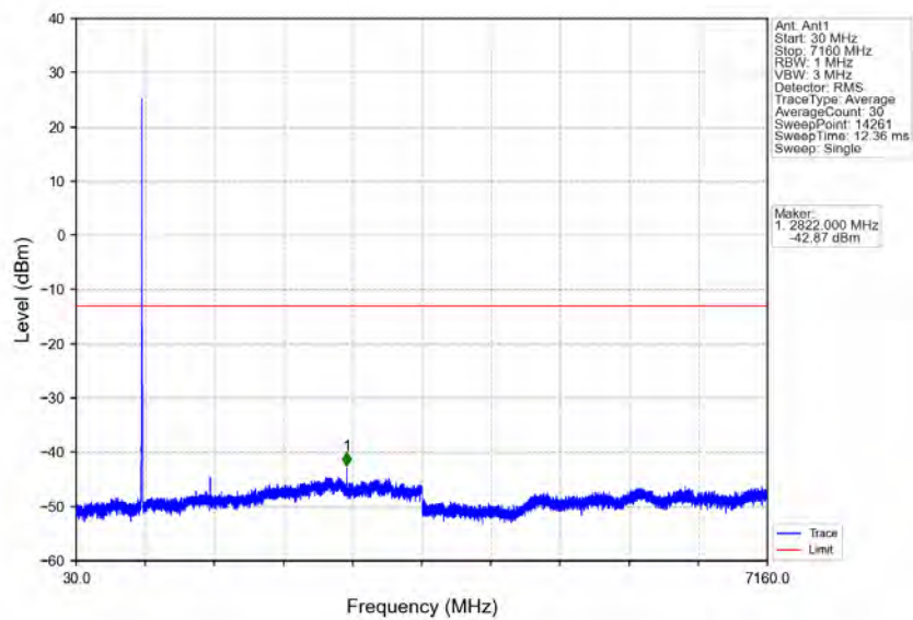
Band12_5MHz_QPSK_MCH_707.5MHz_RB_1_0_NTNV
