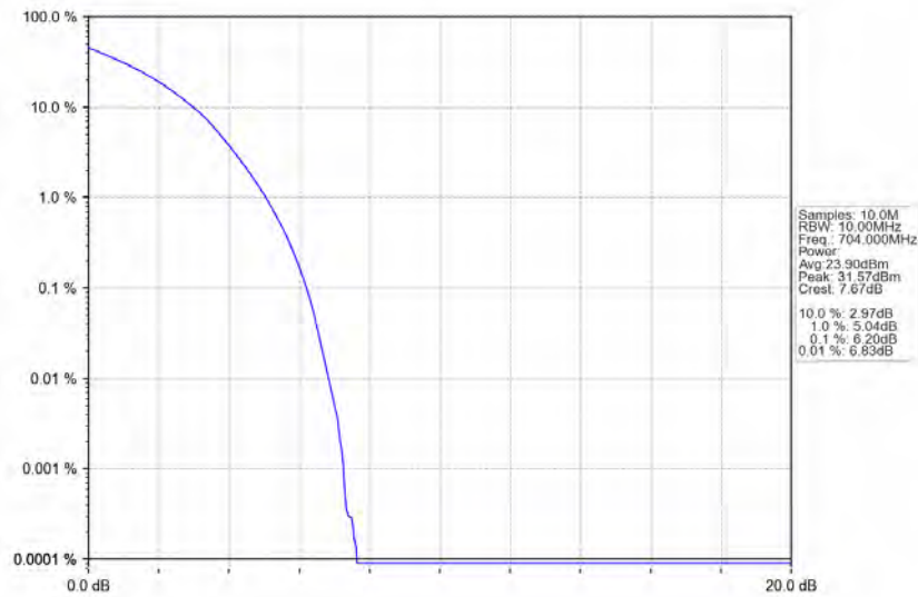
Band12_10MHz_64QAM_LCH_704MHz_RB_50_0_NTNV
