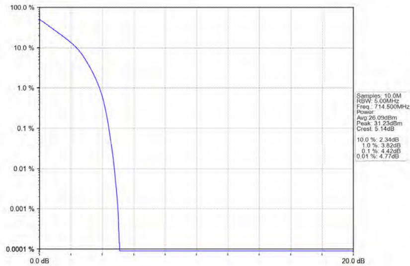
Band12_3MHz_QPSK_HCH_714.5MHz_RB_15_0_NTNV
