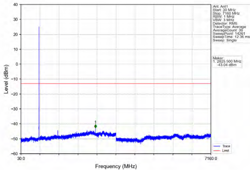
Band12_3MHz_16QAM_HCH_714.5MHz_RB_1_0_NTNV
