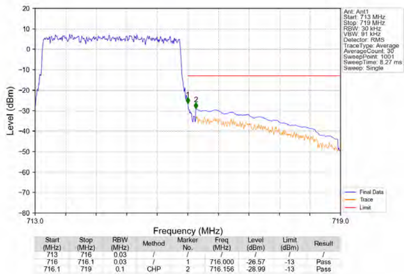
Band12_3MHz_16QAM_HCH_714.5MHz_RB_15_0_NTNV
