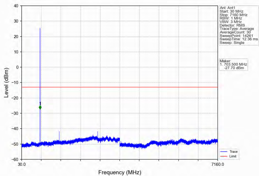
Band12_1.4MHz_QPSK_LCH_699.7MHz_RB_1_0_NTNV
