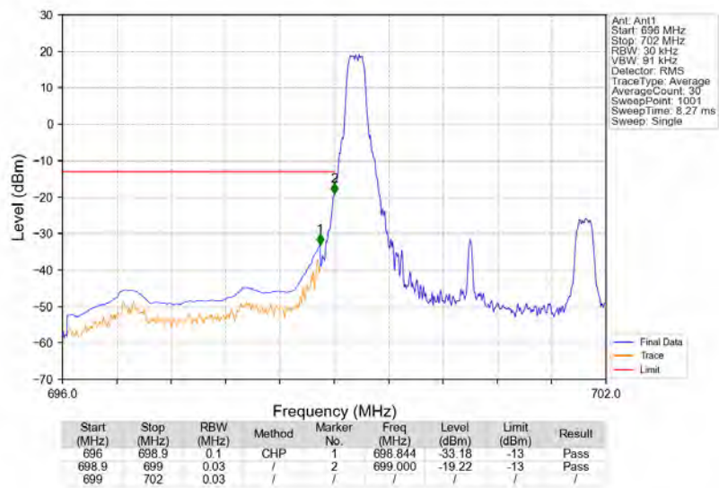
Band12_3MHz_16QAM_LCH_700.5MHz_RB_1_0_NTNV
