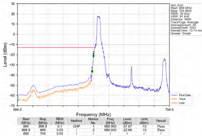
Band12_5MHz_64QAM_LCH_701.5MHz_RB_1_0_NTNV
