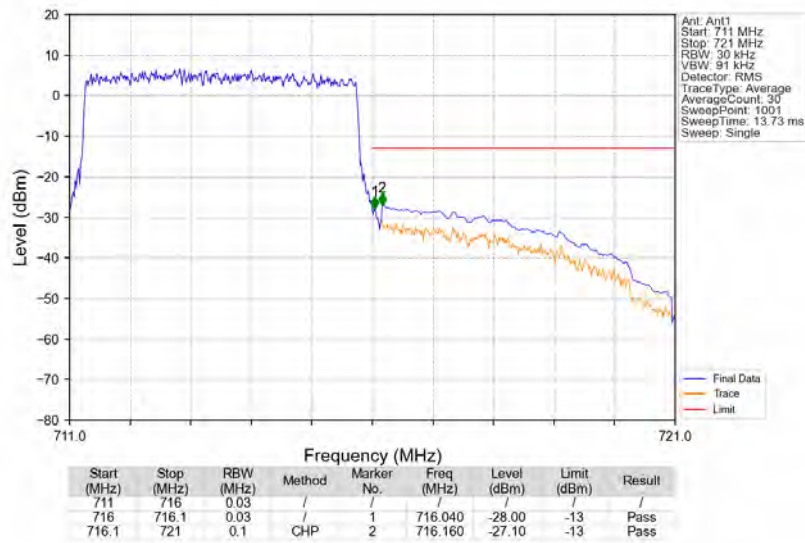
Band12_5MHz_QPSK_HCH_713.5MHz_RB_25_0_NTNV
